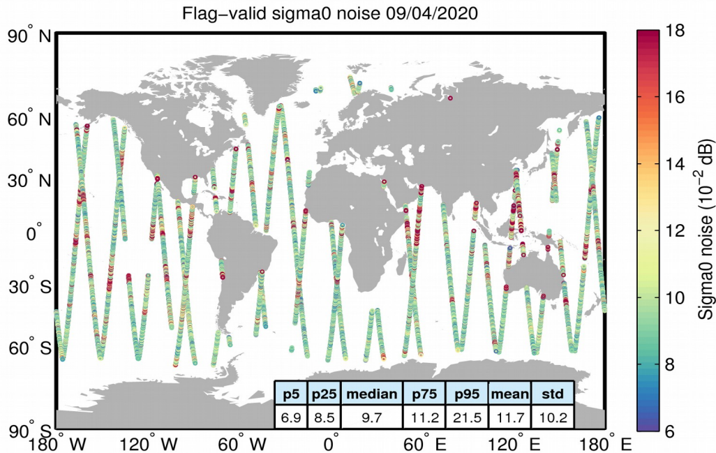
Figure 26. Geographical distribution of flag-valid 20-Hz sigma0 measurement noise over oceans and lakes for 09/04/2020. The statistical values shown in the table refer to the sigma0 noise and are calculated over all measurements shown in the figure.
