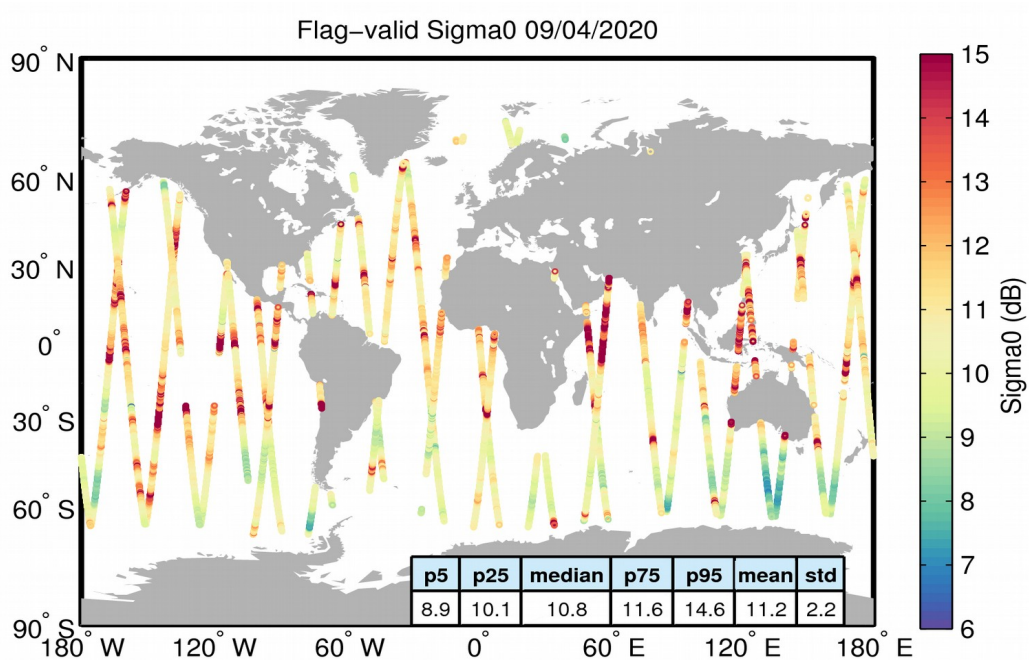
Figure 23. Geographical distribution of flag-valid sigma0 data over oceans and lakes for 09/04/2020. The statistical values shown in the table refer to the sigma0 in dB and are calculated over all measurements shown in the figure.
