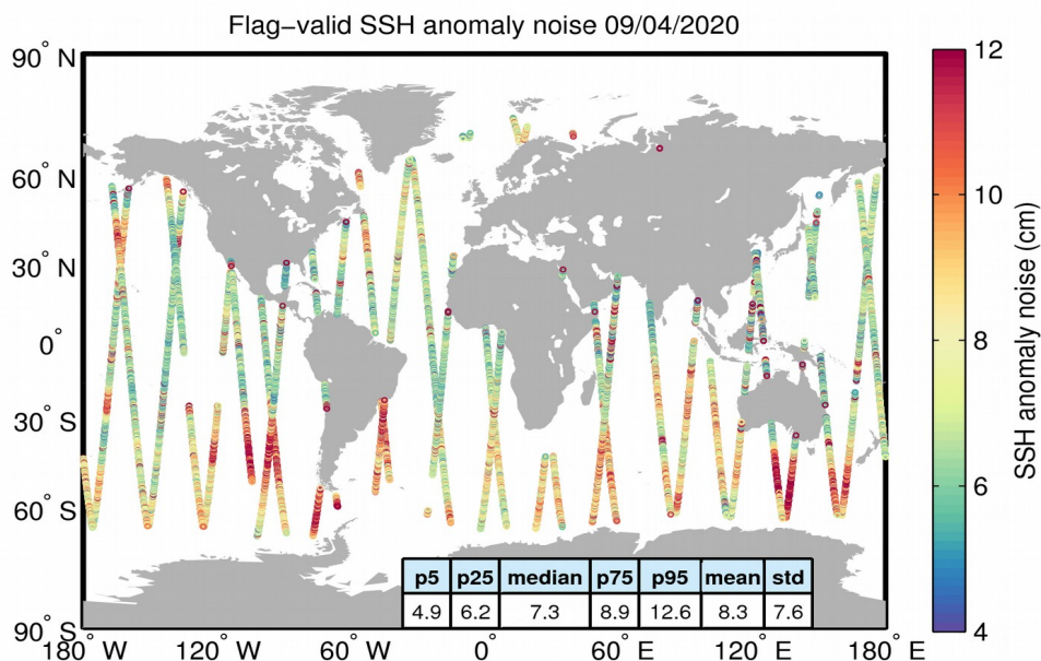
Figure 8. Geographical distribution of flag-valid 20-Hz SSH anomaly measurement noise over oceans and lakes for 09/04/2020. The statistical values shown in the table refer to the SSH anomaly noise and are calculated over all measurements shown in the figure.
