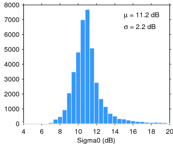
Figure 25. Histogram of flag-valid sigma0 over oceans and lakes for 09/04/2020. The mean ( \mu ) and standard deviation ( \sigma ) are also shown. Note that values outside [4 20] dB are excluded from the histogram for the sake of readability but not from the computation of \mu and \sigma .
