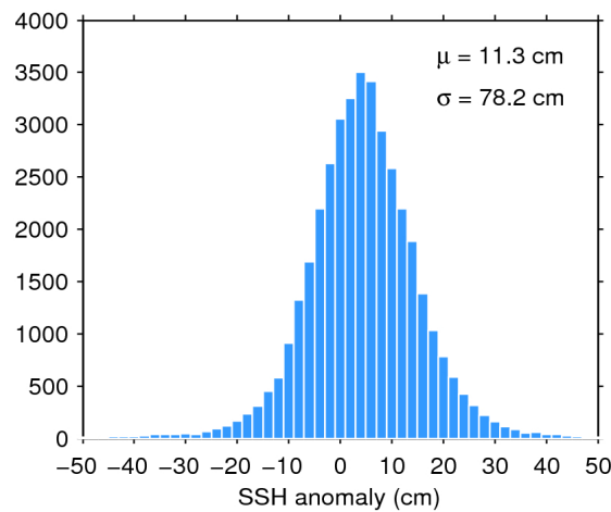
Figure 7. Histogram of flag-valid SSH anomaly over oceans and lakes for 09/04/2020. The mean ( \mu ) and standard deviation ( \sigma ) are also shown. Note that values outside [-50 50] cm are excluded from the histogram for the sake of readability but not from the computation of \mu and \sigma .
