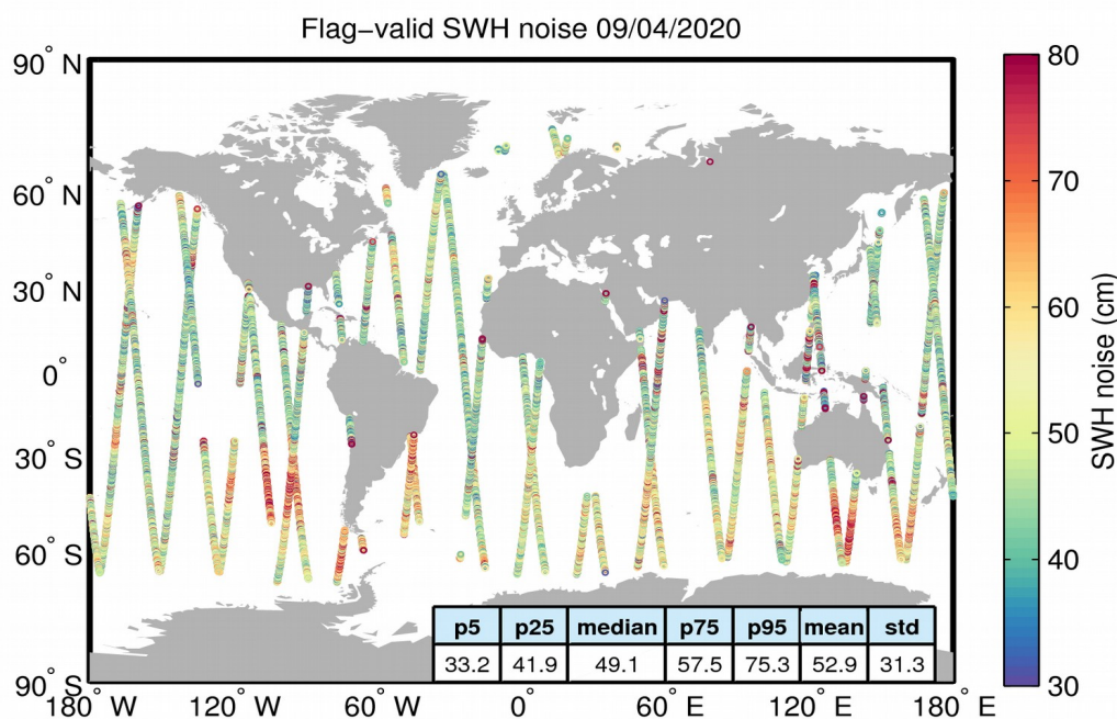
Figure 18. Geographical distribution of flag-valid 20-Hz SWH measurement noise over oceans and lakes for 09/04/2020. The statistical values shown in the figure refer to the SWH noise and are calculated over all measurements shown in the figure.
