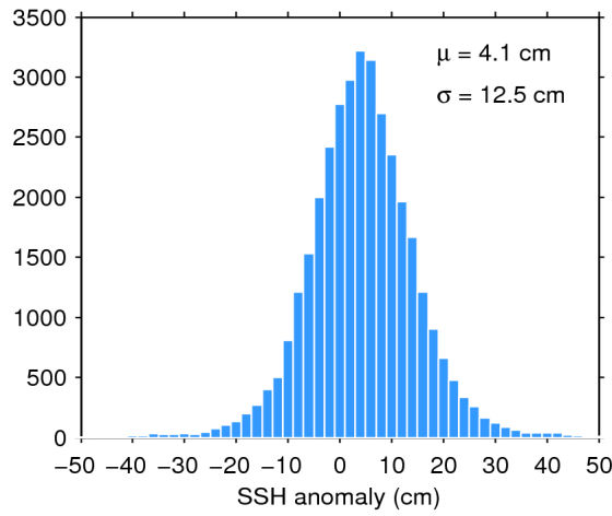
Figure 11. Histogram of science-valid SSH anomaly over oceans and lakes for 09/04/2020. The mean ( \mu ) and standard deviation ( \sigma ) are also shown. Note that values outside [-50 50] cm are excluded from the histogram for the sake of readability but not from the computation of \mu and \sigma .
