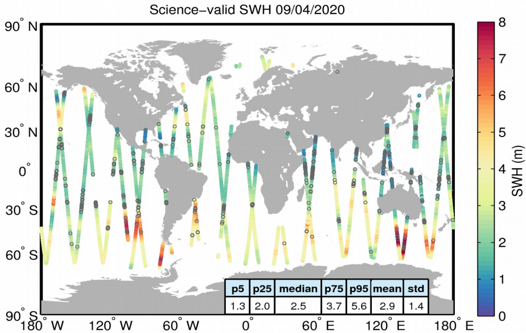
Figure 19. Geographical distribution of science-valid SWH data over oceans and lakes for 09/04/2020. The statistical values shown in the table refer to the SWH in m and are calculated over all measurements shown in the figure. Gray circles denote records that have been rejected based on the editing criteria described in Table 3.
