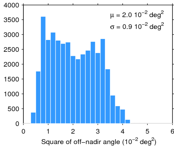
Figure 39. Histogram of flag-valid mispointing over oceans and lakes for 09/04/2020. The mean ( \mu ) and standard deviation ( \sigma ) are also shown. Note that values larger than 6 \cdot 10^{-2} \text{ deg}^2 are excluded from the histogram for the sake of readability but not from the computation of \mu and \sigma .
