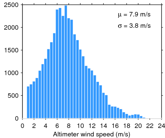
Figure 33. Histogram of flag-valid wind over oceans and lakes for 09/04/2020. The mean ( \mu ) and standard deviation ( \sigma ) are also shown. Note that values larger than 24 m/s are excluded from the histogram for the sake of readability but not from the computation of \mu and \sigma .
