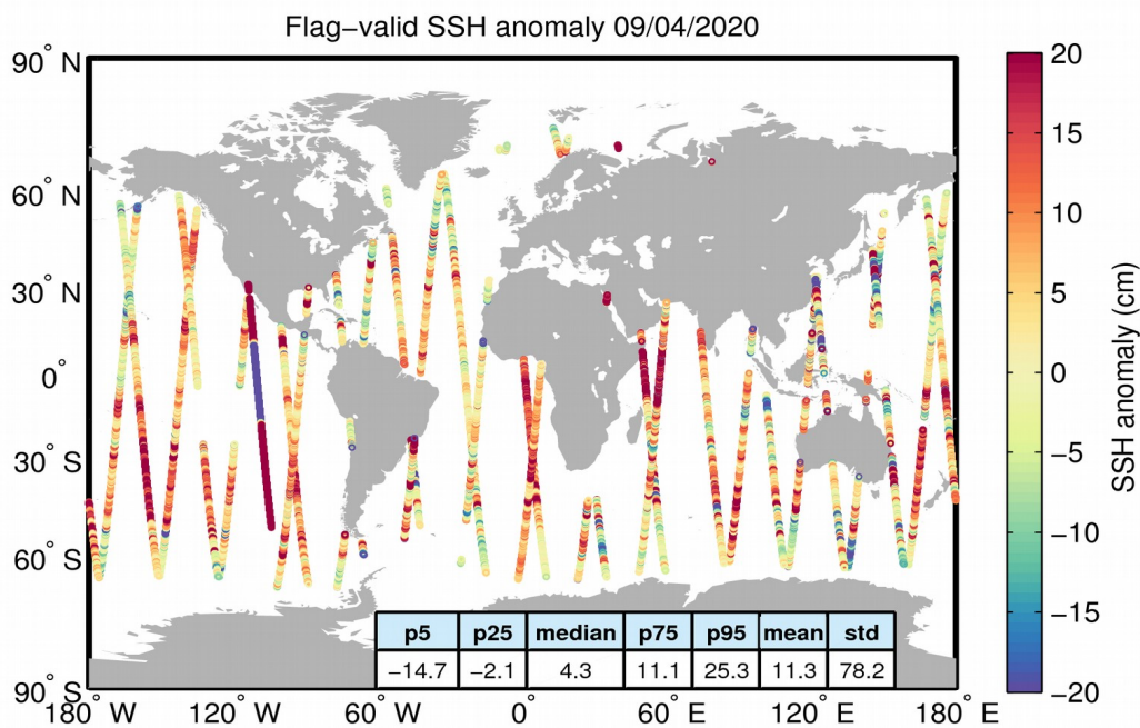
Figure 5. Geographical distribution of flag-valid 1-Hz SSH anomaly data over oceans and lakes for 09/04/2020. The statistical values shown in the table refer to the SSH anomaly in cm and are calculated over all measurements shown in the figure.
