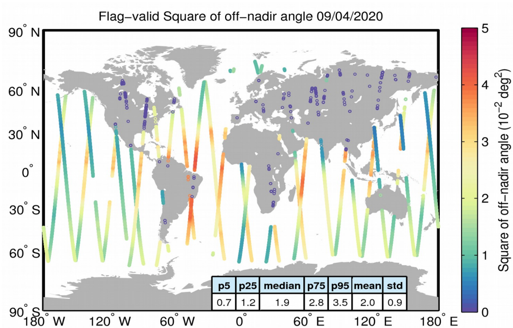
Figure 37. Geographical distribution of flag-valid mispointing data over oceans and lakes for 09/04/2020. The statistical values shown in the table refer to the mispointing in 10^{-2} deg 2 and are calculated over all measurements shown in the figure.
