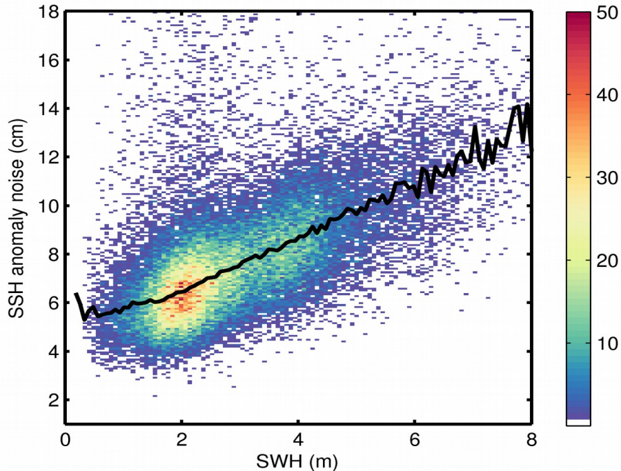
Figure 9. 2D histogram showing flag-valid SSH anomaly noise as a function of SWH for 09/04/2020. The black line denotes the median SSH anomaly noise as a function of SWH.
