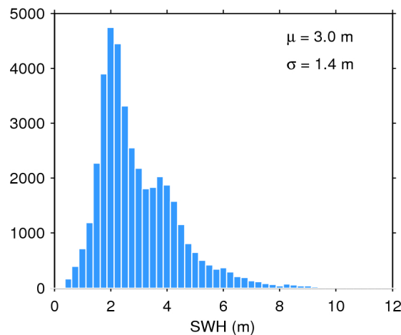
Figure 17. Histogram of flag-valid SWH over oceans and lakes for 09/04/2020. The mean ( \mu ) and standard deviation ( \sigma ) are also shown. Note that values larger than 12 m are excluded from the histogram for the sake of readability but not from the computation of \mu and \sigma .
