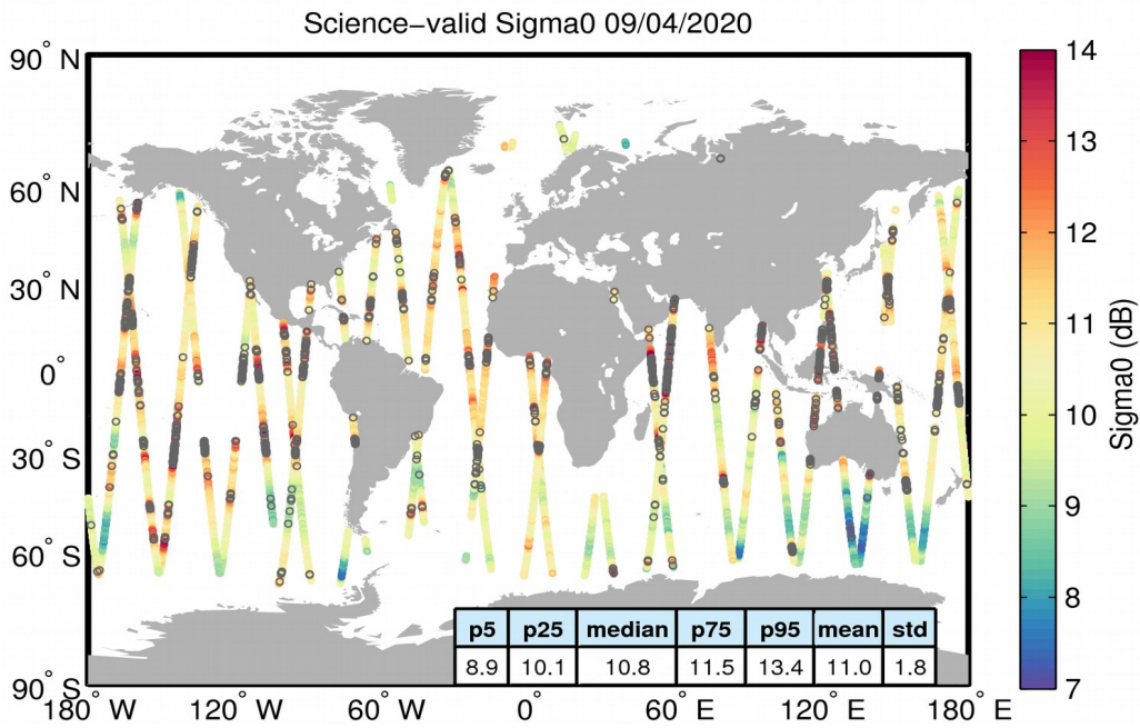
Figure 27. Geographical distribution of science-valid sigma0 data over oceans and lakes for 09/04/2020. The statistical values shown in the table refer to the sigma0 in dB and are calculated over all measurements shown in the figure. Gray circles denote records that have been rejected based on the editing criteria described in Table 4.
