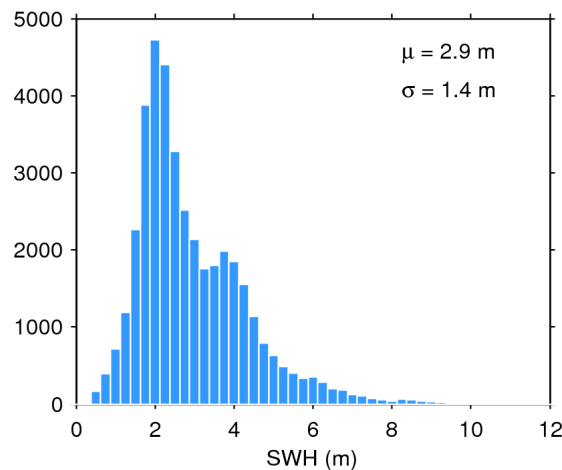
Figure 20. Histogram of science-valid SWH over oceans and lakes for 09/04/2020. The mean ( \mu ) and standard deviation ( \sigma ) are also shown. Note that values larger than 12 m are excluded from the histogram for the sake of readability but not from the computation of \mu and \sigma .
