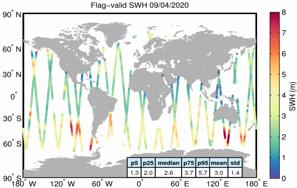
Figure 15. Geographical distribution of flag-valid SWH data over oceans and lakes for 09/04/2020. The statistical values shown in the table refer to the SWH in m and are calculated over all measurements shown in the figure.
