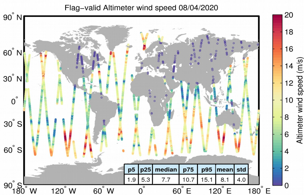
Figure 31. Geographical distribution of flag-valid wind data over oceans and lakes for 08/04/2020. The statistical values shown in the figure refer to the wind in m/s and are calculated over all measurements shown in the figure.
