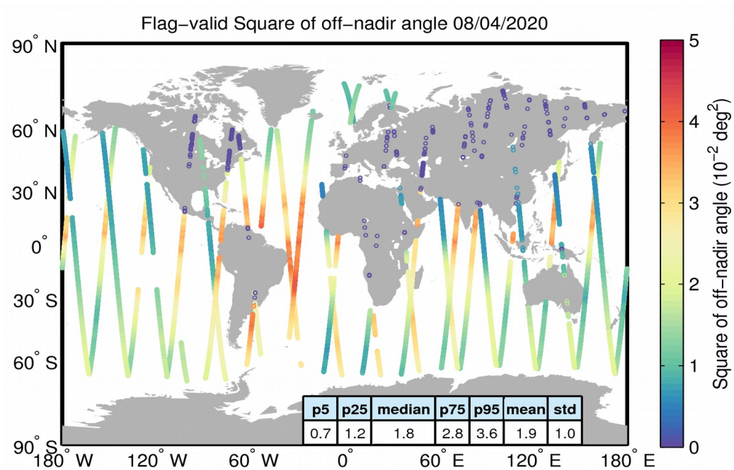
Figure 37. Geographical distribution of flag-valid mispointing data over oceans and lakes for 08/04/2020. The statistical values shown in the table refer to the mispointing in 10^{-2} \text{ deg}^2 and are calculated over all measurements shown in the figure.
