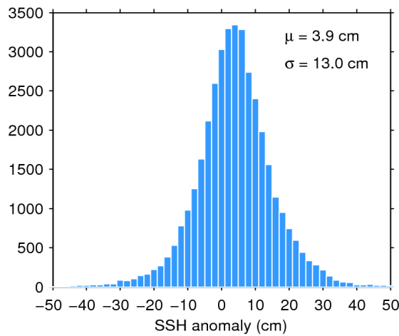
Figure 11. Histogram of science-valid SSH anomaly over oceans and lakes for 08/04/2020. The mean ( \mu ) and standard deviation ( \sigma ) are also shown. Note that values outside [-50 50] cm are excluded from the histogram for the sake of readability but not from the computation of \mu and \sigma .
