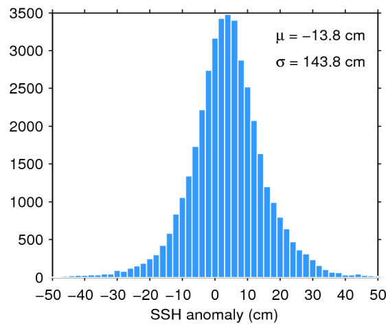
Figure 7. Histogram of flag-valid SSH anomaly over oceans and lakes for 08/04/2020. The mean ( \mu ) and standard deviation ( \sigma ) are also shown. Note that values outside [-50\ 50] cm are excluded from the histogram for the sake of readability but not from the computation of \mu and \sigma .
