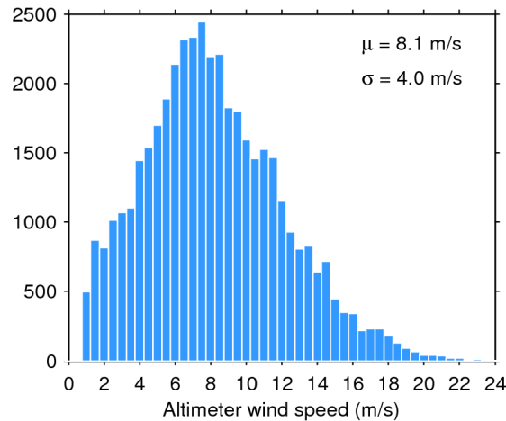
Figure 33. Histogram of flag-valid wind over oceans and lakes for 08/04/2020. The mean ( \mu ) and standard deviation ( \sigma ) are also shown. Note that values larger than 24 m/s are excluded from the histogram for the sake of readability but not from the computation of \mu and \sigma .
