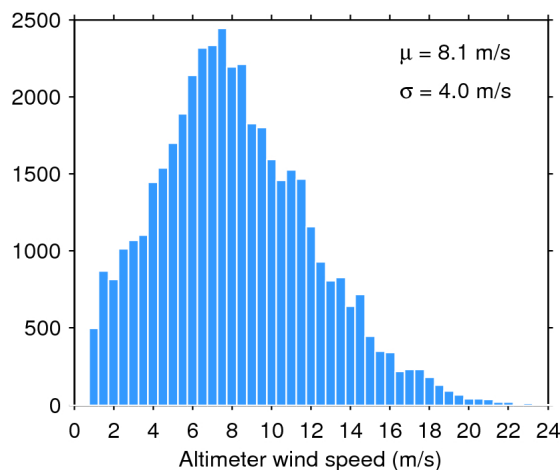
Figure 35. Histogram of science-valid wind over oceans and lakes for 08/04/2020. The mean ( \mu ) and standard deviation ( \sigma ) are also shown. Note that values larger than 24 m/s are excluded from the histogram for the sake of readability but not from the computation of \mu and \sigma .
