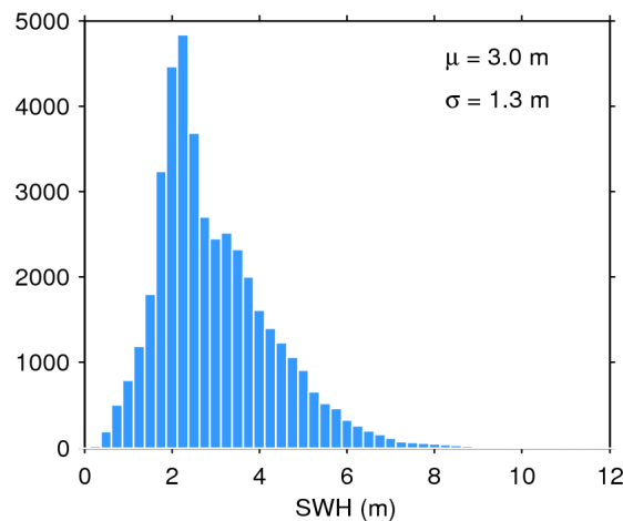
Figure 20. Histogram of science-valid SWH over oceans and lakes for 08/04/2020. The mean ( \mu ) and standard deviation ( \sigma ) are also shown. Note that values larger than 12 m are excluded from the histogram for the sake of readability but not from the computation of \mu and \sigma .
