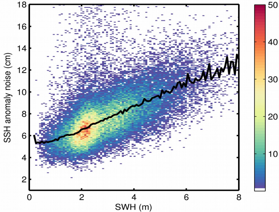
Figure 9. 2D histogram showing flag-valid SSH anomaly noise as a function of SWH for 08/04/2020. The black line denotes the median SSH anomaly noise as a function of SWH.
