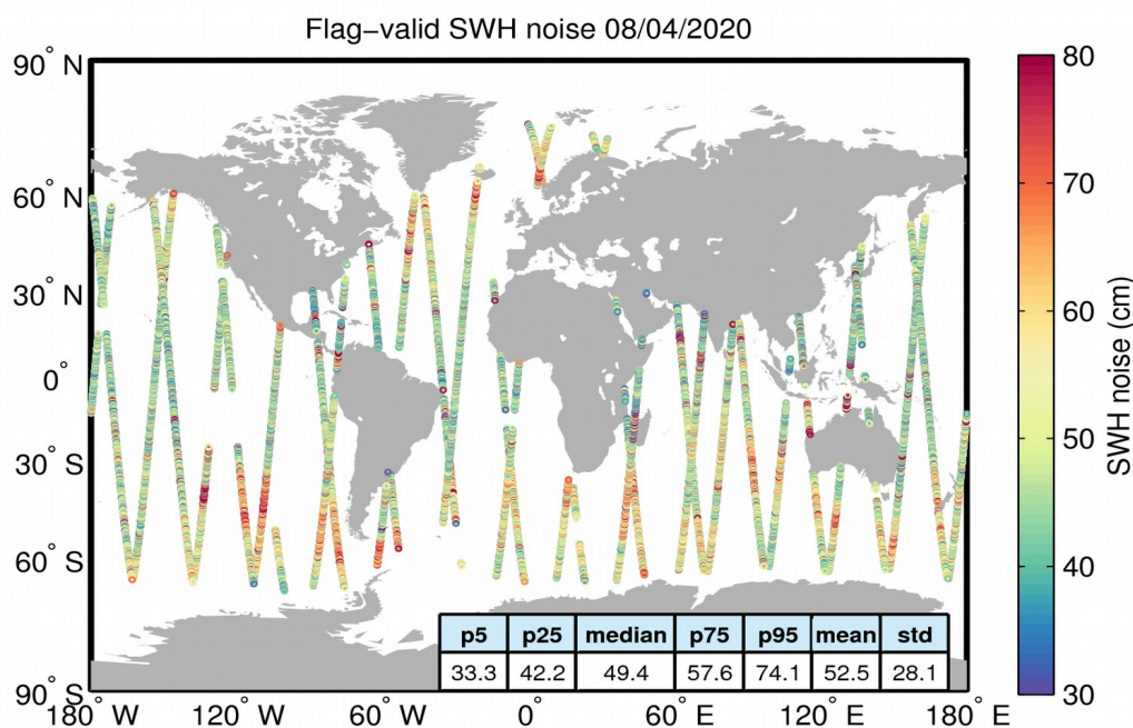
Figure 18. Geographical distribution of flag-valid 20-Hz SWH measurement noise over oceans and lakes for 08/04/2020. The statistical values shown in the figure refer to the SWH noise and are calculated over all measurements shown in the figure.
