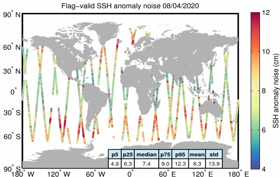
Figure 8. Geographical distribution of flag-valid 20-Hz SSH anomaly measurement noise over oceans and lakes for 08/04/2020. The statistical values shown in the table refer to the SSH anomaly noise and are calculated over all measurements shown in the figure.
