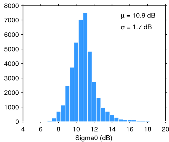
Figure 28. Histogram of science-valid sigma0 over oceans and lakes for 08/04/2020. The mean ( \mu ) and standard deviation ( \sigma ) are also shown. Note that values outside [4 20] dB are excluded from the histogram for the sake of readability but not from the computation of \mu and \sigma .
