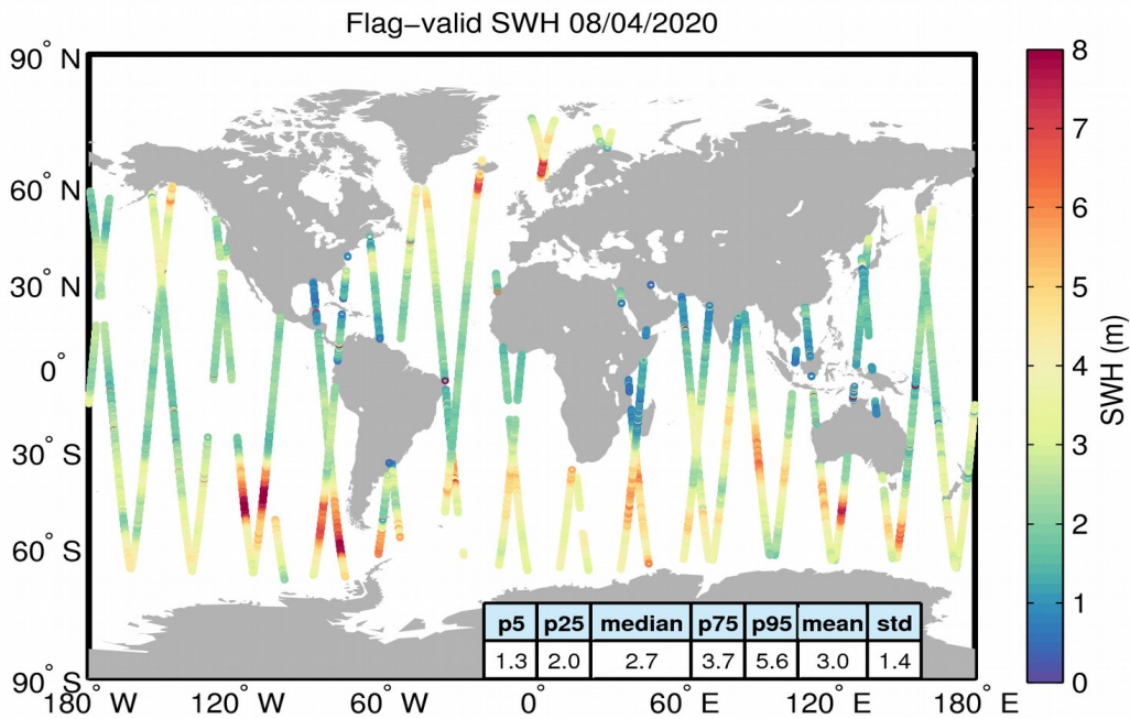
Figure 15. Geographical distribution of flag-valid SWH data over oceans and lakes for 08/04/2020. The statistical values shown in the table refer to the SWH in m and are calculated over all measurements shown in the figure.
