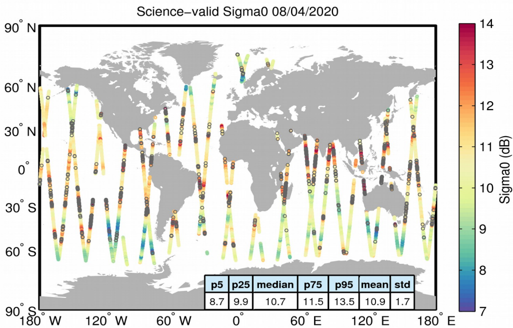
Figure 27. Geographical distribution of science-valid sigma0 data over oceans and lakes for 08/04/2020. The statistical values shown in the table refer to the sigma0 in dB and are calculated over all measurements shown in the figure. Gray circles denote records that have been rejected based on the editing criteria described in Table 4.
