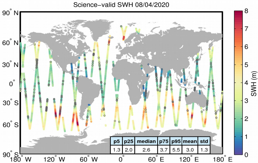
Figure 19. Geographical distribution of science-valid SWH data over oceans and lakes for 08/04/2020. The statistical values shown in the table refer to the SWH in m and are calculated over all measurements shown in the figure. Gray circles denote records that have been rejected based on the editing criteria described in Table 3.
