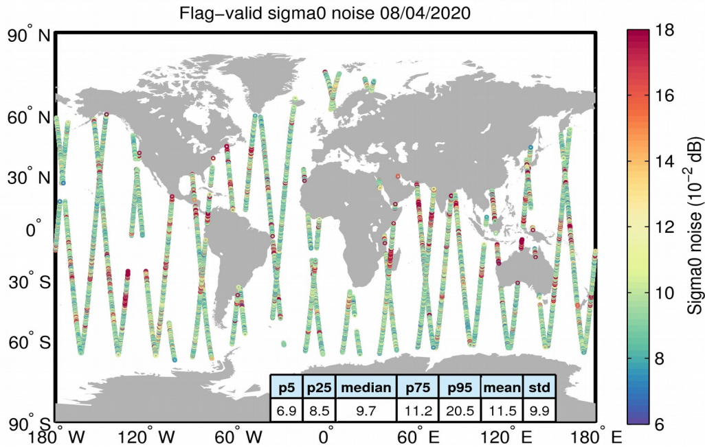
Figure 26. Geographical distribution of flag-valid 20-Hz sigma0 measurement noise over oceans and lakes for 08/04/2020. The statistical values shown in the table refer to the sigma0 noise and are calculated over all measurements shown in the figure.
