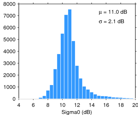
Figure 25. Histogram of flag-valid sigma0 over oceans and lakes for 08/04/2020. The mean ( \mu ) and standard deviation ( \sigma ) are also shown. Note that values outside [4 20] dB are excluded from the histogram for the sake of readability but not from the computation of \mu and \sigma .
