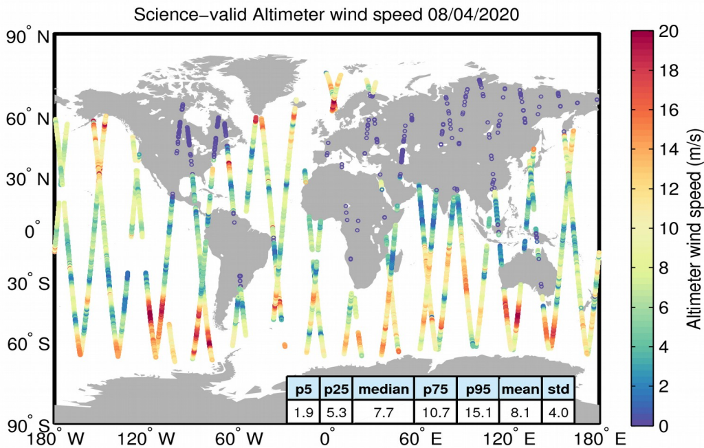
Figure 34. Geographical distribution of science-valid wind data over oceans and lakes for 08/04/2020. The statistical values shown in the table refer to the wind in m/s and are calculated over all measurements shown in the figure. Gray circles denote records that have been rejected based on the editing criteria described in Table 5.
