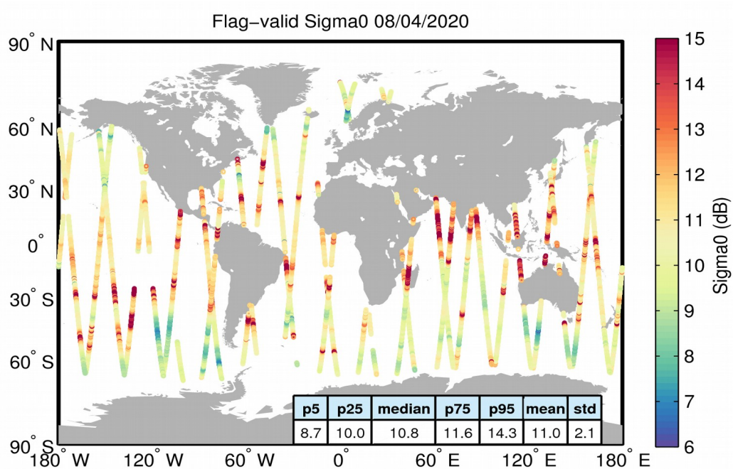
Figure 23. Geographical distribution of flag-valid sigma0 data over oceans and lakes for 08/04/2020. The statistical values shown in the table refer to the sigma0 in dB and are calculated over all measurements shown in the figure.
