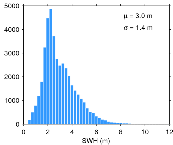
Figure 17. Histogram of flag-valid SWH over oceans and lakes for 08/04/2020. The mean ( \mu ) and standard deviation ( \sigma ) are also shown. Note that values larger than 12 m are excluded from the histogram for the sake of readability but not from the computation of \mu and \sigma .
