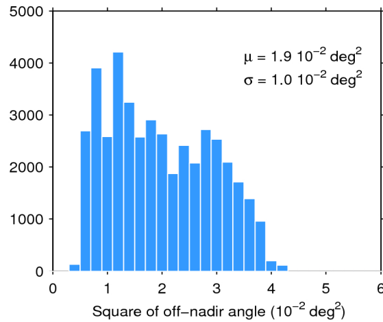
Figure 39. Histogram of flag-valid mispointing over oceans and lakes for 08/04/2020. The mean ( \mu ) and standard deviation ( \sigma ) are also shown. Note that values larger than 6 \cdot 10^{-2} \text{ deg}^2 are excluded from the histogram for the sake of readability but not from the computation of \mu and \sigma .
