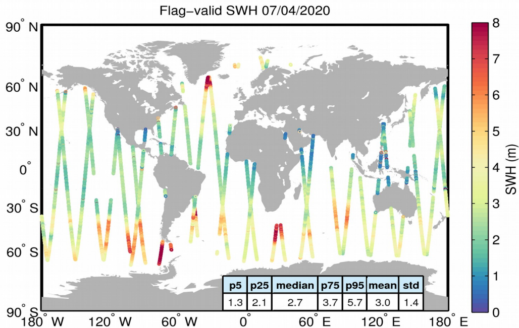
Figure 15. Geographical distribution of flag-valid SWH data over oceans and lakes for 07/04/2020. The statistical values shown in the table refer to the SWH in m and are calculated over all measurements shown in the figure.
