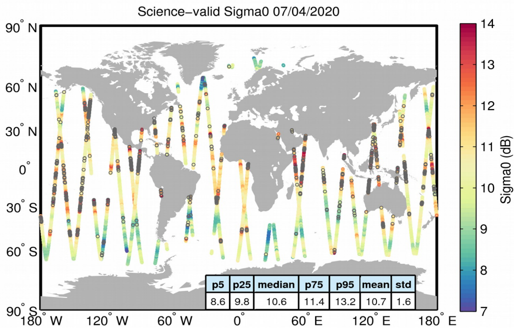
Figure 27. Geographical distribution of science-valid sigma0 data over oceans and lakes for 07/04/2020. The statistical values shown in the table refer to the sigma0 in dB and are calculated over all measurements shown in the figure. Gray circles denote records that have been rejected based on the editing criteria described in Table 4.
