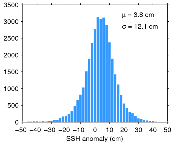
Figure 11. Histogram of science-valid SSH anomaly over oceans and lakes for 07/04/2020. The mean ( \mu ) and standard deviation ( \sigma ) are also shown. Note that values outside [-50 50] cm are excluded from the histogram for the sake of readability but not from the computation of \mu and \sigma .
