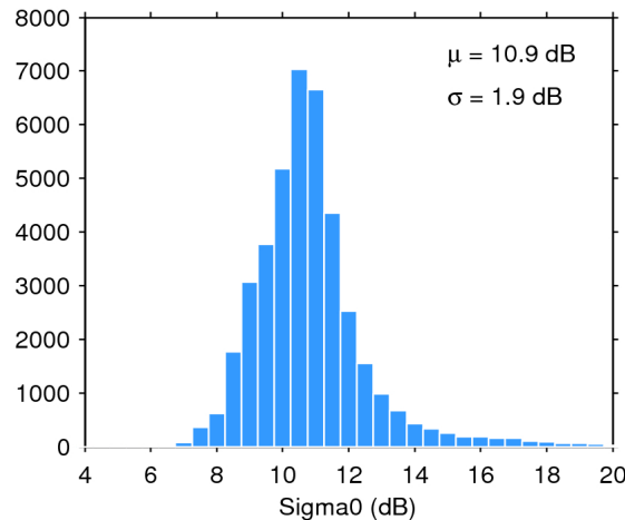
Figure 25. Histogram of flag-valid sigma0 over oceans and lakes for 07/04/2020. The mean ( \mu ) and standard deviation ( \sigma ) are also shown. Note that values outside [4 20] dB are excluded from the histogram for the sake of readability but not from the computation of \mu and \sigma .
