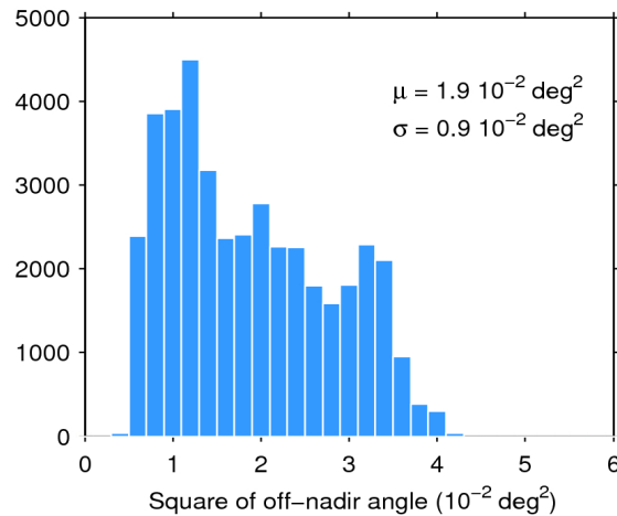
Figure 39. Histogram of flag-valid mispointing over oceans and lakes for 07/04/2020. The mean ( \mu ) and standard deviation ( \sigma ) are also shown. Note that values larger than 6 \cdot 10^{-2} \text{ deg}^2 are excluded from the histogram for the sake of readability but not from the computation of \mu and \sigma .
