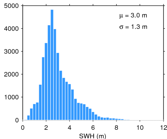
Figure 20. Histogram of science-valid SWH over oceans and lakes for 07/04/2020. The mean ( \mu ) and standard deviation ( \sigma ) are also shown. Note that values larger than 12 m are excluded from the histogram for the sake of readability but not from the computation of \mu and \sigma .
