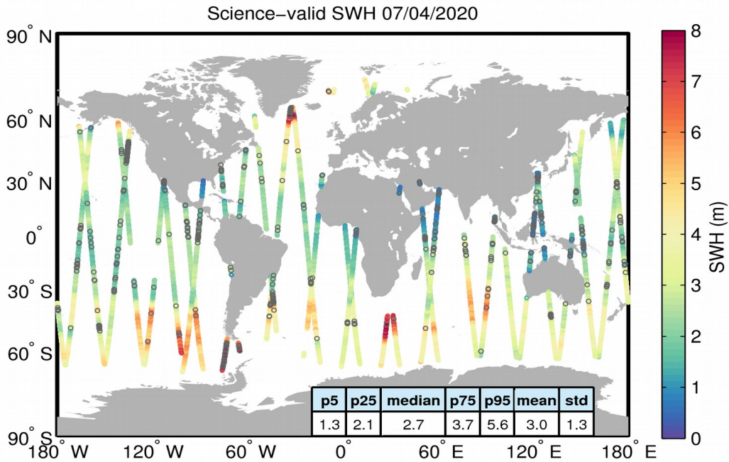
Figure 19. Geographical distribution of science-valid SWH data over oceans and lakes for 07/04/2020. The statistical values shown in the table refer to the SWH in m and are calculated over all measurements shown in the figure. Gray circles denote records that have been rejected based on the editing criteria described in Table 3.
