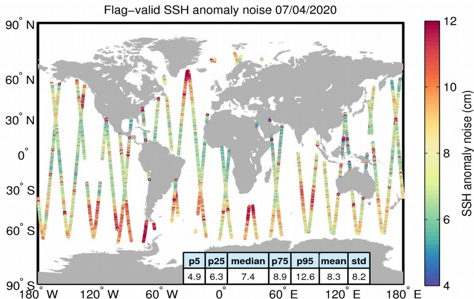
Figure 8. Geographical distribution of flag-valid 20-Hz SSH anomaly measurement noise over oceans and lakes for 07/04/2020. The statistical values shown in the table refer to the SSH anomaly noise and are calculated over all measurements shown in the figure.
