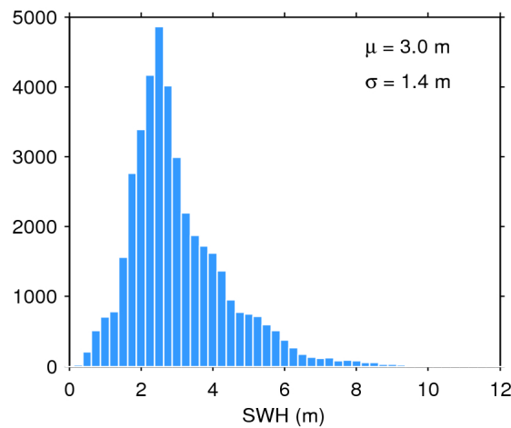
Figure 17. Histogram of flag-valid SWH over oceans and lakes for 07/04/2020. The mean ( \mu ) and standard deviation ( \sigma ) are also shown. Note that values larger than 12 m are excluded from the histogram for the sake of readability but not from the computation of \mu and \sigma .
