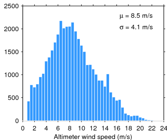
Figure 35. Histogram of science-valid wind over oceans and lakes for 07/04/2020. The mean ( \mu ) and standard deviation ( \sigma ) are also shown. Note that values larger than 24 m/s are excluded from the histogram for the sake of readability but not from the computation of \mu and \sigma .
