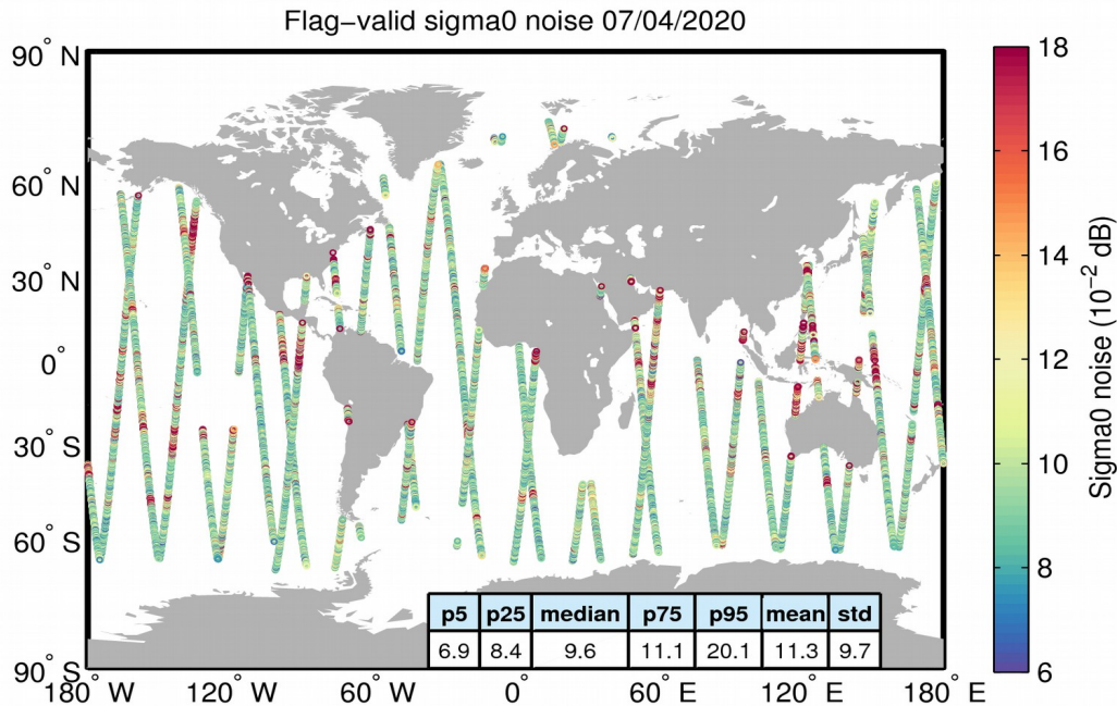
Figure 26. Geographical distribution of flag-valid 20-Hz sigma0 measurement noise over oceans and lakes for 07/04/2020. The statistical values shown in the table refer to the sigma0 noise and are calculated over all measurements shown in the figure.
