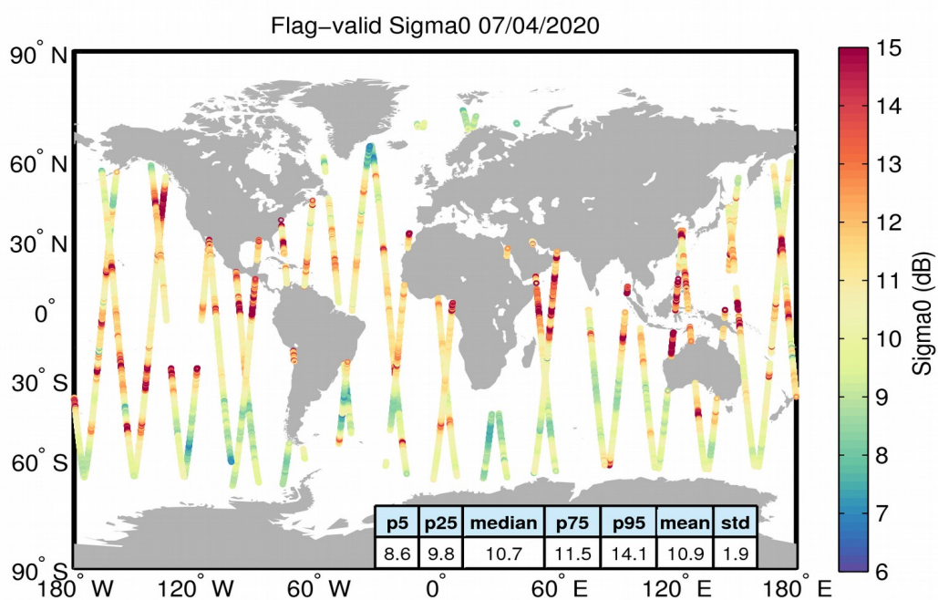
Figure 23. Geographical distribution of flag-valid sigma0 data over oceans and lakes for 07/04/2020. The statistical values shown in the table refer to the sigma0 in dB and are calculated over all measurements shown in the figure.
