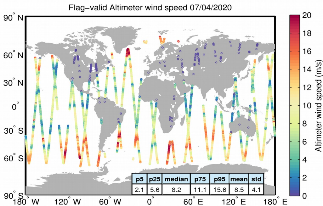
Figure 31. Geographical distribution of flag-valid wind data over oceans and lakes for 07/04/2020. The statistical values shown in the table refer to the wind in m/s and are calculated over all measurements shown in the figure.
