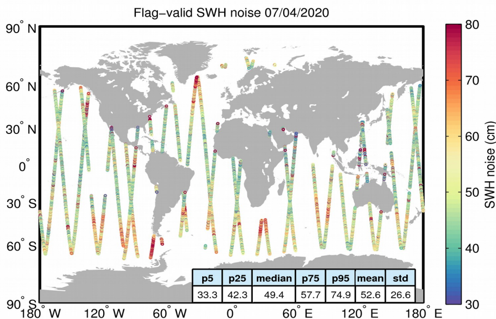
Figure 18. Geographical distribution of flag-valid 20-Hz SWH measurement noise over oceans and lakes for 07/04/2020. The statistical values shown in the figure refer to the SWH noise and are calculated over all measurements shown in the figure.
