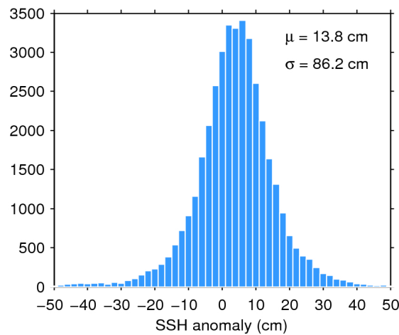
Figure 7. Histogram of flag-valid SSH anomaly over oceans and lakes for 07/04/2020. The mean ( \mu ) and standard deviation ( \sigma ) are also shown. Note that values outside [-50\ 50] cm are excluded from the histogram for the sake of readability but not from the computation of \mu and \sigma .
