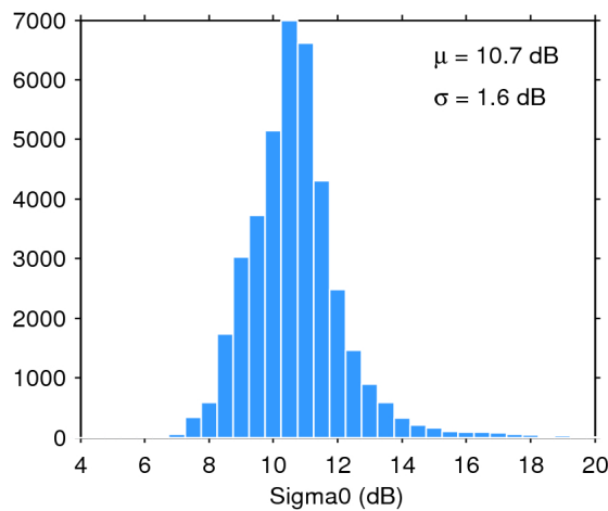
Figure 28. Histogram of science-valid sigma0 over oceans and lakes for 07/04/2020. The mean ( \mu ) and standard deviation ( \sigma ) are also shown. Note that values outside [4 20] dB are excluded from the histogram for the sake of readability but not from the computation of \mu and \sigma .
