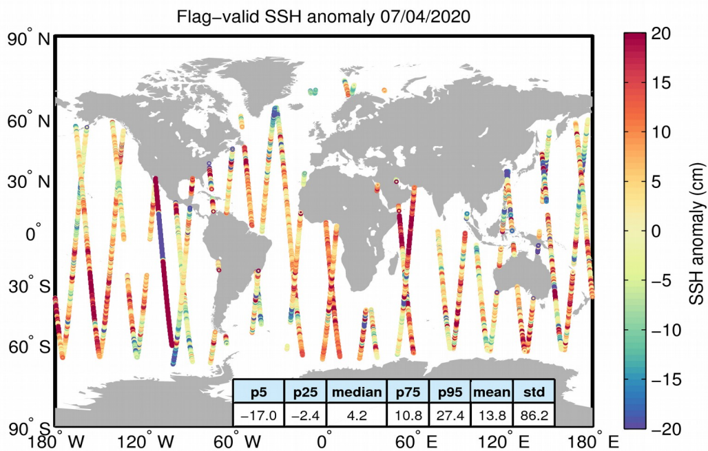
Figure 5. Geographical distribution of flag-valid 1-Hz SSH anomaly data over oceans and lakes for 07/04/2020. The statistical values shown in the table refer to the SSH anomaly in cm and are calculated over all measurements shown in the figure.
