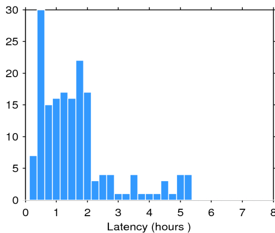
Figure 2. Histogram of the data latency for 07/04/2020. The y-axis denotes the number of files that are made available with a delay of x-hours with respect to the mean time of the records stored in the file.
