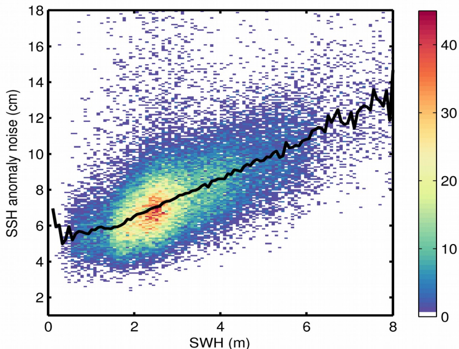
Figure 9. 2D histogram showing flag-valid SSH anomaly noise as a function of SWH for 07/04/2020. The black line denotes the median SSH anomaly noise as a function of SWH.
