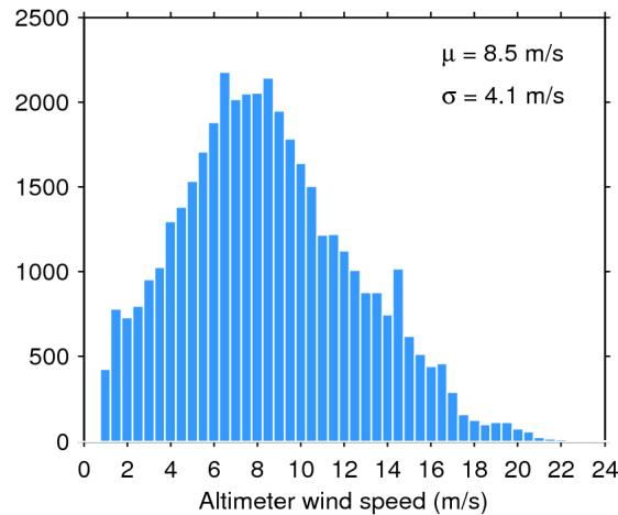
Figure 33. Histogram of flag-valid wind over oceans and lakes for 07/04/2020. The mean ( \mu ) and standard deviation ( \sigma ) are also shown. Note that values larger than 24 m/s are excluded from the histogram for the sake of readability but not from the computation of \mu and \sigma .
