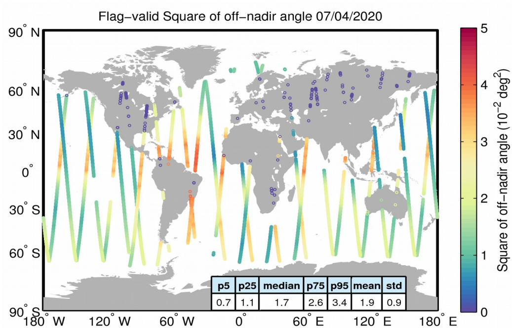
Figure 37. Geographical distribution of flag-valid mispointing data over oceans and lakes for 07/04/2020. The statistical values shown in the table refer to the mispointing in 10^{-2} \text{ deg}^2 and are calculated over all measurements shown in the figure.
