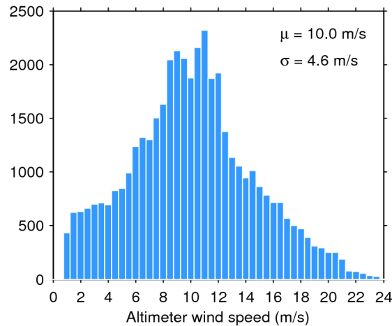
Figure 33. Histogram of flag-valid wind over oceans and lakes for 06/04/2020. The mean ( \mu ) and standard deviation ( \sigma ) are also shown. Note that values larger than 24 m/s are excluded from the histogram for the sake of readability but not from the computation of \mu and \sigma .
