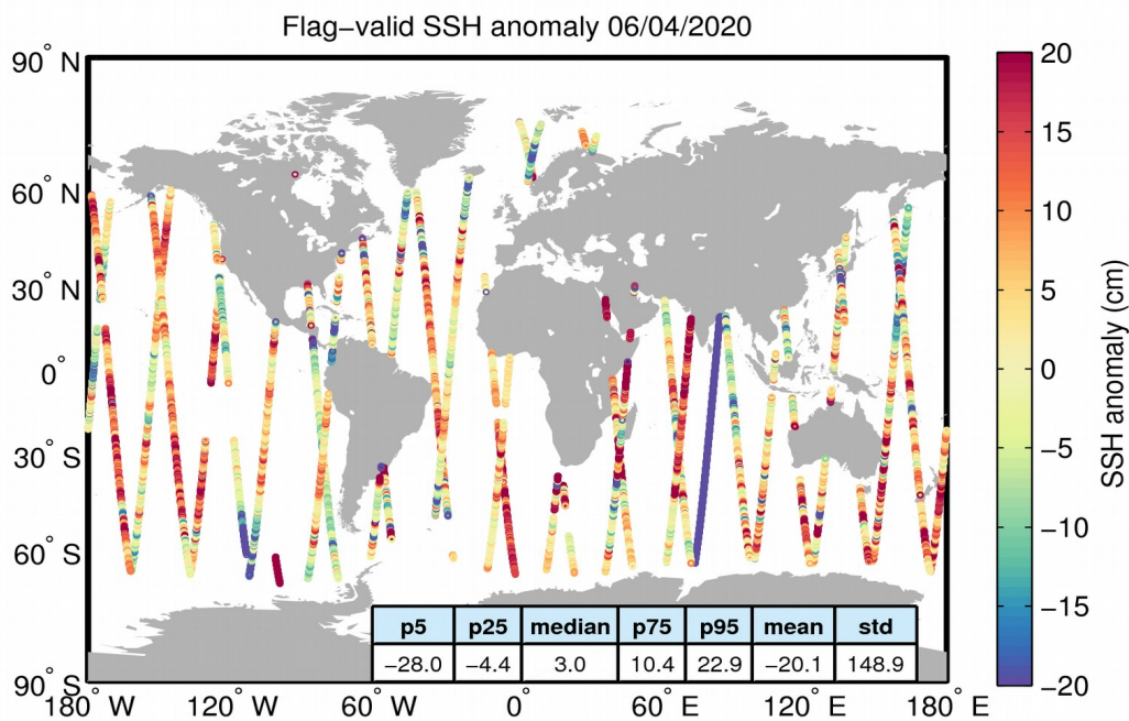
Figure 5. Geographical distribution of flag-valid 1-Hz SSH anomaly data over oceans and lakes for 06/04/2020. The statistical values shown in the table refer to the SSH anomaly in cm and are calculated over all measurements shown in the figure.
