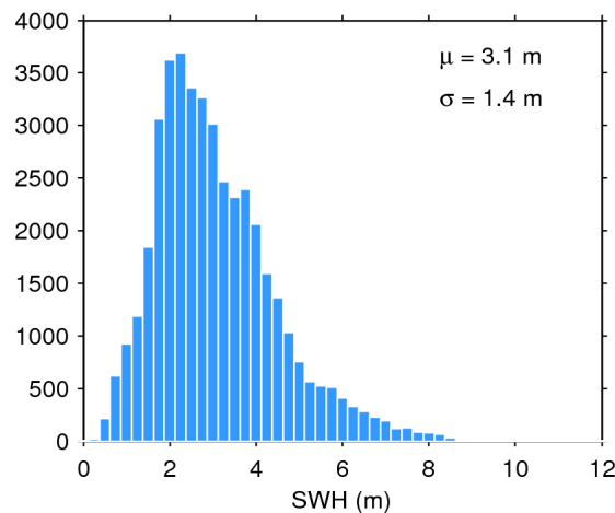
Figure 17. Histogram of flag-valid SWH over oceans and lakes for 06/04/2020. The mean ( \mu ) and standard deviation ( \sigma ) are also shown. Note that values larger than 12 m are excluded from the histogram for the sake of readability but not from the computation of \mu and \sigma .
