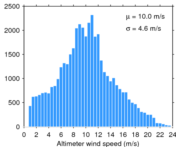
Figure 35. Histogram of science-valid wind over oceans and lakes for 06/04/2020. The mean ( \mu ) and standard deviation ( \sigma ) are also shown. Note that values larger than 24 m/s are excluded from the histogram for the sake of readability but not from the computation of \mu and \sigma .
