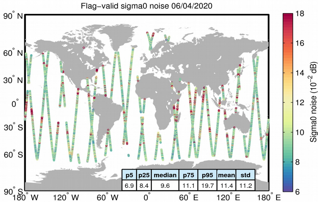
Figure 26. Geographical distribution of flag-valid 20-Hz sigma0 measurement noise over oceans and lakes for 06/04/2020. The statistical values shown in the table refer to the sigma0 noise and are calculated over all measurements shown in the figure.
