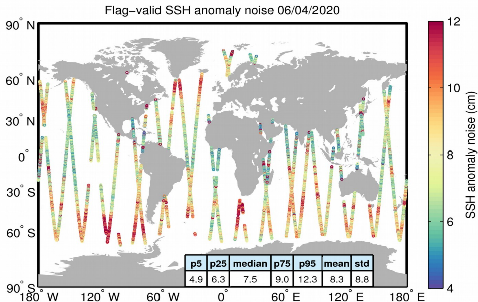
Figure 8. Geographical distribution of flag-valid 20-Hz SSH anomaly measurement noise over oceans and lakes for 06/04/2020. The statistical values shown in the table refer to the SSH anomaly noise and are calculated over all measurements shown in the figure.
