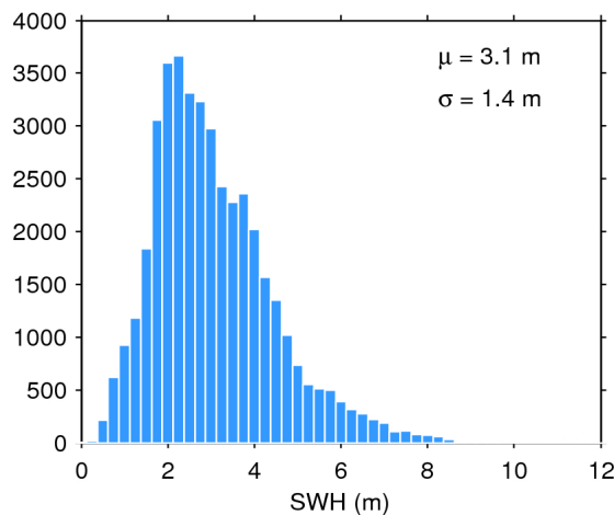
Figure 20. Histogram of science-valid SWH over oceans and lakes for 06/04/2020. The mean ( \mu ) and standard deviation ( \sigma ) are also shown. Note that values larger than 12 m are excluded from the histogram for the sake of readability but not from the computation of \mu and \sigma .
