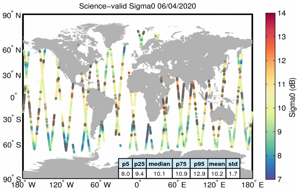
Figure 27. Geographical distribution of science-valid sigma0 data over oceans and lakes for 06/04/2020. The statistical values shown in the table refer to the sigma0 in dB and are calculated over all measurements shown in the figure. Gray circles denote records that have been rejected based on the editing criteria described in Table 4.
