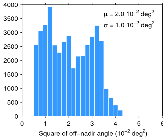
Figure 39. Histogram of flag-valid mispointing over oceans and lakes for 06/04/2020. The mean ( \mu ) and standard deviation ( \sigma ) are also shown. Note that values larger than 6 \cdot 10^{-2} \text{ deg}^2 are excluded from the histogram for the sake of readability but not from the computation of \mu and \sigma .
