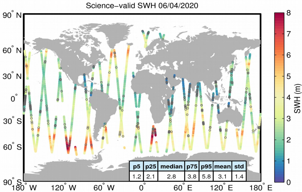
Figure 19. Geographical distribution of science-valid SWH data over oceans and lakes for 06/04/2020. The statistical values shown in the table refer to the SWH in m and are calculated over all measurements shown in the figure. Gray circles denote records that have been rejected based on the editing criteria described in Table 3.
