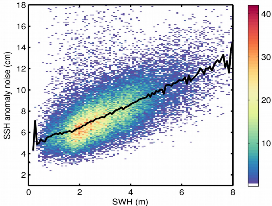
Figure 9. 2D histogram showing flag-valid SSH anomaly noise as a function of SWH for 06/04/2020. The black line denotes the median SSH anomaly noise as a function of SWH.
