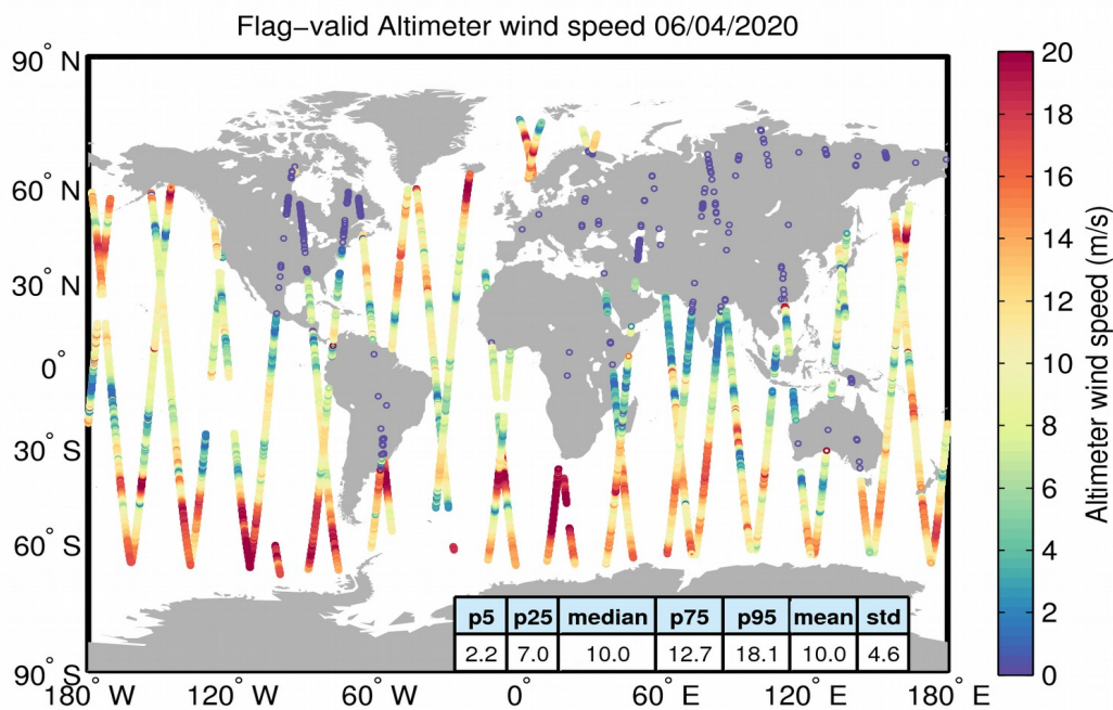
Figure 31. Geographical distribution of flag-valid wind data over oceans and lakes for 06/04/2020. The statistical values shown in the table refer to the wind in m/s and are calculated over all measurements shown in the figure.
