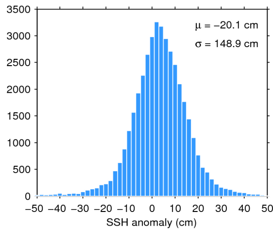
Figure 7. Histogram of flag-valid SSH anomaly over oceans and lakes for 06/04/2020. The mean ( \mu ) and standard deviation ( \sigma ) are also shown. Note that values outside [-50\ 50] cm are excluded from the histogram for the sake of readability but not from the computation of \mu and \sigma .
