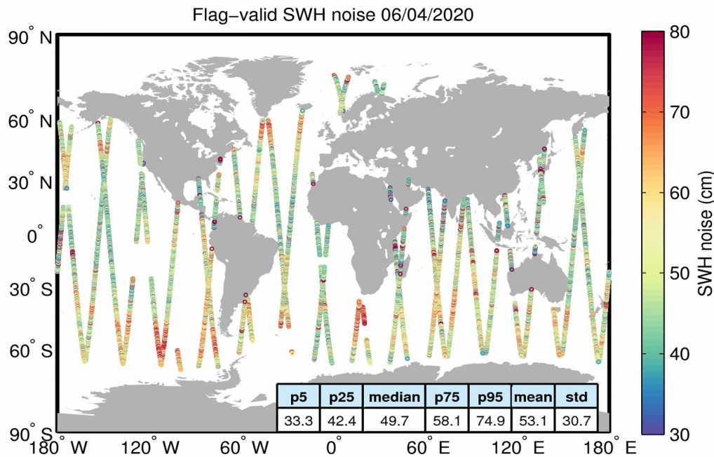
Figure 18. Geographical distribution of flag-valid 20-Hz SWH measurement noise over oceans and lakes for 06/04/2020. The statistical values shown in the figure refer to the SWH noise and are calculated over all measurements shown in the figure.
