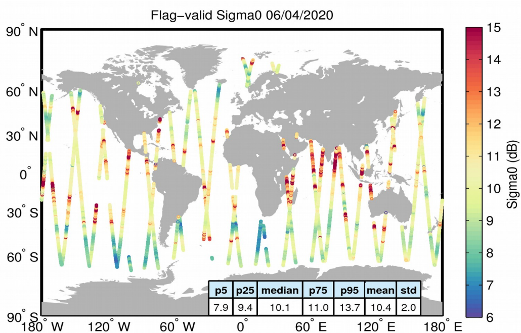
Figure 23. Geographical distribution of flag-valid sigma0 data over oceans and lakes for 06/04/2020. The statistical values shown in the table refer to the sigma0 in dB and are calculated over all measurements shown in the figure.
