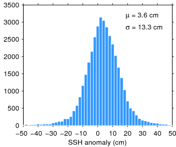
Figure 11. Histogram of science-valid SSH anomaly over oceans and lakes for 06/04/2020. The mean ( \mu ) and standard deviation ( \sigma ) are also shown. Note that values outside [-50 50] cm are excluded from the histogram for the sake of readability but not from the computation of \mu and \sigma .
