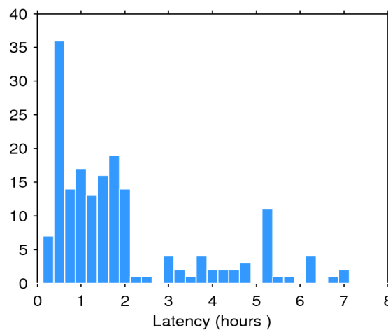
Figure 2. Histogram of the data latency for 06/04/2020. The y-axis denotes the number of files that are made available with a delay of x-hours with respect to the mean time of the records stored in the file.
