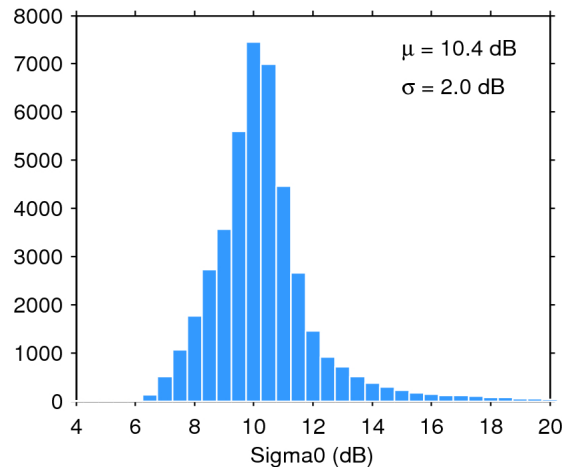
Figure 25. Histogram of flag-valid sigma0 over oceans and lakes for 06/04/2020. The mean ( \mu ) and standard deviation ( \sigma ) are also shown. Note that values outside [4 20] dB are excluded from the histogram for the sake of readability but not from the computation of \mu and \sigma .
