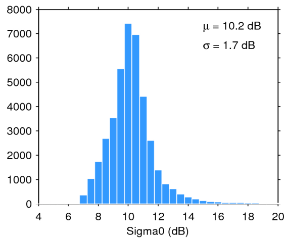
Figure 28. Histogram of science-valid sigma0 over oceans and lakes for 06/04/2020. The mean ( \mu ) and standard deviation ( \sigma ) are also shown. Note that values outside [4 20] dB are excluded from the histogram for the sake of readability but not from the computation of \mu and \sigma .
