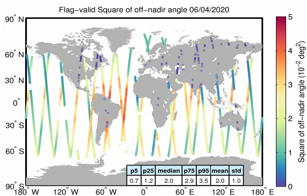
Figure 37. Geographical distribution of flag-valid mispointing data over oceans and lakes for 06/04/2020. The statistical values shown in the table refer to the mispointing in 10^{-2} deg 2 and are calculated over all measurements shown in the figure.
