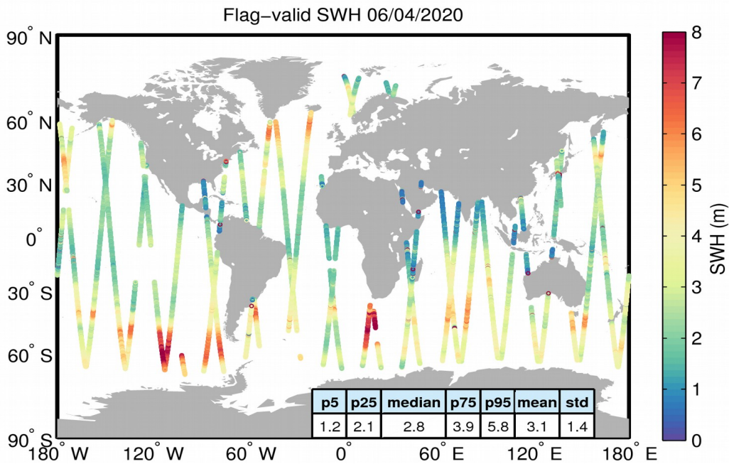
Figure 15. Geographical distribution of flag-valid SWH data over oceans and lakes for 06/04/2020. The statistical values shown in the table refer to the SWH in m and are calculated over all measurements shown in the figure.
