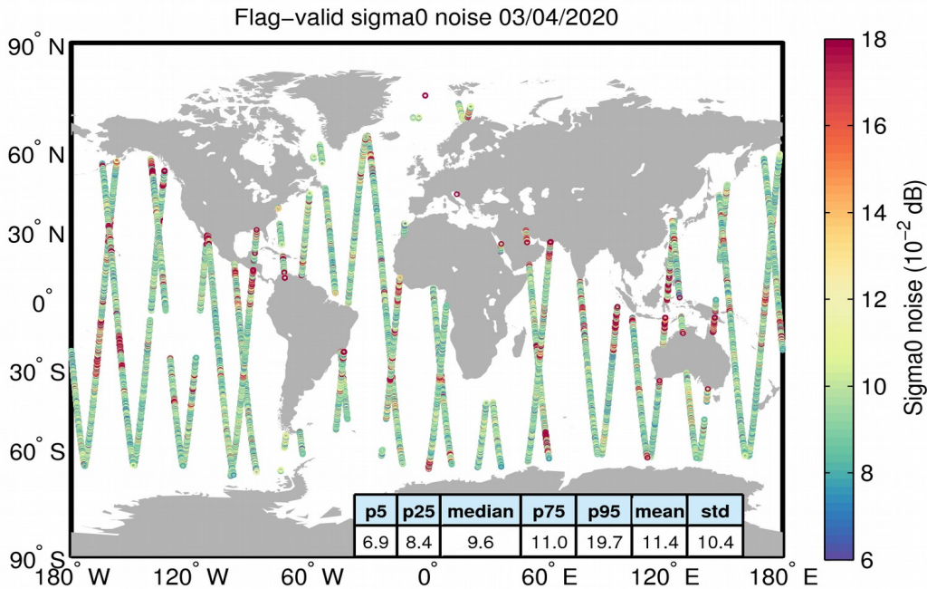
Figure 26. Geographical distribution of flag-valid 20-Hz sigma0 measurement noise over oceans and lakes for 03/04/2020. The statistical values shown in the table refer to the sigma0 noise and are calculated over all measurements shown in the figure.
