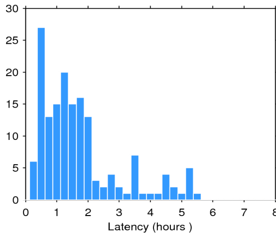
Figure 2. Histogram of the data latency for 03/04/2020. The y-axis denotes the number of files that are made available with a delay of x-hours with respect to the mean time of the records stored in the file.
