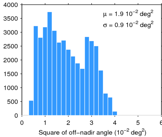
Figure 39. Histogram of flag-valid mispointing over oceans and lakes for 03/04/2020. The mean ( \mu ) and standard deviation ( \sigma ) are also shown. Note that values larger than 6 \cdot 10^{-2} \text{ deg}^2 are excluded from the histogram for the sake of readability but not from the computation of \mu and \sigma .
