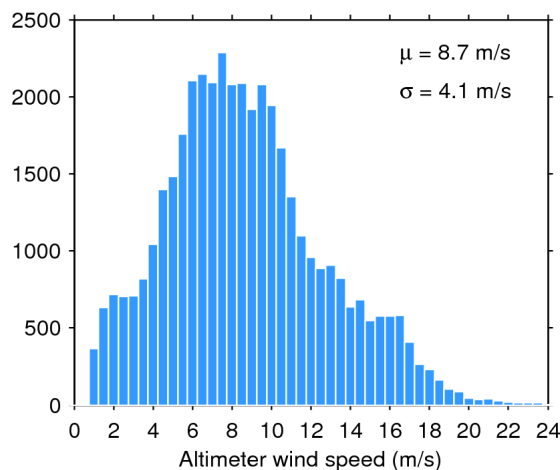
Figure 35. Histogram of science-valid wind over oceans and lakes for 03/04/2020. The mean ( \mu ) and standard deviation ( \sigma ) are also shown. Note that values larger than 24 m/s are excluded from the histogram for the sake of readability but not from the computation of \mu and \sigma .
