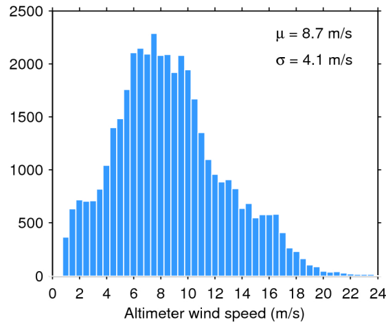
Figure 33. Histogram of flag-valid wind over oceans and lakes for 03/04/2020. The mean ( \mu ) and standard deviation ( \sigma ) are also shown. Note that values larger than 24 m/s are excluded from the histogram for the sake of readability but not from the computation of \mu and \sigma .
