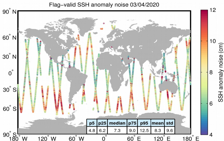
Figure 8. Geographical distribution of flag-valid 20-Hz SSH anomaly measurement noise over oceans and lakes for 03/04/2020. The statistical values shown in the table refer to the SSH anomaly noise and are calculated over all measurements shown in the figure.
