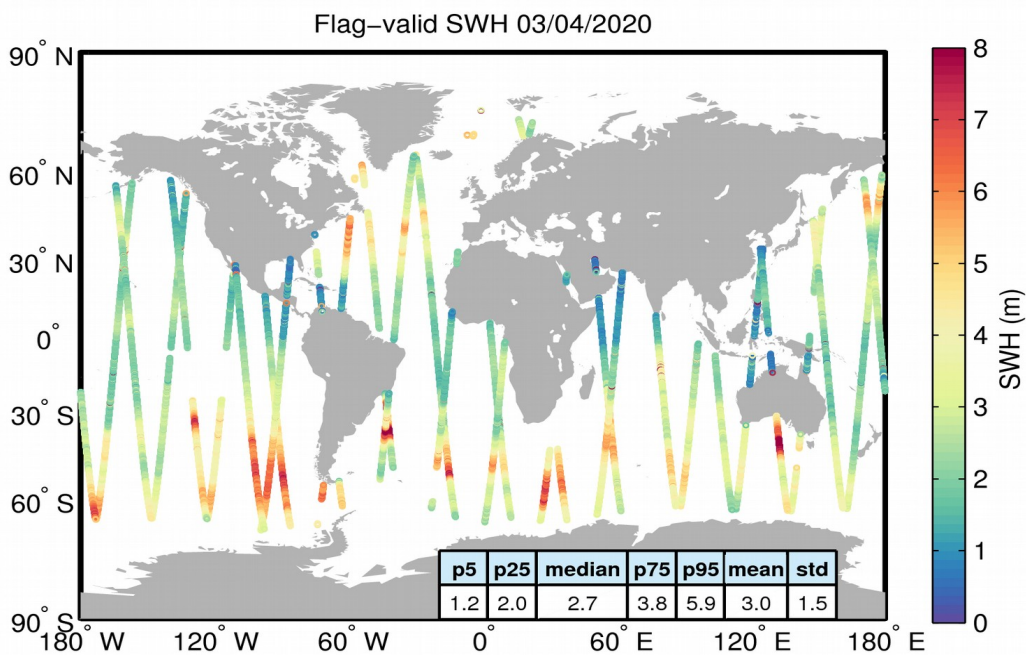
Figure 15. Geographical distribution of flag-valid SWH data over oceans and lakes for 03/04/2020. The statistical values shown in the table refer to the SWH in m and are calculated over all measurements shown in the figure.
