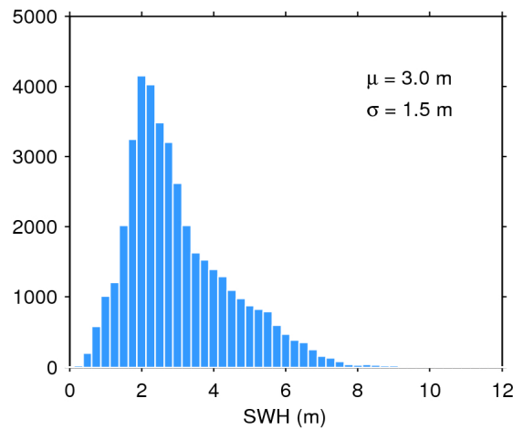
Figure 17. Histogram of flag-valid SWH over oceans and lakes for 03/04/2020. The mean ( \mu ) and standard deviation ( \sigma ) are also shown. Note that values larger than 12 m are excluded from the histogram for the sake of readability but not from the computation of \mu and \sigma .
