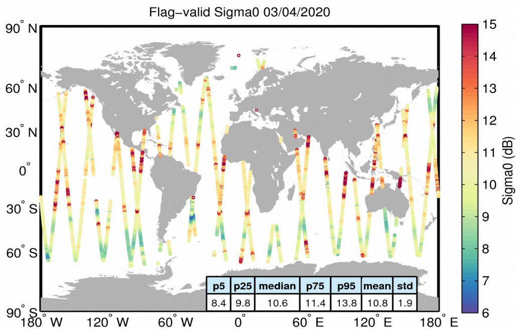
Figure 23. Geographical distribution of flag-valid sigma0 data over oceans and lakes for 03/04/2020. The statistical values shown in the table refer to the sigma0 in dB and are calculated over all measurements shown in the figure.
