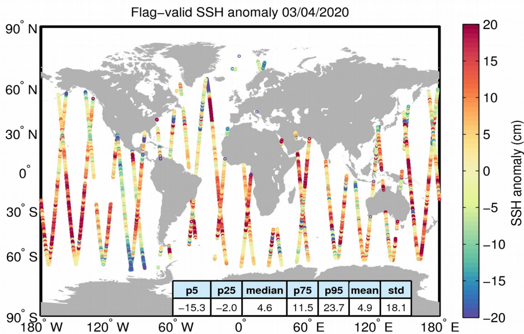
Figure 5. Geographical distribution of flag-valid 1-Hz SSH anomaly data over oceans and lakes for 03/04/2020. The statistical values shown in the table refer to the SSH anomaly in cm and are calculated over all measurements shown in the figure.
