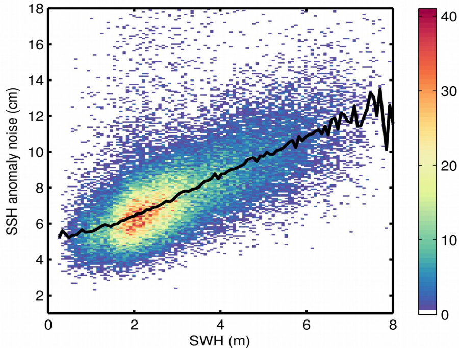
Figure 9. 2D histogram showing flag-valid SSH anomaly noise as a function of SWH for 03/04/2020. The black line denotes the median SSH anomaly noise as a function of SWH.
