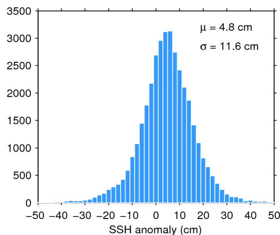
Figure 11. Histogram of science-valid SSH anomaly over oceans and lakes for 03/04/2020. The mean ( \mu ) and standard deviation ( \sigma ) are also shown. Note that values outside [-50 50] cm are excluded from the histogram for the sake of readability but not from the computation of \mu and \sigma .
