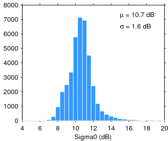
Figure 28. Histogram of science-valid sigma0 over oceans and lakes for 03/04/2020. The mean ( \mu ) and standard deviation ( \sigma ) are also shown. Note that values outside [4 20] dB are excluded from the histogram for the sake of readability but not from the computation of \mu and \sigma .
