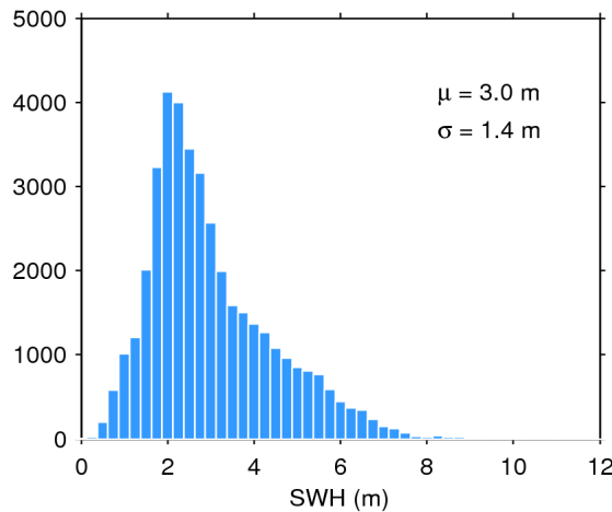
Figure 20. Histogram of science-valid SWH over oceans and lakes for 03/04/2020. The mean ( \mu ) and standard deviation ( \sigma ) are also shown. Note that values larger than 12 m are excluded from the histogram for the sake of readability but not from the computation of \mu and \sigma .
