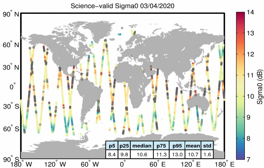
Figure 27. Geographical distribution of science-valid sigma0 data over oceans and lakes for 03/04/2020. The statistical values shown in the table refer to the sigma0 in dB and are calculated over all measurements shown in the figure. Gray circles denote records that have been rejected based on the editing criteria described in Table 4.
