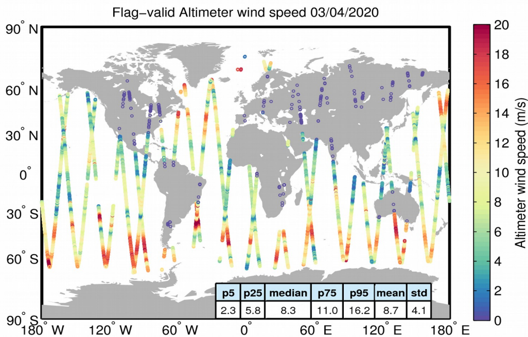
Figure 31. Geographical distribution of flag-valid wind data over oceans and lakes for 03/04/2020. The statistical values shown in the figure refer to the wind in m/s and are calculated over all measurements shown in the figure.
