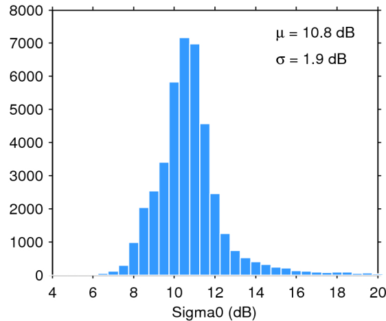
Figure 25. Histogram of flag-valid sigma0 over oceans and lakes for 03/04/2020. The mean ( \mu ) and standard deviation ( \sigma ) are also shown. Note that values outside [4 20] dB are excluded from the histogram for the sake of readability but not from the computation of \mu and \sigma .
