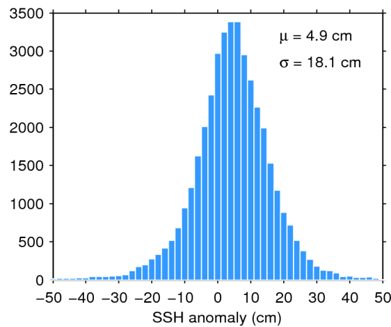
Figure 7. Histogram of flag-valid SSH anomaly over oceans and lakes for 03/04/2020. The mean ( \mu ) and standard deviation ( \sigma ) are also shown. Note that values outside [-50\ 50] cm are excluded from the histogram for the sake of readability but not from the computation of \mu and \sigma .
