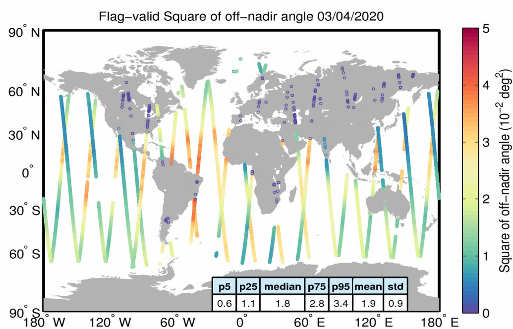
Figure 37. Geographical distribution of flag-valid mispointing data over oceans and lakes for 03/04/2020. The statistical values shown in the table refer to the mispointing in 10^{-2} \text{ deg}^2 and are calculated over all measurements shown in the figure.
