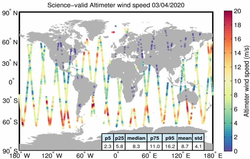
Figure 34. Geographical distribution of science-valid wind data over oceans and lakes for 03/04/2020. The statistical values shown in the table refer to the wind in m/s and are calculated over all measurements shown in the figure. Gray circles denote records that have been rejected based on the editing criteria described in Table 5.
