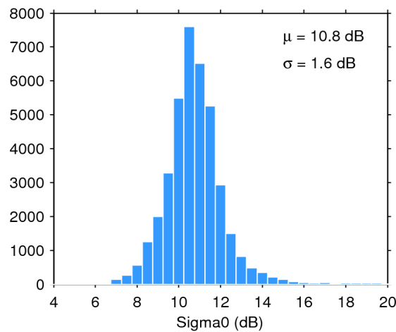
Figure 28. Histogram of science-valid sigma0 over oceans and lakes for 01/04/2020. The mean ( \mu ) and standard deviation ( \sigma ) are also shown. Note that values outside [4 20] dB are excluded from the histogram for the sake of readability but not from the computation of \mu and \sigma .
