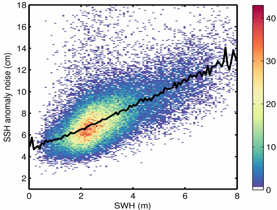
Figure 9. 2D histogram showing flag-valid SSH anomaly noise as a function of SWH for 01/04/2020. The black line denotes the median SSH anomaly noise as a function of SWH.
