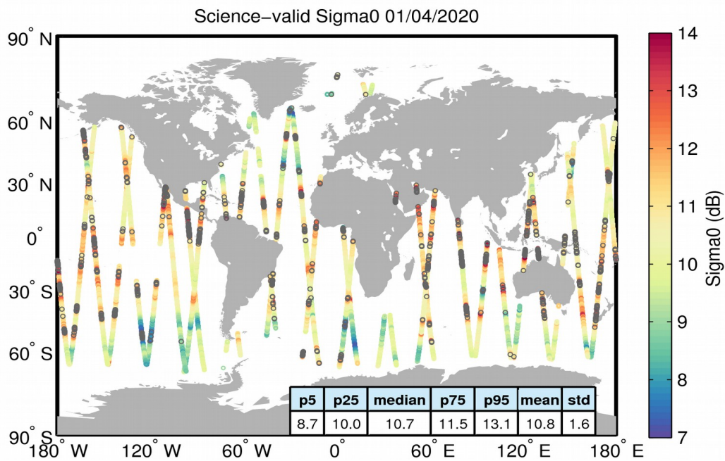
Figure 27. Geographical distribution of science-valid sigma0 data over oceans and lakes for 01/04/2020. The statistical values shown in the table refer to the sigma0 in dB and are calculated over all measurements shown in the figure. Gray circles denote records that have been rejected based on the editing criteria described in Table 4.
