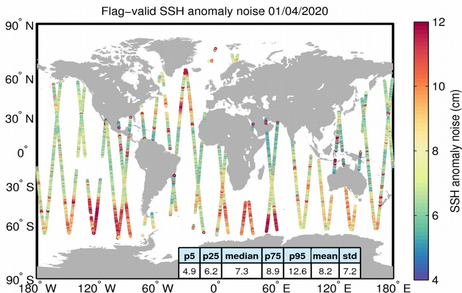
Figure 8. Geographical distribution of flag-valid 20-Hz SSH anomaly measurement noise over oceans and lakes for 01/04/2020. The statistical values shown in the table refer to the SSH anomaly noise and are calculated over all measurements shown in the figure.
