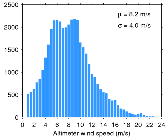
Figure 33. Histogram of flag-valid wind over oceans and lakes for 01/04/2020. The mean ( \mu ) and standard deviation ( \sigma ) are also shown. Note that values larger than 24 m/s are excluded from the histogram for the sake of readability but not from the computation of \mu and \sigma .
