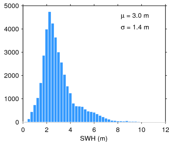
Figure 20. Histogram of science-valid SWH over oceans and lakes for 01/04/2020. The mean ( \mu ) and standard deviation ( \sigma ) are also shown. Note that values larger than 12 m are excluded from the histogram for the sake of readability but not from the computation of \mu and \sigma .
