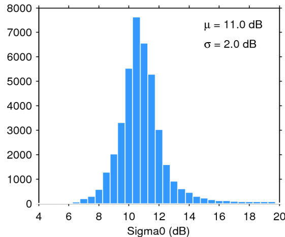
Figure 25. Histogram of flag-valid sigma0 over oceans and lakes for 01/04/2020. The mean ( \mu ) and standard deviation ( \sigma ) are also shown. Note that values outside [4 20] dB are excluded from the histogram for the sake of readability but not from the computation of \mu and \sigma .
