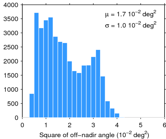
Figure 39. Histogram of flag-valid mispointing over oceans and lakes for 01/04/2020. The mean ( \mu ) and standard deviation ( \sigma ) are also shown. Note that values larger than 6 \cdot 10^{-2} \text{ deg}^2 are excluded from the histogram for the sake of readability but not from the computation of \mu and \sigma .
