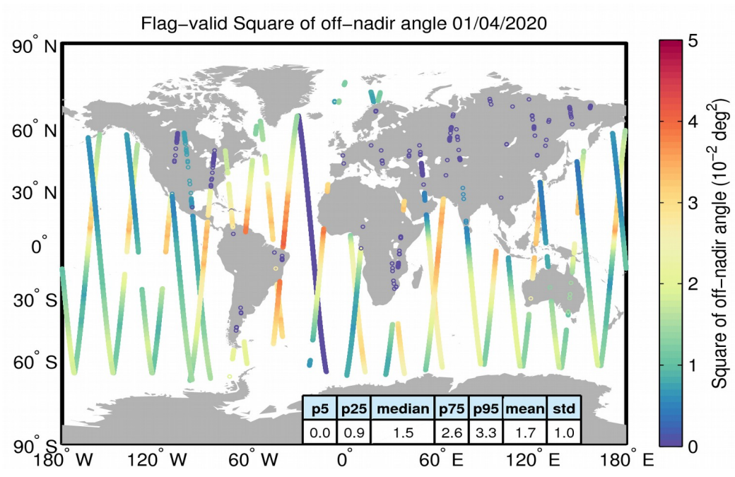
Figure 37. Geographical distribution of flag-valid mispointing data over oceans and lakes for 01/04/2020. The statistical values shown in the table refer to the mispointing in 10^{-2} \text{ deg}^2 and are calculated over all measurements shown in the figure.
