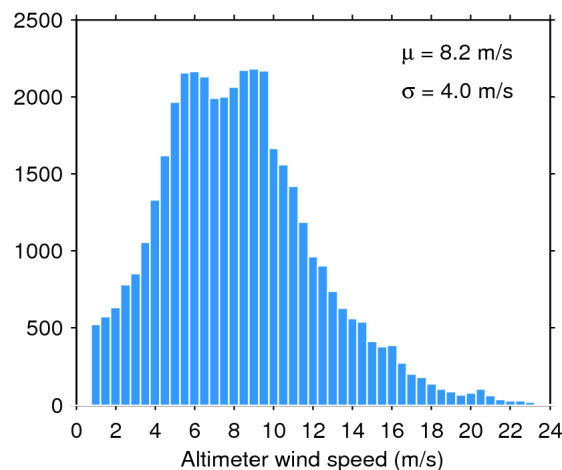
Figure 35. Histogram of science-valid wind over oceans and lakes for 01/04/2020. The mean ( \mu ) and standard deviation ( \sigma ) are also shown. Note that values larger than 24 m/s are excluded from the histogram for the sake of readability but not from the computation of \mu and \sigma .
