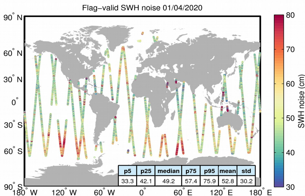
Figure 18. Geographical distribution of flag-valid 20-Hz SWH measurement noise over oceans and lakes for 01/04/2020. The statistical values shown in the figure refer to the SWH noise and are calculated over all measurements shown in the figure.
