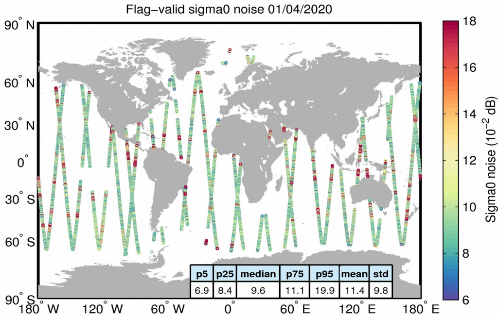
Figure 26. Geographical distribution of flag-valid 20-Hz sigma0 measurement noise over oceans and lakes for 01/04/2020. The statistical values shown in the table refer to the sigma0 noise and are calculated over all measurements shown in the figure.
