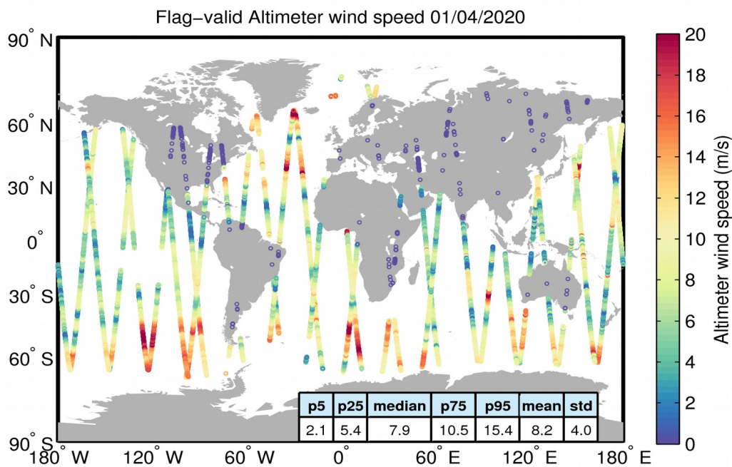
Figure 31. Geographical distribution of flag-valid wind data over oceans and lakes for 01/04/2020. The statistical values shown in the table refer to the wind in m/s and are calculated over all measurements shown in the figure.
