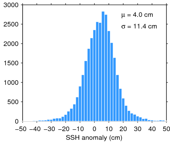
Figure 11. Histogram of science-valid SSH anomaly over oceans and lakes for 01/04/2020. The mean ( \mu ) and standard deviation ( \sigma ) are also shown. Note that values outside [-50 50] cm are excluded from the histogram for the sake of readability but not from the computation of \mu and \sigma .
