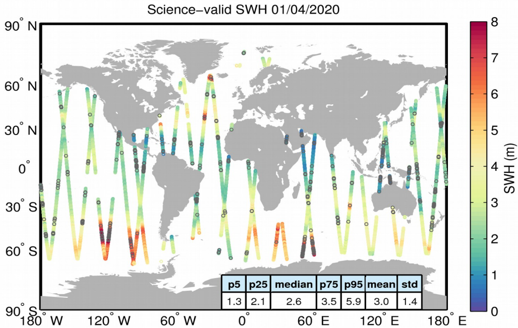
Figure 19. Geographical distribution of science-valid SWH data over oceans and lakes for 01/04/2020. The statistical values shown in the table refer to the SWH in m and are calculated over all measurements shown in the figure. Gray circles denote records that have been rejected based on the editing criteria described in Table 3.
