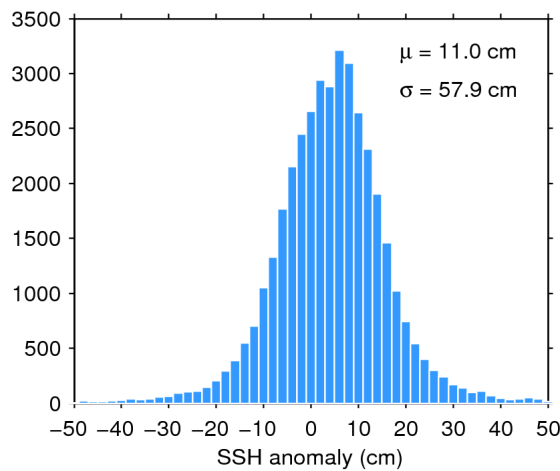
Figure 7. Histogram of flag-valid SSH anomaly over oceans and lakes for 01/04/2020. The mean ( \mu ) and standard deviation ( \sigma ) are also shown. Note that values outside [-50\ 50] cm are excluded from the histogram for the sake of readability but not from the computation of \mu and \sigma .
