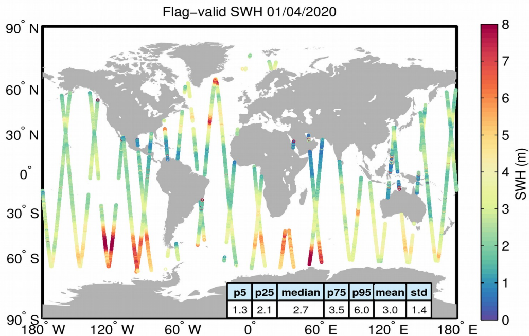
Figure 15. Geographical distribution of flag-valid SWH data over oceans and lakes for 01/04/2020. The statistical values shown in the table refer to the SWH in m and are calculated over all measurements shown in the figure.
