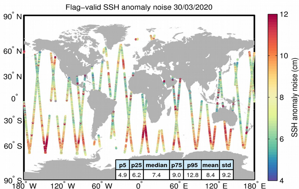
Figure 8. Geographical distribution of flag-valid 20-Hz SSH anomaly measurement noise over oceans and lakes for 30/03/2020. The statistical values shown in the table refer to the SSH anomaly noise and are calculated over all measurements shown in the figure.
