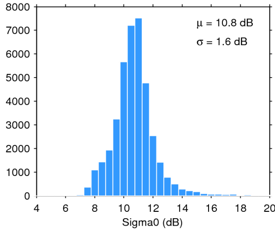
Figure 28. Histogram of science-valid sigma0 over oceans and lakes for 30/03/2020. The mean ( \mu ) and standard deviation ( \sigma ) are also shown. Note that values outside [4 20] dB are excluded from the histogram for the sake of readability but not from the computation of \mu and \sigma .
