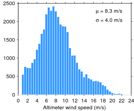
Figure 33. Histogram of flag-valid wind over oceans and lakes for 30/03/2020. The mean ( \mu ) and standard deviation ( \sigma ) are also shown. Note that values larger than 24 m/s are excluded from the histogram for the sake of readability but not from the computation of \mu and \sigma .
