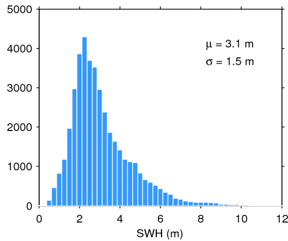
Figure 17. Histogram of flag-valid SWH over oceans and lakes for 30/03/2020. The mean ( \mu ) and standard deviation ( \sigma ) are also shown. Note that values larger than 12 m are excluded from the histogram for the sake of readability but not from the computation of \mu and \sigma .
