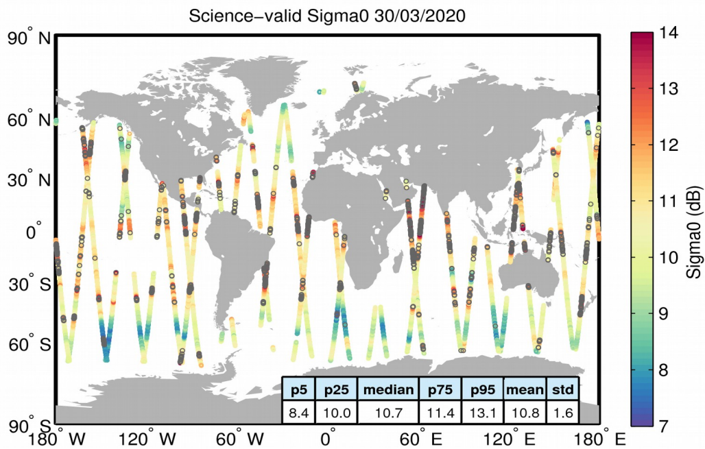
Figure 27. Geographical distribution of science-valid sigma0 data over oceans and lakes for 30/03/2020. The statistical values shown in the table refer to the sigma0 in dB and are calculated over all measurements shown in the figure. Gray circles denote records that have been rejected based on the editing criteria described in Table 4.
