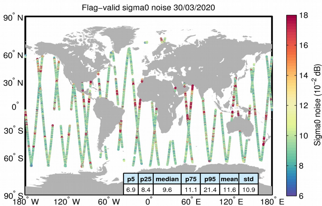
Figure 26. Geographical distribution of flag-valid 20-Hz sigma0 measurement noise over oceans and lakes for 30/03/2020. The statistical values shown in the table refer to the sigma0 noise and are calculated over all measurements shown in the figure.
