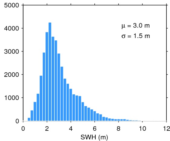
Figure 20. Histogram of science-valid SWH over oceans and lakes for 30/03/2020. The mean ( \mu ) and standard deviation ( \sigma ) are also shown. Note that values larger than 12 m are excluded from the histogram for the sake of readability but not from the computation of \mu and \sigma .
