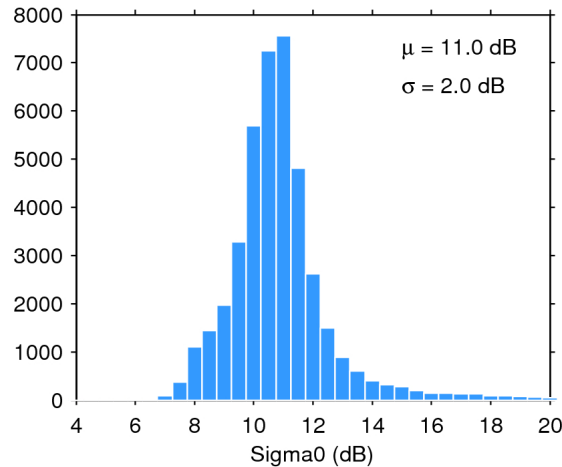
Figure 25. Histogram of flag-valid sigma0 over oceans and lakes for 30/03/2020. The mean ( \mu ) and standard deviation ( \sigma ) are also shown. Note that values outside [4 20] dB are excluded from the histogram for the sake of readability but not from the computation of \mu and \sigma .
