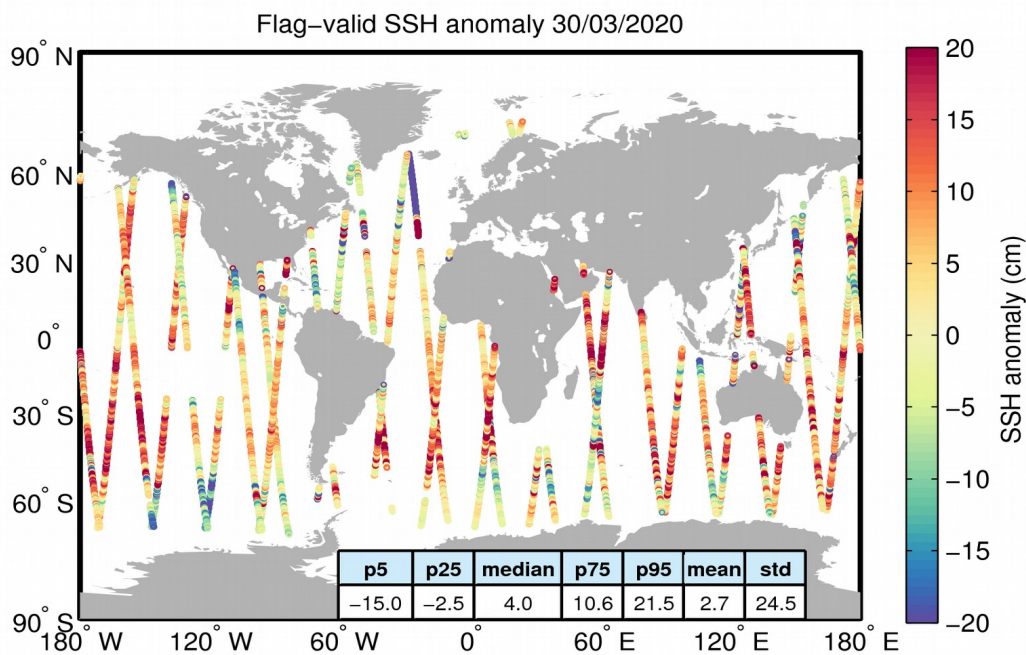
Figure 5. Geographical distribution of flag-valid 1-Hz SSH anomaly data over oceans and lakes for 30/03/2020. The statistical values shown in the table refer to the SSH anomaly in cm and are calculated over all measurements shown in the figure.
