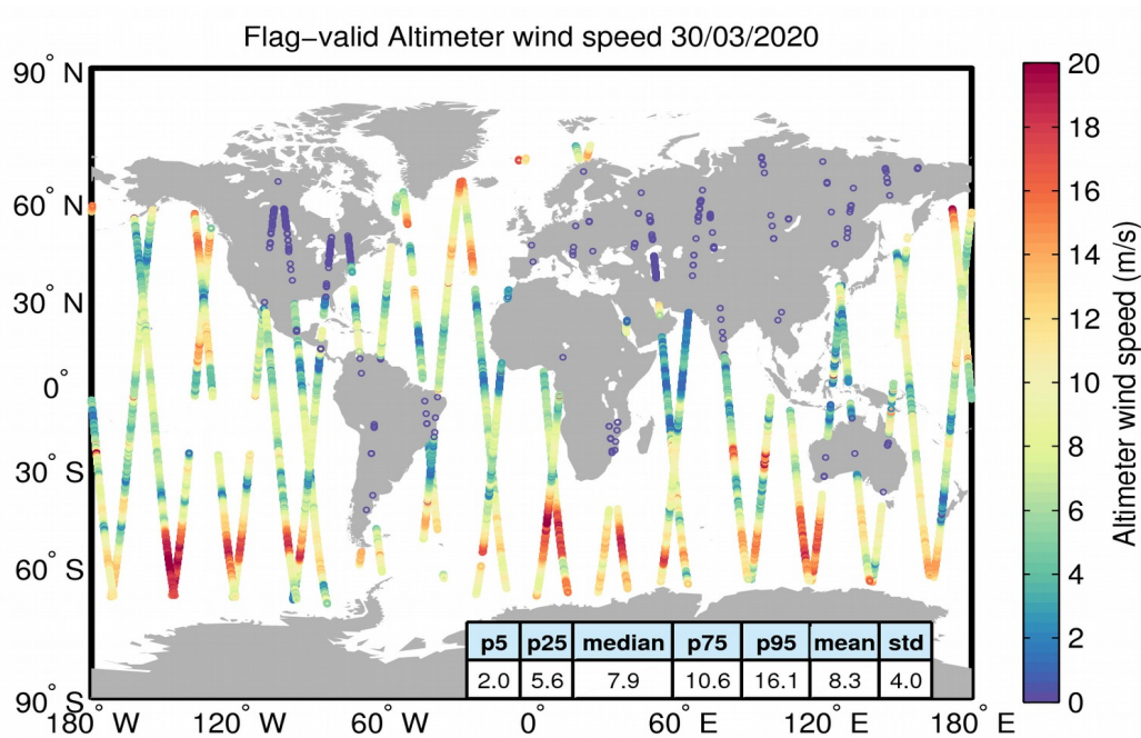
Figure 31. Geographical distribution of flag-valid wind data over oceans and lakes for 30/03/2020. The statistical values shown in the table refer to the wind in m/s and are calculated over all measurements shown in the figure.
