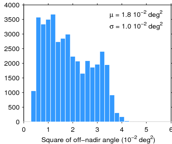
Figure 39. Histogram of flag-valid mispointing over oceans and lakes for 30/03/2020. The mean ( \mu ) and standard deviation ( \sigma ) are also shown. Note that values larger than 6 \cdot 10^{-2} \text{ deg}^2 are excluded from the histogram for the sake of readability but not from the computation of \mu and \sigma .
