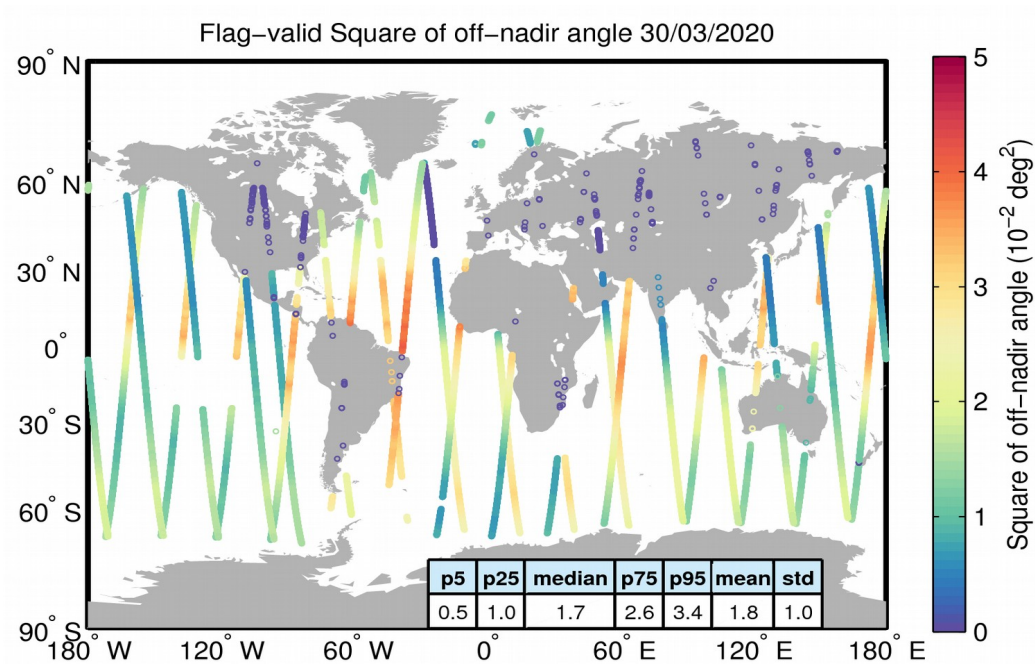
Figure 37. Geographical distribution of flag-valid mispointing data over oceans and lakes for 30/03/2020. The statistical values shown in the table refer to the mispointing in 10^{-2} \text{ deg}^2 and are calculated over all measurements shown in the figure.
