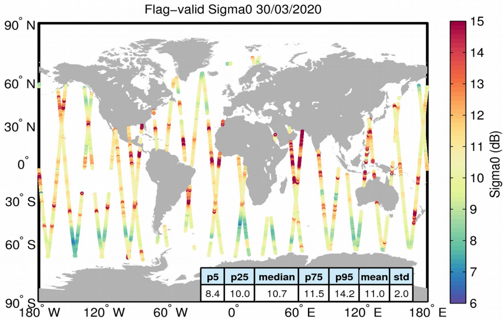
Figure 23. Geographical distribution of flag-valid sigma0 data over oceans and lakes for 30/03/2020. The statistical values shown in the table refer to the sigma0 in dB and are calculated over all measurements shown in the figure.
