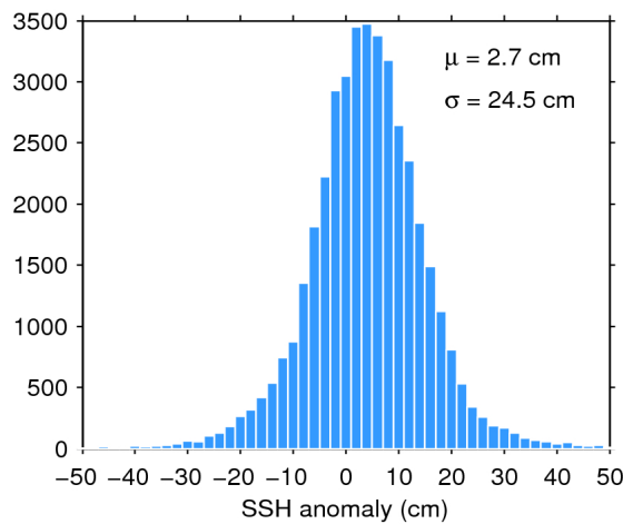
Figure 7. Histogram of flag-valid SSH anomaly over oceans and lakes for 30/03/2020. The mean ( \mu ) and standard deviation ( \sigma ) are also shown. Note that values outside [-50\ 50] cm are excluded from the histogram for the sake of readability but not from the computation of \mu and \sigma .
