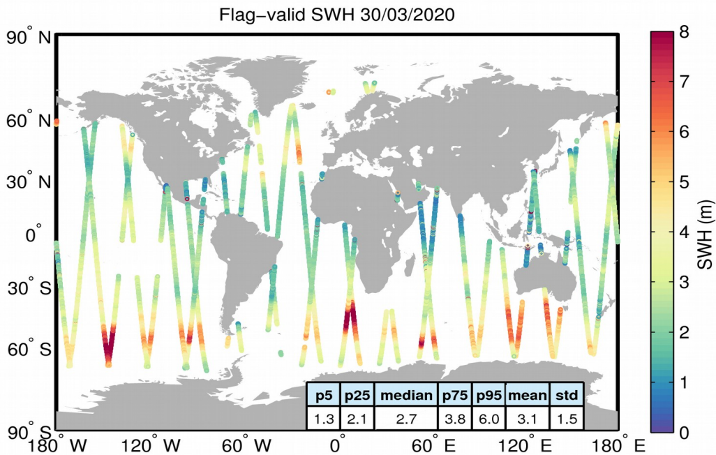
Figure 15. Geographical distribution of flag-valid SWH data over oceans and lakes for 30/03/2020. The statistical values shown in the table refer to the SWH in m and are calculated over all measurements shown in the figure.
