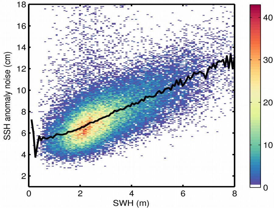
Figure 9. 2D histogram showing flag-valid SSH anomaly noise as a function of SWH for 30/03/2020. The black line denotes the median SSH anomaly noise as a function of SWH.
