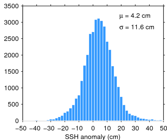
Figure 11. Histogram of science-valid SSH anomaly over oceans and lakes for 30/03/2020. The mean ( \mu ) and standard deviation ( \sigma ) are also shown. Note that values outside [-50 50] cm are excluded from the histogram for the sake of readability but not from the computation of \mu and \sigma .
