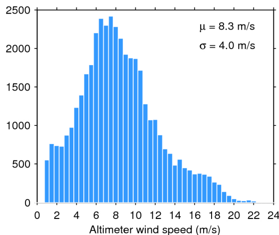
Figure 35. Histogram of science-valid wind over oceans and lakes for 30/03/2020. The mean ( \mu ) and standard deviation ( \sigma ) are also shown. Note that values larger than 24 m/s are excluded from the histogram for the sake of readability but not from the computation of \mu and \sigma .
