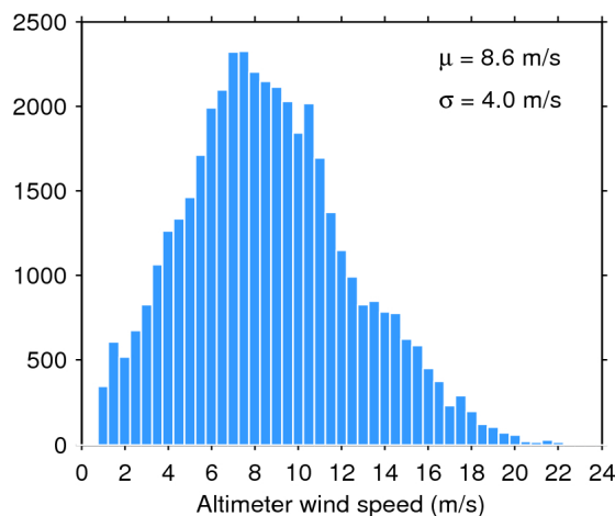
Figure 35. Histogram of science-valid wind over oceans and lakes for 29/03/2020. The mean ( \mu ) and standard deviation ( \sigma ) are also shown. Note that values larger than 24 m/s are excluded from the histogram for the sake of readability but not from the computation of \mu and \sigma .
