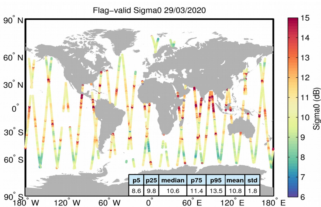
Figure 23. Geographical distribution of flag-valid sigma0 data over oceans and lakes for 29/03/2020. The statistical values shown in the table refer to the sigma0 in dB and are calculated over all measurements shown in the figure.
