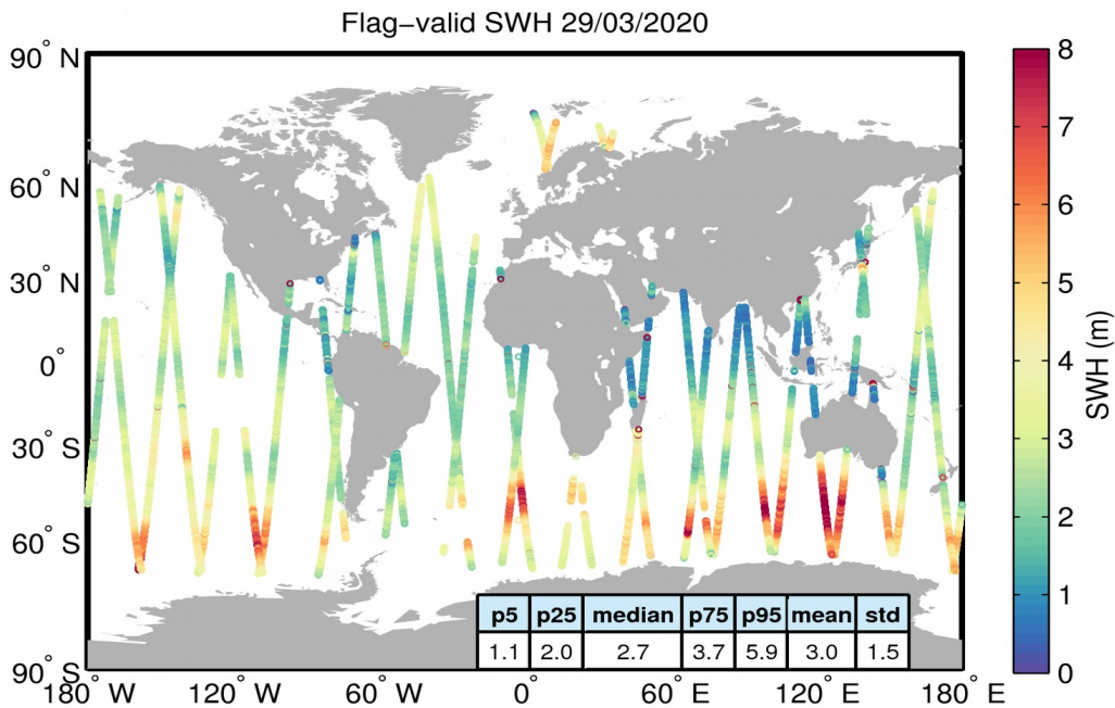
Figure 15. Geographical distribution of flag-valid SWH data over oceans and lakes for 29/03/2020. The statistical values shown in the table refer to the SWH in m and are calculated over all measurements shown in the figure.
