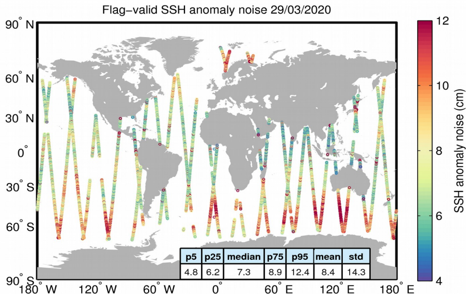
Figure 8. Geographical distribution of flag-valid 20-Hz SSH anomaly measurement noise over oceans and lakes for 29/03/2020. The statistical values shown in the table refer to the SSH anomaly noise and are calculated over all measurements shown in the figure.
