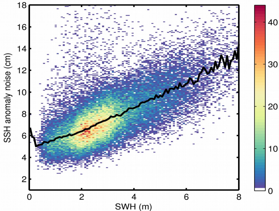
Figure 9. 2D histogram showing flag-valid SSH anomaly noise as a function of SWH for 29/03/2020. The black line denotes the median SSH anomaly noise as a function of SWH.
