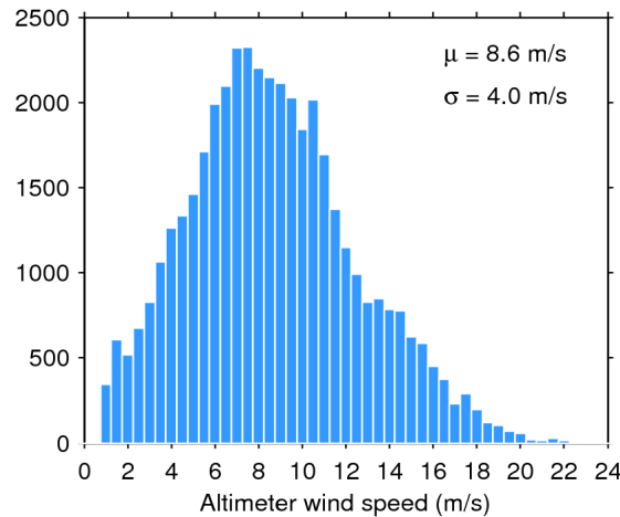
Figure 33. Histogram of flag-valid wind over oceans and lakes for 29/03/2020. The mean ( \mu ) and standard deviation ( \sigma ) are also shown. Note that values larger than 24 m/s are excluded from the histogram for the sake of readability but not from the computation of \mu and \sigma .
