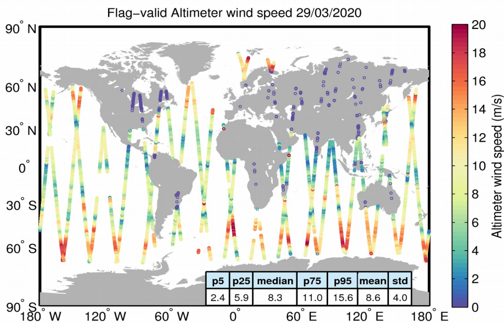
Figure 31. Geographical distribution of flag-valid wind data over oceans and lakes for 29/03/2020. The statistical values shown in the table refer to the wind in m/s and are calculated over all measurements shown in the figure.
