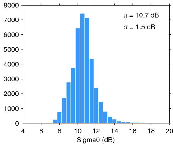
Figure 28. Histogram of science-valid sigma0 over oceans and lakes for 29/03/2020. The mean ( \mu ) and standard deviation ( \sigma ) are also shown. Note that values outside [4 20] dB are excluded from the histogram for the sake of readability but not from the computation of \mu and \sigma .
