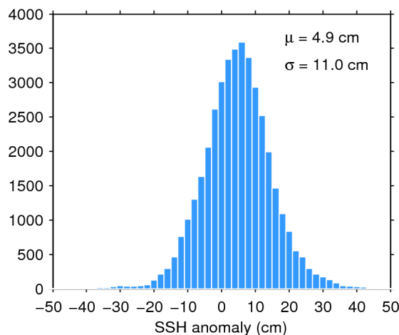
Figure 11. Histogram of science-valid SSH anomaly over oceans and lakes for 29/03/2020. The mean ( \mu ) and standard deviation ( \sigma ) are also shown. Note that values outside [-50 50] cm are excluded from the histogram for the sake of readability but not from the computation of \mu and \sigma .
