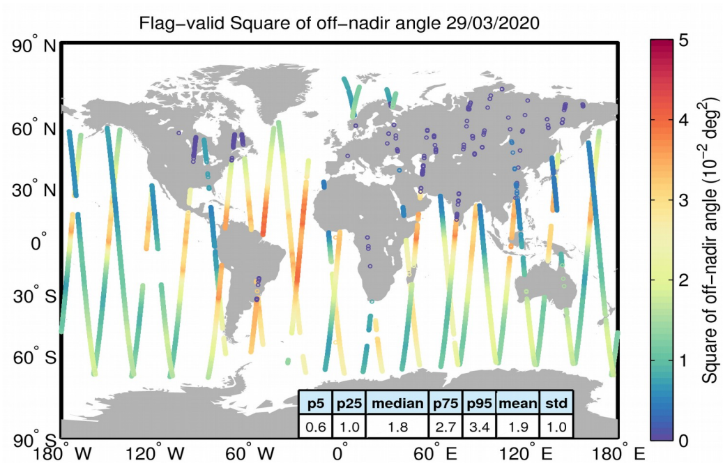
Figure 37. Geographical distribution of flag-valid mispointing data over oceans and lakes for 29/03/2020. The statistical values shown in the table refer to the mispointing in 10^{-2} deg 2 and are calculated over all measurements shown in the figure.
