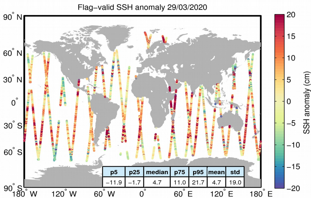
Figure 5. Geographical distribution of flag-valid 1-Hz SSH anomaly data over oceans and lakes for 29/03/2020. The statistical values shown in the table refer to the SSH anomaly in cm and are calculated over all measurements shown in the figure.
