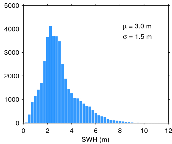
Figure 17. Histogram of flag-valid SWH over oceans and lakes for 29/03/2020. The mean ( \mu ) and standard deviation ( \sigma ) are also shown. Note that values larger than 12 m are excluded from the histogram for the sake of readability but not from the computation of \mu and \sigma .
