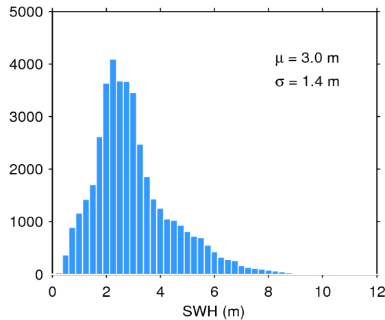
Figure 20. Histogram of science-valid SWH over oceans and lakes for 29/03/2020. The mean ( \mu ) and standard deviation ( \sigma ) are also shown. Note that values larger than 12 m are excluded from the histogram for the sake of readability but not from the computation of \mu and \sigma .
