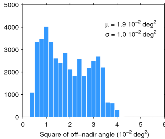
Figure 39. Histogram of flag-valid mispointing over oceans and lakes for 29/03/2020. The mean ( \mu ) and standard deviation ( \sigma ) are also shown. Note that values larger than 6 \cdot 10^{-2} \text{ deg}^2 are excluded from the histogram for the sake of readability but not from the computation of \mu and \sigma .
