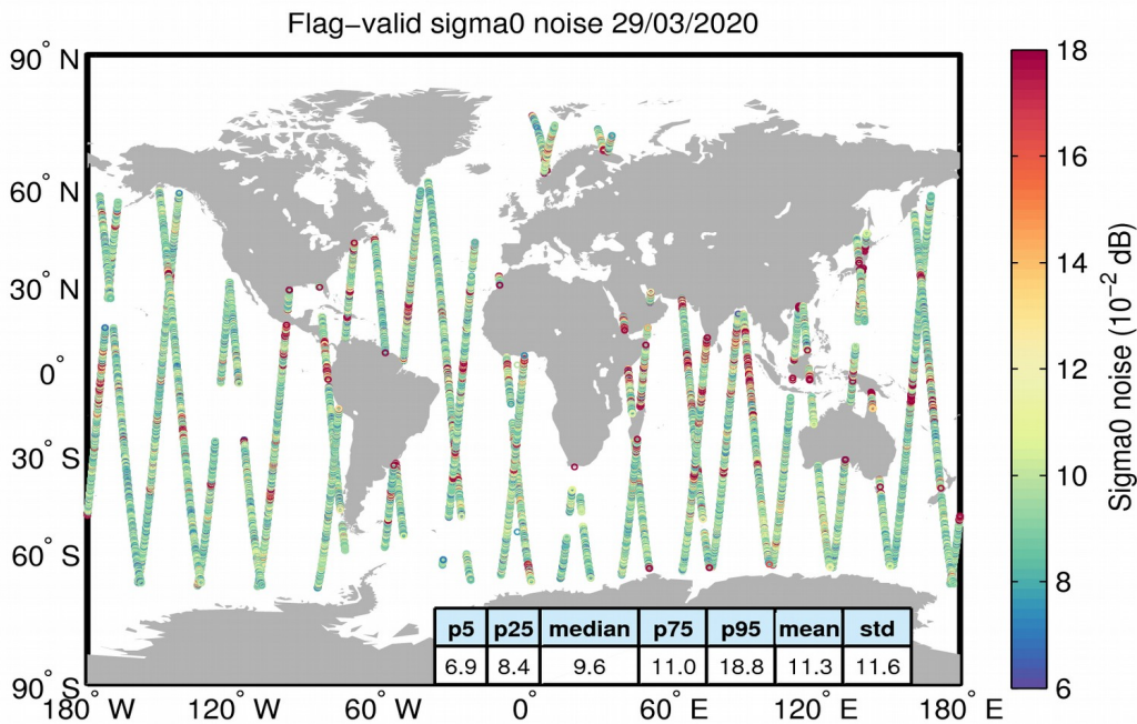
Figure 26. Geographical distribution of flag-valid 20-Hz sigma0 measurement noise over oceans and lakes for 29/03/2020. The statistical values shown in the figure refer to the sigma0 noise and are calculated over all measurements shown in the figure.
