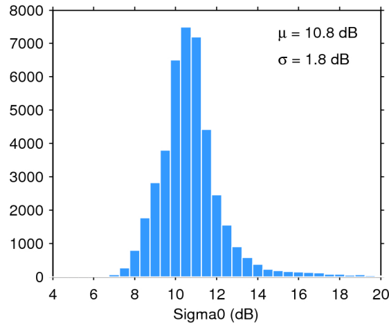
Figure 25. Histogram of flag-valid sigma0 over oceans and lakes for 29/03/2020. The mean ( \mu ) and standard deviation ( \sigma ) are also shown. Note that values outside [4 20] dB are excluded from the histogram for the sake of readability but not from the computation of \mu and \sigma .
