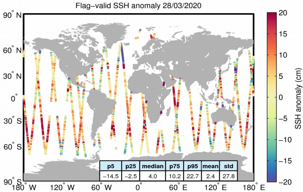
Figure 5. Geographical distribution of flag-valid 1-Hz SSH anomaly data over oceans and lakes for 28/03/2020. The statistical values shown in the table refer to the SSH anomaly in cm and are calculated over all measurements shown in the figure.
