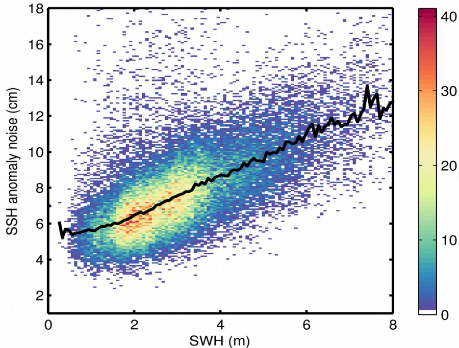
Figure 9. 2D histogram showing flag-valid SSH anomaly noise as a function of SWH for 28/03/2020. The black line denotes the median SSH anomaly noise as a function of SWH.
