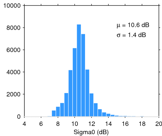
Figure 28. Histogram of science-valid sigma0 over oceans and lakes for 28/03/2020. The mean ( \mu ) and standard deviation ( \sigma ) are also shown. Note that values outside [4 20] dB are excluded from the histogram for the sake of readability but not from the computation of \mu and \sigma .
