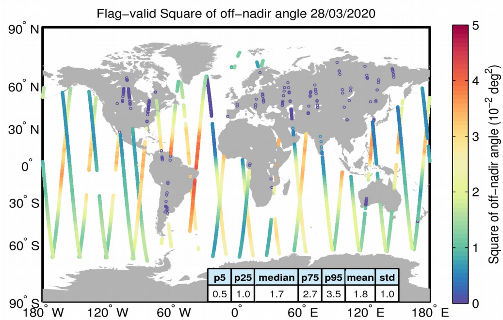
Figure 37. Geographical distribution of flag-valid mispointing data over oceans and lakes for 28/03/2020. The statistical values shown in the table refer to the mispointing in 10^{-2} \text{ deg}^2 and are calculated over all measurements shown in the figure.
