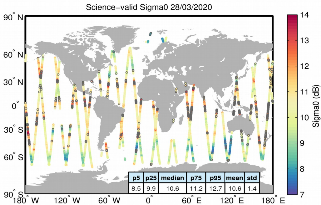
Figure 27. Geographical distribution of science-valid sigma0 data over oceans and lakes for 28/03/2020. The statistical values shown in the table refer to the sigma0 in dB and are calculated over all measurements shown in the figure. Gray circles denote records that have been rejected based on the editing criteria described in Table 4.
