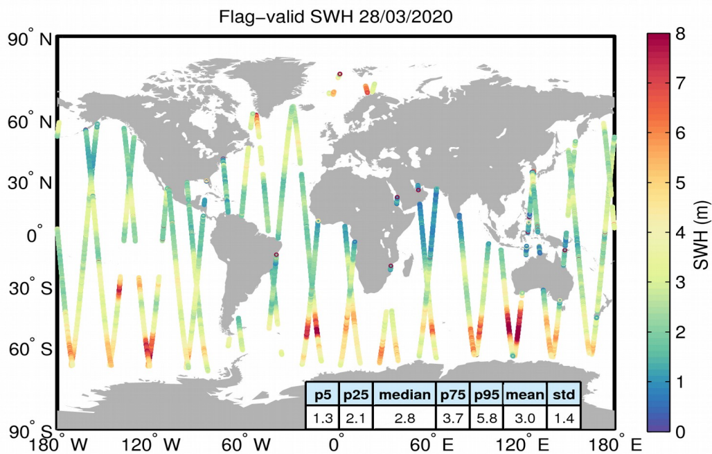
Figure 15. Geographical distribution of flag-valid SWH data over oceans and lakes for 28/03/2020. The statistical values shown in the table refer to the SWH in m and are calculated over all measurements shown in the figure.
