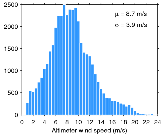
Figure 33. Histogram of flag-valid wind over oceans and lakes for 28/03/2020. The mean ( \mu ) and standard deviation ( \sigma ) are also shown. Note that values larger than 24 m/s are excluded from the histogram for the sake of readability but not from the computation of \mu and \sigma .
