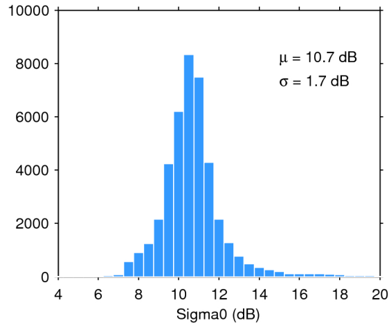
Figure 25. Histogram of flag-valid sigma0 over oceans and lakes for 28/03/2020. The mean ( \mu ) and standard deviation ( \sigma ) are also shown. Note that values outside [4 20] dB are excluded from the histogram for the sake of readability but not from the computation of \mu and \sigma .
