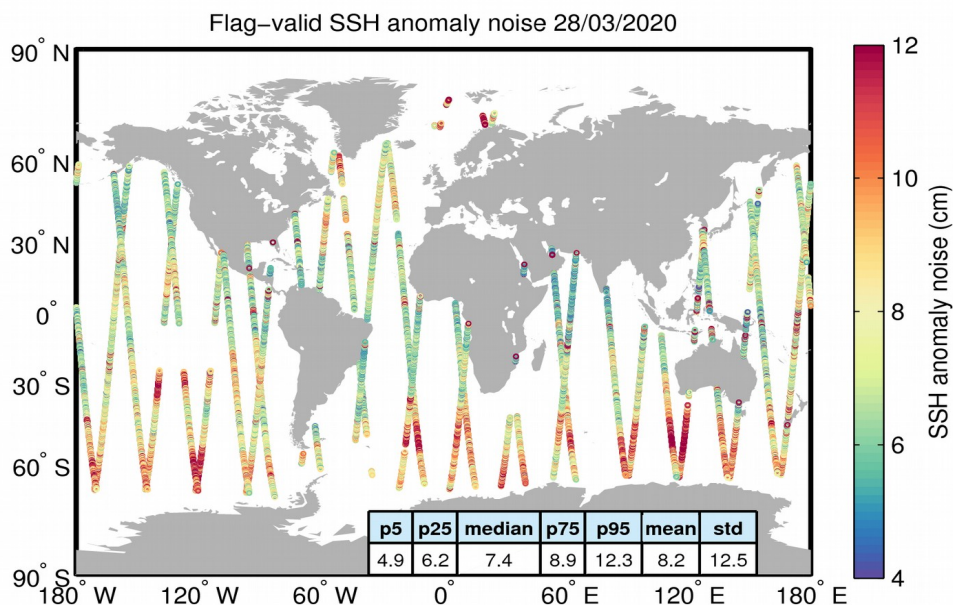
Figure 8. Geographical distribution of flag-valid 20-Hz SSH anomaly measurement noise over oceans and lakes for 28/03/2020. The statistical values shown in the table refer to the SSH anomaly noise and are calculated over all measurements shown in the figure.
