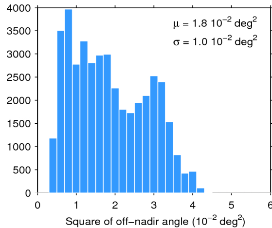
Figure 39. Histogram of flag-valid mispointing over oceans and lakes for 28/03/2020. The mean ( \mu ) and standard deviation ( \sigma ) are also shown. Note that values larger than 6 \cdot 10^{-2} \text{ deg}^2 are excluded from the histogram for the sake of readability but not from the computation of \mu and \sigma .
