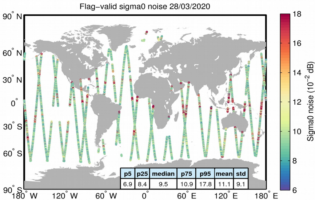
Figure 26. Geographical distribution of flag-valid 20-Hz sigma0 measurement noise over oceans and lakes for 28/03/2020. The statistical values shown in the table refer to the sigma0 noise and are calculated over all measurements shown in the figure.
