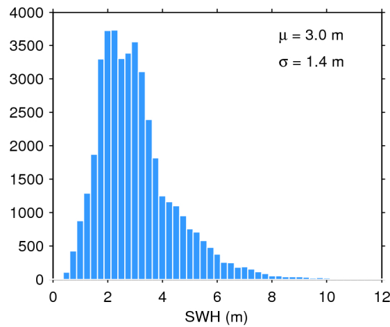
Figure 17. Histogram of flag-valid SWH over oceans and lakes for 28/03/2020. The mean ( \mu ) and standard deviation ( \sigma ) are also shown. Note that values larger than 12 m are excluded from the histogram for the sake of readability but not from the computation of \mu and \sigma .
