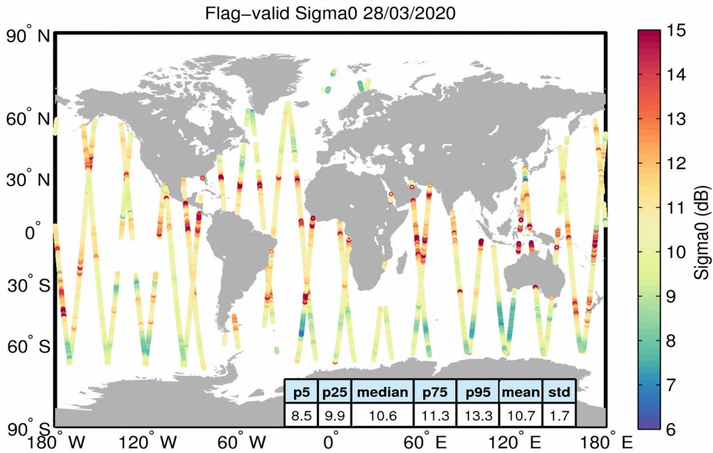
Figure 23. Geographical distribution of flag-valid sigma0 data over oceans and lakes for 28/03/2020. The statistical values shown in the table refer to the sigma0 in dB and are calculated over all measurements shown in the figure.
