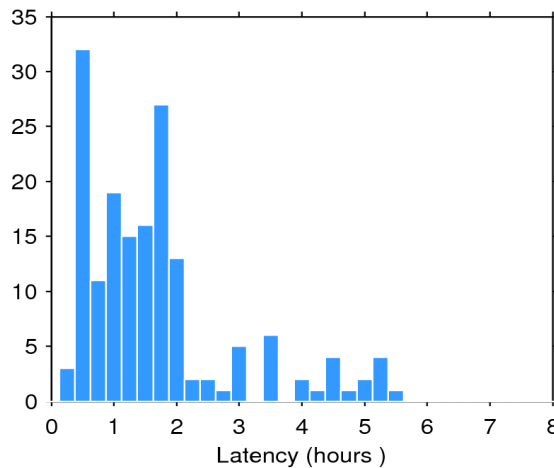
Figure 2. Histogram of the data latency for 27/03/2020. The y-axis denotes the number of files that are made available with a delay of x-hours with respect to the mean time of the records stored in the file.
