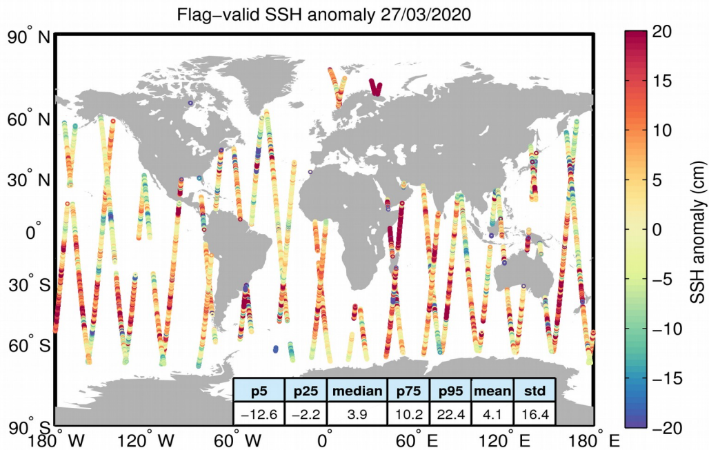
Figure 5. Geographical distribution of flag-valid 1-Hz SSH anomaly data over oceans and lakes for 27/03/2020. The statistical values shown in the table refer to the SSH anomaly in cm and are calculated over all measurements shown in the figure.
