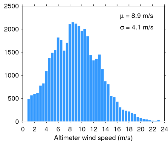
Figure 35. Histogram of science-valid wind over oceans and lakes for 27/03/2020. The mean ( \mu ) and standard deviation ( \sigma ) are also shown. Note that values larger than 24 m/s are excluded from the histogram for the sake of readability but not from the computation of \mu and \sigma .
