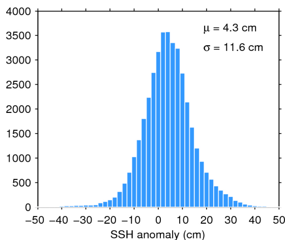
Figure 11. Histogram of science-valid SSH anomaly over oceans and lakes for 27/03/2020. The mean ( \mu ) and standard deviation ( \sigma ) are also shown. Note that values outside [-50 50] cm are excluded from the histogram for the sake of readability but not from the computation of \mu and \sigma .
