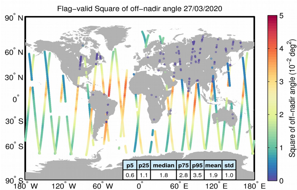
Figure 37. Geographical distribution of flag-valid mispointing data over oceans and lakes for 27/03/2020. The statistical values shown in the table refer to the mispointing in 10^{-2} \text{ deg}^2 and are calculated over all measurements shown in the figure.
