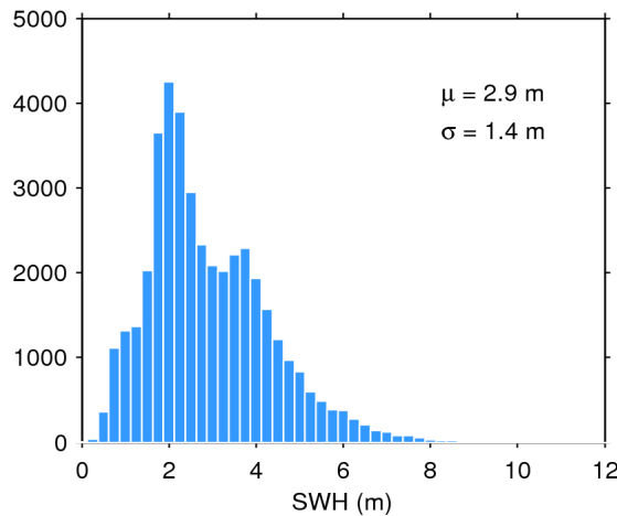
Figure 20. Histogram of science-valid SWH over oceans and lakes for 27/03/2020. The mean ( \mu ) and standard deviation ( \sigma ) are also shown. Note that values larger than 12 m are excluded from the histogram for the sake of readability but not from the computation of \mu and \sigma .
