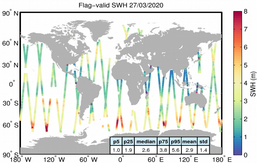
Figure 15. Geographical distribution of flag-valid SWH data over oceans and lakes for 27/03/2020. The statistical values shown in the table refer to the SWH in m and are calculated over all measurements shown in the figure.
