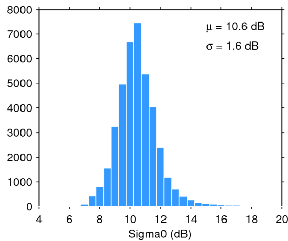
Figure 28. Histogram of science-valid sigma0 over oceans and lakes for 27/03/2020. The mean ( \mu ) and standard deviation ( \sigma ) are also shown. Note that values outside [4 20] dB are excluded from the histogram for the sake of readability but not from the computation of \mu and \sigma .
