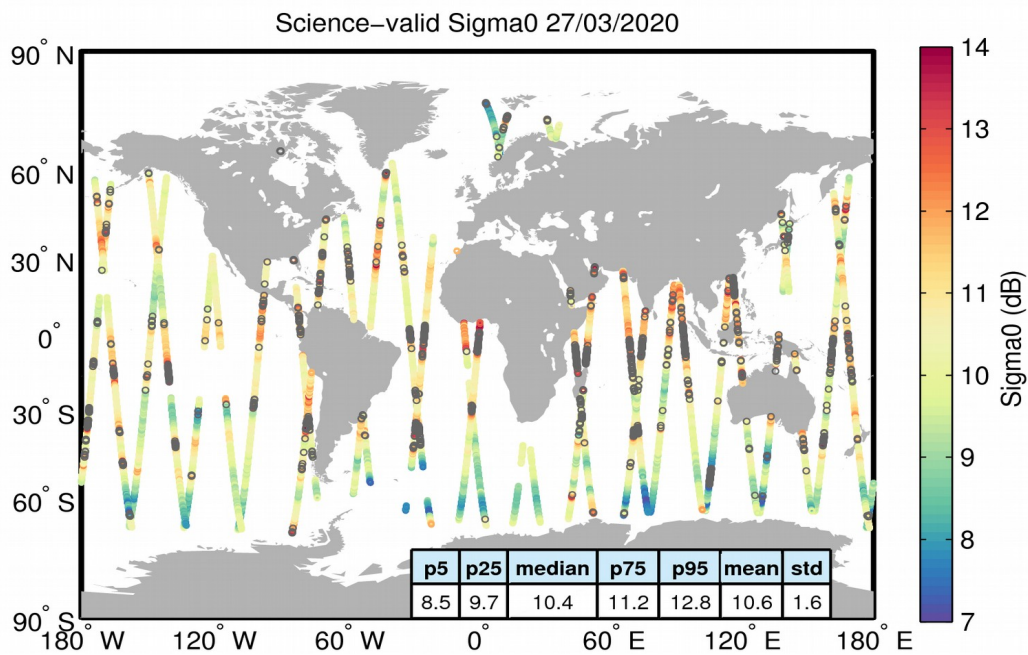
Figure 27. Geographical distribution of science-valid sigma0 data over oceans and lakes for 27/03/2020. The statistical values shown in the table refer to the sigma0 in dB and are calculated over all measurements shown in the figure. Gray circles denote records that have been rejected based on the editing criteria described in Table 4.
