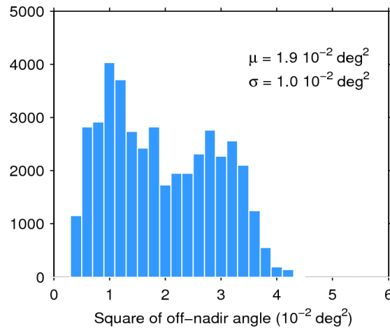
Figure 39. Histogram of flag-valid mispointing over oceans and lakes for 27/03/2020. The mean ( \mu ) and standard deviation ( \sigma ) are also shown. Note that values larger than 6 \cdot 10^{-2} \text{ deg}^2 are excluded from the histogram for the sake of readability but not from the computation of \mu and \sigma .
