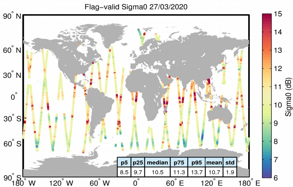
Figure 23. Geographical distribution of flag-valid sigma0 data over oceans and lakes for 27/03/2020. The statistical values shown in the table refer to the sigma0 in dB and are calculated over all measurements shown in the figure.
