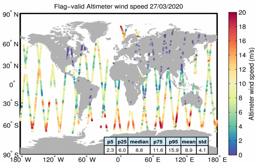
Figure 31. Geographical distribution of flag-valid wind data over oceans and lakes for 27/03/2020. The statistical values shown in the table refer to the wind in m/s and are calculated over all measurements shown in the figure.
