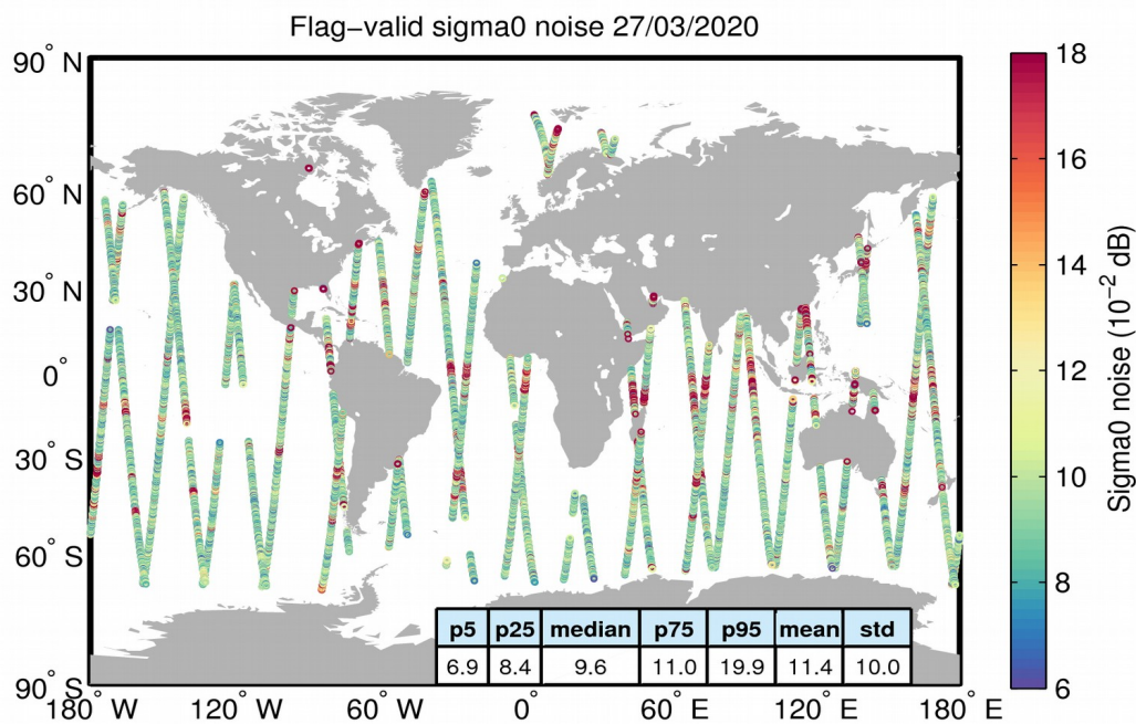
Figure 26. Geographical distribution of flag-valid 20-Hz sigma0 measurement noise over oceans and lakes for 27/03/2020. The statistical values shown in the table refer to the sigma0 noise and are calculated over all measurements shown in the figure.
