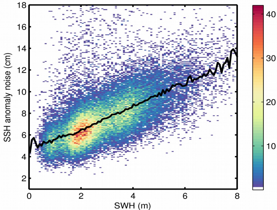
Figure 9. 2D histogram showing flag-valid SSH anomaly noise as a function of SWH for 27/03/2020. The black line denotes the median SSH anomaly noise as a function of SWH.
