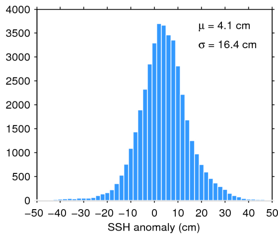
Figure 7. Histogram of flag-valid SSH anomaly over oceans and lakes for 27/03/2020. The mean ( \mu ) and standard deviation ( \sigma ) are also shown. Note that values outside [-50 50] cm are excluded from the histogram for the sake of readability but not from the computation of \mu and \sigma .
