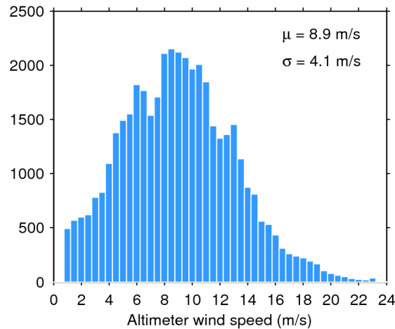
Figure 33. Histogram of flag-valid wind over oceans and lakes for 27/03/2020. The mean ( \mu ) and standard deviation ( \sigma ) are also shown. Note that values larger than 24 m/s are excluded from the histogram for the sake of readability but not from the computation of \mu and \sigma .
