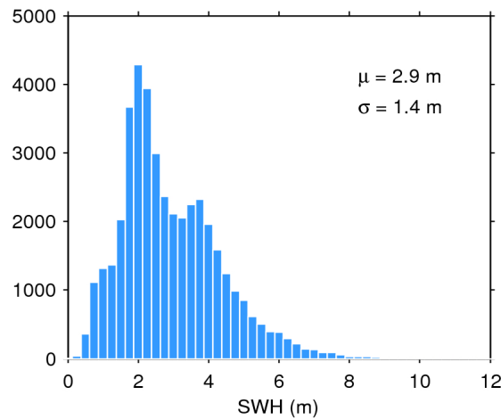
Figure 17. Histogram of flag-valid SWH over oceans and lakes for 27/03/2020. The mean ( \mu ) and standard deviation ( \sigma ) are also shown. Note that values larger than 12 m are excluded from the histogram for the sake of readability but not from the computation of \mu and \sigma .
