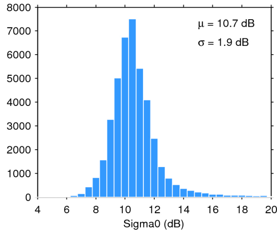
Figure 25. Histogram of flag-valid sigma0 over oceans and lakes for 27/03/2020. The mean ( \mu ) and standard deviation ( \sigma ) are also shown. Note that values outside [4 20] dB are excluded from the histogram for the sake of readability but not from the computation of \mu and \sigma .
