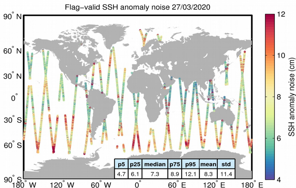
Figure 8. Geographical distribution of flag-valid 20-Hz SSH anomaly measurement noise over oceans and lakes for 27/03/2020. The statistical values shown in the table refer to the SSH anomaly noise and are calculated over all measurements shown in the figure.
