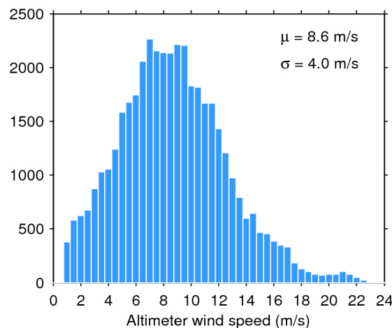
Figure 35. Histogram of science-valid wind over oceans and lakes for 26/03/2020. The mean ( \mu ) and standard deviation ( \sigma ) are also shown. Note that values larger than 24 m/s are excluded from the histogram for the sake of readability but not from the computation of \mu and \sigma .
