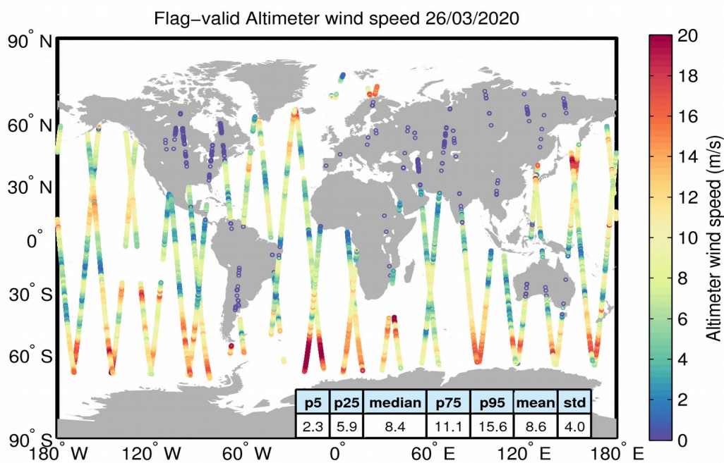
Figure 31. Geographical distribution of flag-valid wind data over oceans and lakes for 26/03/2020. The statistical values shown in the table refer to the wind in m/s and are calculated over all measurements shown in the figure.
