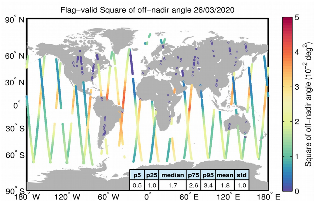
Figure 37. Geographical distribution of flag-valid mispointing data over oceans and lakes for 26/03/2020. The statistical values shown in the table refer to the mispointing in 10^{-2} \text{ deg}^2 and are calculated over all measurements shown in the figure.
