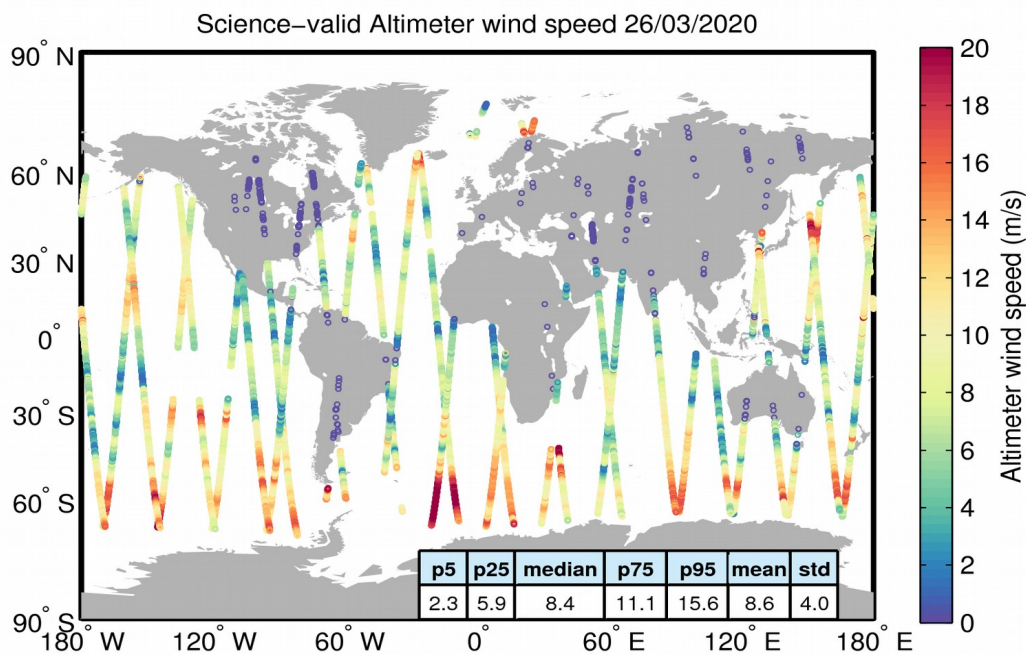
Figure 34. Geographical distribution of science-valid wind data over oceans and lakes for 26/03/2020. The statistical values shown in the table refer to the wind in m/s and are calculated over all measurements shown in the figure. Gray circles denote records that have been rejected based on the editing criteria described in Table 5.
