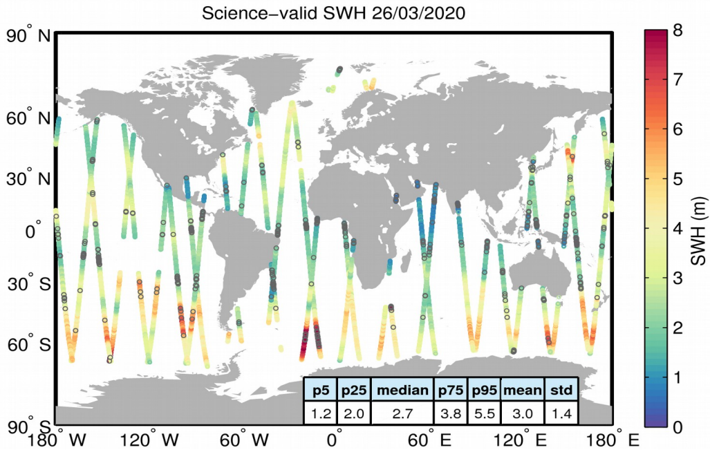
Figure 19. Geographical distribution of science-valid SWH data over oceans and lakes for 26/03/2020. The statistical values shown in the table refer to the SWH in m and are calculated over all measurements shown in the figure. Gray circles denote records that have been rejected based on the editing criteria described in Table 3.
