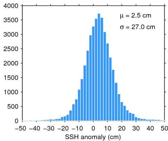
Figure 7. Histogram of flag-valid SSH anomaly over oceans and lakes for 26/03/2020. The mean ( \mu ) and standard deviation ( \sigma ) are also shown. Note that values outside [-50 50] cm are excluded from the histogram for the sake of readability but not from the computation of \mu and \sigma .
