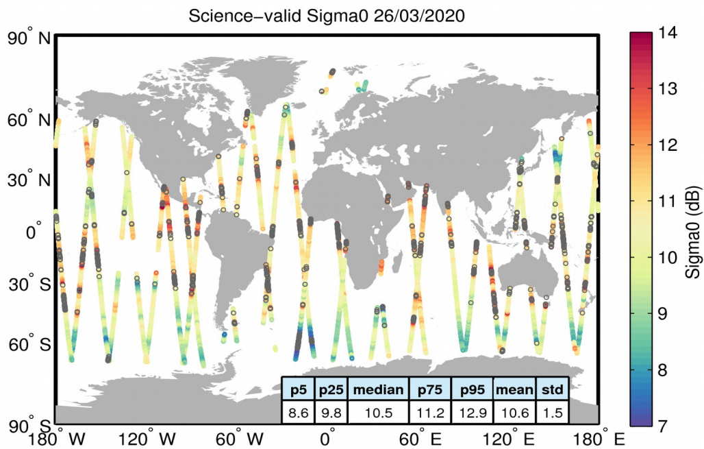
Figure 27. Geographical distribution of science-valid sigma0 data over oceans and lakes for 26/03/2020. The statistical values shown in the table refer to the sigma0 in dB and are calculated over all measurements shown in the figure. Gray circles denote records that have been rejected based on the editing criteria described in Table 4.
