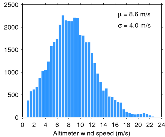
Figure 33. Histogram of flag-valid wind over oceans and lakes for 26/03/2020. The mean ( \mu ) and standard deviation ( \sigma ) are also shown. Note that values larger than 24 m/s are excluded from the histogram for the sake of readability but not from the computation of \mu and \sigma .
