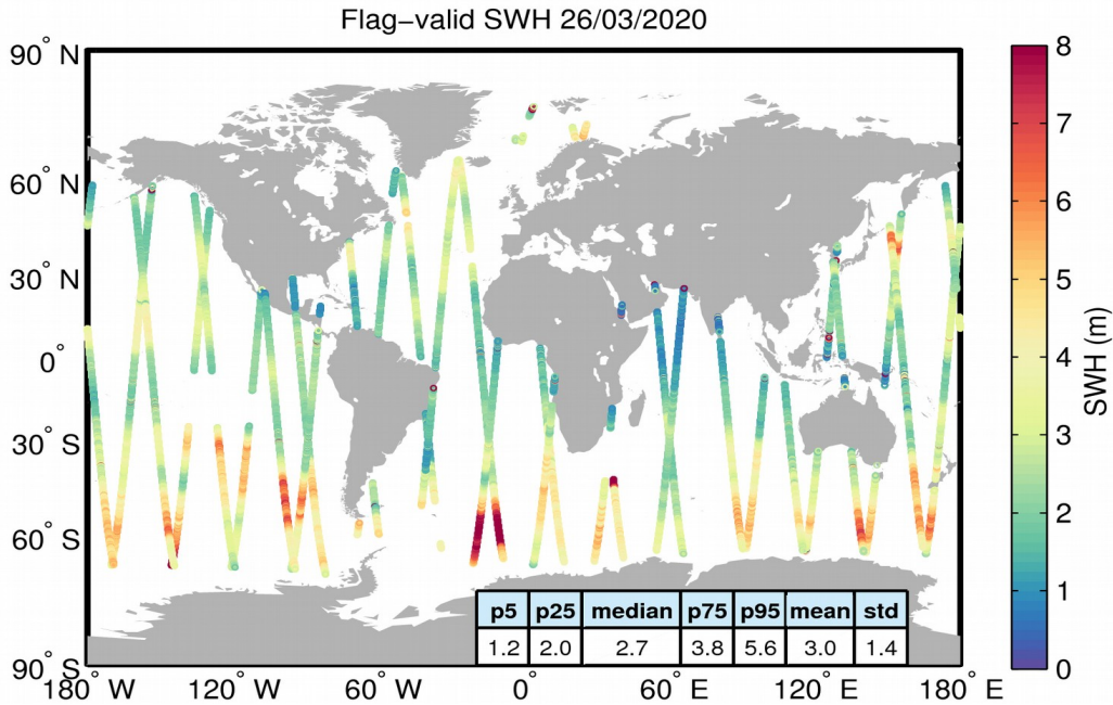
Figure 15. Geographical distribution of flag-valid SWH data over oceans and lakes for 26/03/2020. The statistical values shown in the table refer to the SWH in m and are calculated over all measurements shown in the figure.
