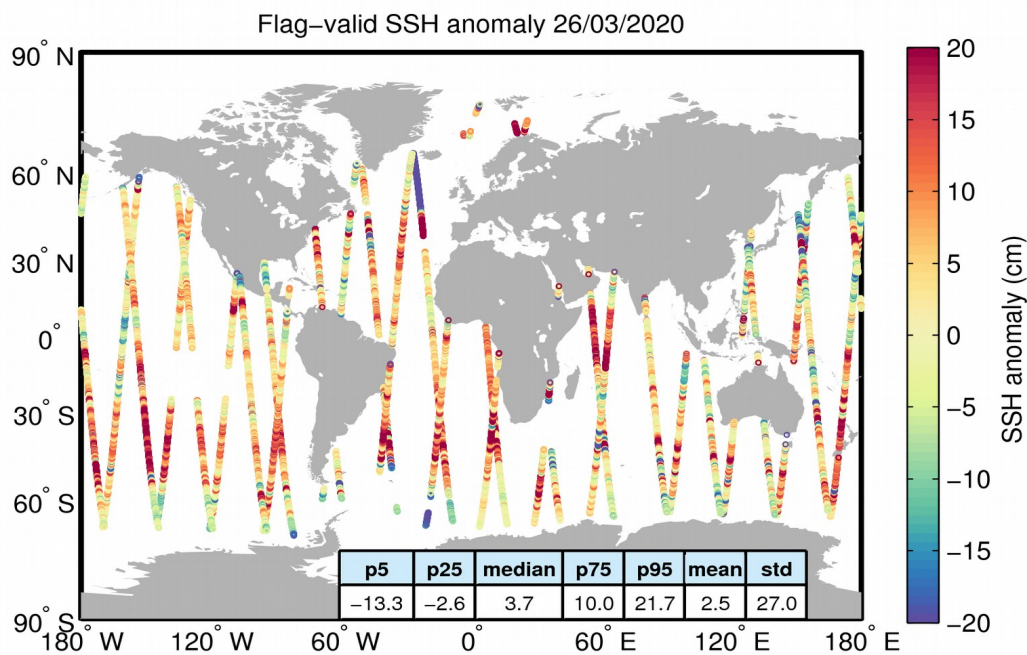
Figure 5. Geographical distribution of flag-valid 1-Hz SSH anomaly data over oceans and lakes for 26/03/2020. The statistical values shown in the table refer to the SSH anomaly in cm and are calculated over all measurements shown in the figure.
