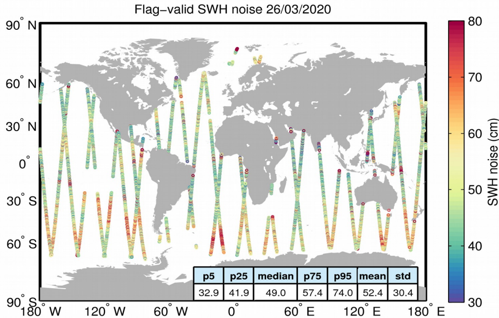
Figure 18. Geographical distribution of flag-valid 20-Hz SWH measurement noise over oceans and lakes for 26/03/2020. The statistical values shown in the figure refer to the SWH noise and are calculated over all measurements shown in the figure.
