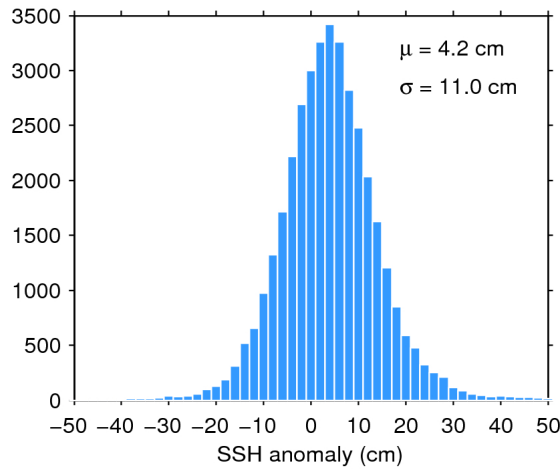
Figure 11. Histogram of science-valid SSH anomaly over oceans and lakes for 26/03/2020. The mean ( \mu ) and standard deviation ( \sigma ) are also shown. Note that values outside [-50 50] cm are excluded from the histogram for the sake of readability but not from the computation of \mu and \sigma .
