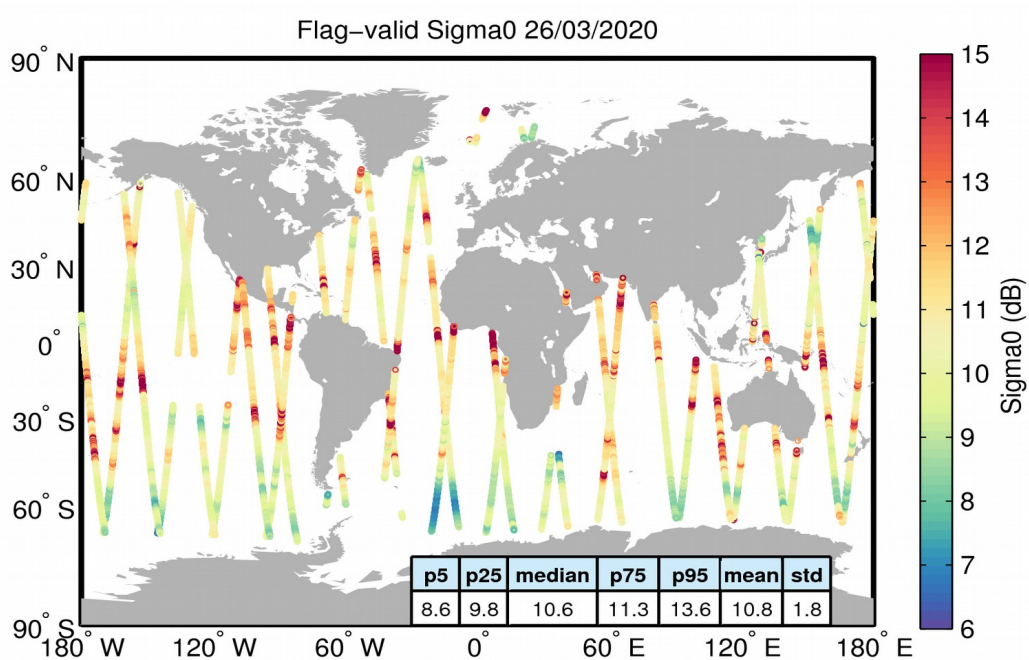
Figure 23. Geographical distribution of flag-valid sigma0 data over oceans and lakes for 26/03/2020. The statistical values shown in the table refer to the sigma0 in dB and are calculated over all measurements shown in the figure.
