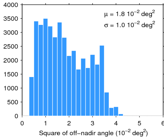
Figure 39. Histogram of flag-valid mispointing over oceans and lakes for 26/03/2020. The mean ( \mu ) and standard deviation ( \sigma ) are also shown. Note that values larger than 6 \cdot 10^{-2} \text{ deg}^2 are excluded from the histogram for the sake of readability but not from the computation of \mu and \sigma .
