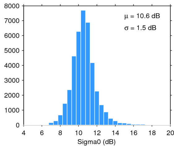
Figure 28. Histogram of science-valid sigma0 over oceans and lakes for 26/03/2020. The mean ( \mu ) and standard deviation ( \sigma ) are also shown. Note that values outside [4 20] dB are excluded from the histogram for the sake of readability but not from the computation of \mu and \sigma .
