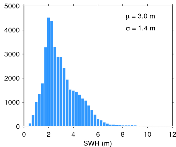
Figure 17. Histogram of flag-valid SWH over oceans and lakes for 26/03/2020. The mean ( \mu ) and standard deviation ( \sigma ) are also shown. Note that values larger than 12 m are excluded from the histogram for the sake of readability but not from the computation of \mu and \sigma .
