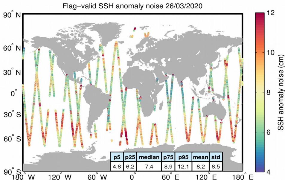
Figure 8. Geographical distribution of flag-valid 20-Hz SSH anomaly measurement noise over oceans and lakes for 26/03/2020. The statistical values shown in the table refer to the SSH anomaly noise and are calculated over all measurements shown in the figure.
