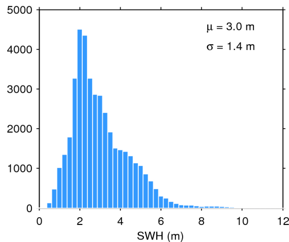
Figure 20. Histogram of science-valid SWH over oceans and lakes for 26/03/2020. The mean ( \mu ) and standard deviation ( \sigma ) are also shown. Note that values larger than 12 m are excluded from the histogram for the sake of readability but not from the computation of \mu and \sigma .
