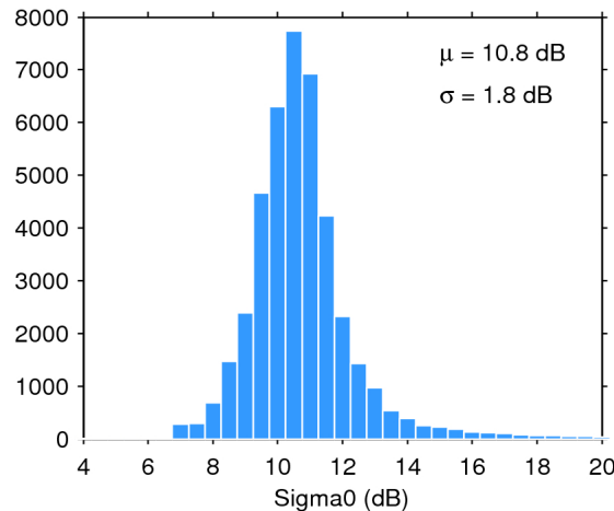
Figure 25. Histogram of flag-valid sigma0 over oceans and lakes for 26/03/2020. The mean ( \mu ) and standard deviation ( \sigma ) are also shown. Note that values outside [4 20] dB are excluded from the histogram for the sake of readability but not from the computation of \mu and \sigma .
