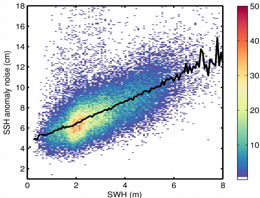
Figure 9. 2D histogram showing flag-valid SSH anomaly noise as a function of SWH for 26/03/2020. The black line denotes the median SSH anomaly noise as a function of SWH.
