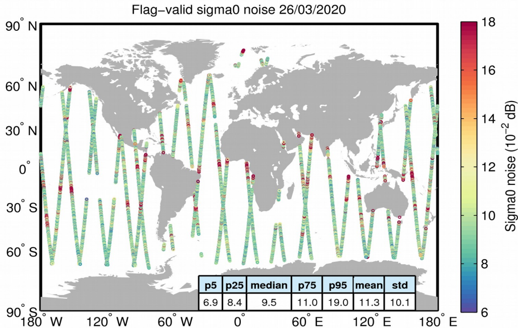
Figure 26. Geographical distribution of flag-valid 20-Hz sigma0 measurement noise over oceans and lakes for 26/03/2020. The statistical values shown in the table refer to the sigma0 noise and are calculated over all measurements shown in the figure.
