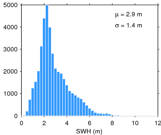
Figure 20. Histogram of science-valid SWH over oceans and lakes for 25/03/2020. The mean ( \mu ) and standard deviation ( \sigma ) are also shown. Note that values larger than 12 m are excluded from the histogram for the sake of readability but not from the computation of \mu and \sigma .
