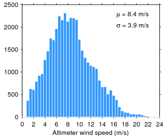
Figure 33. Histogram of flag-valid wind over oceans and lakes for 25/03/2020. The mean ( \mu ) and standard deviation ( \sigma ) are also shown. Note that values larger than 24 m/s are excluded from the histogram for the sake of readability but not from the computation of \mu and \sigma .
