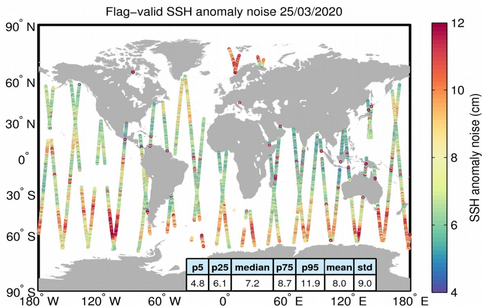
Figure 8. Geographical distribution of flag-valid 20-Hz SSH anomaly measurement noise over oceans and lakes for 25/03/2020. The statistical values shown in the table refer to the SSH anomaly noise and are calculated over all measurements shown in the figure.
