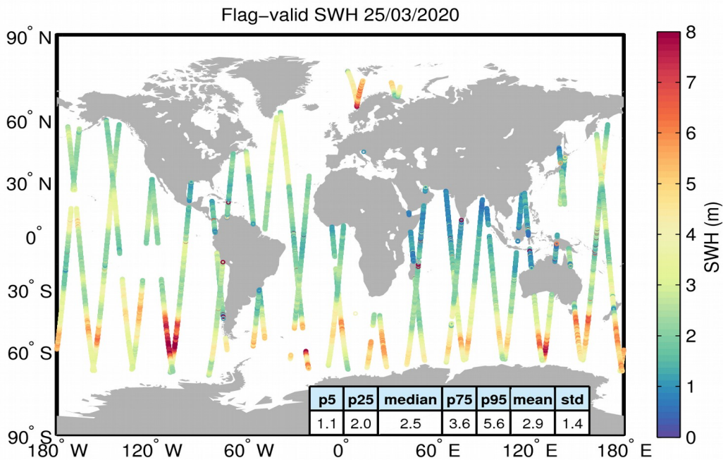
Figure 15. Geographical distribution of flag-valid SWH data over oceans and lakes for 25/03/2020. The statistical values shown in the table refer to the SWH in m and are calculated over all measurements shown in the figure.
