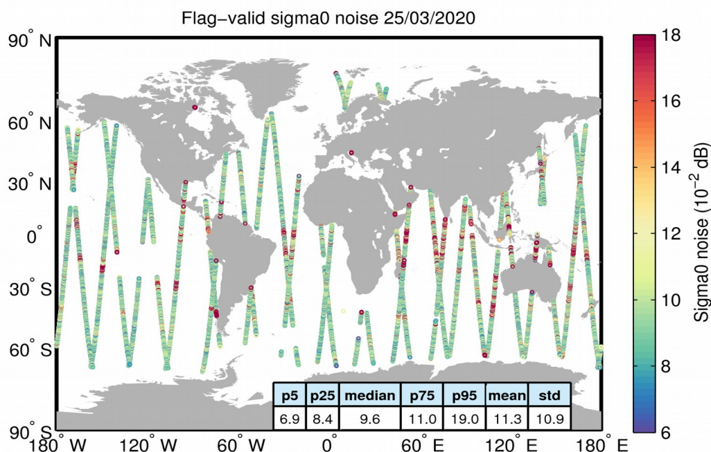
Figure 26. Geographical distribution of flag-valid 20-Hz sigma0 measurement noise over oceans and lakes for 25/03/2020. The statistical values shown in the table refer to the sigma0 noise and are calculated over all measurements shown in the figure.
