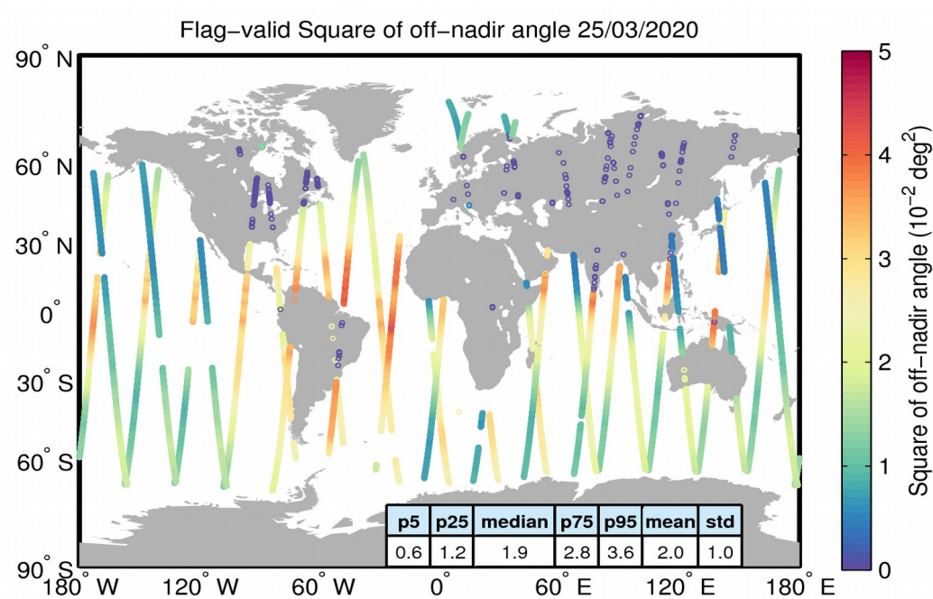
Figure 37. Geographical distribution of flag-valid mispointing data over oceans and lakes for 25/03/2020. The statistical values shown in the table refer to the mispointing in 10^{-2} \text{ deg}^2 and are calculated over all measurements shown in the figure.
