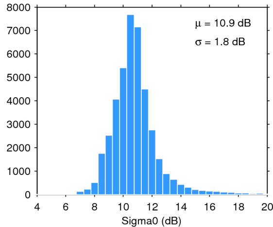
Figure 25. Histogram of flag-valid sigma0 over oceans and lakes for 25/03/2020. The mean ( \mu ) and standard deviation ( \sigma ) are also shown. Note that values outside [4 20] dB are excluded from the histogram for the sake of readability but not from the computation of \mu and \sigma .
