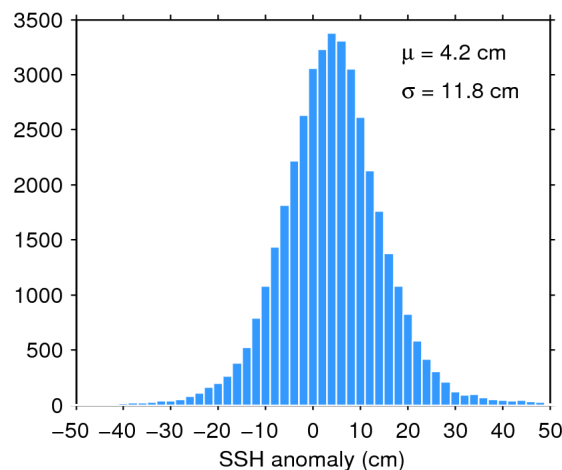
Figure 11. Histogram of science-valid SSH anomaly over oceans and lakes for 25/03/2020. The mean ( \mu ) and standard deviation ( \sigma ) are also shown. Note that values outside [-50 50] cm are excluded from the histogram for the sake of readability but not from the computation of \mu and \sigma .
