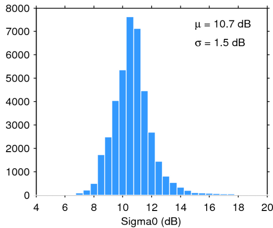
Figure 28. Histogram of science-valid sigma0 over oceans and lakes for 25/03/2020. The mean ( \mu ) and standard deviation ( \sigma ) are also shown. Note that values outside [4 20] dB are excluded from the histogram for the sake of readability but not from the computation of \mu and \sigma .
