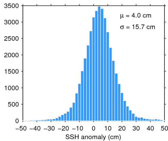
Figure 7. Histogram of flag-valid SSH anomaly over oceans and lakes for 25/03/2020. The mean ( \mu ) and standard deviation ( \sigma ) are also shown. Note that values outside [-50 50] cm are excluded from the histogram for the sake of readability but not from the computation of \mu and \sigma .
