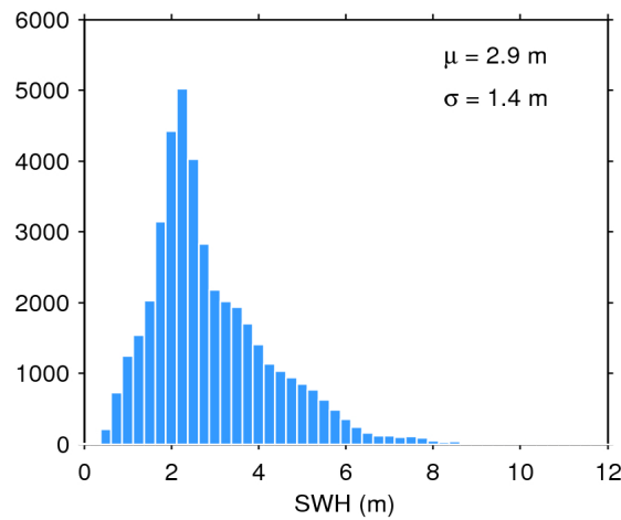
Figure 17. Histogram of flag-valid SWH over oceans and lakes for 25/03/2020. The mean ( \mu ) and standard deviation ( \sigma ) are also shown. Note that values larger than 12 m are excluded from the histogram for the sake of readability but not from the computation of \mu and \sigma .
