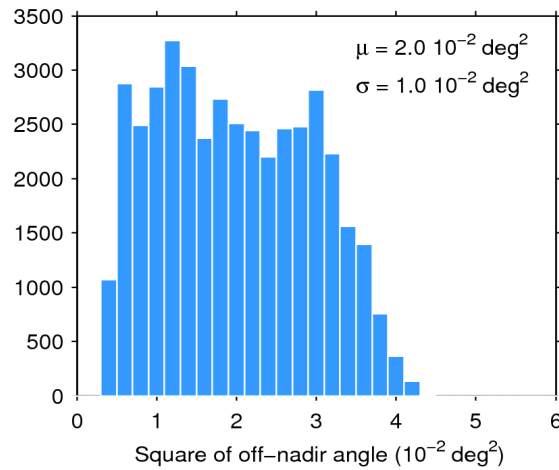
Figure 39. Histogram of flag-valid mispointing over oceans and lakes for 25/03/2020. The mean ( \mu ) and standard deviation ( \sigma ) are also shown. Note that values larger than 6 \cdot 10^{-2} \text{ deg}^2 are excluded from the histogram for the sake of readability but not from the computation of \mu and \sigma .
