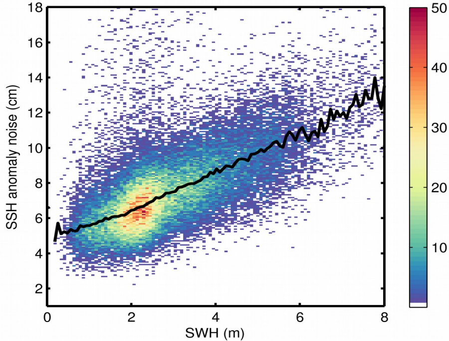
Figure 9. 2D histogram showing flag-valid SSH anomaly noise as a function of SWH for 25/03/2020. The black line denotes the median SSH anomaly noise as a function of SWH.
