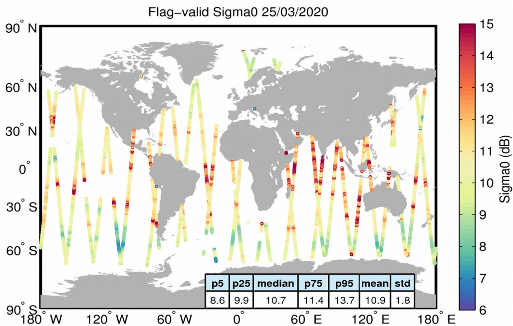
Figure 23. Geographical distribution of flag-valid sigma0 data over oceans and lakes for 25/03/2020. The statistical values shown in the table refer to the sigma0 in dB and are calculated over all measurements shown in the figure.
