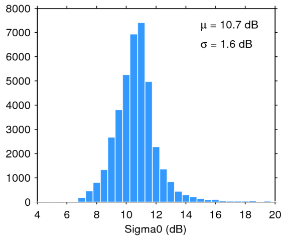
Figure 28. Histogram of science-valid sigma0 over oceans and lakes for 24/03/2020. The mean ( \mu ) and standard deviation ( \sigma ) are also shown. Note that values outside [4 20] dB are excluded from the histogram for the sake of readability but not from the computation of \mu and \sigma .
