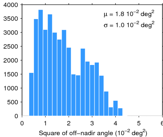
Figure 39. Histogram of flag-valid mispointing over oceans and lakes for 24/03/2020. The mean ( \mu ) and standard deviation ( \sigma ) are also shown. Note that values larger than 6 \cdot 10^{-2} \text{ deg}^2 are excluded from the histogram for the sake of readability but not from the computation of \mu and \sigma .
