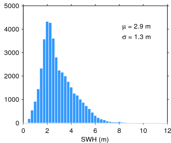
Figure 20. Histogram of science-valid SWH over oceans and lakes for 24/03/2020. The mean ( \mu ) and standard deviation ( \sigma ) are also shown. Note that values larger than 12 m are excluded from the histogram for the sake of readability but not from the computation of \mu and \sigma .
