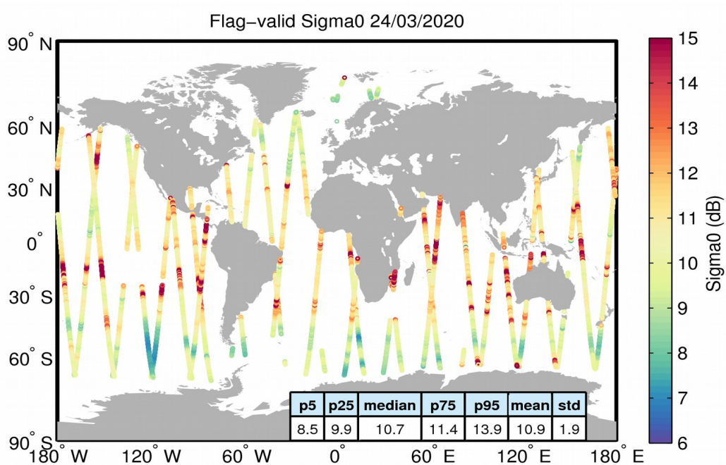
Figure 23. Geographical distribution of flag-valid sigma0 data over oceans and lakes for 24/03/2020. The statistical values shown in the table refer to the sigma0 in dB and are calculated over all measurements shown in the figure.
