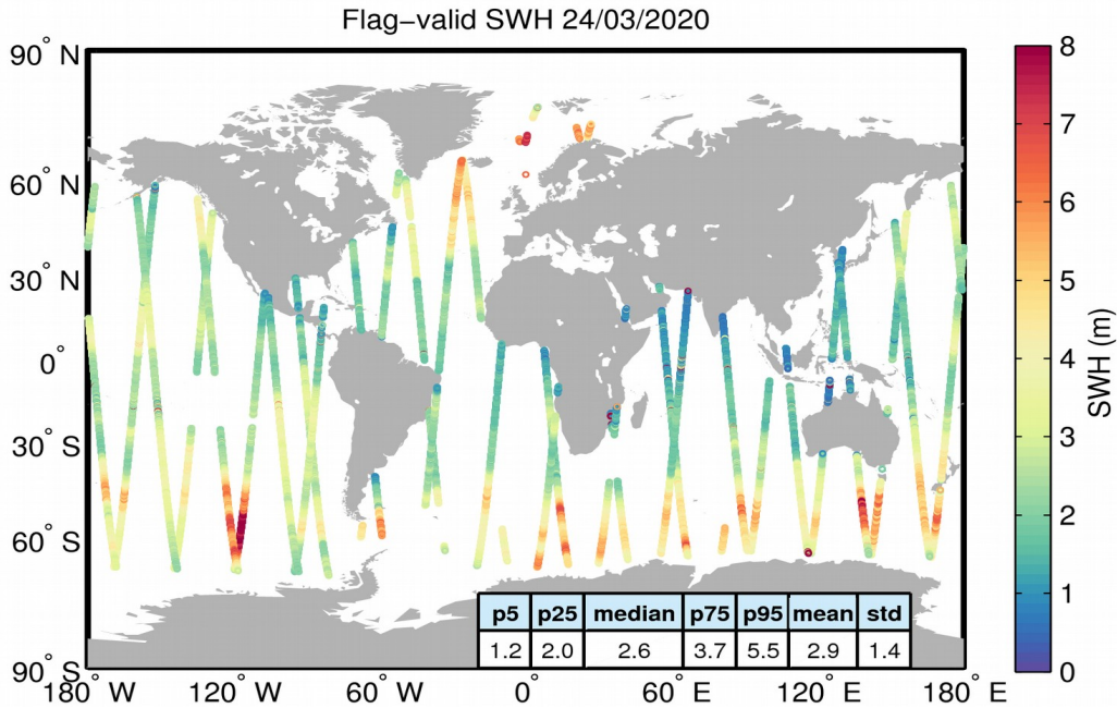
Figure 15. Geographical distribution of flag-valid SWH data over oceans and lakes for 24/03/2020. The statistical values shown in the table refer to the SWH in m and are calculated over all measurements shown in the figure.
