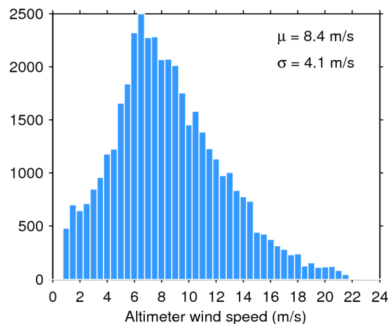
Figure 35. Histogram of science-valid wind over oceans and lakes for 24/03/2020. The mean ( \mu ) and standard deviation ( \sigma ) are also shown. Note that values larger than 24 m/s are excluded from the histogram for the sake of readability but not from the computation of \mu and \sigma .
