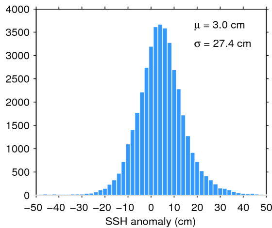
Figure 7. Histogram of flag-valid SSH anomaly over oceans and lakes for 24/03/2020. The mean ( \mu ) and standard deviation ( \sigma ) are also shown. Note that values outside [-50\ 50] cm are excluded from the histogram for the sake of readability but not from the computation of \mu and \sigma .
