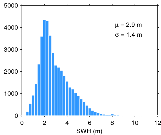
Figure 17. Histogram of flag-valid SWH over oceans and lakes for 24/03/2020. The mean ( \mu ) and standard deviation ( \sigma ) are also shown. Note that values larger than 12 m are excluded from the histogram for the sake of readability but not from the computation of \mu and \sigma .
