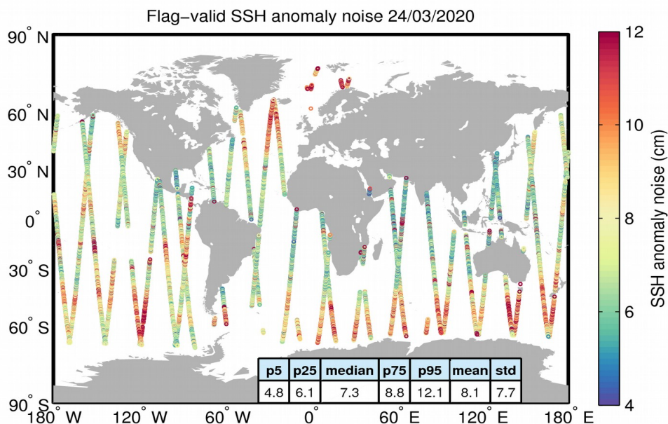
Figure 8. Geographical distribution of flag-valid 20-Hz SSH anomaly measurement noise over oceans and lakes for 24/03/2020. The statistical values shown in the table refer to the SSH anomaly noise and are calculated over all measurements shown in the figure.
