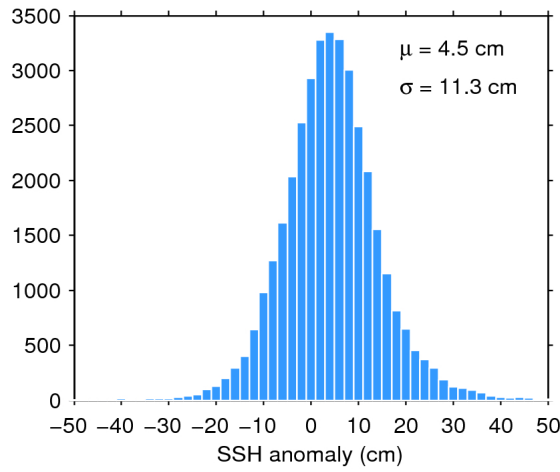
Figure 11. Histogram of science-valid SSH anomaly over oceans and lakes for 24/03/2020. The mean ( \mu ) and standard deviation ( \sigma ) are also shown. Note that values outside [-50 50] cm are excluded from the histogram for the sake of readability but not from the computation of \mu and \sigma .
