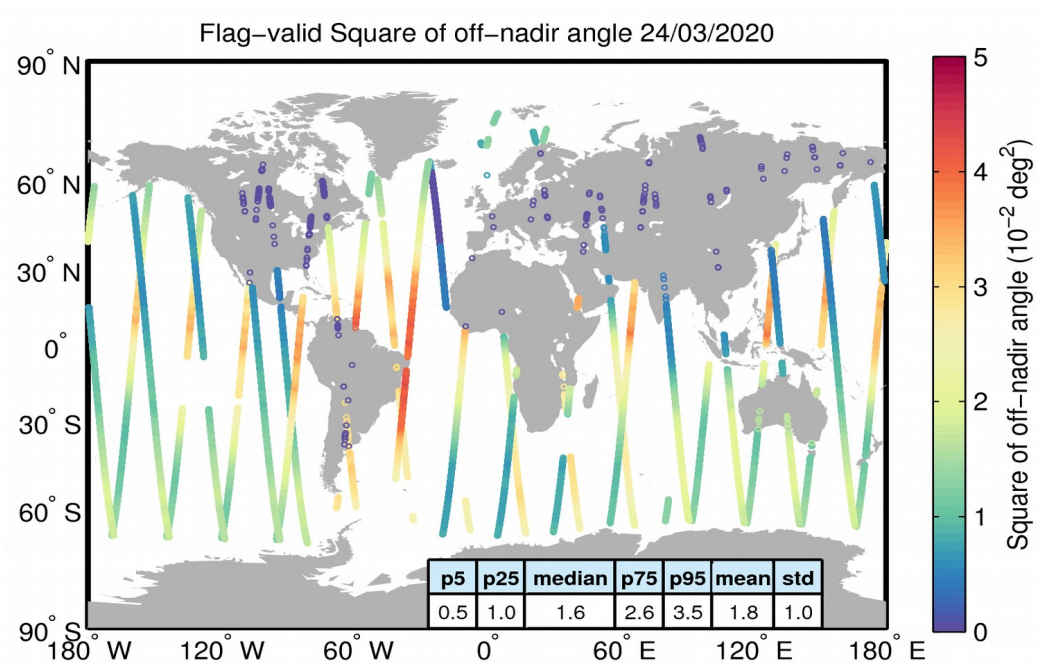
Figure 37. Geographical distribution of flag-valid mispointing data over oceans and lakes for 24/03/2020. The statistical values shown in the table refer to the mispointing in 10^{-2} \text{ deg}^2 and are calculated over all measurements shown in the figure.
