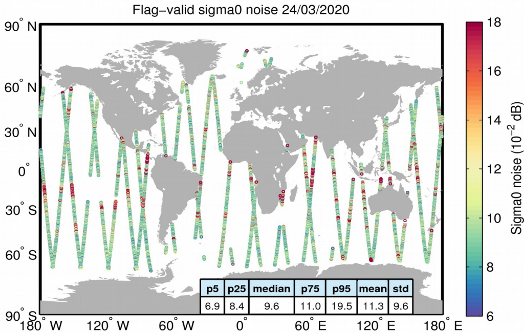
Figure 26. Geographical distribution of flag-valid 20-Hz sigma0 measurement noise over oceans and lakes for 24/03/2020. The statistical values shown in the table refer to the sigma0 noise and are calculated over all measurements shown in the figure.
