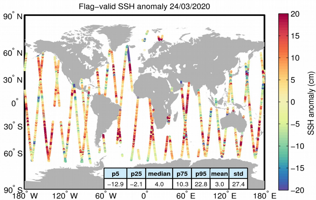
Figure 5. Geographical distribution of flag-valid 1-Hz SSH anomaly data over oceans and lakes for 24/03/2020. The statistical values shown in the table refer to the SSH anomaly in cm and are calculated over all measurements shown in the figure.
