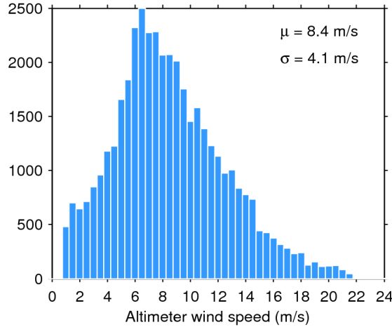
Figure 33. Histogram of flag-valid wind over oceans and lakes for 24/03/2020. The mean ( \mu ) and standard deviation ( \sigma ) are also shown. Note that values larger than 24 m/s are excluded from the histogram for the sake of readability but not from the computation of \mu and \sigma .
