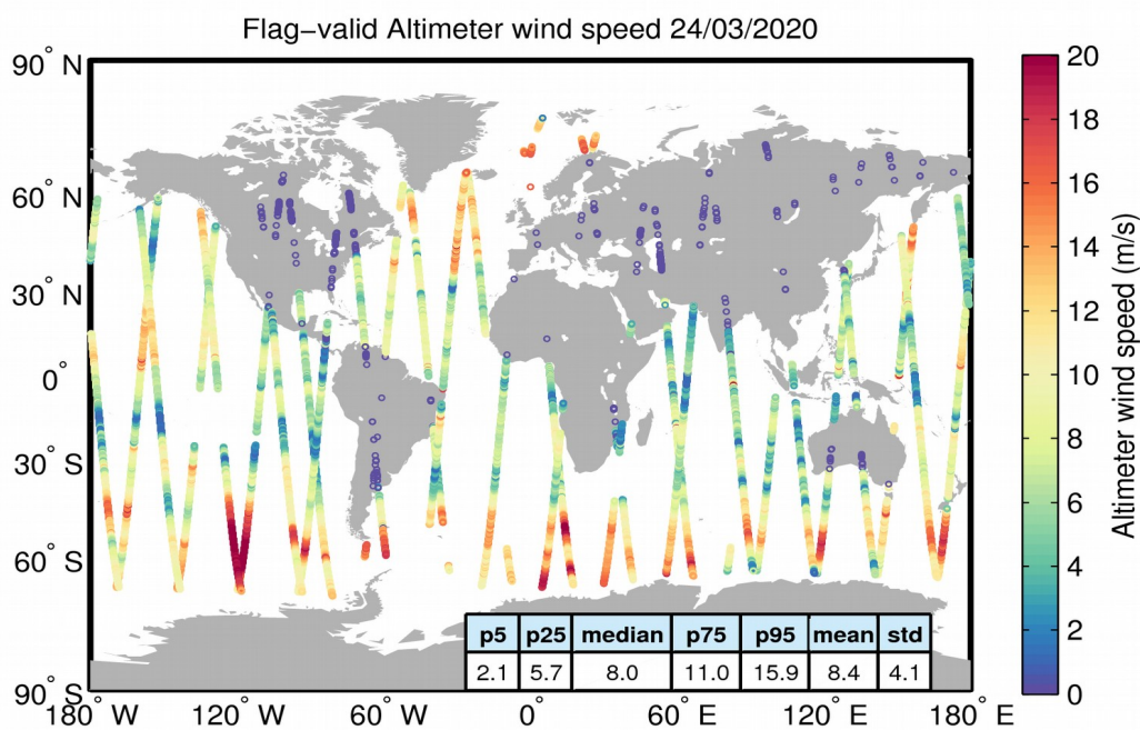
Figure 31. Geographical distribution of flag-valid wind data over oceans and lakes for 24/03/2020. The statistical values shown in the table refer to the wind in m/s and are calculated over all measurements shown in the figure.
