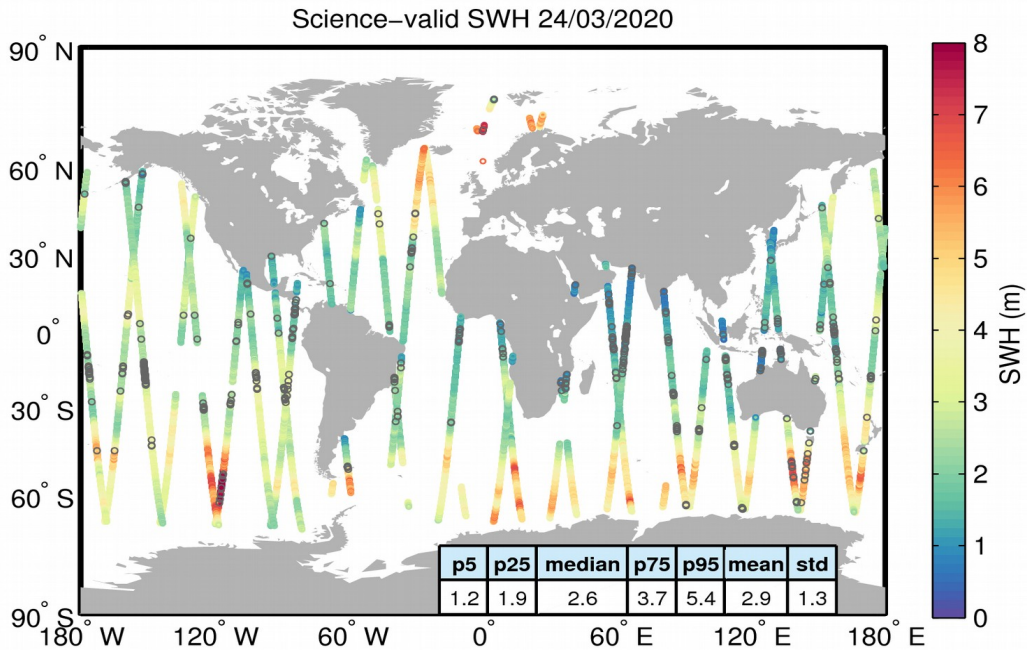
Figure 19. Geographical distribution of science-valid SWH data over oceans and lakes for 24/03/2020. The statistical values shown in the table refer to the SWH in m and are calculated over all measurements shown in the figure. Gray circles denote records that have been rejected based on the editing criteria described in Table 3.
