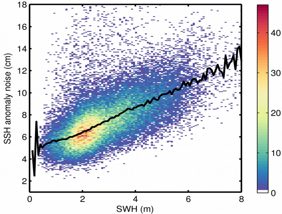
Figure 9. 2D histogram showing flag-valid SSH anomaly noise as a function of SWH for 24/03/2020. The black line denotes the median SSH anomaly noise as a function of SWH.
