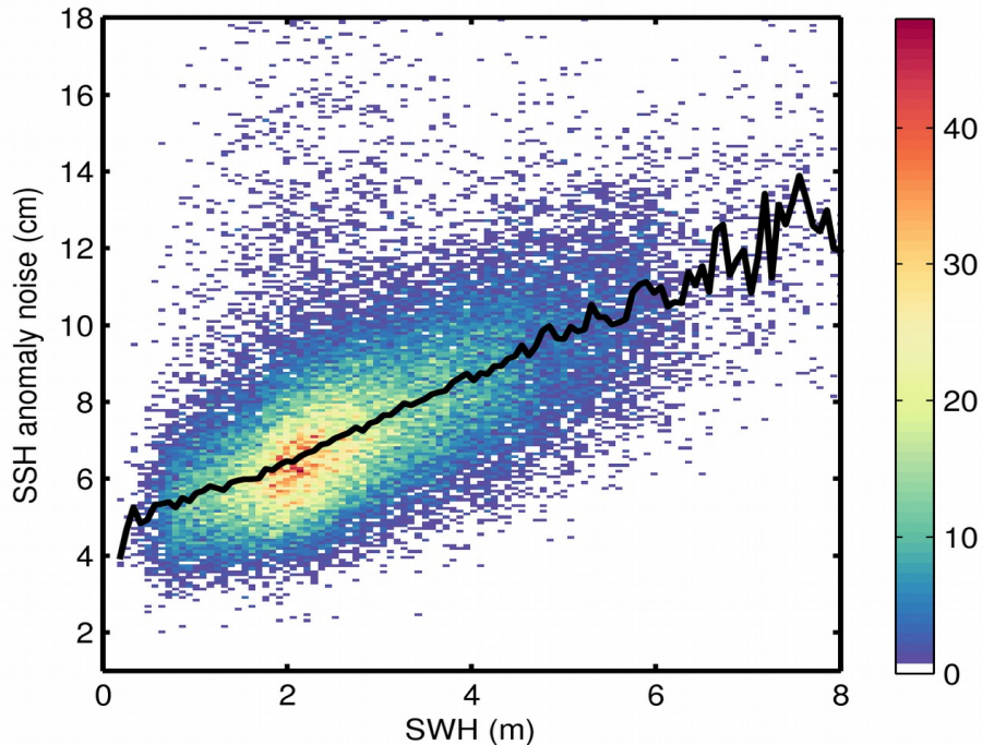
Figure 9. 2D histogram showing flag-valid SSH anomaly noise as a function of SWH for 23/03/2020. The black line denotes the median SSH anomaly noise as a function of SWH.
