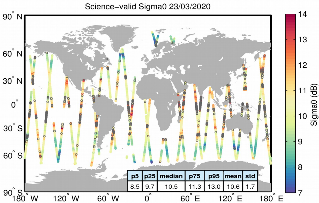
Figure 27. Geographical distribution of science-valid sigma0 data over oceans and lakes for 23/03/2020. The statistical values shown in the table refer to the sigma0 in dB and are calculated over all measurements shown in the figure. Gray circles denote records that have been rejected based on the editing criteria described in Table 4.
