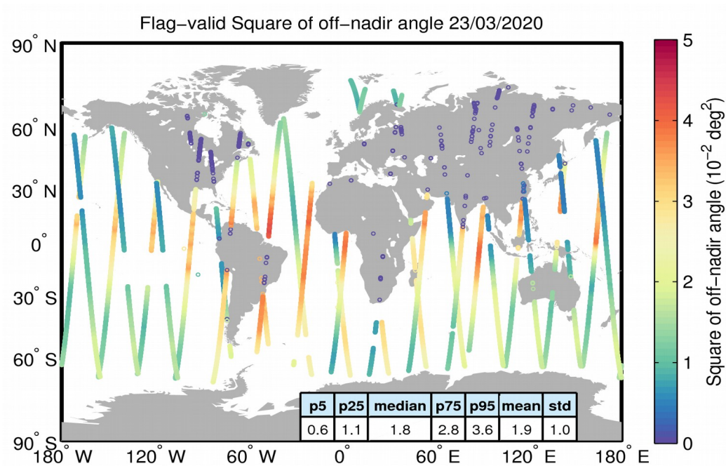
Figure 37. Geographical distribution of flag-valid mispointing data over oceans and lakes for 23/03/2020. The statistical values shown in the table refer to the mispointing in 10^{-2} deg 2 and are calculated over all measurements shown in the figure.
