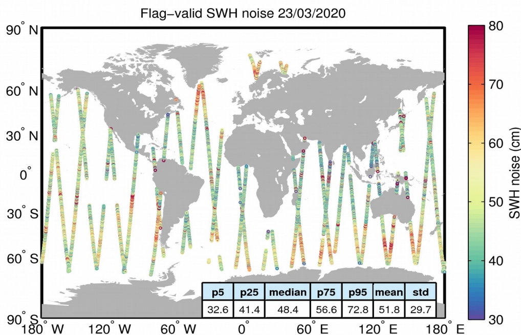
Figure 18. Geographical distribution of flag-valid 20-Hz SWH measurement noise over oceans and lakes for 23/03/2020. The statistical values shown in the figure refer to the SWH noise and are calculated over all measurements shown in the figure.
