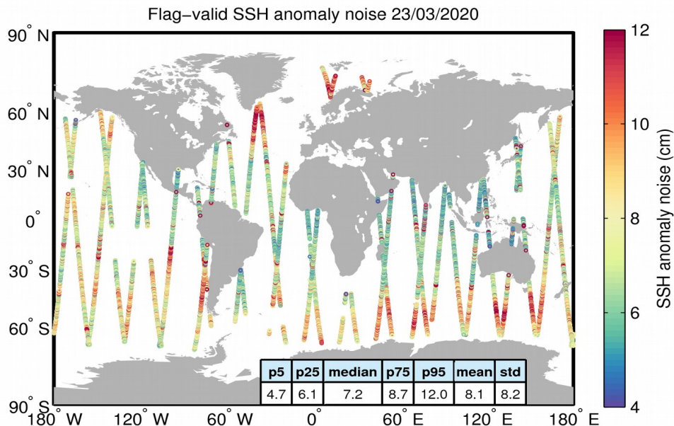
Figure 8. Geographical distribution of flag-valid 20-Hz SSH anomaly measurement noise over oceans and lakes for 23/03/2020. The statistical values shown in the table refer to the SSH anomaly noise and are calculated over all measurements shown in the figure.
