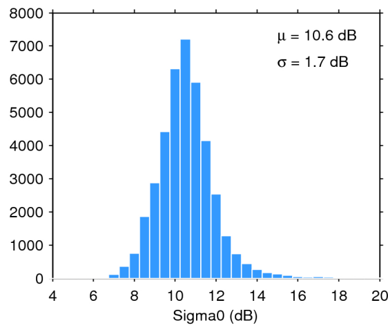
Figure 28. Histogram of science-valid sigma0 over oceans and lakes for 23/03/2020. The mean ( \mu ) and standard deviation ( \sigma ) are also shown. Note that values outside [4 20] dB are excluded from the histogram for the sake of readability but not from the computation of \mu and \sigma .
