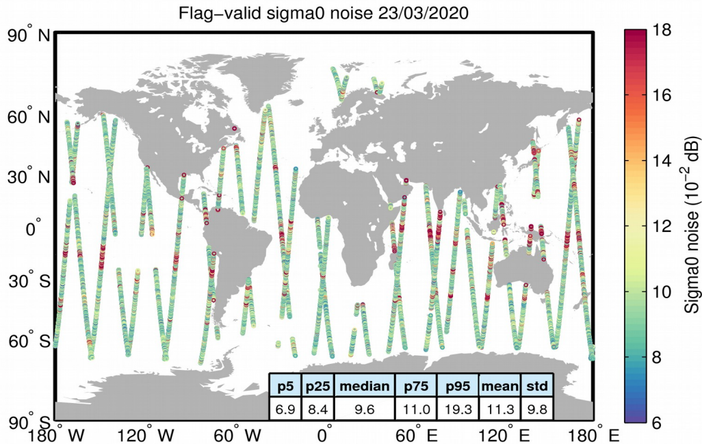
Figure 26. Geographical distribution of flag-valid 20-Hz sigma0 measurement noise over oceans and lakes for 23/03/2020. The statistical values shown in the table refer to the sigma0 noise and are calculated over all measurements shown in the figure.
