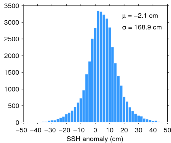
Figure 7. Histogram of flag-valid SSH anomaly over oceans and lakes for 23/03/2020. The mean ( \mu ) and standard deviation ( \sigma ) are also shown. Note that values outside [-50 50] cm are excluded from the histogram for the sake of readability but not from the computation of \mu and \sigma .
