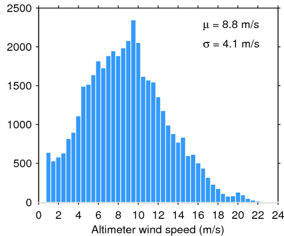
Figure 33. Histogram of flag-valid wind over oceans and lakes for 23/03/2020. The mean ( \mu ) and standard deviation ( \sigma ) are also shown. Note that values larger than 24 m/s are excluded from the histogram for the sake of readability but not from the computation of \mu and \sigma .
