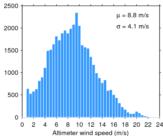
Figure 35. Histogram of science-valid wind over oceans and lakes for 23/03/2020. The mean ( \mu ) and standard deviation ( \sigma ) are also shown. Note that values larger than 24 m/s are excluded from the histogram for the sake of readability but not from the computation of \mu and \sigma .
