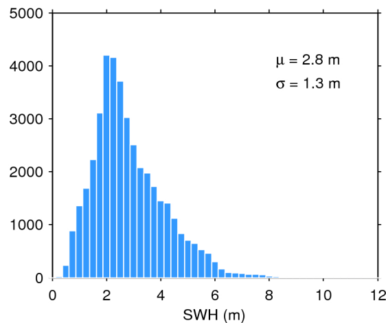
Figure 20. Histogram of science-valid SWH over oceans and lakes for 23/03/2020. The mean ( \mu ) and standard deviation ( \sigma ) are also shown. Note that values larger than 12 m are excluded from the histogram for the sake of readability but not from the computation of \mu and \sigma .
