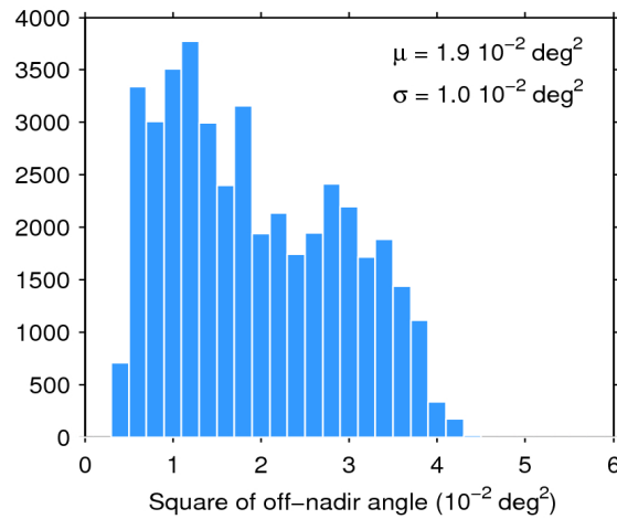
Figure 39. Histogram of flag-valid mispointing over oceans and lakes for 23/03/2020. The mean ( \mu ) and standard deviation ( \sigma ) are also shown. Note that values larger than 6 \cdot 10^{-2} \text{ deg}^2 are excluded from the histogram for the sake of readability but not from the computation of \mu and \sigma .
