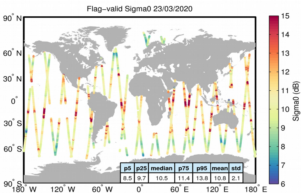
Figure 23. Geographical distribution of flag-valid sigma0 data over oceans and lakes for 23/03/2020. The statistical values shown in the table refer to the sigma0 in dB and are calculated over all measurements shown in the figure.
