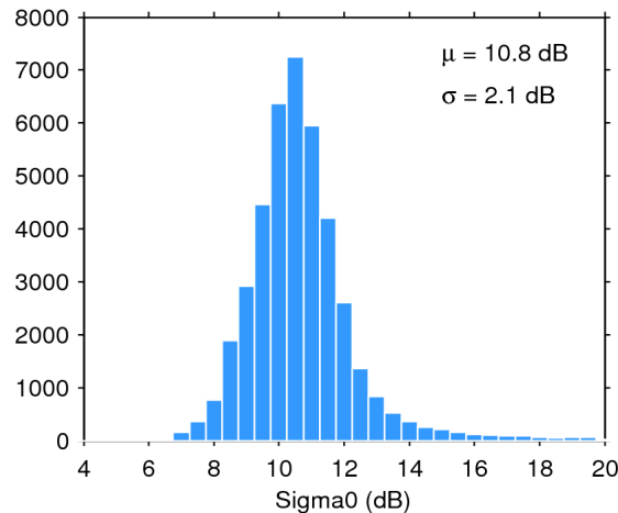
Figure 25. Histogram of flag-valid sigma0 over oceans and lakes for 23/03/2020. The mean ( \mu ) and standard deviation ( \sigma ) are also shown. Note that values outside [4 20] dB are excluded from the histogram for the sake of readability but not from the computation of \mu and \sigma .
