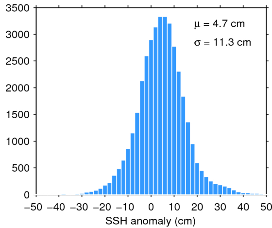
Figure 11. Histogram of science-valid SSH anomaly over oceans and lakes for 22/03/2020. The mean ( \mu ) and standard deviation ( \sigma ) are also shown. Note that values outside [-50 50] cm are excluded from the histogram for the sake of readability but not from the computation of \mu and \sigma .
