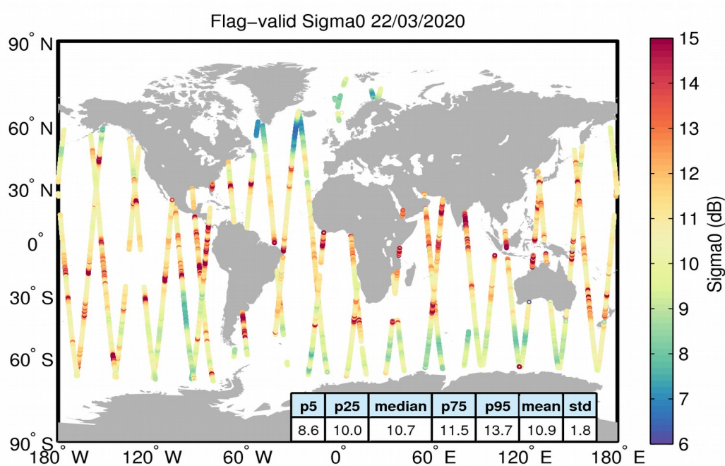
Figure 23. Geographical distribution of flag-valid sigma0 data over oceans and lakes for 22/03/2020. The statistical values shown in the table refer to the sigma0 in dB and are calculated over all measurements shown in the figure.
