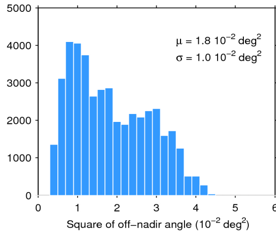
Figure 39. Histogram of flag-valid mispointing over oceans and lakes for 22/03/2020. The mean ( \mu ) and standard deviation ( \sigma ) are also shown. Note that values larger than 6 \cdot 10^{-2} \text{ deg}^2 are excluded from the histogram for the sake of readability but not from the computation of \mu and \sigma .
