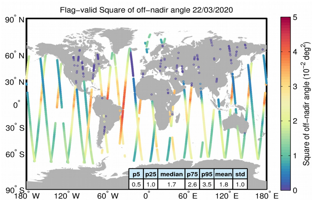
Figure 37. Geographical distribution of flag-valid mispointing data over oceans and lakes for 22/03/2020. The statistical values shown in the table refer to the mispointing in 10^{-2} \text{ deg}^2 and are calculated over all measurements shown in the figure.
