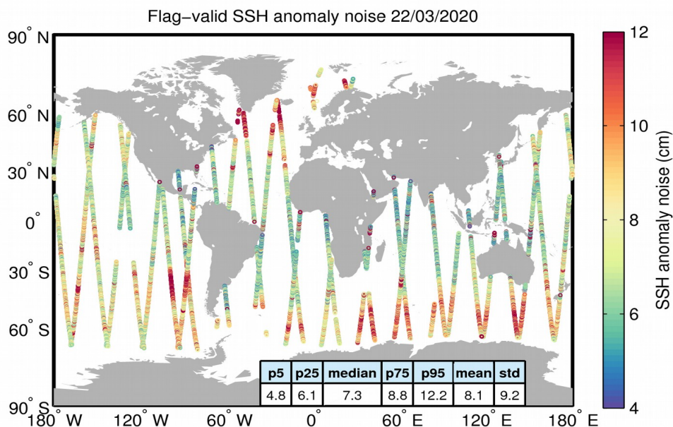
Figure 8. Geographical distribution of flag-valid 20-Hz SSH anomaly measurement noise over oceans and lakes for 22/03/2020. The statistical values shown in the table refer to the SSH anomaly noise and are calculated over all measurements shown in the figure.
