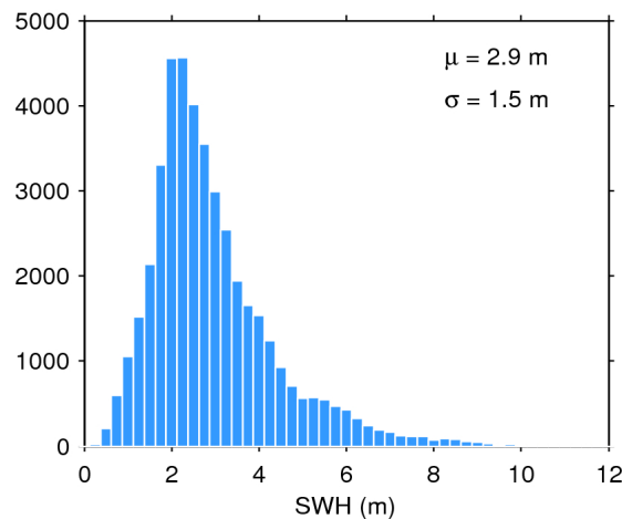
Figure 17. Histogram of flag-valid SWH over oceans and lakes for 22/03/2020. The mean ( \mu ) and standard deviation ( \sigma ) are also shown. Note that values larger than 12 m are excluded from the histogram for the sake of readability but not from the computation of \mu and \sigma .
