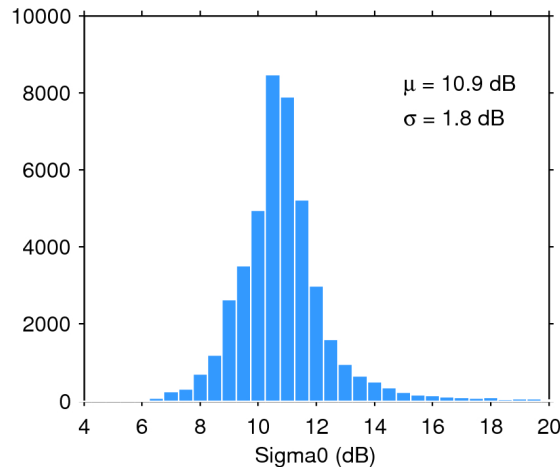
Figure 25. Histogram of flag-valid sigma0 over oceans and lakes for 22/03/2020. The mean ( \mu ) and standard deviation ( \sigma ) are also shown. Note that values outside [4 20] dB are excluded from the histogram for the sake of readability but not from the computation of \mu and \sigma .
