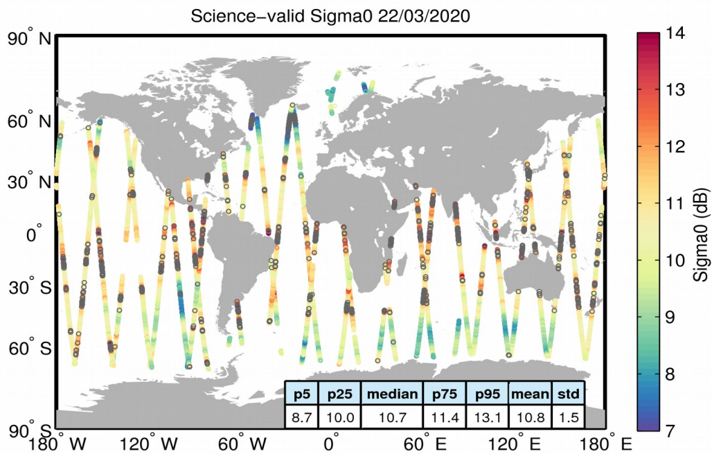
Figure 27. Geographical distribution of science-valid sigma0 data over oceans and lakes for 22/03/2020. The statistical values shown in the table refer to the sigma0 in dB and are calculated over all measurements shown in the figure. Gray circles denote records that have been rejected based on the editing criteria described in Table 4.
