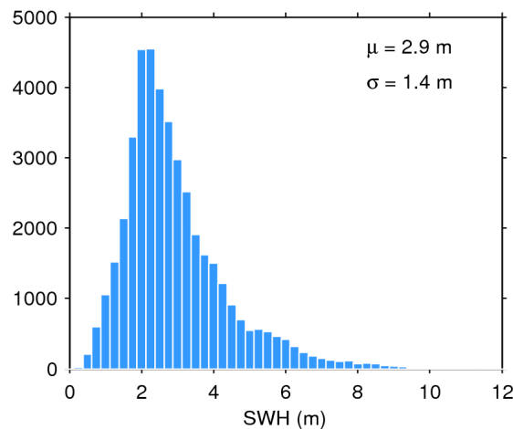
Figure 20. Histogram of science-valid SWH over oceans and lakes for 22/03/2020. The mean ( \mu ) and standard deviation ( \sigma ) are also shown. Note that values larger than 12 m are excluded from the histogram for the sake of readability but not from the computation of \mu and \sigma .
