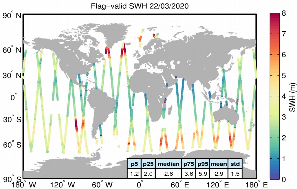
Figure 15. Geographical distribution of flag-valid SWH data over oceans and lakes for 22/03/2020. The statistical values shown in the table refer to the SWH in m and are calculated over all measurements shown in the figure.
