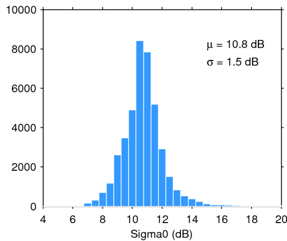
Figure 28. Histogram of science-valid sigma0 over oceans and lakes for 22/03/2020. The mean ( \mu ) and standard deviation ( \sigma ) are also shown. Note that values outside [4 20] dB are excluded from the histogram for the sake of readability but not from the computation of \mu and \sigma .
