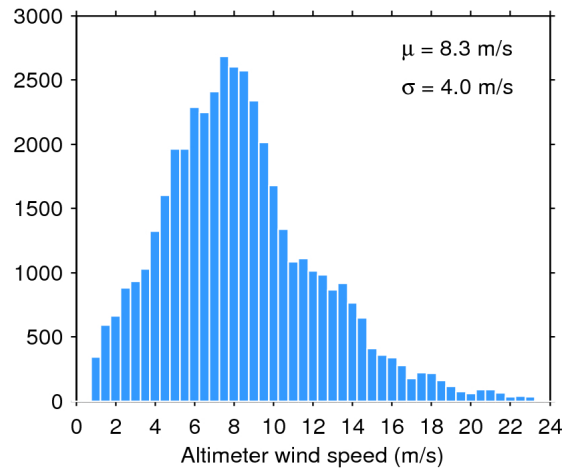
Figure 33. Histogram of flag-valid wind over oceans and lakes for 22/03/2020. The mean ( \mu ) and standard deviation ( \sigma ) are also shown. Note that values larger than 24 m/s are excluded from the histogram for the sake of readability but not from the computation of \mu and \sigma .
