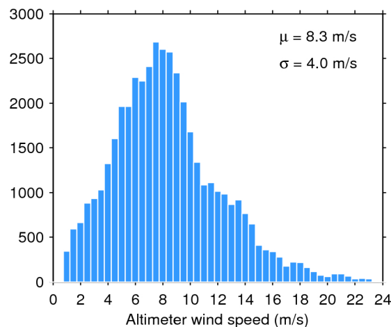
Figure 35. Histogram of science-valid wind over oceans and lakes for 22/03/2020. The mean ( \mu ) and standard deviation ( \sigma ) are also shown. Note that values larger than 24 m/s are excluded from the histogram for the sake of readability but not from the computation of \mu and \sigma .
