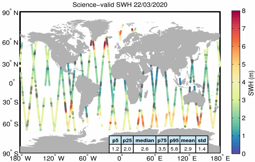
Figure 19. Geographical distribution of science-valid SWH data over oceans and lakes for 22/03/2020. The statistical values shown in the table refer to the SWH in m and are calculated over all measurements shown in the figure. Gray circles denote records that have been rejected based on the editing criteria described in Table 3.
