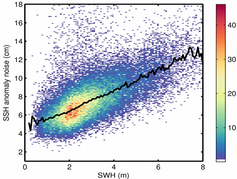
Figure 9. 2D histogram showing flag-valid SSH anomaly noise as a function of SWH for 22/03/2020. The black line denotes the median SSH anomaly noise as a function of SWH.
