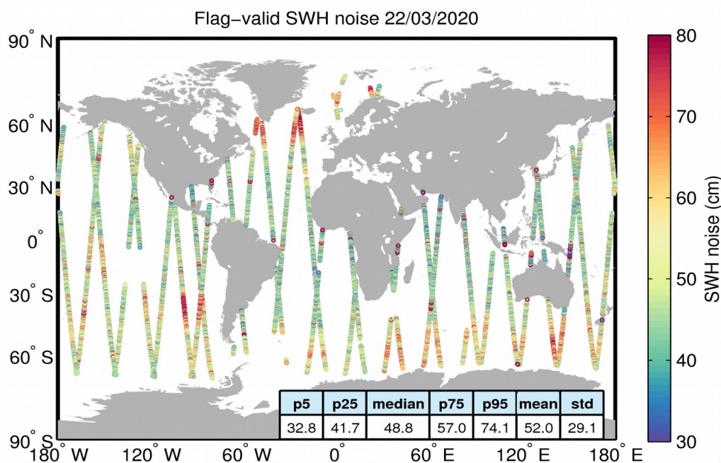
Figure 18. Geographical distribution of flag-valid 20-Hz SWH measurement noise over oceans and lakes for 22/03/2020. The statistical values shown in the figure refer to the SWH noise and are calculated over all measurements shown in the figure.
