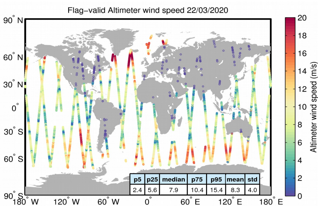
Figure 31. Geographical distribution of flag-valid wind data over oceans and lakes for 22/03/2020. The statistical values shown in the table refer to the wind in m/s and are calculated over all measurements shown in the figure.
