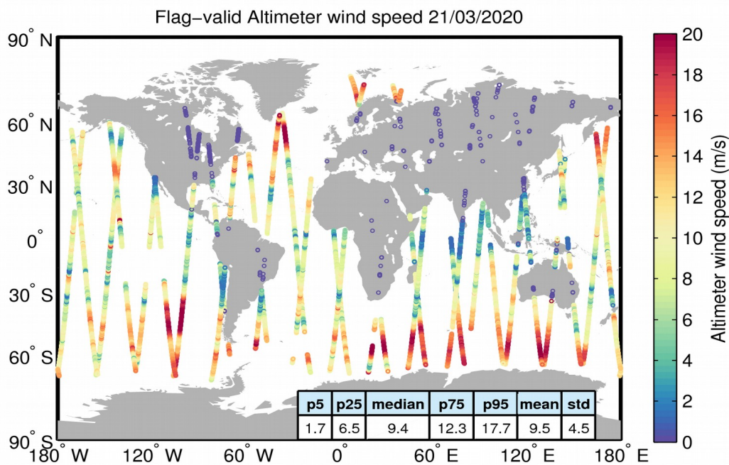
Figure 31. Geographical distribution of flag-valid wind data over oceans and lakes for 21/03/2020. The statistical values shown in the figure refer to the wind in m/s and are calculated over all measurements shown in the figure.
