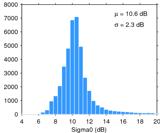
Figure 25. Histogram of flag-valid sigma0 over oceans and lakes for 21/03/2020. The mean ( \mu ) and standard deviation ( \sigma ) are also shown. Note that values outside [4 20] dB are excluded from the histogram for the sake of readability but not from the computation of \mu and \sigma .
