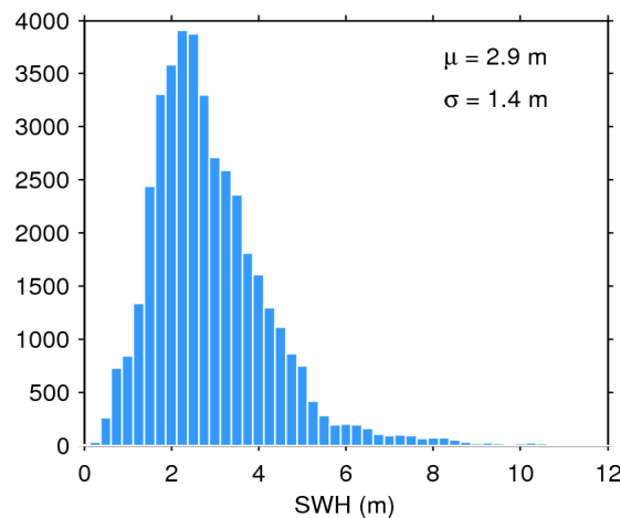
Figure 17. Histogram of flag-valid SWH over oceans and lakes for 21/03/2020. The mean ( \mu ) and standard deviation ( \sigma ) are also shown. Note that values larger than 12 m are excluded from the histogram for the sake of readability but not from the computation of \mu and \sigma .
