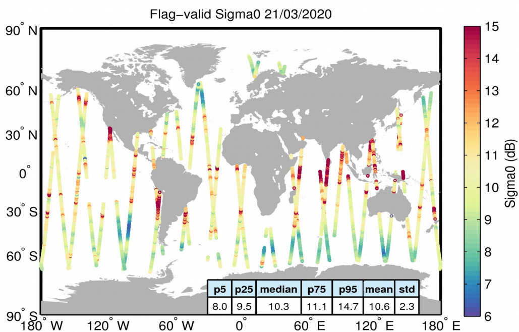
Figure 23. Geographical distribution of flag-valid sigma0 data over oceans and lakes for 21/03/2020. The statistical values shown in the table refer to the sigma0 in dB and are calculated over all measurements shown in the figure.
