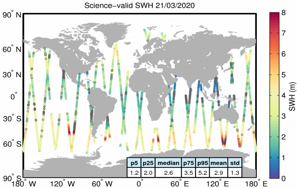
Figure 19. Geographical distribution of science-valid SWH data over oceans and lakes for 21/03/2020. The statistical values shown in the table refer to the SWH in m and are calculated over all measurements shown in the figure. Gray circles denote records that have been rejected based on the editing criteria described in Table 3.
