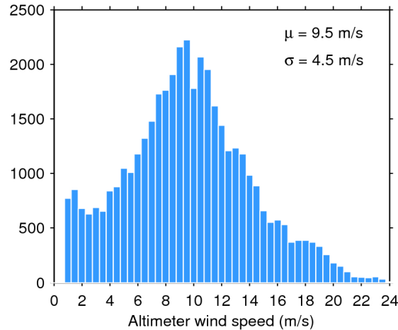
Figure 33. Histogram of flag-valid wind over oceans and lakes for 21/03/2020. The mean ( \mu ) and standard deviation ( \sigma ) are also shown. Note that values larger than 24 m/s are excluded from the histogram for the sake of readability but not from the computation of \mu and \sigma .
