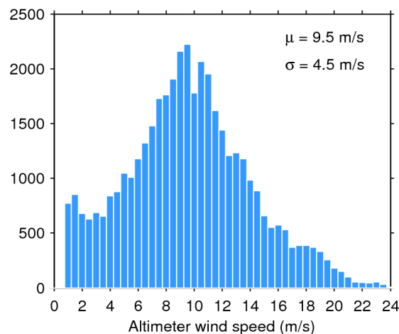
Figure 35. Histogram of science-valid wind over oceans and lakes for 21/03/2020. The mean ( \mu ) and standard deviation ( \sigma ) are also shown. Note that values larger than 24 m/s are excluded from the histogram for the sake of readability but not from the computation of \mu and \sigma .
