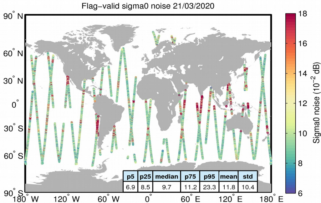
Figure 26. Geographical distribution of flag-valid 20-Hz sigma0 measurement noise over oceans and lakes for 21/03/2020. The statistical values shown in the table refer to the sigma0 noise and are calculated over all measurements shown in the figure.
