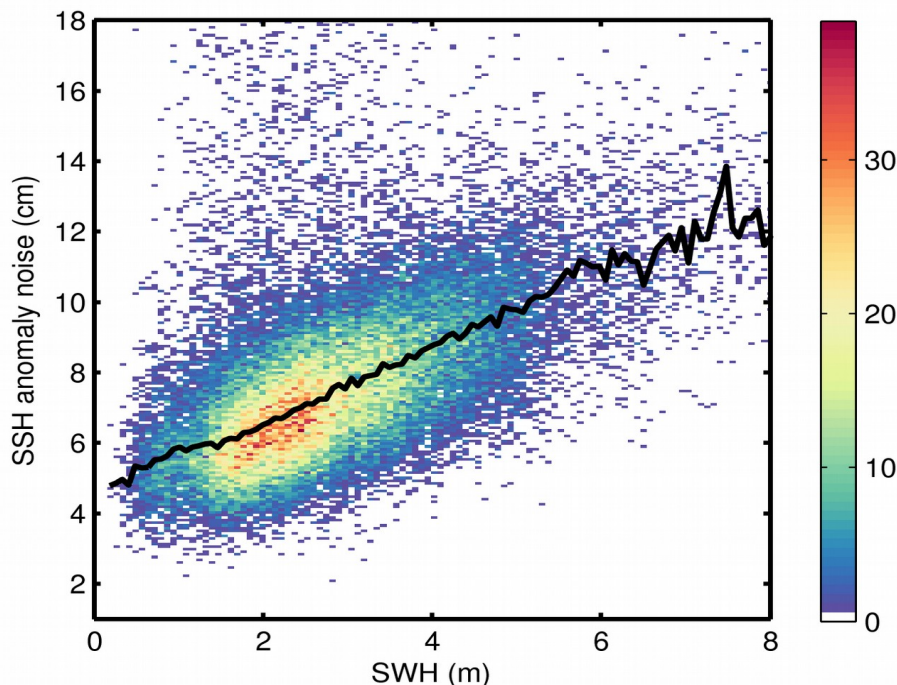
Figure 9. 2D histogram showing flag-valid SSH anomaly noise as a function of SWH for 21/03/2020. The black line denotes the median SSH anomaly noise as a function of SWH.
