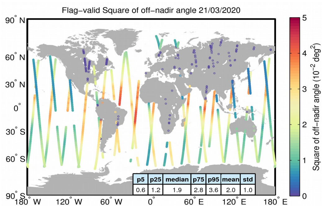
Figure 37. Geographical distribution of flag-valid mispointing data over oceans and lakes for 21/03/2020. The statistical values shown in the table refer to the mispointing in 10^{-2} \text{ deg}^2 and are calculated over all measurements shown in the figure.
