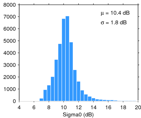
Figure 28. Histogram of science-valid sigma0 over oceans and lakes for 21/03/2020. The mean ( \mu ) and standard deviation ( \sigma ) are also shown. Note that values outside [4 20] dB are excluded from the histogram for the sake of readability but not from the computation of \mu and \sigma .
