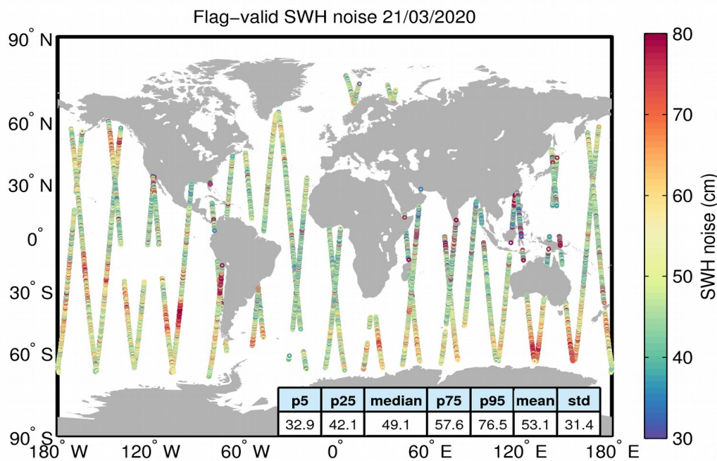
Figure 18. Geographical distribution of flag-valid 20-Hz SWH measurement noise over oceans and lakes for 21/03/2020. The statistical values shown in the figure refer to the SWH noise and are calculated over all measurements shown in the figure.
