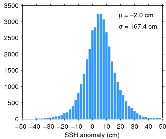
Figure 7. Histogram of flag-valid SSH anomaly over oceans and lakes for 21/03/2020. The mean ( \mu ) and standard deviation ( \sigma ) are also shown. Note that values outside [-50\ 50] cm are excluded from the histogram for the sake of readability but not from the computation of \mu and \sigma .
