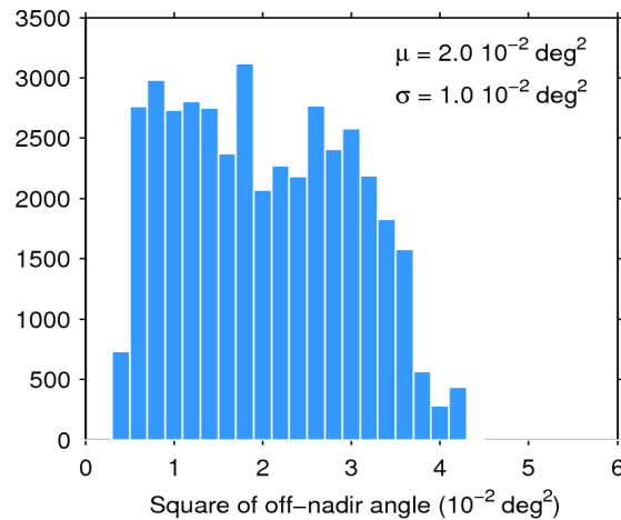
Figure 39. Histogram of flag-valid mispointing over oceans and lakes for 21/03/2020. The mean ( \mu ) and standard deviation ( \sigma ) are also shown. Note that values larger than 6 \cdot 10^{-2} \text{ deg}^2 are excluded from the histogram for the sake of readability but not from the computation of \mu and \sigma .
