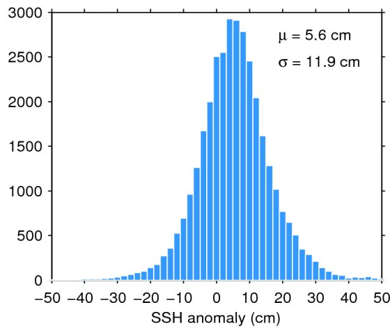
Figure 11. Histogram of science-valid SSH anomaly over oceans and lakes for 21/03/2020. The mean ( \mu ) and standard deviation ( \sigma ) are also shown. Note that values outside [-50 50] cm are excluded from the histogram for the sake of readability but not from the computation of \mu and \sigma .
