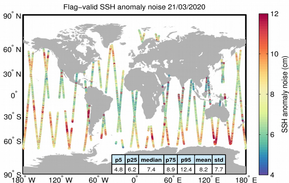
Figure 8. Geographical distribution of flag-valid 20-Hz SSH anomaly measurement noise over oceans and lakes for 21/03/2020. The statistical values shown in the table refer to the SSH anomaly noise and are calculated over all measurements shown in the figure.
