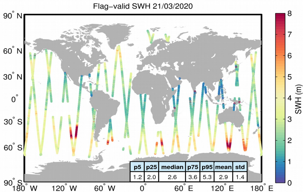
Figure 15. Geographical distribution of flag-valid SWH data over oceans and lakes for 21/03/2020. The statistical values shown in the table refer to the SWH in m and are calculated over all measurements shown in the figure.
