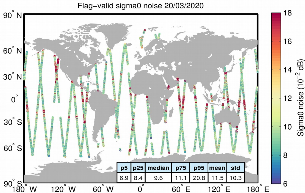
Figure 26. Geographical distribution of flag-valid 20-Hz sigma0 measurement noise over oceans and lakes for 20/03/2020. The statistical values shown in the table refer to the sigma0 noise and are calculated over all measurements shown in the figure.
