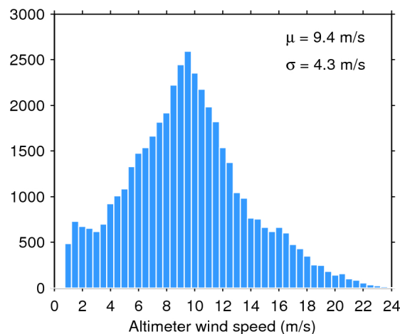
Figure 35. Histogram of science-valid wind over oceans and lakes for 20/03/2020. The mean ( \mu ) and standard deviation ( \sigma ) are also shown. Note that values larger than 24 m/s are excluded from the histogram for the sake of readability but not from the computation of \mu and \sigma .
