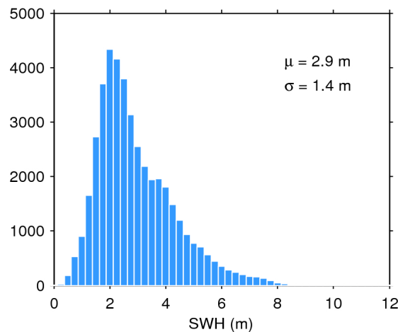
Figure 17. Histogram of flag-valid SWH over oceans and lakes for 20/03/2020. The mean ( \mu ) and standard deviation ( \sigma ) are also shown. Note that values larger than 12 m are excluded from the histogram for the sake of readability but not from the computation of \mu and \sigma .
