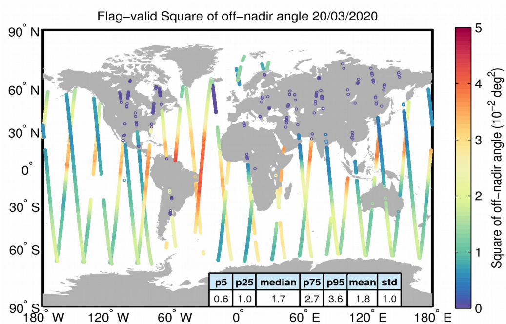
Figure 37. Geographical distribution of flag-valid mispointing data over oceans and lakes for 20/03/2020. The statistical values shown in the table refer to the mispointing in 10^{-2} deg 2 and are calculated over all measurements shown in the figure.
