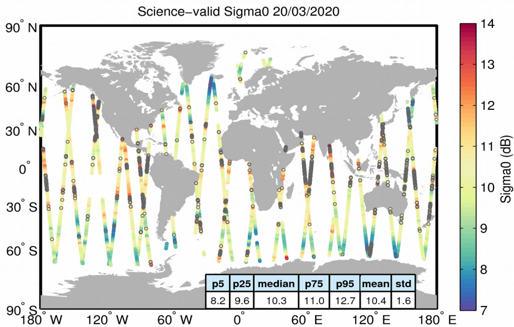
Figure 27. Geographical distribution of science-valid sigma0 data over oceans and lakes for 20/03/2020. The statistical values shown in the table refer to the sigma0 in dB and are calculated over all measurements shown in the figure. Gray circles denote records that have been rejected based on the editing criteria described in Table 4.
