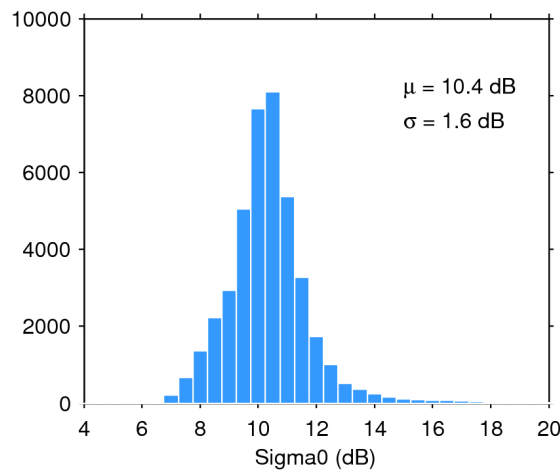
Figure 28. Histogram of science-valid sigma0 over oceans and lakes for 20/03/2020. The mean ( \mu ) and standard deviation ( \sigma ) are also shown. Note that values outside [4 20] dB are excluded from the histogram for the sake of readability but not from the computation of \mu and \sigma .
