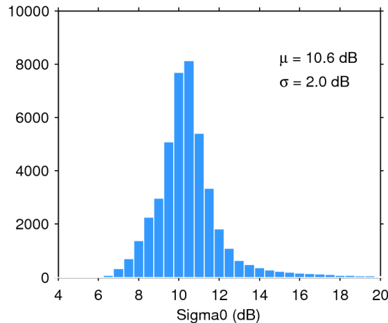
Figure 25. Histogram of flag-valid sigma0 over oceans and lakes for 20/03/2020. The mean ( \mu ) and standard deviation ( \sigma ) are also shown. Note that values outside [4 20] dB are excluded from the histogram for the sake of readability but not from the computation of \mu and \sigma .
