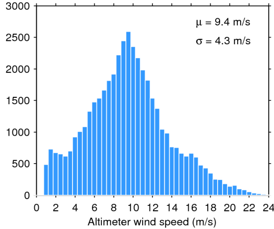
Figure 33. Histogram of flag-valid wind over oceans and lakes for 20/03/2020. The mean ( \mu ) and standard deviation ( \sigma ) are also shown. Note that values larger than 24 m/s are excluded from the histogram for the sake of readability but not from the computation of \mu and \sigma .
