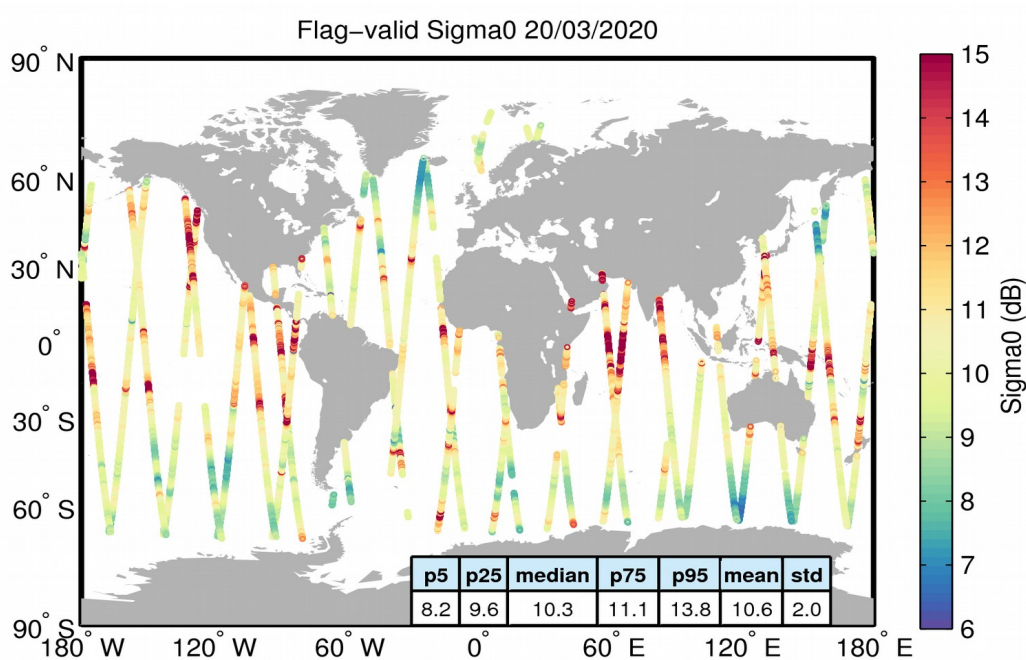
Figure 23. Geographical distribution of flag-valid sigma0 data over oceans and lakes for 20/03/2020. The statistical values shown in the table refer to the sigma0 in dB and are calculated over all measurements shown in the figure.
