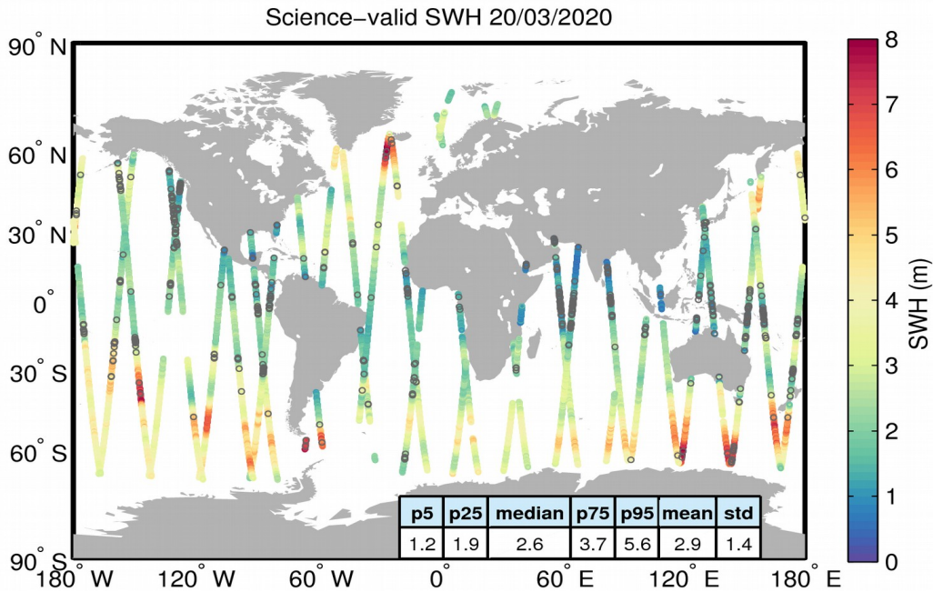
Figure 19. Geographical distribution of science-valid SWH data over oceans and lakes for 20/03/2020. The statistical values shown in the table refer to the SWH in m and are calculated over all measurements shown in the figure. Gray circles denote records that have been rejected based on the editing criteria described in Table 3.
