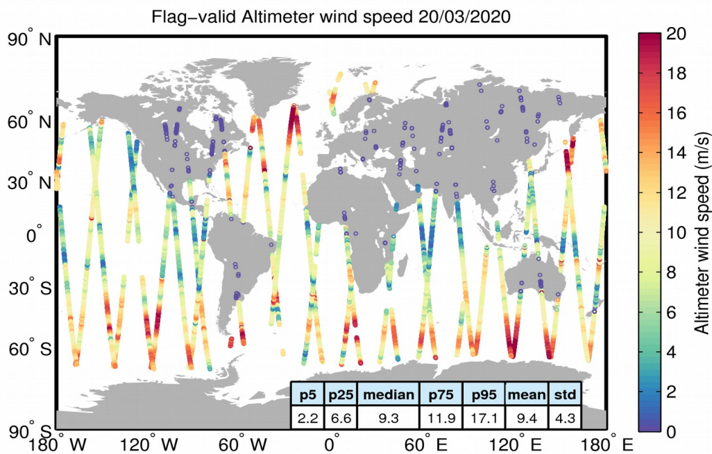
Figure 31. Geographical distribution of flag-valid wind data over oceans and lakes for 20/03/2020. The statistical values shown in the table refer to the wind in m/s and are calculated over all measurements shown in the figure.
