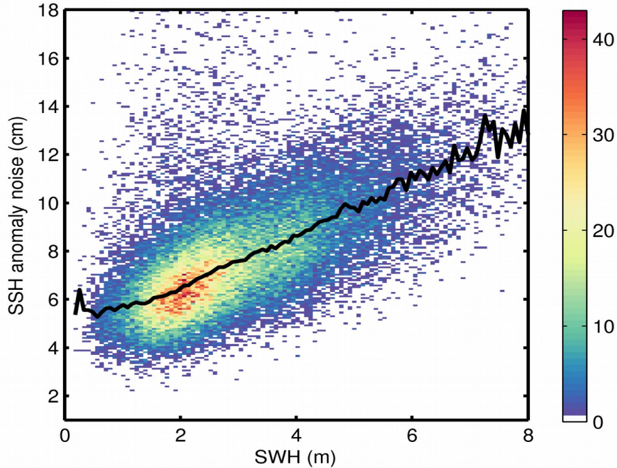
Figure 9. 2D histogram showing flag-valid SSH anomaly noise as a function of SWH for 20/03/2020. The black line denotes the median SSH anomaly noise as a function of SWH.
