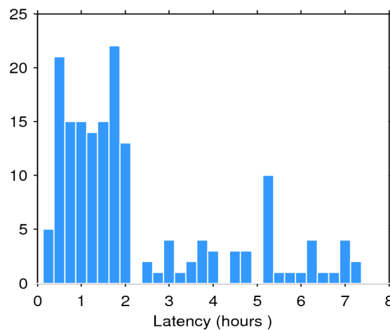
Figure 2. Histogram of the data latency for 20/03/2020. The y-axis denotes the number of files that are made available with a delay of x-hours with respect to the mean time of the records stored in the file.
