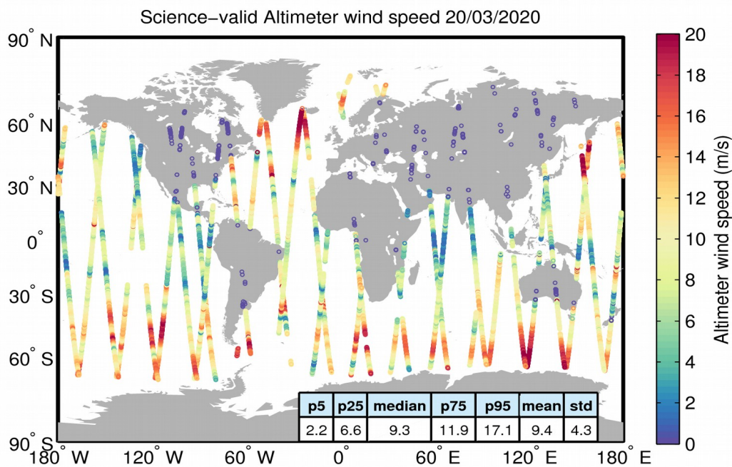
Figure 34. Geographical distribution of science-valid wind data over oceans and lakes for 20/03/2020. The statistical values shown in the table refer to the wind in m/s and are calculated over all measurements shown in the figure. Gray circles denote records that have been rejected based on the editing criteria described in Table 5.
