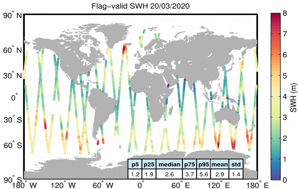
Figure 15. Geographical distribution of flag-valid SWH data over oceans and lakes for 20/03/2020. The statistical values shown in the table refer to the SWH in m and are calculated over all measurements shown in the figure.
