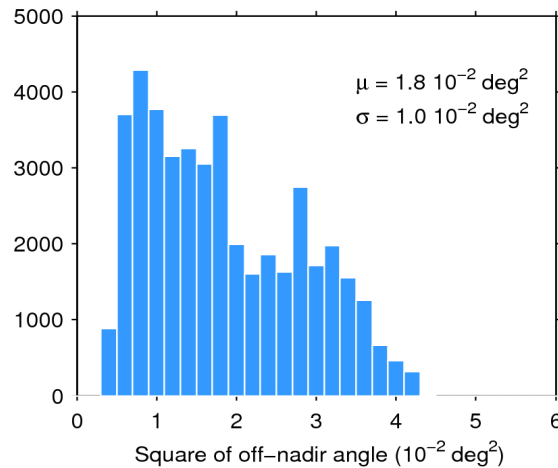
Figure 39. Histogram of flag-valid mispointing over oceans and lakes for 20/03/2020. The mean ( \mu ) and standard deviation ( \sigma ) are also shown. Note that values larger than 6 \cdot 10^{-2} \text{ deg}^2 are excluded from the histogram for the sake of readability but not from the computation of \mu and \sigma .
