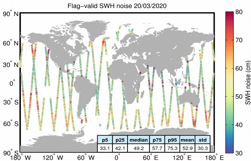
Figure 18. Geographical distribution of flag-valid 20-Hz SWH measurement noise over oceans and lakes for 20/03/2020. The statistical values shown in the figure refer to the SWH noise and are calculated over all measurements shown in the figure.
