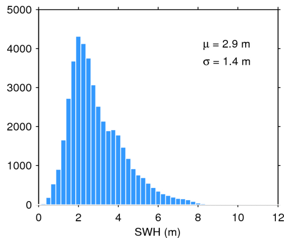
Figure 20. Histogram of science-valid SWH over oceans and lakes for 20/03/2020. The mean ( \mu ) and standard deviation ( \sigma ) are also shown. Note that values larger than 12 m are excluded from the histogram for the sake of readability but not from the computation of \mu and \sigma .
