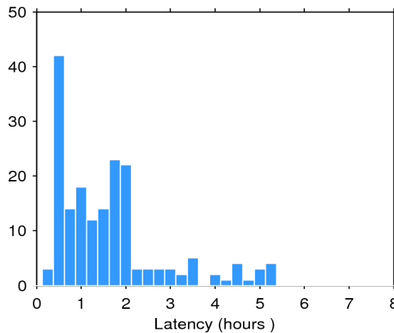
Figure 2. Histogram of the data latency for 19/03/2020. The y-axis denotes the number of files that are made available with a delay of x-hours with respect to the mean time of the records stored in the file.
