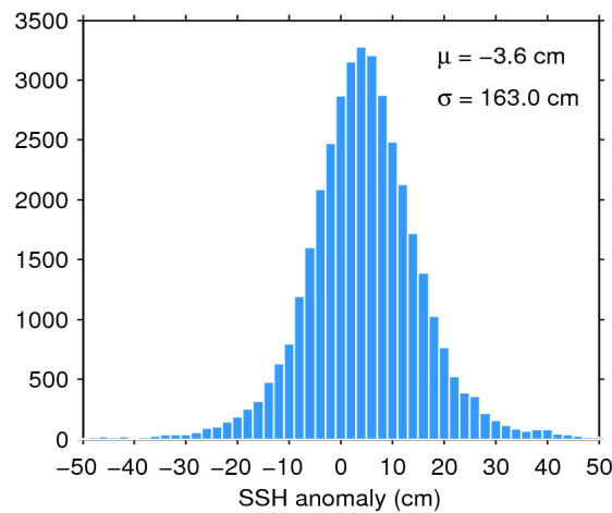
Figure 7. Histogram of flag-valid SSH anomaly over oceans and lakes for 19/03/2020. The mean ( \mu ) and standard deviation ( \sigma ) are also shown. Note that values outside [-50 50] cm are excluded from the histogram for the sake of readability but not from the computation of \mu and \sigma .
