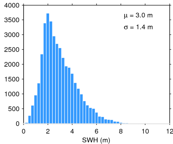
Figure 20. Histogram of science-valid SWH over oceans and lakes for 19/03/2020. The mean ( \mu ) and standard deviation ( \sigma ) are also shown. Note that values larger than 12 m are excluded from the histogram for the sake of readability but not from the computation of \mu and \sigma .
