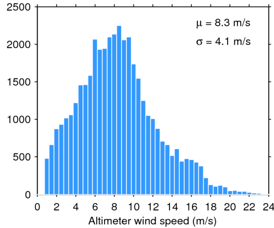
Figure 33. Histogram of flag-valid wind over oceans and lakes for 19/03/2020. The mean ( \mu ) and standard deviation ( \sigma ) are also shown. Note that values larger than 24 m/s are excluded from the histogram for the sake of readability but not from the computation of \mu and \sigma .
