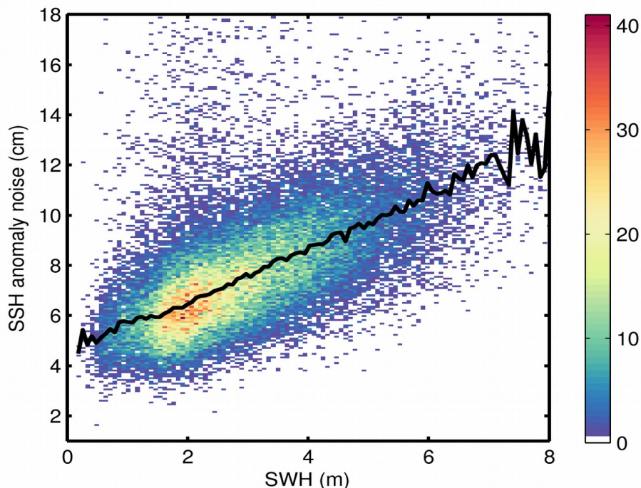
Figure 9. 2D histogram showing flag-valid SSH anomaly noise as a function of SWH for 19/03/2020. The black line denotes the median SSH anomaly noise as a function of SWH.
