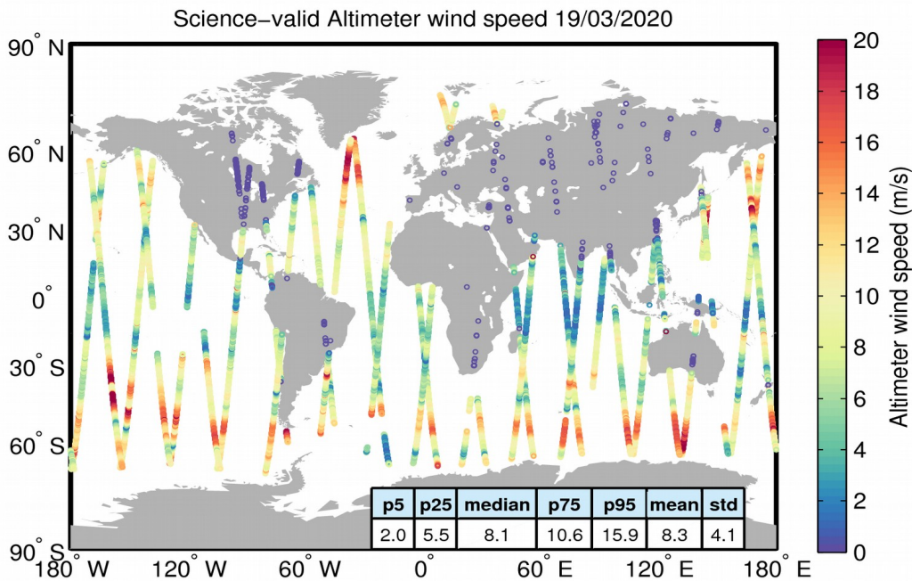
Figure 34. Geographical distribution of science-valid wind data over oceans and lakes for 19/03/2020. The statistical values shown in the table refer to the wind in m/s and are calculated over all measurements shown in the figure. Gray circles denote records that have been rejected based on the editing criteria described in Table 5.
