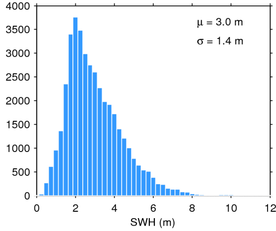
Figure 17. Histogram of flag-valid SWH over oceans and lakes for 19/03/2020. The mean ( \mu ) and standard deviation ( \sigma ) are also shown. Note that values larger than 12 m are excluded from the histogram for the sake of readability but not from the computation of \mu and \sigma .
