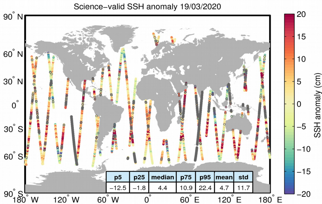
Figure 10. Geographical distribution of science-valid SSH anomaly data over oceans and lakes for 19/03/2020. The statistical values shown in the table refer to the SSH anomaly in cm and are calculated over all measurements shown in the figure. Gray circles denote records that have been rejected based on the editing criteria described in Table 2.
