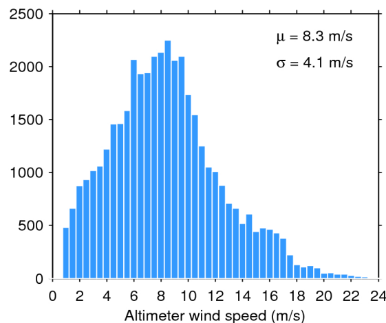
Figure 35. Histogram of science-valid wind over oceans and lakes for 19/03/2020. The mean ( \mu ) and standard deviation ( \sigma ) are also shown. Note that values larger than 24 m/s are excluded from the histogram for the sake of readability but not from the computation of \mu and \sigma .
