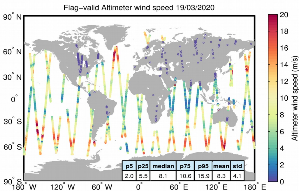
Figure 31. Geographical distribution of flag-valid wind data over oceans and lakes for 19/03/2020. The statistical values shown in the table refer to the wind in m/s and are calculated over all measurements shown in the figure.
