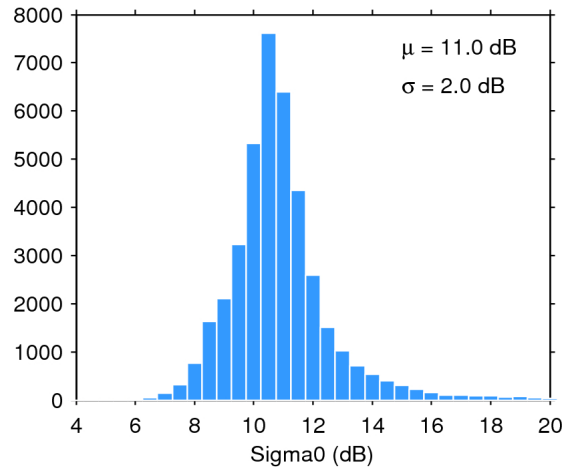
Figure 25. Histogram of flag-valid sigma0 over oceans and lakes for 19/03/2020. The mean ( \mu ) and standard deviation ( \sigma ) are also shown. Note that values outside [4 20] dB are excluded from the histogram for the sake of readability but not from the computation of \mu and \sigma .
