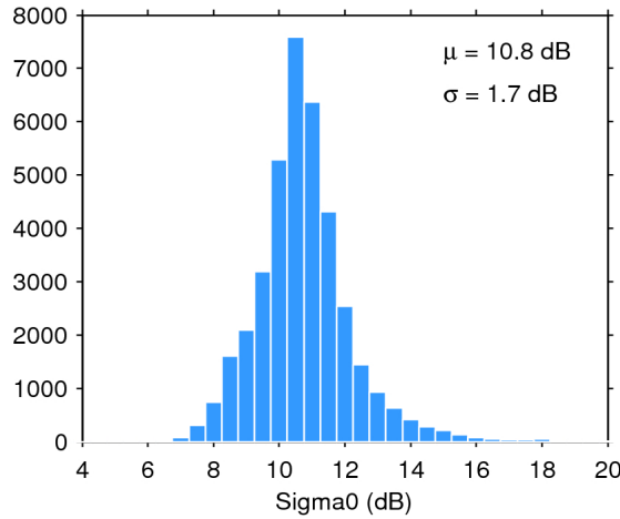
Figure 28. Histogram of science-valid sigma0 over oceans and lakes for 19/03/2020. The mean ( \mu ) and standard deviation ( \sigma ) are also shown. Note that values outside [4 20] dB are excluded from the histogram for the sake of readability but not from the computation of \mu and \sigma .
