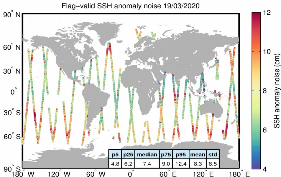
Figure 8. Geographical distribution of flag-valid 20-Hz SSH anomaly measurement noise over oceans and lakes for 19/03/2020. The statistical values shown in the table refer to the SSH anomaly noise and are calculated over all measurements shown in the figure.
