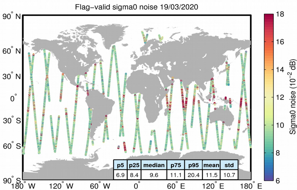
Figure 26. Geographical distribution of flag-valid 20-Hz sigma0 measurement noise over oceans and lakes for 19/03/2020. The statistical values shown in the table refer to the sigma0 noise and are calculated over all measurements shown in the figure.
