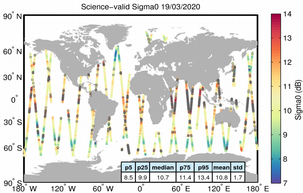
Figure 27. Geographical distribution of science-valid sigma0 data over oceans and lakes for 19/03/2020. The statistical values shown in the table refer to the sigma0 in dB and are calculated over all measurements shown in the figure. Gray circles denote records that have been rejected based on the editing criteria described in Table 4.
