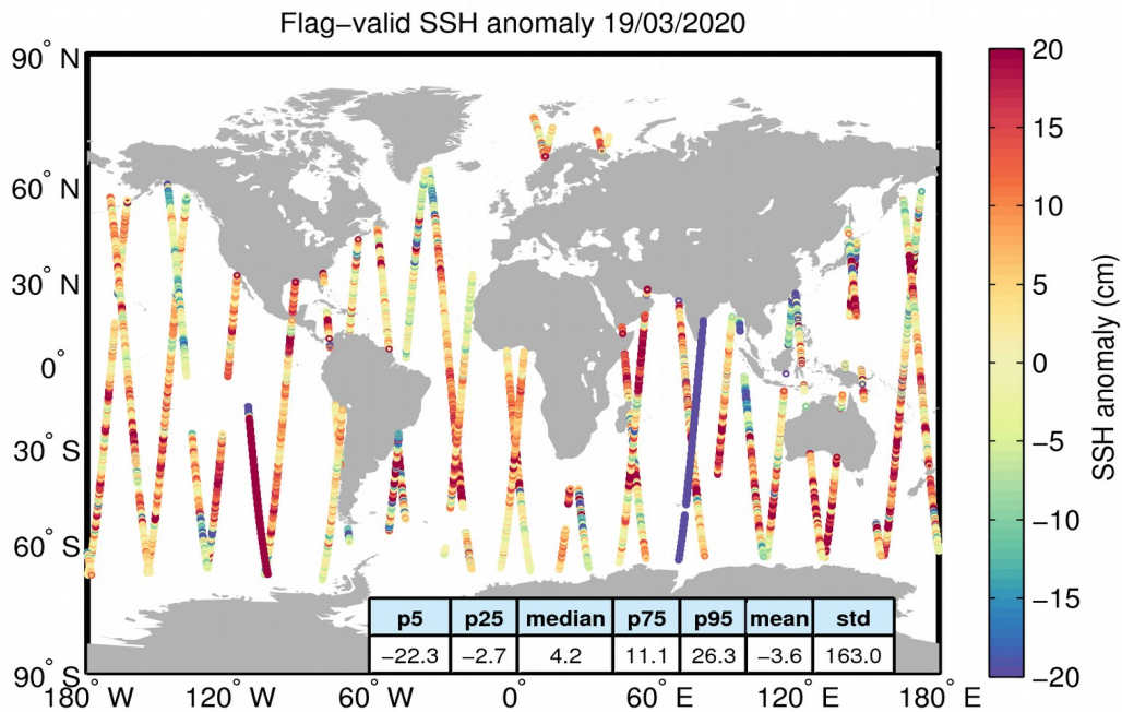
Figure 5. Geographical distribution of flag-valid 1-Hz SSH anomaly data over oceans and lakes for 19/03/2020. The statistical values shown in the table refer to the SSH anomaly in cm and are calculated over all measurements shown in the figure.
