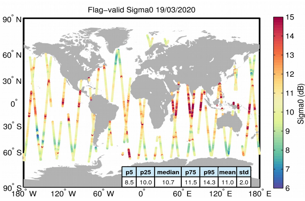
Figure 23. Geographical distribution of flag-valid sigma0 data over oceans and lakes for 19/03/2020. The statistical values shown in the table refer to the sigma0 in dB and are calculated over all measurements shown in the figure.
