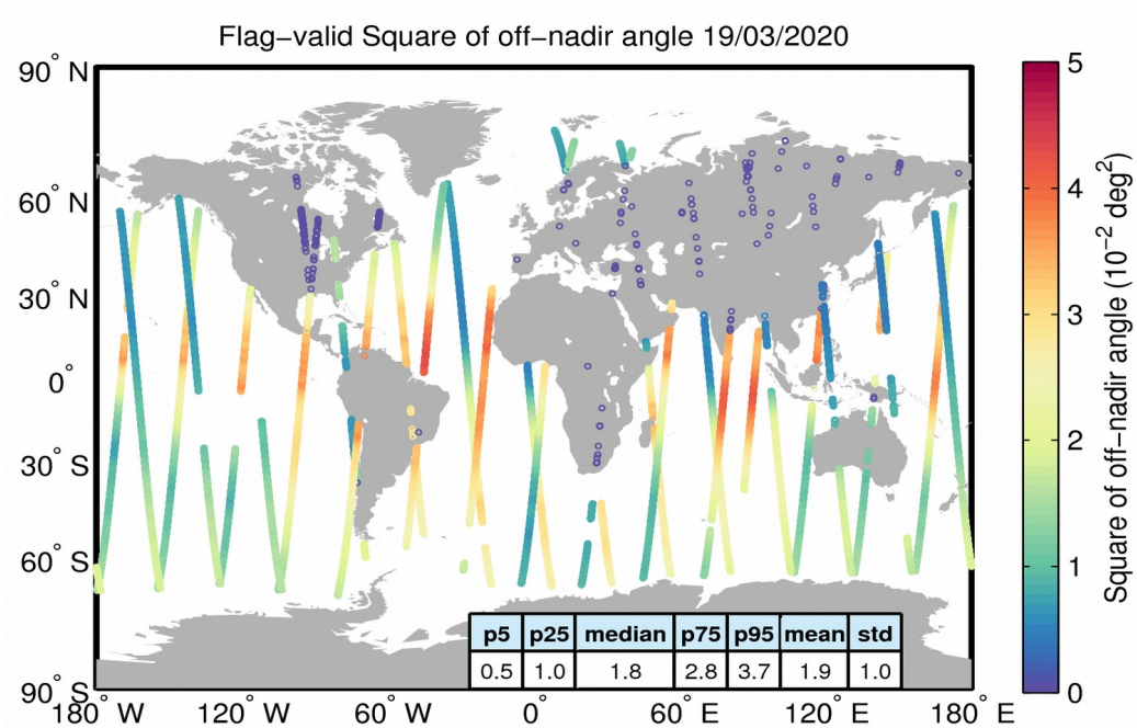
Figure 37. Geographical distribution of flag-valid mispointing data over oceans and lakes for 19/03/2020. The statistical values shown in the table refer to the mispointing in 10^{-2} \text{ deg}^2 and are calculated over all measurements shown in the figure.
