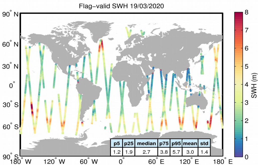
Figure 15. Geographical distribution of flag-valid SWH data over oceans and lakes for 19/03/2020. The statistical values shown in the table refer to the SWH in m and are calculated over all measurements shown in the figure.
