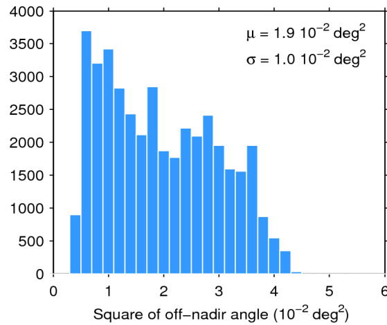
Figure 39. Histogram of flag-valid mispointing over oceans and lakes for 19/03/2020. The mean ( \mu ) and standard deviation ( \sigma ) are also shown. Note that values larger than 6 \cdot 10^{-2} \text{ deg}^2 are excluded from the histogram for the sake of readability but not from the computation of \mu and \sigma .
