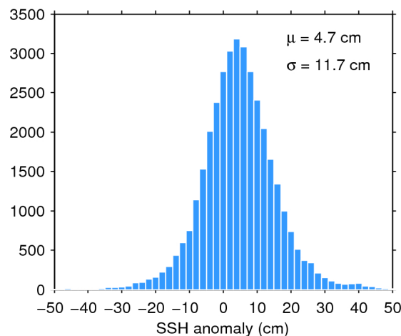
Figure 11. Histogram of science-valid SSH anomaly over oceans and lakes for 19/03/2020. The mean ( \mu ) and standard deviation ( \sigma ) are also shown. Note that values outside [-50 50] cm are excluded from the histogram for the sake of readability but not from the computation of \mu and \sigma .
