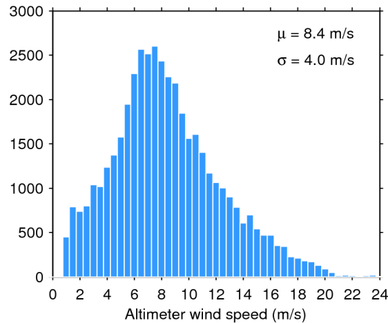
Figure 33. Histogram of flag-valid wind over oceans and lakes for 18/03/2020. The mean ( \mu ) and standard deviation ( \sigma ) are also shown. Note that values larger than 24 m/s are excluded from the histogram for the sake of readability but not from the computation of \mu and \sigma .
