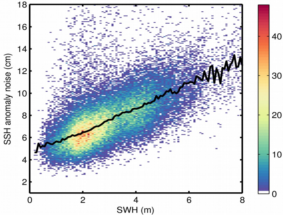
Figure 9. 2D histogram showing flag-valid SSH anomaly noise as a function of SWH for 18/03/2020. The black line denotes the median SSH anomaly noise as a function of SWH.
