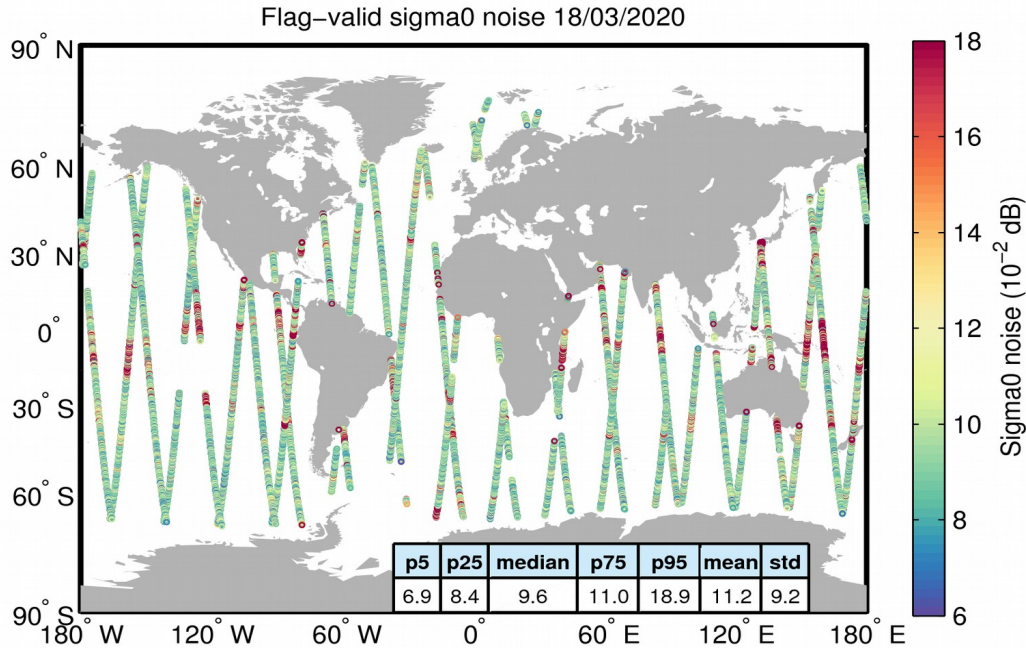
Figure 26. Geographical distribution of flag-valid 20-Hz sigma0 measurement noise over oceans and lakes for 18/03/2020. The statistical values shown in the table refer to the sigma0 noise and are calculated over all measurements shown in the figure.
