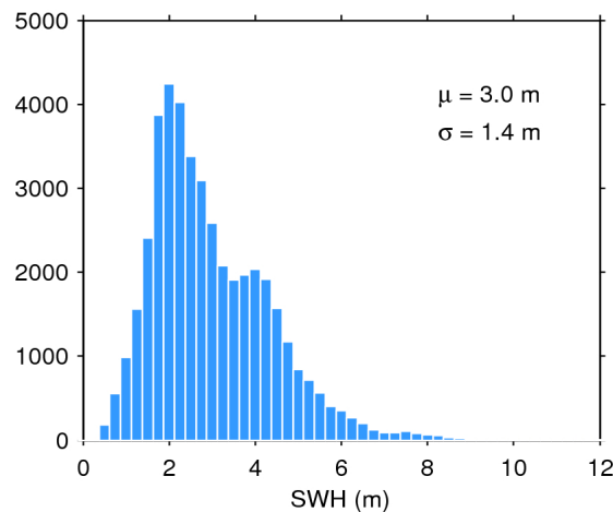
Figure 17. Histogram of flag-valid SWH over oceans and lakes for 18/03/2020. The mean ( \mu ) and standard deviation ( \sigma ) are also shown. Note that values larger than 12 m are excluded from the histogram for the sake of readability but not from the computation of \mu and \sigma .
