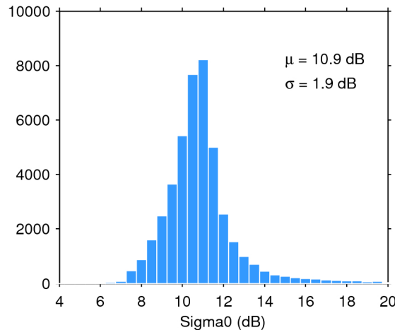
Figure 25. Histogram of flag-valid sigma0 over oceans and lakes for 18/03/2020. The mean ( \mu ) and standard deviation ( \sigma ) are also shown. Note that values outside [4 20] dB are excluded from the histogram for the sake of readability but not from the computation of \mu and \sigma .
