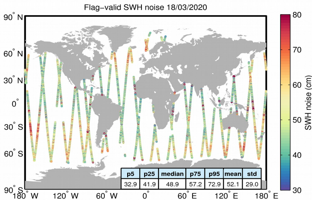
Figure 18. Geographical distribution of flag-valid 20-Hz SWH measurement noise over oceans and lakes for 18/03/2020. The statistical values shown in the figure refer to the SWH noise and are calculated over all measurements shown in the figure.
