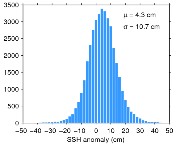
Figure 11. Histogram of science-valid SSH anomaly over oceans and lakes for 18/03/2020. The mean ( \mu ) and standard deviation ( \sigma ) are also shown. Note that values outside [-50 50] cm are excluded from the histogram for the sake of readability but not from the computation of \mu and \sigma .
