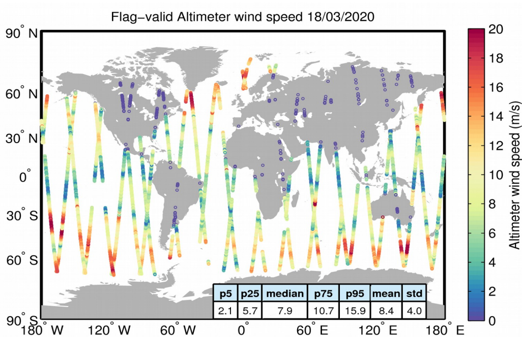
Figure 31. Geographical distribution of flag-valid wind data over oceans and lakes for 18/03/2020. The statistical values shown in the table refer to the wind in m/s and are calculated over all measurements shown in the figure.
