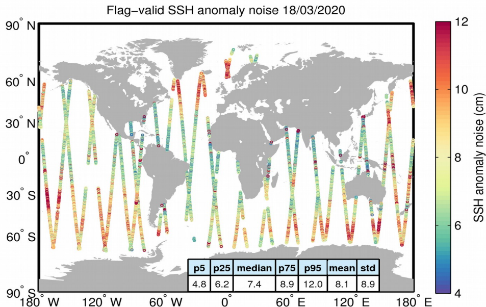
Figure 8. Geographical distribution of flag-valid 20-Hz SSH anomaly measurement noise over oceans and lakes for 18/03/2020. The statistical values shown in the table refer to the SSH anomaly noise and are calculated over all measurements shown in the figure.
