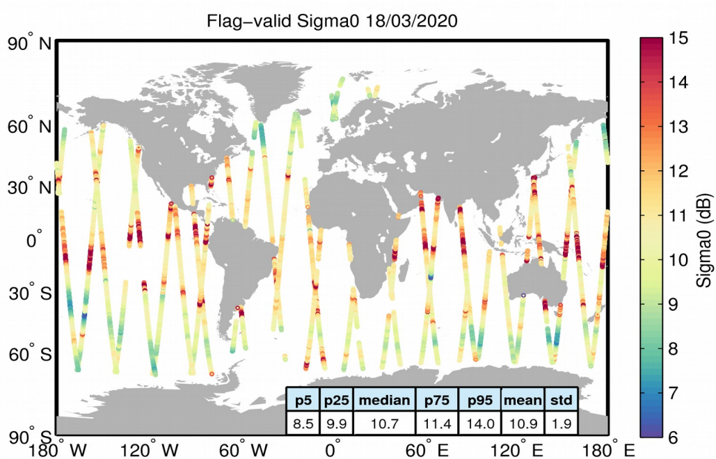
Figure 23. Geographical distribution of flag-valid sigma0 data over oceans and lakes for 18/03/2020. The statistical values shown in the table refer to the sigma0 in dB and are calculated over all measurements shown in the figure.
