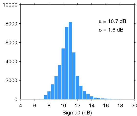
Figure 28. Histogram of science-valid sigma0 over oceans and lakes for 18/03/2020. The mean ( \mu ) and standard deviation ( \sigma ) are also shown. Note that values outside [4 20] dB are excluded from the histogram for the sake of readability but not from the computation of \mu and \sigma .
