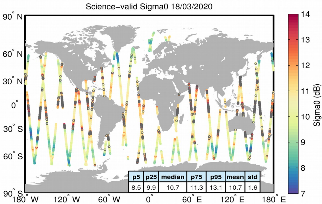
Figure 27. Geographical distribution of science-valid sigma0 data over oceans and lakes for 18/03/2020. The statistical values shown in the table refer to the sigma0 in dB and are calculated over all measurements shown in the figure. Gray circles denote records that have been rejected based on the editing criteria described in Table 4.
