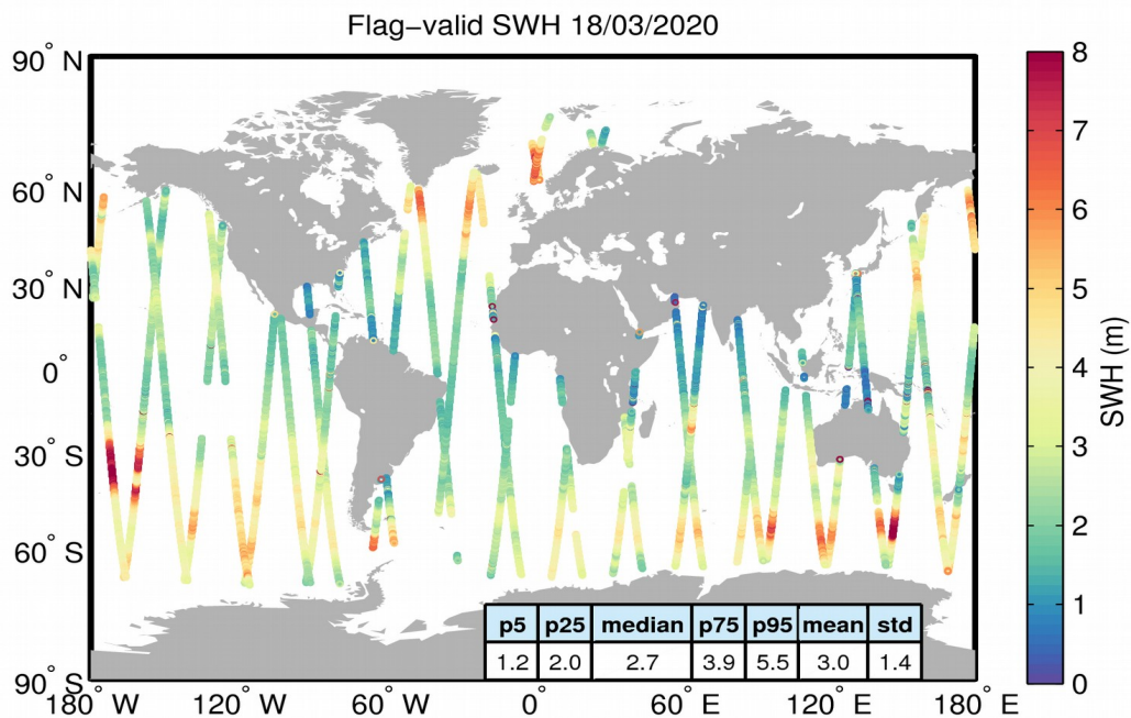
Figure 15. Geographical distribution of flag-valid SWH data over oceans and lakes for 18/03/2020. The statistical values shown in the table refer to the SWH in m and are calculated over all measurements shown in the figure.
