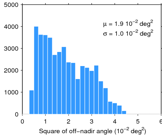
Figure 39. Histogram of flag-valid mispointing over oceans and lakes for 18/03/2020. The mean ( \mu ) and standard deviation ( \sigma ) are also shown. Note that values larger than 6 \cdot 10^{-2} \text{ deg}^2 are excluded from the histogram for the sake of readability but not from the computation of \mu and \sigma .
