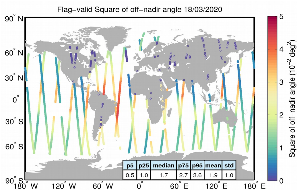
Figure 37. Geographical distribution of flag-valid mispointing data over oceans and lakes for 18/03/2020. The statistical values shown in the table refer to the mispointing in 10^{-2} deg 2 and are calculated over all measurements shown in the figure.
