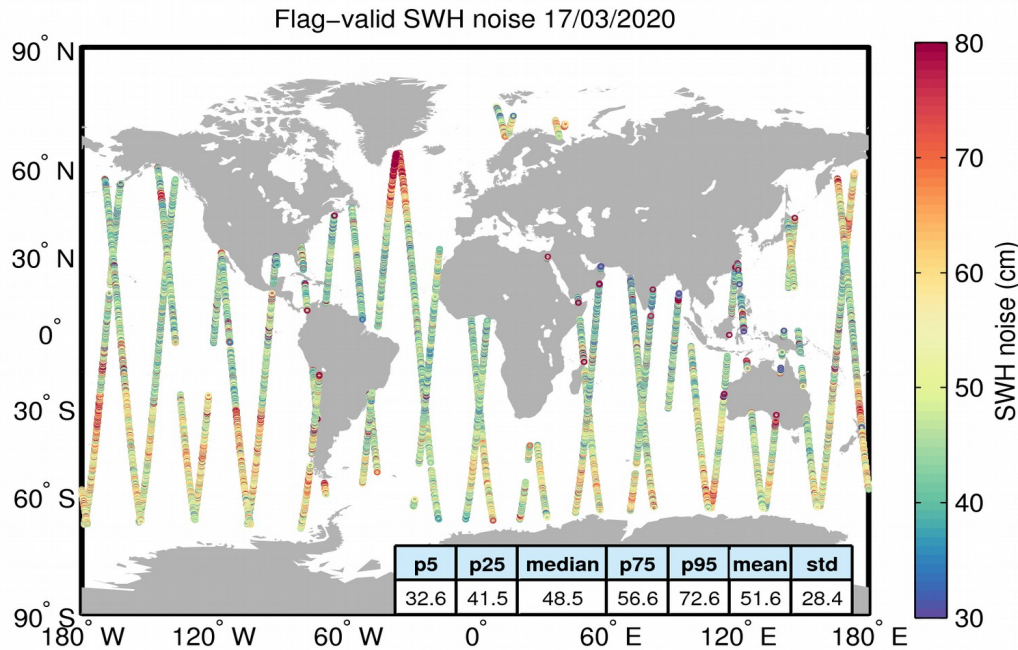
Figure 18. Geographical distribution of flag-valid 20-Hz SWH measurement noise over oceans and lakes for 17/03/2020. The statistical values shown in the figure refer to the SWH noise and are calculated over all measurements shown in the figure.
