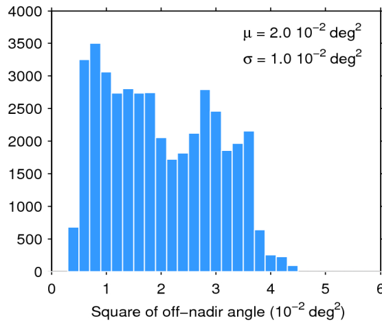
Figure 39. Histogram of flag-valid mispointing over oceans and lakes for 17/03/2020. The mean ( \mu ) and standard deviation ( \sigma ) are also shown. Note that values larger than 6 \cdot 10^{-2} \text{ deg}^2 are excluded from the histogram for the sake of readability but not from the computation of \mu and \sigma .
