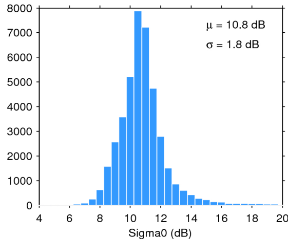
Figure 25. Histogram of flag-valid sigma0 over oceans and lakes for 17/03/2020. The mean ( \mu ) and standard deviation ( \sigma ) are also shown. Note that values outside [4 20] dB are excluded from the histogram for the sake of readability but not from the computation of \mu and \sigma .
