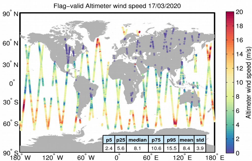
Figure 31. Geographical distribution of flag-valid wind data over oceans and lakes for 17/03/2020. The statistical values shown in the table refer to the wind in m/s and are calculated over all measurements shown in the figure.
