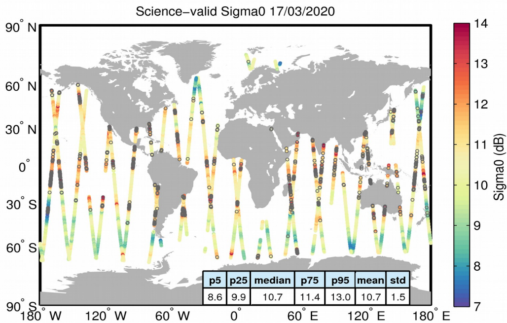
Figure 27. Geographical distribution of science-valid sigma0 data over oceans and lakes for 17/03/2020. The statistical values shown in the table refer to the sigma0 in dB and are calculated over all measurements shown in the figure. Gray circles denote records that have been rejected based on the editing criteria described in Table 4.
