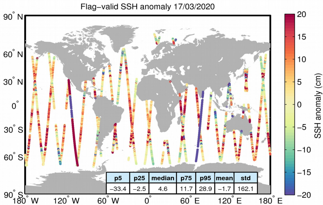
Figure 5. Geographical distribution of flag-valid 1-Hz SSH anomaly data over oceans and lakes for 17/03/2020. The statistical values shown in the table refer to the SSH anomaly in cm and are calculated over all measurements shown in the figure.
