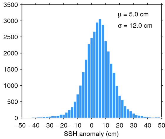
Figure 11. Histogram of science-valid SSH anomaly over oceans and lakes for 17/03/2020. The mean ( \mu ) and standard deviation ( \sigma ) are also shown. Note that values outside [-50 50] cm are excluded from the histogram for the sake of readability but not from the computation of \mu and \sigma .
