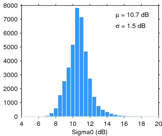
Figure 28. Histogram of science-valid sigma0 over oceans and lakes for 17/03/2020. The mean ( \mu ) and standard deviation ( \sigma ) are also shown. Note that values outside [4 20] dB are excluded from the histogram for the sake of readability but not from the computation of \mu and \sigma .
