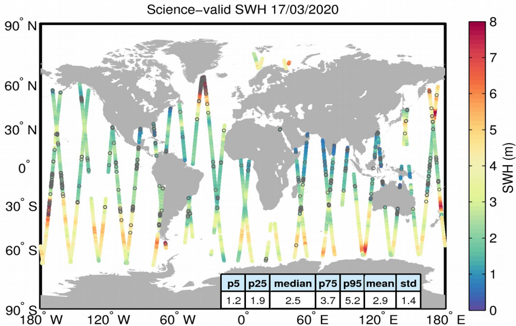
Figure 19. Geographical distribution of science-valid SWH data over oceans and lakes for 17/03/2020. The statistical values shown in the table refer to the SWH in m and are calculated over all measurements shown in the figure. Gray circles denote records that have been rejected based on the editing criteria described in Table 3.
