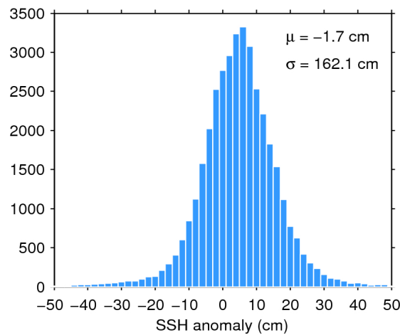
Figure 7. Histogram of flag-valid SSH anomaly over oceans and lakes for 17/03/2020. The mean ( \mu ) and standard deviation ( \sigma ) are also shown. Note that values outside [-50\ 50] cm are excluded from the histogram for the sake of readability but not from the computation of \mu and \sigma .
