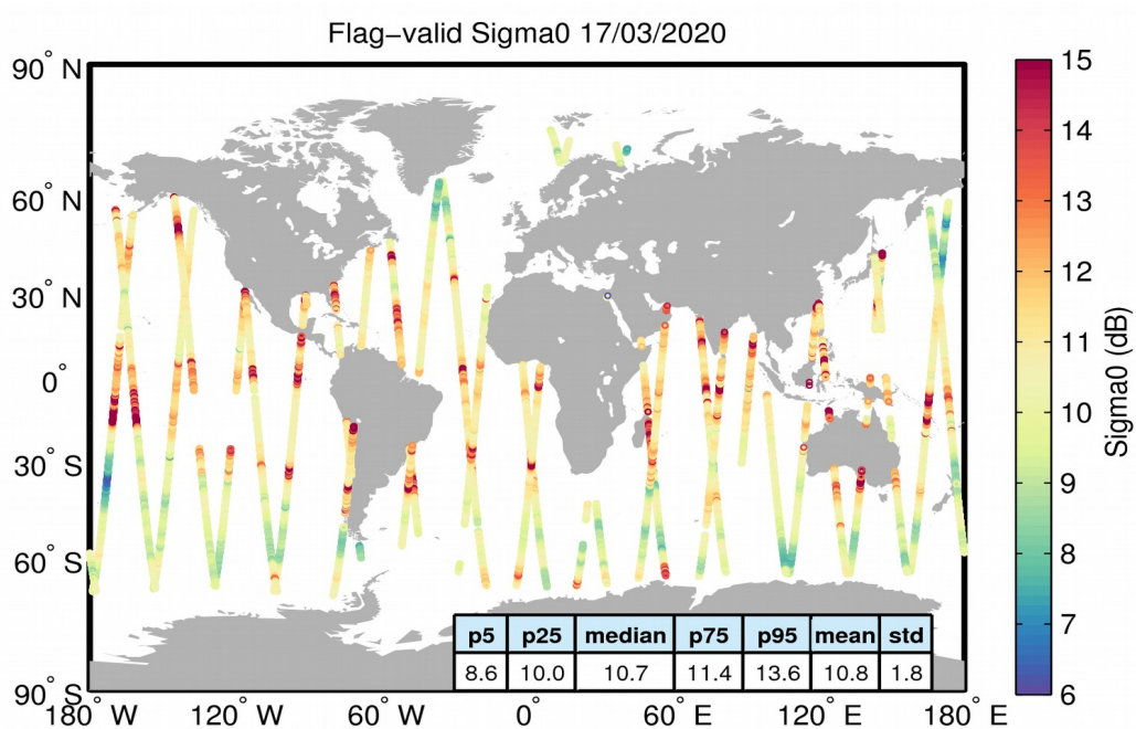
Figure 23. Geographical distribution of flag-valid sigma0 data over oceans and lakes for 17/03/2020. The statistical values shown in the table refer to the sigma0 in dB and are calculated over all measurements shown in the figure.
