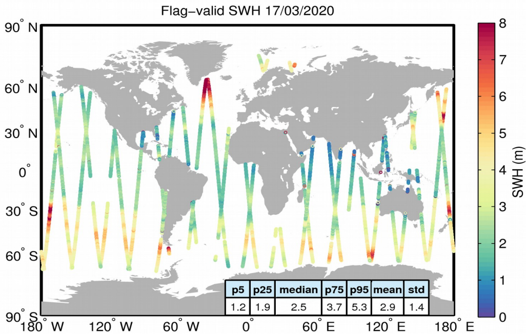
Figure 15. Geographical distribution of flag-valid SWH data over oceans and lakes for 17/03/2020. The statistical values shown in the table refer to the SWH in m and are calculated over all measurements shown in the figure.
