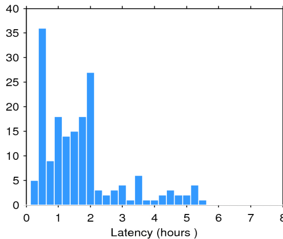
Figure 2. Histogram of the data latency for 17/03/2020. The y-axis denotes the number of files that are made available with a delay of x-hours with respect to the mean time of the records stored in the file.
