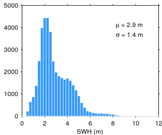
Figure 17. Histogram of flag-valid SWH over oceans and lakes for 17/03/2020. The mean ( \mu ) and standard deviation ( \sigma ) are also shown. Note that values larger than 12 m are excluded from the histogram for the sake of readability but not from the computation of \mu and \sigma .
