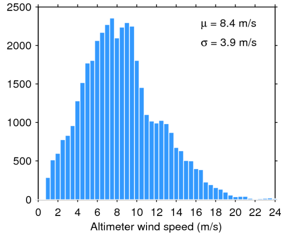
Figure 33. Histogram of flag-valid wind over oceans and lakes for 17/03/2020. The mean ( \mu ) and standard deviation ( \sigma ) are also shown. Note that values larger than 24 m/s are excluded from the histogram for the sake of readability but not from the computation of \mu and \sigma .
