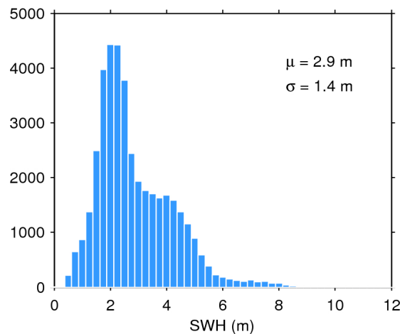
Figure 20. Histogram of science-valid SWH over oceans and lakes for 17/03/2020. The mean ( \mu ) and standard deviation ( \sigma ) are also shown. Note that values larger than 12 m are excluded from the histogram for the sake of readability but not from the computation of \mu and \sigma .
