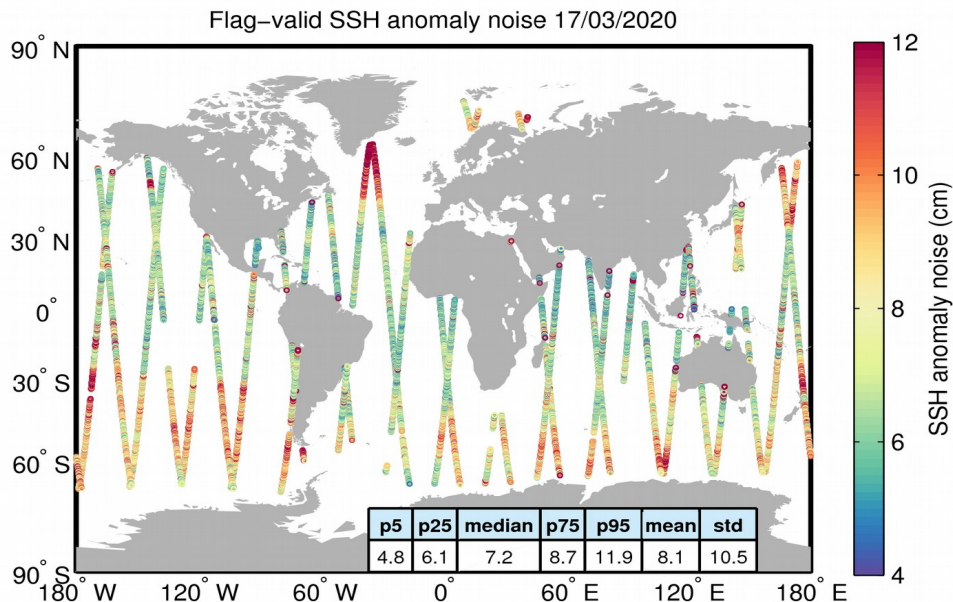
Figure 8. Geographical distribution of flag-valid 20-Hz SSH anomaly measurement noise over oceans and lakes for 17/03/2020. The statistical values shown in the table refer to the SSH anomaly noise and are calculated over all measurements shown in the figure.
