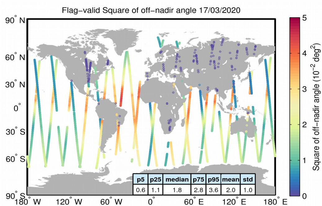
Figure 37. Geographical distribution of flag-valid mispointing data over oceans and lakes for 17/03/2020. The statistical values shown in the table refer to the mispointing in 10^{-2} deg 2 and are calculated over all measurements shown in the figure.
