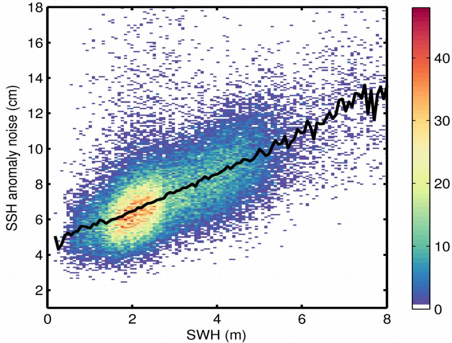
Figure 9. 2D histogram showing flag-valid SSH anomaly noise as a function of SWH for 17/03/2020. The black line denotes the median SSH anomaly noise as a function of SWH.
