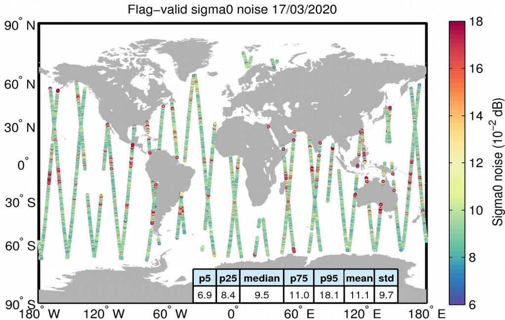
Figure 26. Geographical distribution of flag-valid 20-Hz sigma0 measurement noise over oceans and lakes for 17/03/2020. The statistical values shown in the table refer to the sigma0 noise and are calculated over all measurements shown in the figure.
