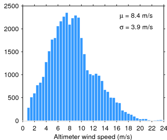
Figure 35. Histogram of science-valid wind over oceans and lakes for 17/03/2020. The mean ( \mu ) and standard deviation ( \sigma ) are also shown. Note that values larger than 24 m/s are excluded from the histogram for the sake of readability but not from the computation of \mu and \sigma .
