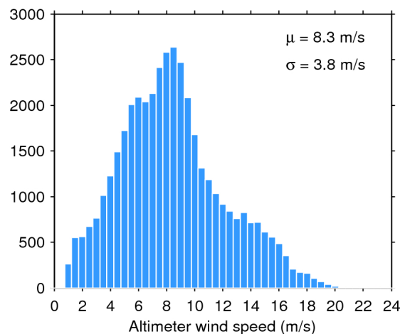
Figure 35. Histogram of science-valid wind over oceans and lakes for 15/03/2020. The mean ( \mu ) and standard deviation ( \sigma ) are also shown. Note that values larger than 24 m/s are excluded from the histogram for the sake of readability but not from the computation of \mu and \sigma .
