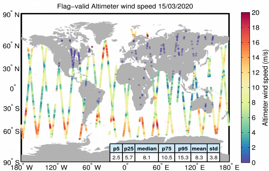
Figure 31. Geographical distribution of flag-valid wind data over oceans and lakes for 15/03/2020. The statistical values shown in the table refer to the wind in m/s and are calculated over all measurements shown in the figure.
