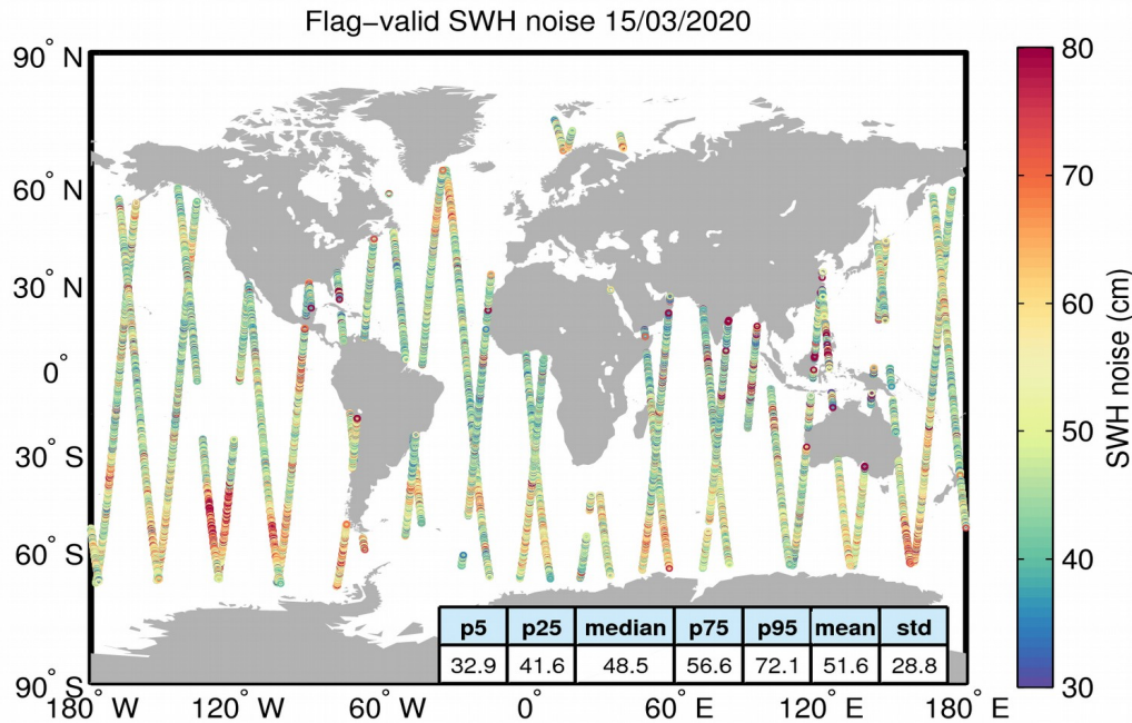
Figure 18. Geographical distribution of flag-valid 20-Hz SWH measurement noise over oceans and lakes for 15/03/2020. The statistical values shown in the figure refer to the SWH noise and are calculated over all measurements shown in the figure.
