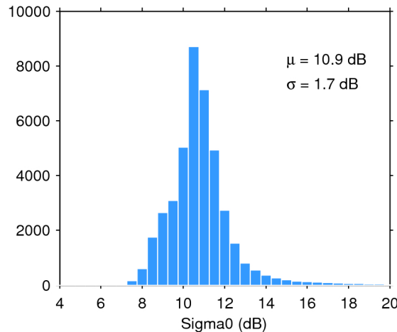
Figure 25. Histogram of flag-valid sigma0 over oceans and lakes for 15/03/2020. The mean ( \mu ) and standard deviation ( \sigma ) are also shown. Note that values outside [4 20] dB are excluded from the histogram for the sake of readability but not from the computation of \mu and \sigma .
