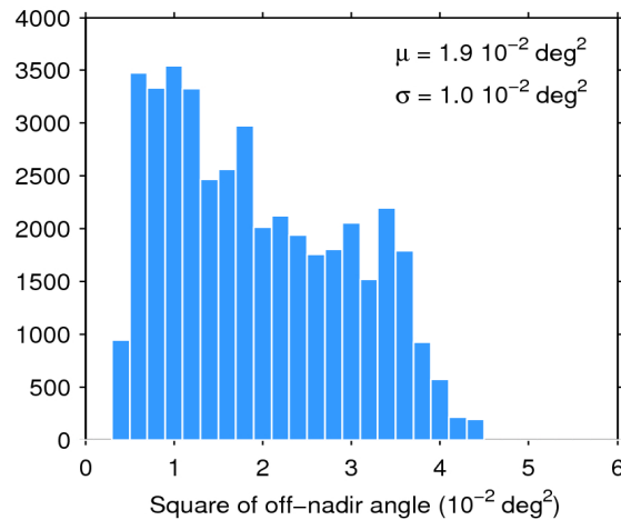
Figure 39. Histogram of flag-valid mispointing over oceans and lakes for 15/03/2020. The mean ( \mu ) and standard deviation ( \sigma ) are also shown. Note that values larger than 6 \cdot 10^{-2} \text{ deg}^2 are excluded from the histogram for the sake of readability but not from the computation of \mu and \sigma .
