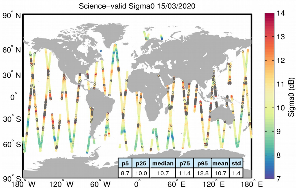
Figure 27. Geographical distribution of science-valid sigma0 data over oceans and lakes for 15/03/2020. The statistical values shown in the table refer to the sigma0 in dB and are calculated over all measurements shown in the figure. Gray circles denote records that have been rejected based on the editing criteria described in Table 4.
