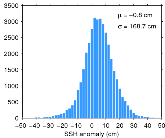
Figure 7. Histogram of flag-valid SSH anomaly over oceans and lakes for 15/03/2020. The mean ( \mu ) and standard deviation ( \sigma ) are also shown. Note that values outside [-50\ 50] cm are excluded from the histogram for the sake of readability but not from the computation of \mu and \sigma .
