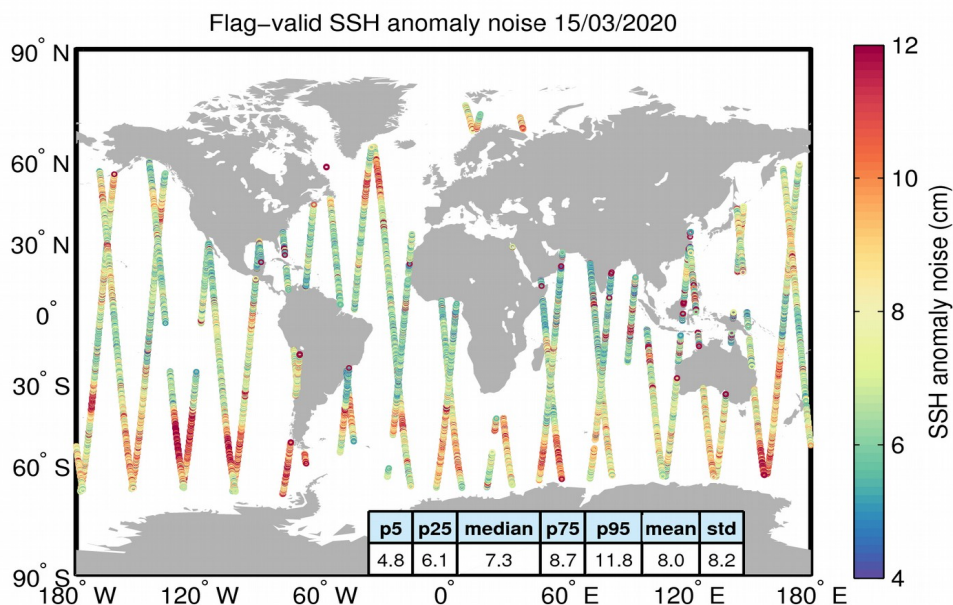
Figure 8. Geographical distribution of flag-valid 20-Hz SSH anomaly measurement noise over oceans and lakes for 15/03/2020. The statistical values shown in the table refer to the SSH anomaly noise and are calculated over all measurements shown in the figure.
