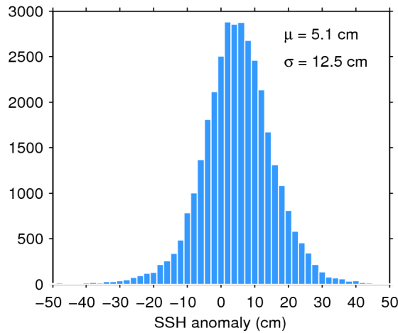
Figure 11. Histogram of science-valid SSH anomaly over oceans and lakes for 15/03/2020. The mean ( \mu ) and standard deviation ( \sigma ) are also shown. Note that values outside [-50 50] cm are excluded from the histogram for the sake of readability but not from the computation of \mu and \sigma .
