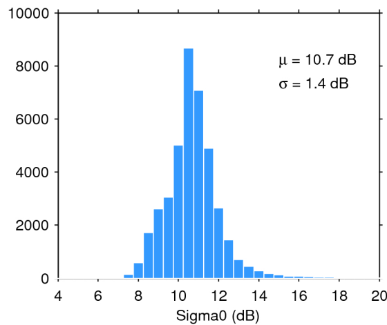
Figure 28. Histogram of science-valid sigma0 over oceans and lakes for 15/03/2020. The mean ( \mu ) and standard deviation ( \sigma ) are also shown. Note that values outside [4 20] dB are excluded from the histogram for the sake of readability but not from the computation of \mu and \sigma .
