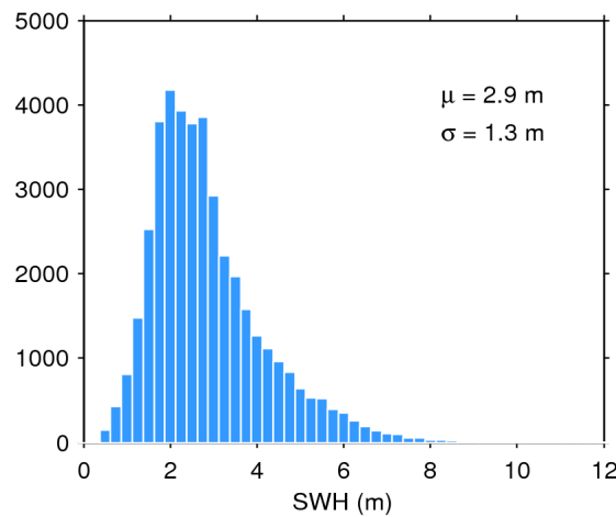
Figure 17. Histogram of flag-valid SWH over oceans and lakes for 15/03/2020. The mean ( \mu ) and standard deviation ( \sigma ) are also shown. Note that values larger than 12 m are excluded from the histogram for the sake of readability but not from the computation of \mu and \sigma .
