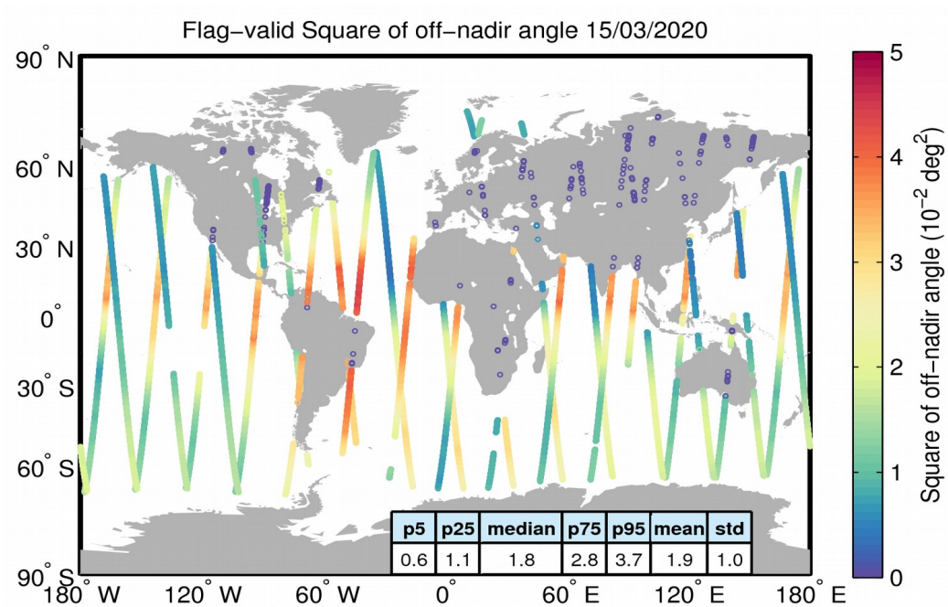
Figure 37. Geographical distribution of flag-valid mispointing data over oceans and lakes for 15/03/2020. The statistical values shown in the table refer to the mispointing in 10^{-2} deg 2 and are calculated over all measurements shown in the figure.
