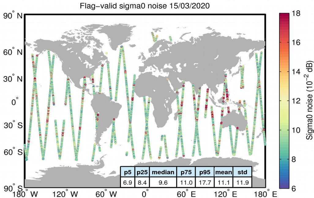
Figure 26. Geographical distribution of flag-valid 20-Hz sigma0 measurement noise over oceans and lakes for 15/03/2020. The statistical values shown in the table refer to the sigma0 noise and are calculated over all measurements shown in the figure.
