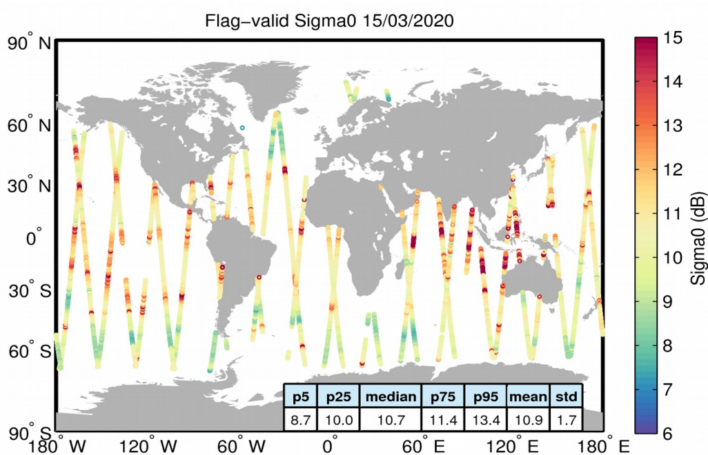
Figure 23. Geographical distribution of flag-valid sigma0 data over oceans and lakes for 15/03/2020. The statistical values shown in the table refer to the sigma0 in dB and are calculated over all measurements shown in the figure.
