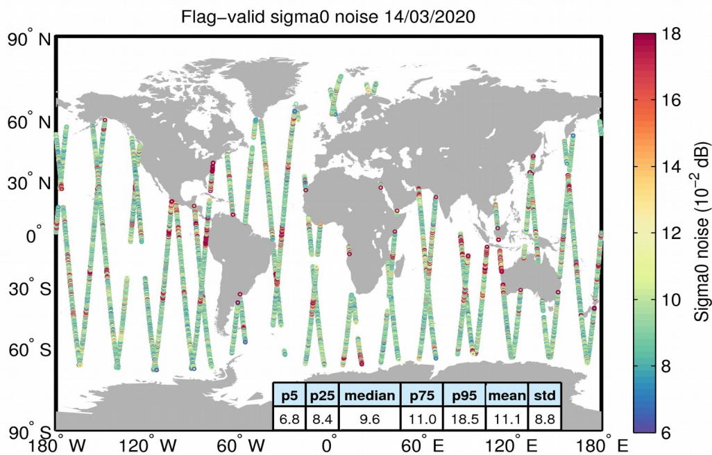
Figure 26. Geographical distribution of flag-valid 20-Hz sigma0 measurement noise over oceans and lakes for 14/03/2020. The statistical values shown in the table refer to the sigma0 noise and are calculated over all measurements shown in the figure.
