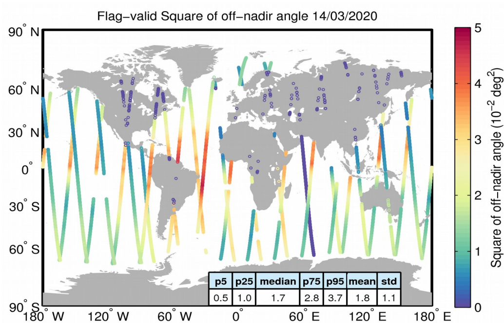
Figure 37. Geographical distribution of flag-valid mispointing data over oceans and lakes for 14/03/2020. The statistical values shown in the table refer to the mispointing in 10^{-2} \text{ deg}^2 and are calculated over all measurements shown in the figure.
