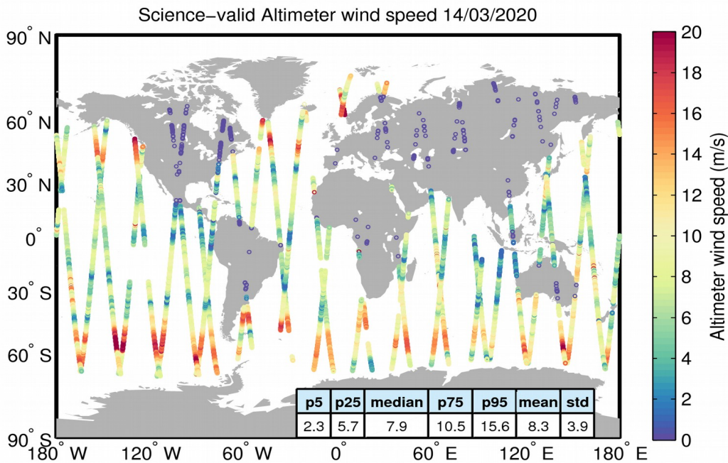
Figure 34. Geographical distribution of science-valid wind data over oceans and lakes for 14/03/2020. The statistical values shown in the table refer to the wind in m/s and are calculated over all measurements shown in the figure. Gray circles denote records that have been rejected based on the editing criteria described in Table 5.
