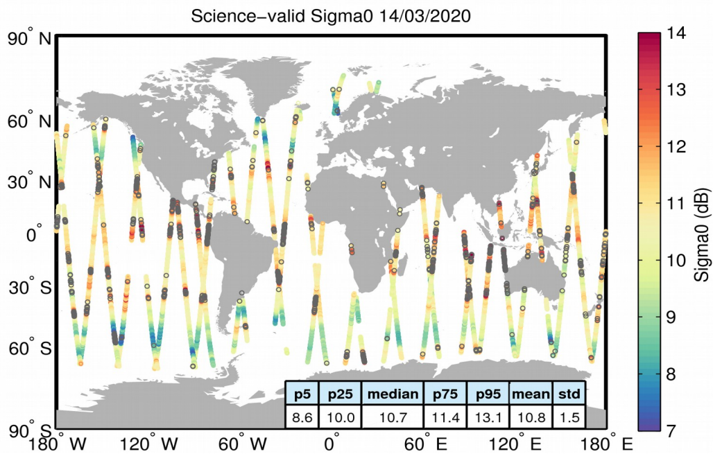
Figure 27. Geographical distribution of science-valid sigma0 data over oceans and lakes for 14/03/2020. The statistical values shown in the table refer to the sigma0 in dB and are calculated over all measurements shown in the figure. Gray circles denote records that have been rejected based on the editing criteria described in Table 4.
