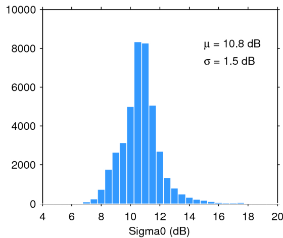
Figure 28. Histogram of science-valid sigma0 over oceans and lakes for 14/03/2020. The mean ( \mu ) and standard deviation ( \sigma ) are also shown. Note that values outside [4 20] dB are excluded from the histogram for the sake of readability but not from the computation of \mu and \sigma .
