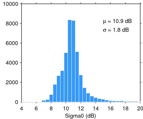
Figure 25. Histogram of flag-valid sigma0 over oceans and lakes for 14/03/2020. The mean ( \mu ) and standard deviation ( \sigma ) are also shown. Note that values outside [4 20] dB are excluded from the histogram for the sake of readability but not from the computation of \mu and \sigma .
