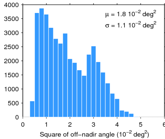
Figure 39. Histogram of flag-valid mispointing over oceans and lakes for 14/03/2020. The mean ( \mu ) and standard deviation ( \sigma ) are also shown. Note that values larger than 6 \cdot 10^{-2} \text{ deg}^2 are excluded from the histogram for the sake of readability but not from the computation of \mu and \sigma .
