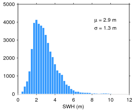
Figure 17. Histogram of flag-valid SWH over oceans and lakes for 14/03/2020. The mean ( \mu ) and standard deviation ( \sigma ) are also shown. Note that values larger than 12 m are excluded from the histogram for the sake of readability but not from the computation of \mu and \sigma .
