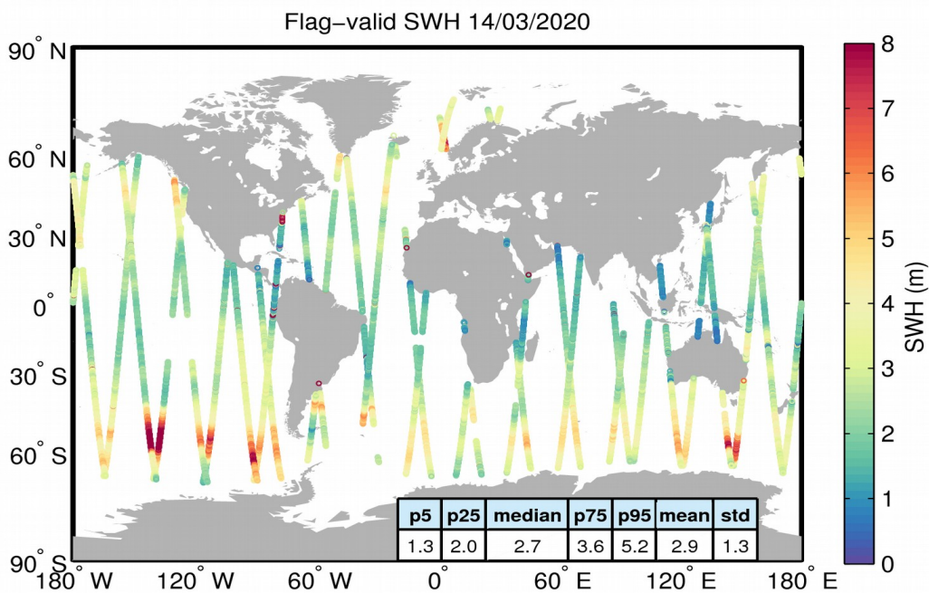
Figure 15. Geographical distribution of flag-valid SWH data over oceans and lakes for 14/03/2020. The statistical values shown in the table refer to the SWH in m and are calculated over all measurements shown in the figure.
