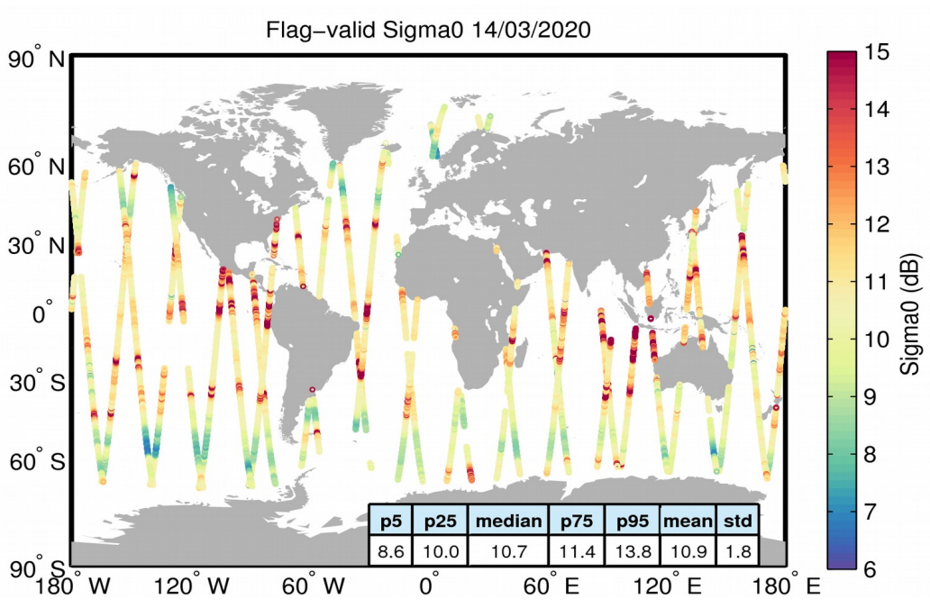
Figure 23. Geographical distribution of flag-valid sigma0 data over oceans and lakes for 14/03/2020. The statistical values shown in the table refer to the sigma0 in dB and are calculated over all measurements shown in the figure.
