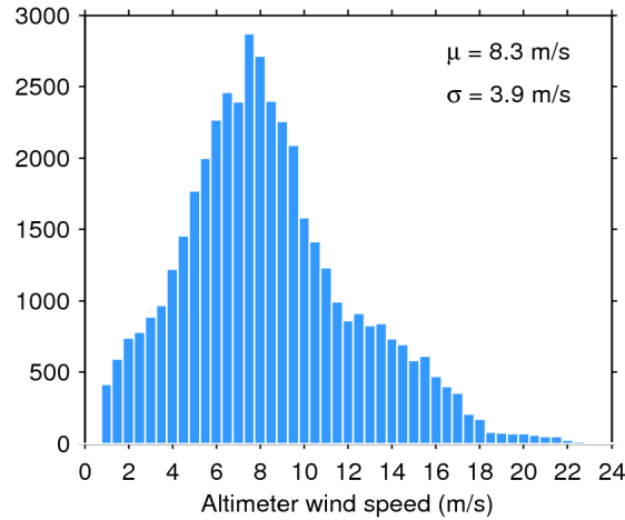
Figure 33. Histogram of flag-valid wind over oceans and lakes for 14/03/2020. The mean ( \mu ) and standard deviation ( \sigma ) are also shown. Note that values larger than 24 m/s are excluded from the histogram for the sake of readability but not from the computation of \mu and \sigma .
