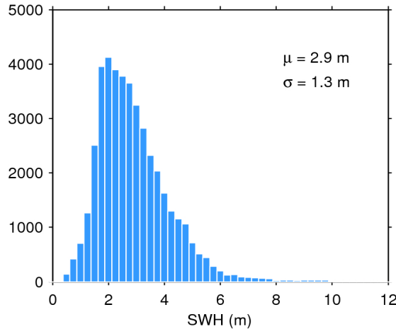
Figure 20. Histogram of science-valid SWH over oceans and lakes for 14/03/2020. The mean ( \mu ) and standard deviation ( \sigma ) are also shown. Note that values larger than 12 m are excluded from the histogram for the sake of readability but not from the computation of \mu and \sigma .
