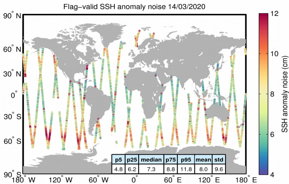
Figure 8. Geographical distribution of flag-valid 20-Hz SSH anomaly measurement noise over oceans and lakes for 14/03/2020. The statistical values shown in the table refer to the SSH anomaly noise and are calculated over all measurements shown in the figure.
