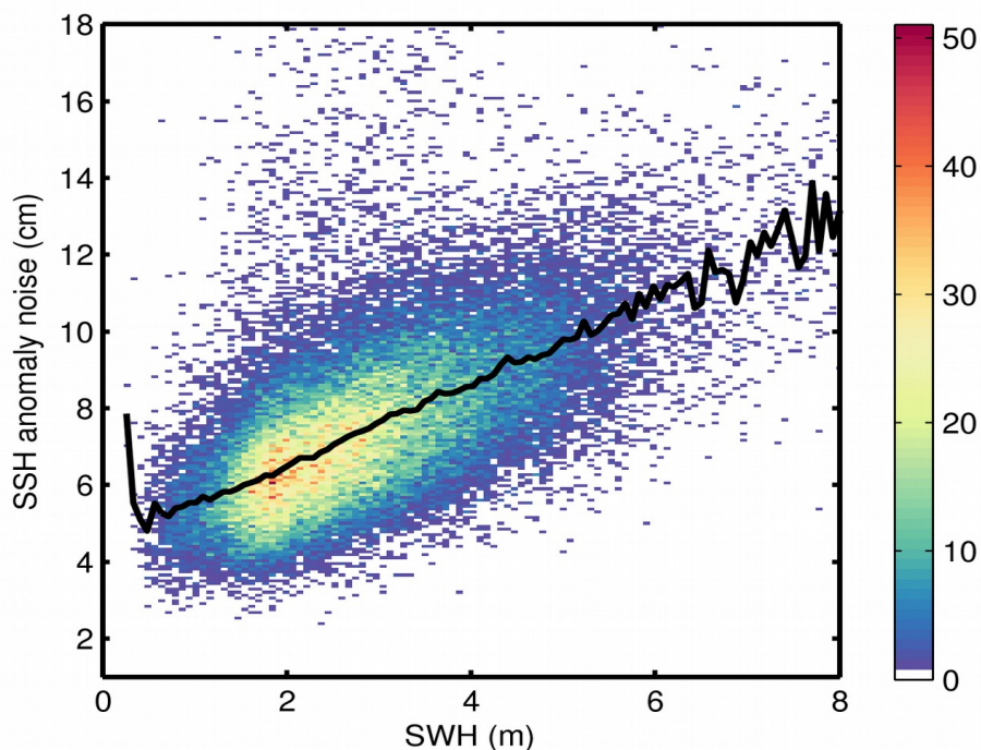
Figure 9. 2D histogram showing flag-valid SSH anomaly noise as a function of SWH for 14/03/2020. The black line denotes the median SSH anomaly noise as a function of SWH.
