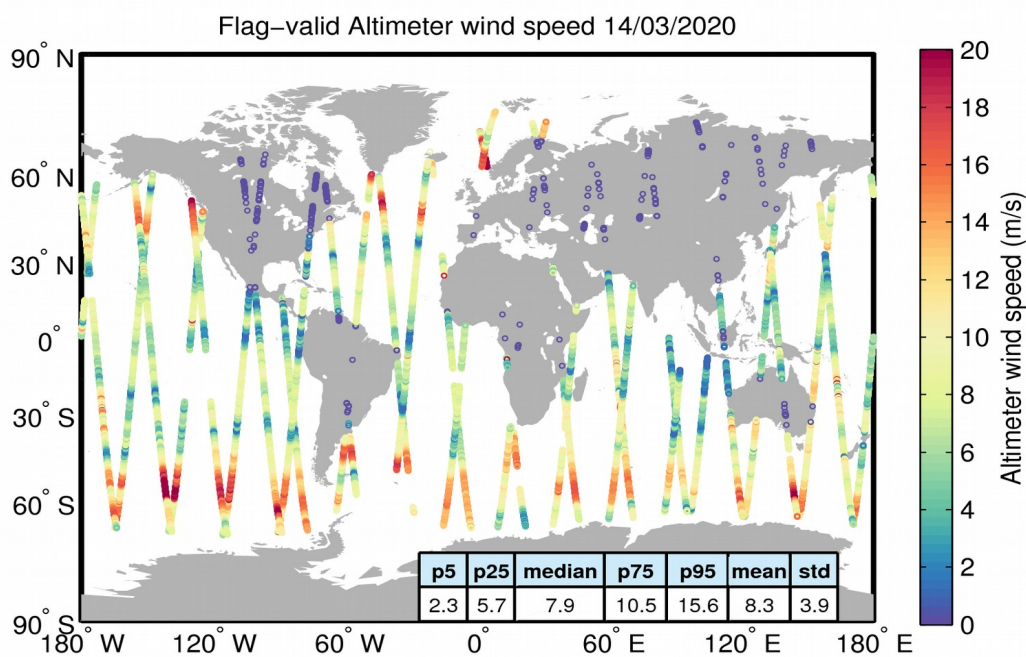
Figure 31. Geographical distribution of flag-valid wind data over oceans and lakes for 14/03/2020. The statistical values shown in the table refer to the wind in m/s and are calculated over all measurements shown in the figure.
