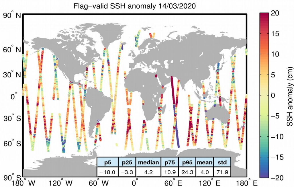
Figure 5. Geographical distribution of flag-valid 1-Hz SSH anomaly data over oceans and lakes for 14/03/2020. The statistical values shown in the table refer to the SSH anomaly in cm and are calculated over all measurements shown in the figure.
