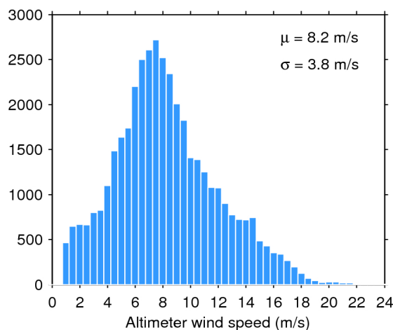
Figure 33. Histogram of flag-valid wind over oceans and lakes for 13/03/2020. The mean ( \mu ) and standard deviation ( \sigma ) are also shown. Note that values larger than 24 m/s are excluded from the histogram for the sake of readability but not from the computation of \mu and \sigma .
