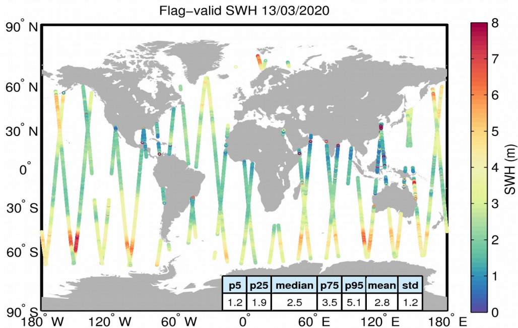
Figure 15. Geographical distribution of flag-valid SWH data over oceans and lakes for 13/03/2020. The statistical values shown in the table refer to the SWH in m and are calculated over all measurements shown in the figure.
