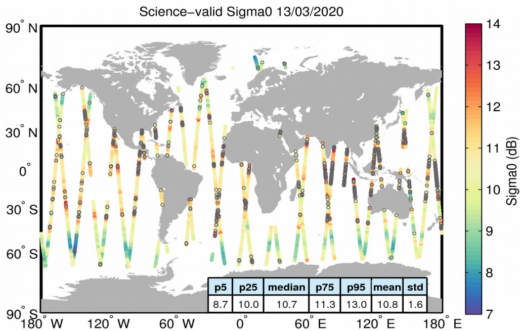
Figure 27. Geographical distribution of science-valid sigma0 data over oceans and lakes for 13/03/2020. The statistical values shown in the table refer to the sigma0 in dB and are calculated over all measurements shown in the figure. Gray circles denote records that have been rejected based on the editing criteria described in Table 4.
