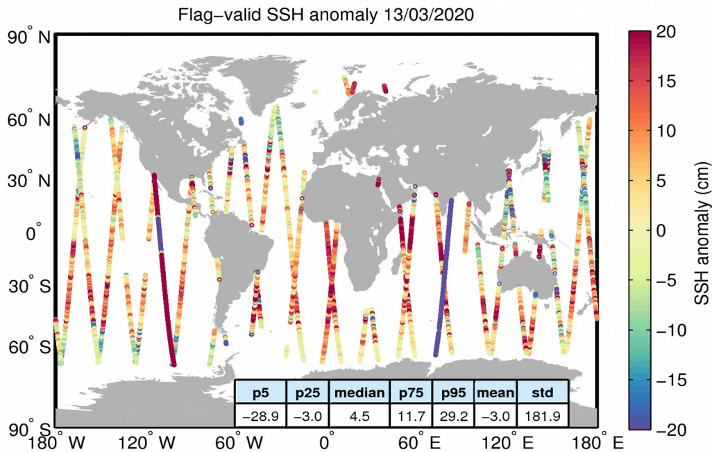
Figure 5. Geographical distribution of flag-valid 1-Hz SSH anomaly data over oceans and lakes for 13/03/2020. The statistical values shown in the table refer to the SSH anomaly in cm and are calculated over all measurements shown in the figure.
