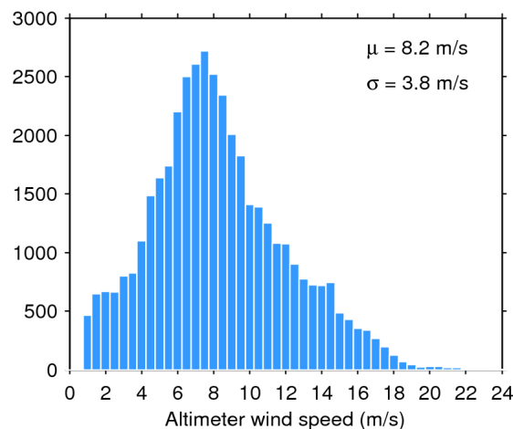
Figure 35. Histogram of science-valid wind over oceans and lakes for 13/03/2020. The mean ( \mu ) and standard deviation ( \sigma ) are also shown. Note that values larger than 24 m/s are excluded from the histogram for the sake of readability but not from the computation of \mu and \sigma .
