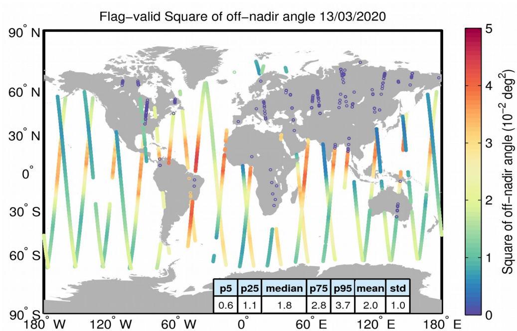
Figure 37. Geographical distribution of flag-valid mispointing data over oceans and lakes for 13/03/2020. The statistical values shown in the table refer to the mispointing in 10^{-2} \text{deg}^2 and are calculated over all measurements shown in the figure.
