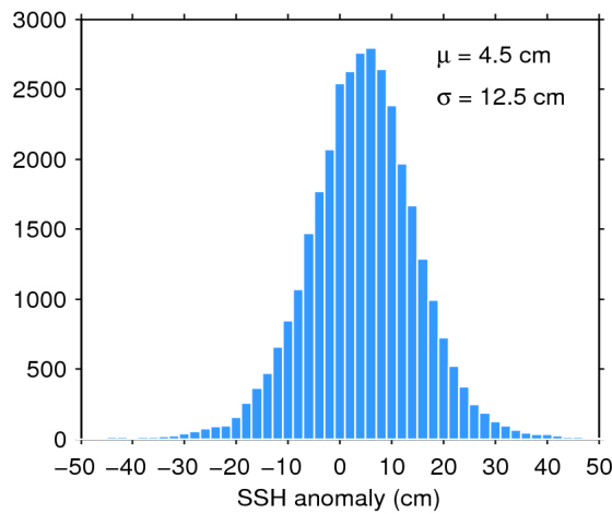
Figure 11. Histogram of science-valid SSH anomaly over oceans and lakes for 13/03/2020. The mean ( \mu ) and standard deviation ( \sigma ) are also shown. Note that values outside [-50 50] cm are excluded from the histogram for the sake of readability but not from the computation of \mu and \sigma .
