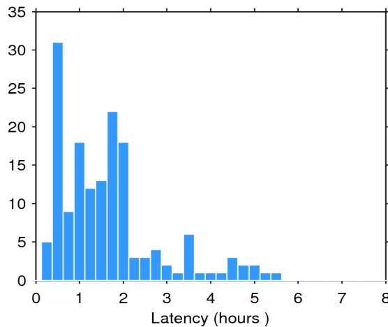
Figure 2. Histogram of the data latency for 13/03/2020. The y-axis denotes the number of files that are made available with a delay of x-hours with respect to the mean time of the records stored in the file.
