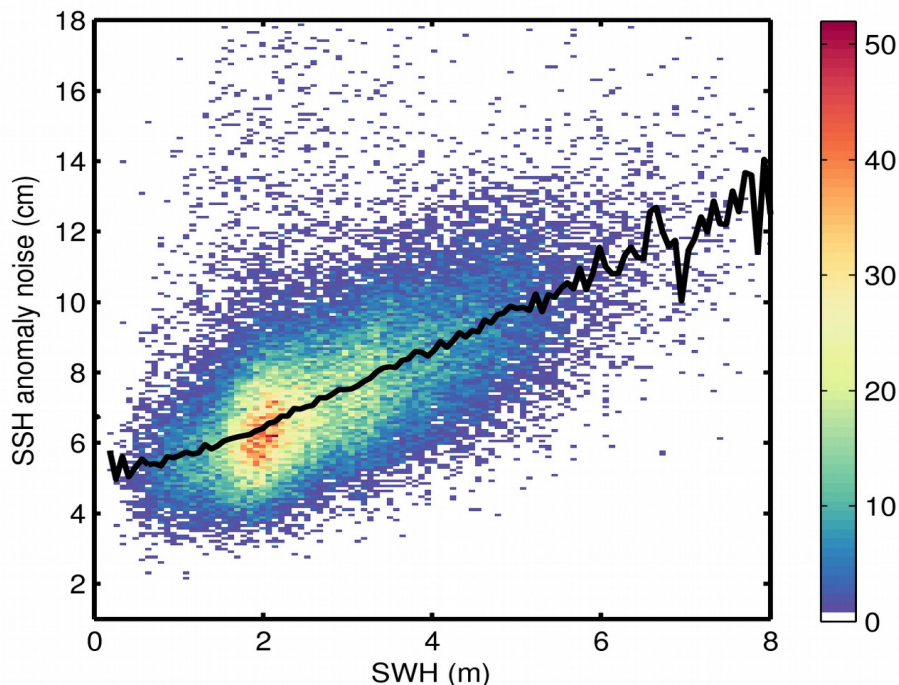
Figure 9. 2D histogram showing flag-valid SSH anomaly noise as a function of SWH for 13/03/2020. The black line denotes the median SSH anomaly noise as a function of SWH.
