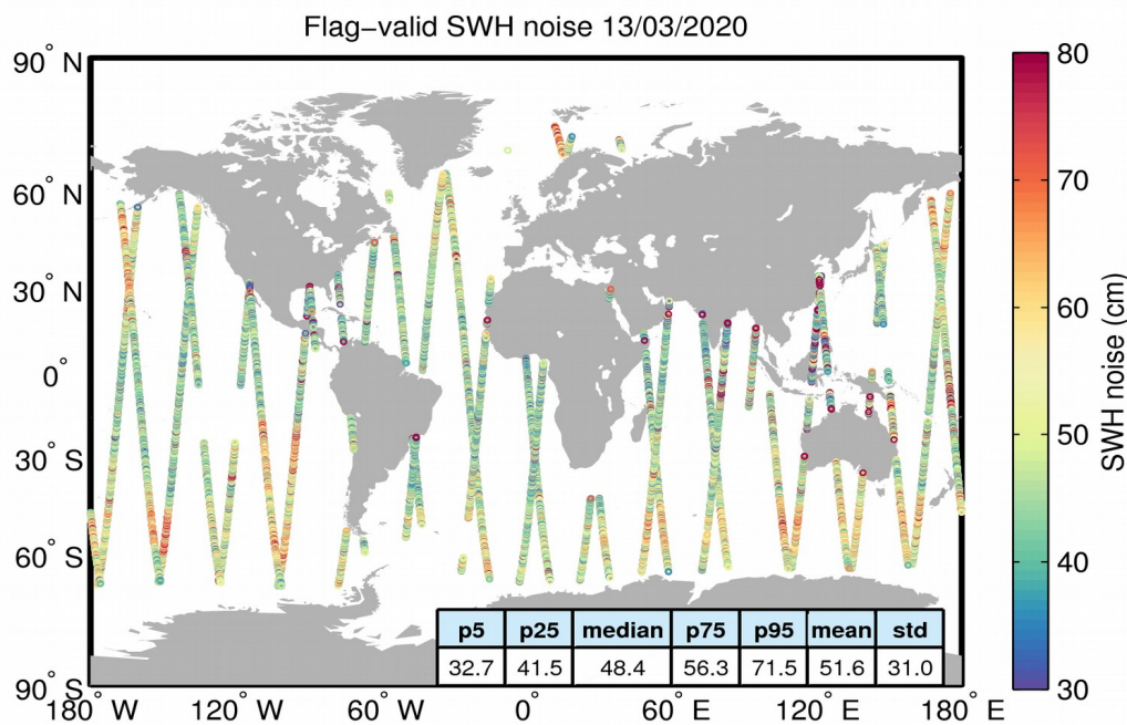
Figure 18. Geographical distribution of flag-valid 20-Hz SWH measurement noise over oceans and lakes for 13/03/2020. The statistical values shown in the table refer to the SWH noise and are calculated over all measurements shown in the figure.
