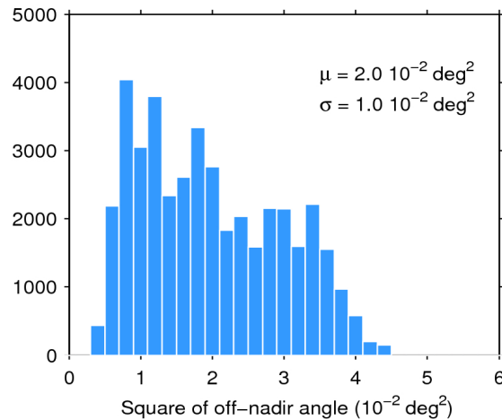
Figure 39. Histogram of flag-valid mispointing over oceans and lakes for 13/03/2020. The mean ( \mu ) and standard deviation ( \sigma ) are also shown. Note that values larger than 6 \cdot 10^{-2} \text{ deg}^2 are excluded from the histogram for the sake of readability but not from the computation of \mu and \sigma .
