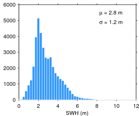
Figure 17. Histogram of flag-valid SWH over oceans and lakes for 13/03/2020. The mean ( \mu ) and standard deviation ( \sigma ) are also shown. Note that values larger than 12 m are excluded from the histogram for the sake of readability but not from the computation of \mu and \sigma .
