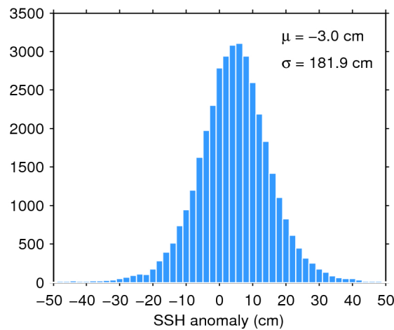
Figure 7. Histogram of flag-valid SSH anomaly over oceans and lakes for 13/03/2020. The mean ( \mu ) and standard deviation ( \sigma ) are also shown. Note that values outside [-50 50] cm are excluded from the histogram for the sake of readability but not from the computation of \mu and \sigma .
