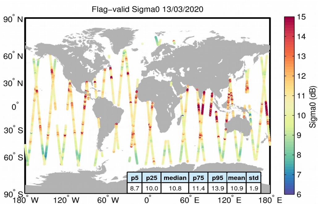
Figure 23. Geographical distribution of flag-valid sigma0 data over oceans and lakes for 13/03/2020. The statistical values shown in the table refer to the sigma0 in dB and are calculated over all measurements shown in the figure.
