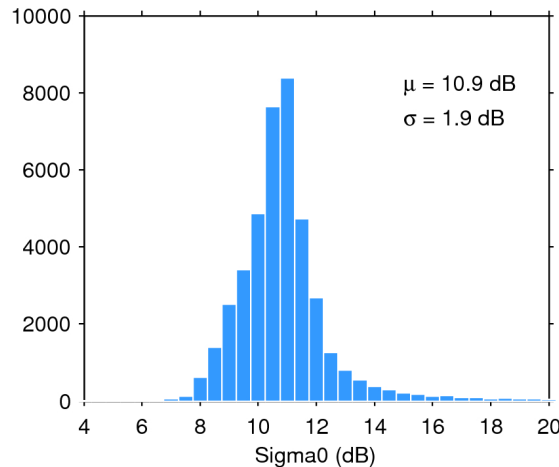
Figure 25. Histogram of flag-valid sigma0 over oceans and lakes for 13/03/2020. The mean ( \mu ) and standard deviation ( \sigma ) are also shown. Note that values outside [4 20] dB are excluded from the histogram for the sake of readability but not from the computation of \mu and \sigma .
