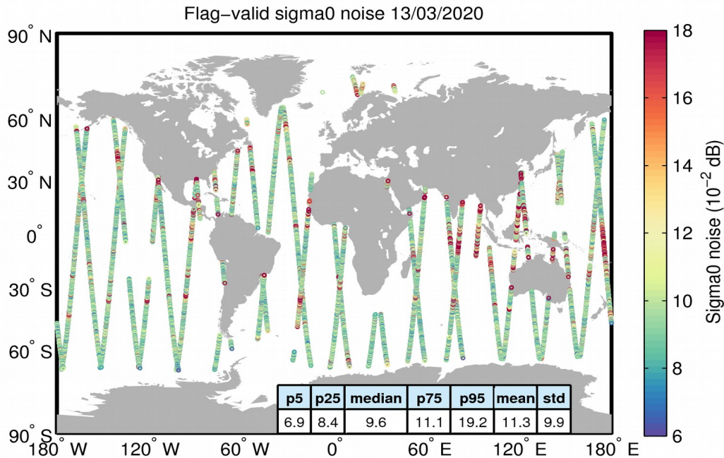
Figure 26. Geographical distribution of flag-valid 20-Hz sigma0 measurement noise over oceans and lakes for 13/03/2020. The statistical values shown in the table refer to the sigma0 noise and are calculated over all measurements shown in the figure.
