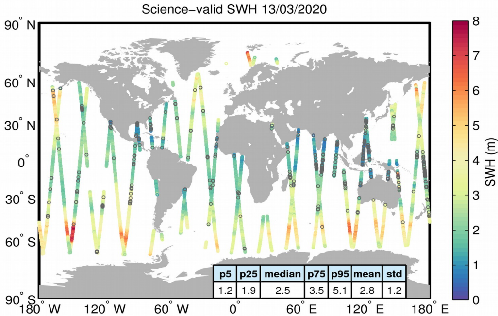
Figure 19. Geographical distribution of science-valid SWH data over oceans and lakes for 13/03/2020. The statistical values shown in the table refer to the SWH in m and are calculated over all measurements shown in the figure. Gray circles denote records that have been rejected based on the editing criteria described in Table 3.
