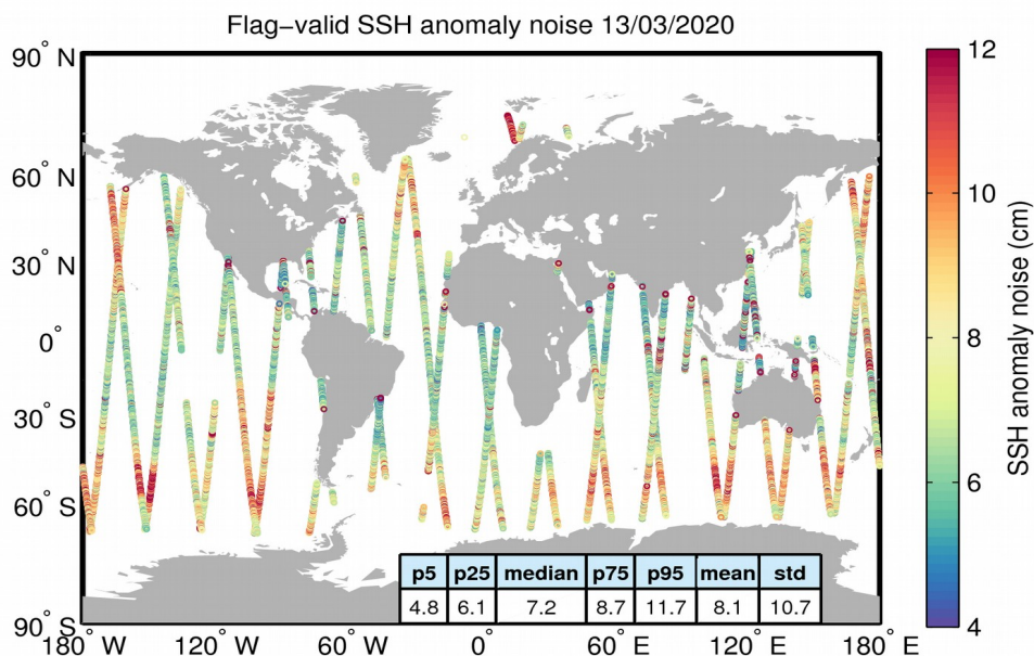
Figure 8. Geographical distribution of flag-valid 20-Hz SSH anomaly measurement noise over oceans and lakes for 13/03/2020. The statistical values shown in the table refer to the SSH anomaly noise and are calculated over all measurements shown in the figure.
