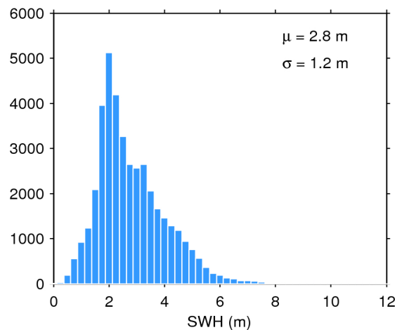
Figure 20. Histogram of science-valid SWH over oceans and lakes for 13/03/2020. The mean ( \mu ) and standard deviation ( \sigma ) are also shown. Note that values larger than 12 m are excluded from the histogram for the sake of readability but not from the computation of \mu and \sigma .
