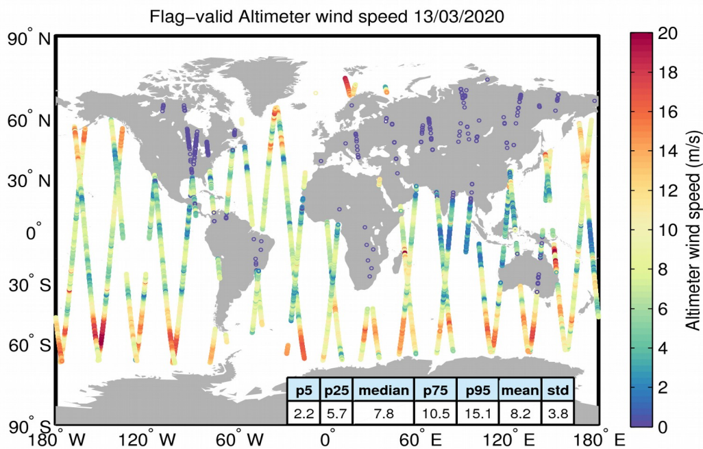
Figure 31. Geographical distribution of flag-valid wind data over oceans and lakes for 13/03/2020. The statistical values shown in the figure refer to the wind in m/s and are calculated over all measurements shown in the figure.
