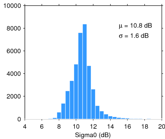
Figure 28. Histogram of science-valid sigma0 over oceans and lakes for 13/03/2020. The mean ( \mu ) and standard deviation ( \sigma ) are also shown. Note that values outside [4 20] dB are excluded from the histogram for the sake of readability but not from the computation of \mu and \sigma .
