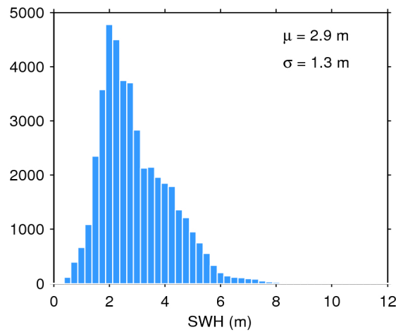
Figure 17. Histogram of flag-valid SWH over oceans and lakes for 12/03/2020. The mean ( \mu ) and standard deviation ( \sigma ) are also shown. Note that values larger than 12 m are excluded from the histogram for the sake of readability but not from the computation of \mu and \sigma .
