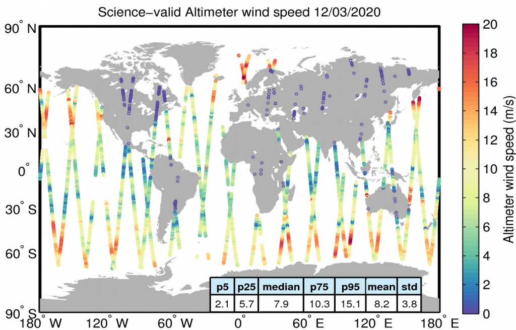
Figure 34. Geographical distribution of science-valid wind data over oceans and lakes for 12/03/2020. The statistical values shown in the table refer to the wind in m/s and are calculated over all measurements shown in the figure. Gray circles denote records that have been rejected based on the editing criteria described in Table 5.
