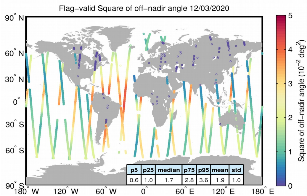
Figure 37. Geographical distribution of flag-valid mispointing data over oceans and lakes for 12/03/2020. The statistical values shown in the table refer to the mispointing in 10^{-2} \text{ deg}^2 and are calculated over all measurements shown in the figure.
