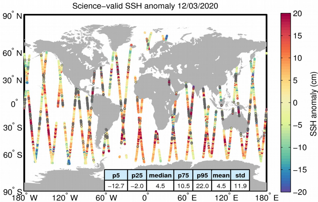
Figure 10. Geographical distribution of science-valid SSH anomaly data over oceans and lakes for 12/03/2020. The statistical values shown in the table refer to the SSH anomaly in cm and are calculated over all measurements shown in the figure. Gray circles denote records that have been rejected based on the editing criteria described in Table 2.
