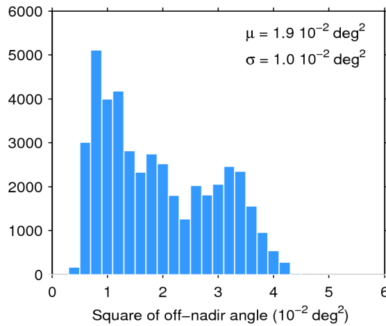
Figure 39. Histogram of flag-valid mispointing over oceans and lakes for 12/03/2020. The mean ( \mu ) and standard deviation ( \sigma ) are also shown. Note that values larger than 6 \cdot 10^{-2} \text{ deg}^2 are excluded from the histogram for the sake of readability but not from the computation of \mu and \sigma .
