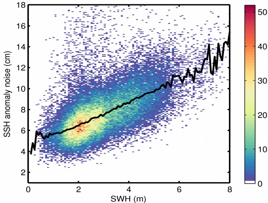
Figure 9. 2D histogram showing flag-valid SSH anomaly noise as a function of SWH for 12/03/2020. The black line denotes the median SSH anomaly noise as a function of SWH.
