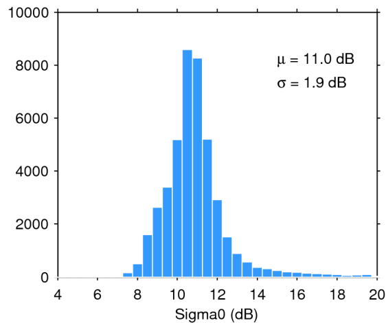
Figure 25. Histogram of flag-valid sigma0 over oceans and lakes for 12/03/2020. The mean ( \mu ) and standard deviation ( \sigma ) are also shown. Note that values outside [4 20] dB are excluded from the histogram for the sake of readability but not from the computation of \mu and \sigma .
