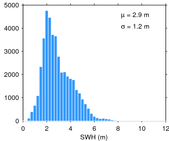
Figure 20. Histogram of science-valid SWH over oceans and lakes for 12/03/2020. The mean ( \mu ) and standard deviation ( \sigma ) are also shown. Note that values larger than 12 m are excluded from the histogram for the sake of readability but not from the computation of \mu and \sigma .
