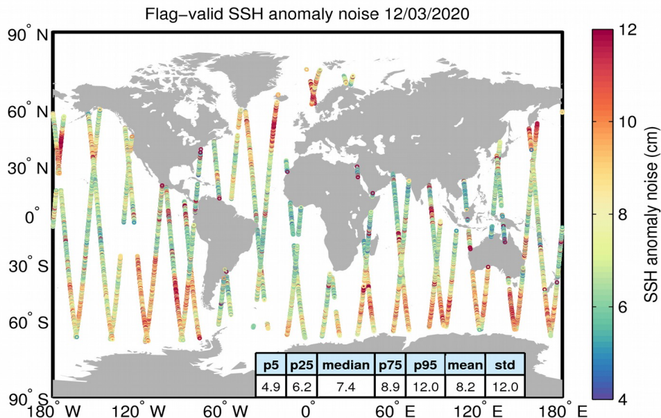
Figure 8. Geographical distribution of flag-valid 20-Hz SSH anomaly measurement noise over oceans and lakes for 12/03/2020. The statistical values shown in the table refer to the SSH anomaly noise and are calculated over all measurements shown in the figure.
