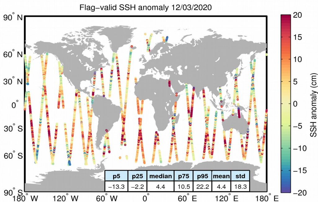
Figure 5. Geographical distribution of flag-valid 1-Hz SSH anomaly data over oceans and lakes for 12/03/2020. The statistical values shown in the table refer to the SSH anomaly in cm and are calculated over all measurements shown in the figure.
