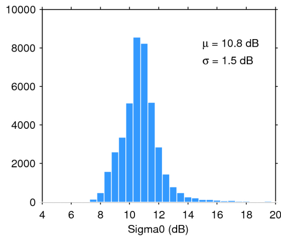
Figure 28. Histogram of science-valid sigma0 over oceans and lakes for 12/03/2020. The mean ( \mu ) and standard deviation ( \sigma ) are also shown. Note that values outside [4 20] dB are excluded from the histogram for the sake of readability but not from the computation of \mu and \sigma .
