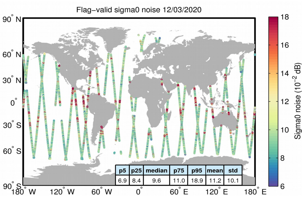
Figure 26. Geographical distribution of flag-valid 20-Hz sigma0 measurement noise over oceans and lakes for 12/03/2020. The statistical values shown in the table refer to the sigma0 noise and are calculated over all measurements shown in the figure.
