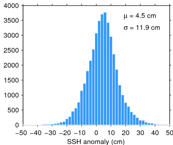
Figure 11. Histogram of science-valid SSH anomaly over oceans and lakes for 12/03/2020. The mean ( \mu ) and standard deviation ( \sigma ) are also shown. Note that values outside [-50 50] cm are excluded from the histogram for the sake of readability but not from the computation of \mu and \sigma .
