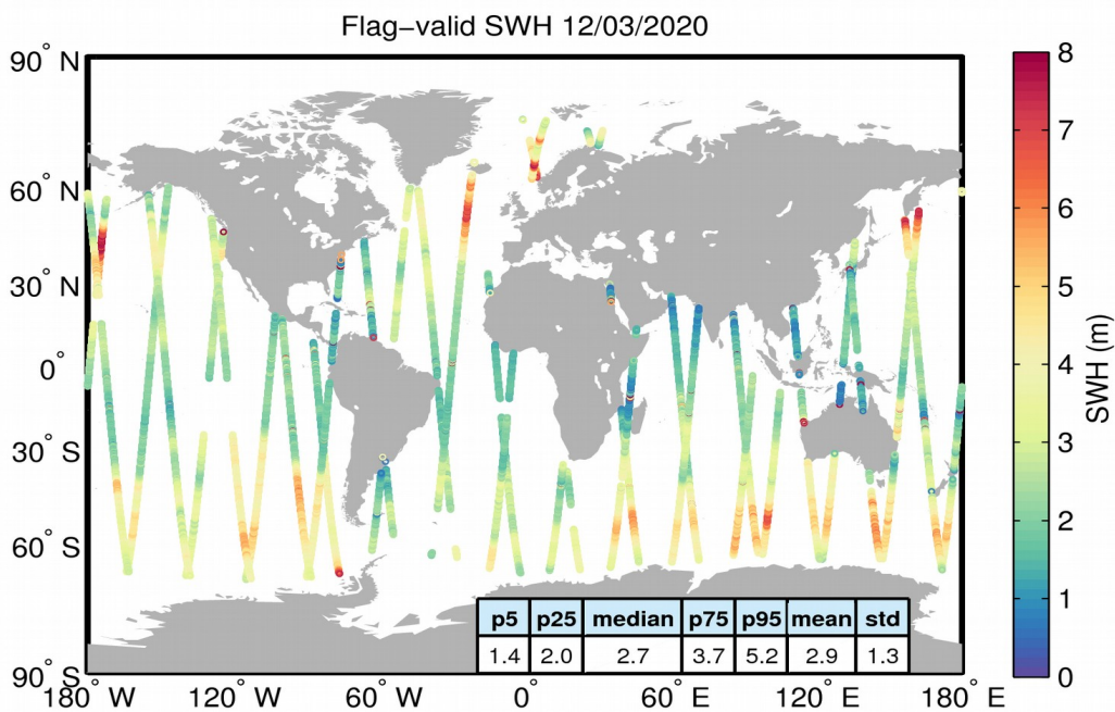
Figure 15. Geographical distribution of flag-valid SWH data over oceans and lakes for 12/03/2020. The statistical values shown in the table refer to the SWH in m and are calculated over all measurements shown in the figure.
