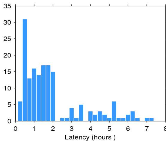
Figure 2. Histogram of the data latency for 12/03/2020. The y-axis denotes the number of files that are made available with a delay of x-hours with respect to the mean time of the records stored in the file.
