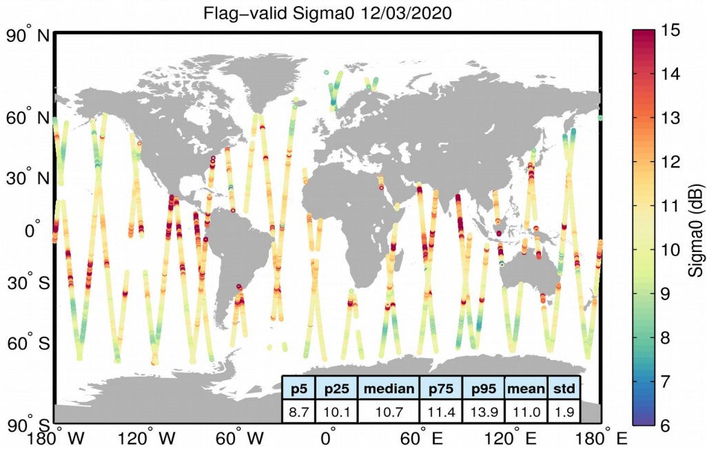
Figure 23. Geographical distribution of flag-valid sigma0 data over oceans and lakes for 12/03/2020. The statistical values shown in the table refer to the sigma0 in dB and are calculated over all measurements shown in the figure.
