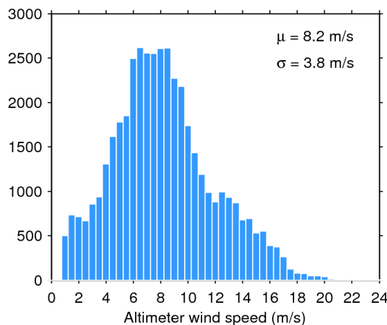
Figure 35. Histogram of science-valid wind over oceans and lakes for 12/03/2020. The mean ( \mu ) and standard deviation ( \sigma ) are also shown. Note that values larger than 24 m/s are excluded from the histogram for the sake of readability but not from the computation of \mu and \sigma .
