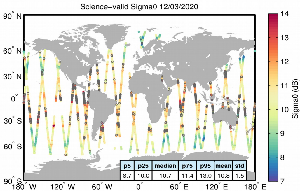
Figure 27. Geographical distribution of science-valid sigma0 data over oceans and lakes for 12/03/2020. The statistical values shown in the table refer to the sigma0 in dB and are calculated over all measurements shown in the figure. Gray circles denote records that have been rejected based on the editing criteria described in Table 4.
