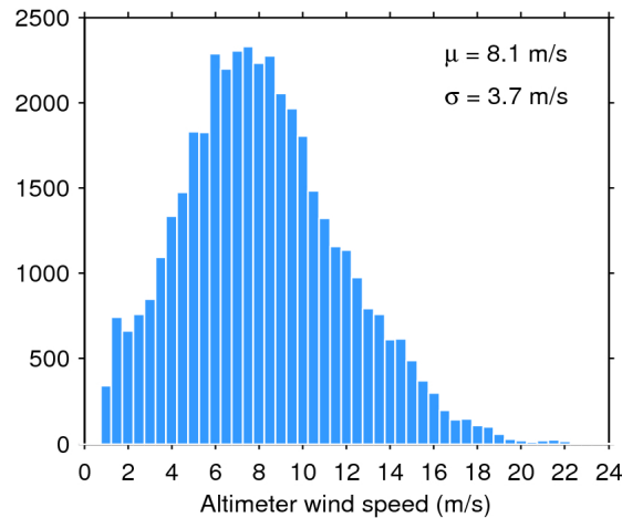
Figure 33. Histogram of flag-valid wind over oceans and lakes for 11/03/2020. The mean ( \mu ) and standard deviation ( \sigma ) are also shown. Note that values larger than 24 m/s are excluded from the histogram for the sake of readability but not from the computation of \mu and \sigma .
