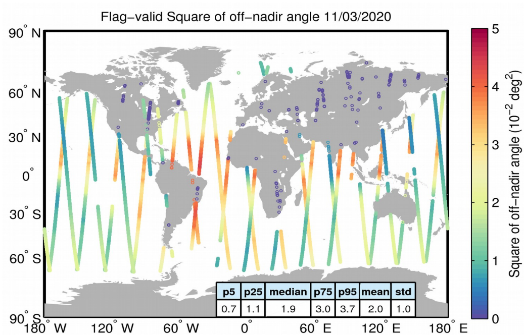
Figure 37. Geographical distribution of flag-valid mispointing data over oceans and lakes for 11/03/2020. The statistical values shown in the table refer to the mispointing in 10^{-2} \text{ deg}^2 and are calculated over all measurements shown in the figure.
