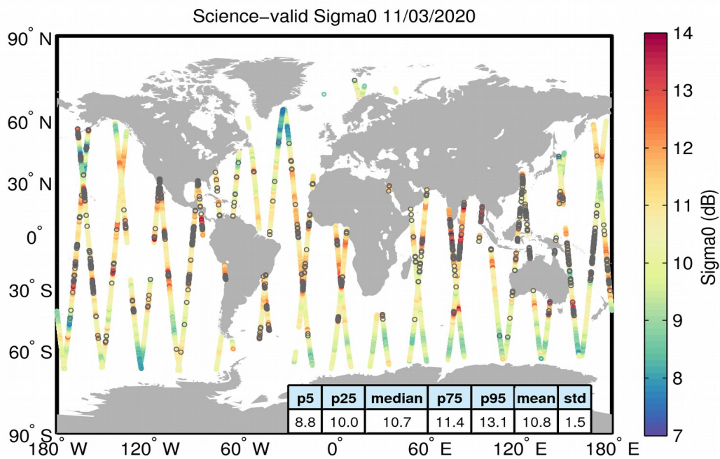
Figure 27. Geographical distribution of science-valid sigma0 data over oceans and lakes for 11/03/2020. The statistical values shown in the table refer to the sigma0 in dB and are calculated over all measurements shown in the figure. Gray circles denote records that have been rejected based on the editing criteria described in Table 4.
