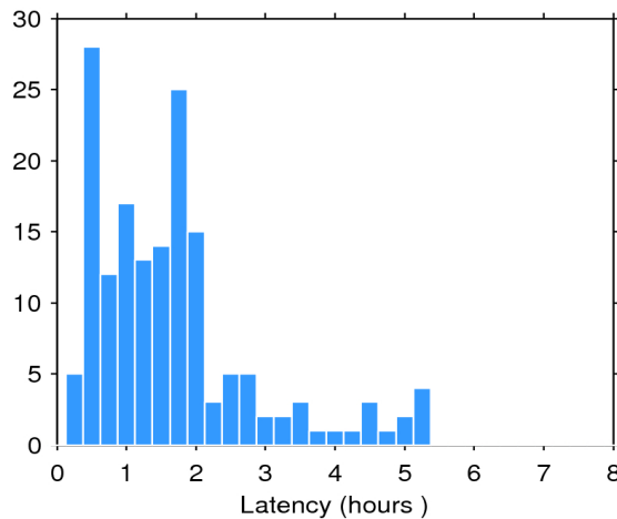
Figure 2. Histogram of the data latency for 11/03/2020. The y-axis denotes the number of files that are made available with a delay of x-hours with respect to the mean time of the records stored in the file.
