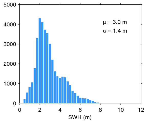
Figure 17. Histogram of flag-valid SWH over oceans and lakes for 11/03/2020. The mean ( \mu ) and standard deviation ( \sigma ) are also shown. Note that values larger than 12 m are excluded from the histogram for the sake of readability but not from the computation of \mu and \sigma .
