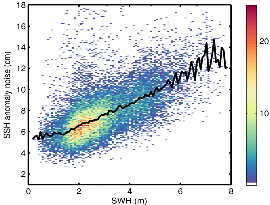
Figure 9. 2D histogram showing flag-valid SSH anomaly noise as a function of SWH for 11/03/2020. The black line denotes the median SSH anomaly noise as a function of SWH.
