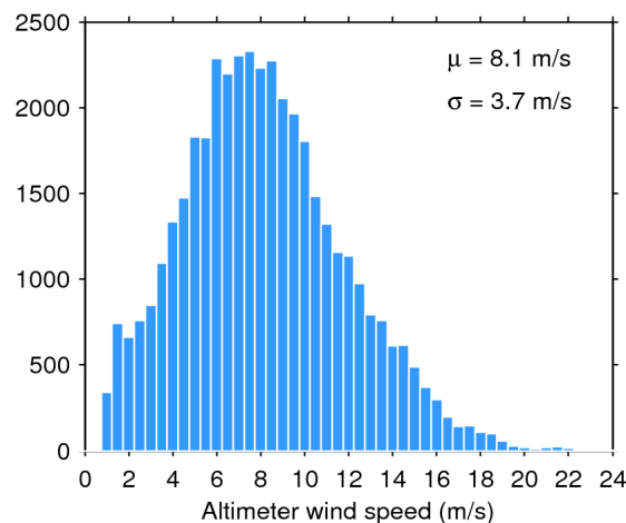
Figure 35. Histogram of science-valid wind over oceans and lakes for 11/03/2020. The mean ( \mu ) and standard deviation ( \sigma ) are also shown. Note that values larger than 24 m/s are excluded from the histogram for the sake of readability but not from the computation of \mu and \sigma .
