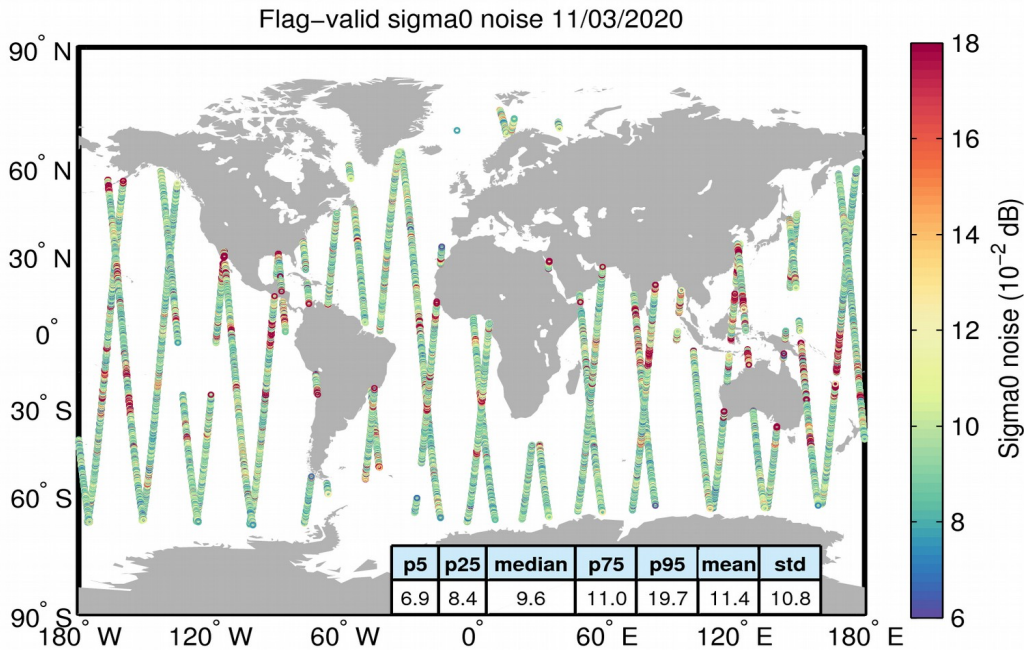
Figure 26. Geographical distribution of flag-valid 20-Hz sigma0 measurement noise over oceans and lakes for 11/03/2020. The statistical values shown in the table refer to the sigma0 noise and are calculated over all measurements shown in the figure.
