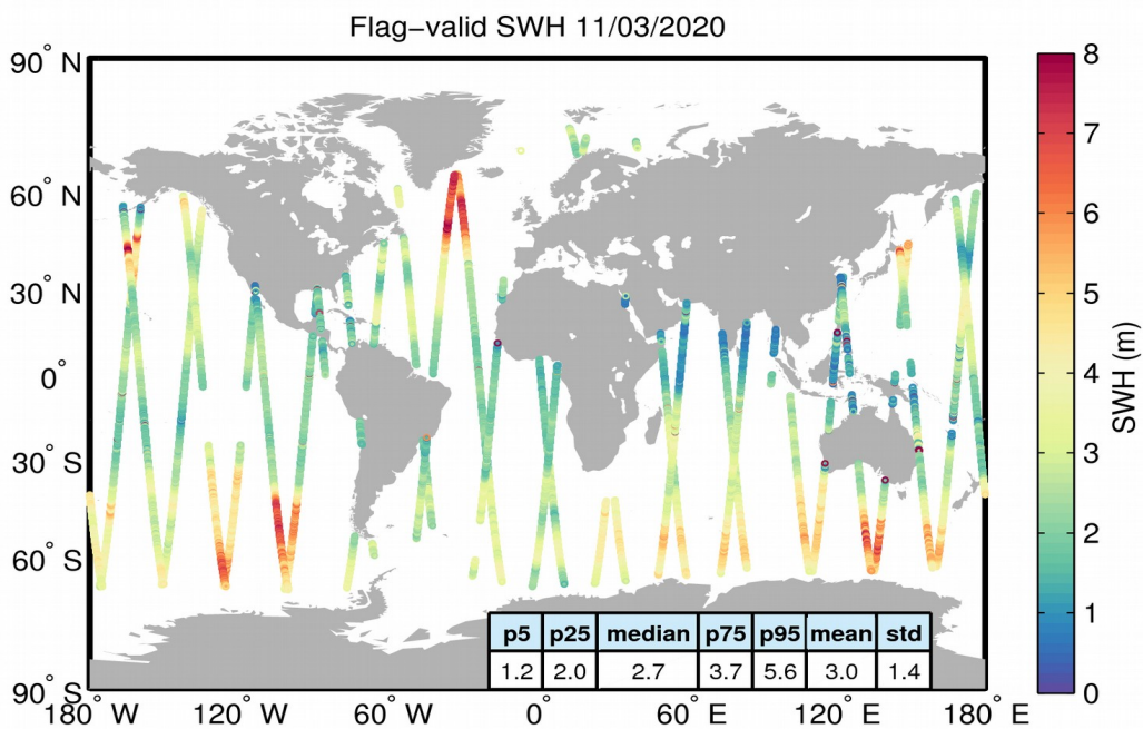
Figure 15. Geographical distribution of flag-valid SWH data over oceans and lakes for 11/03/2020. The statistical values shown in the table refer to the SWH in m and are calculated over all measurements shown in the figure.
