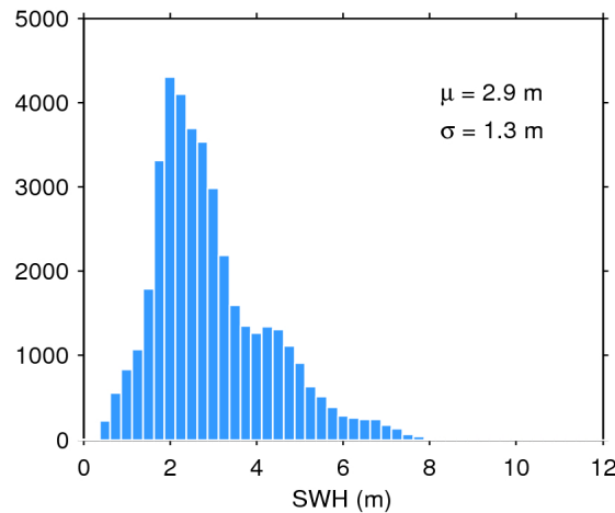
Figure 20. Histogram of science-valid SWH over oceans and lakes for 11/03/2020. The mean ( \mu ) and standard deviation ( \sigma ) are also shown. Note that values larger than 12 m are excluded from the histogram for the sake of readability but not from the computation of \mu and \sigma .
