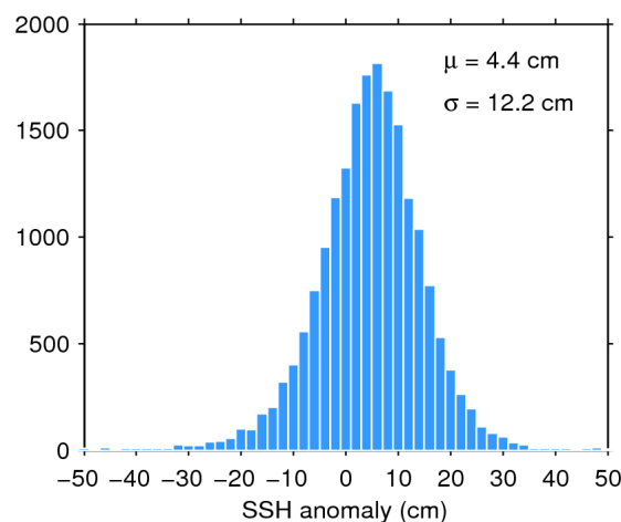
Figure 11. Histogram of science-valid SSH anomaly over oceans and lakes for 11/03/2020. The mean ( \mu ) and standard deviation ( \sigma ) are also shown. Note that values outside [-50 50] cm are excluded from the histogram for the sake of readability but not from the computation of \mu and \sigma .
