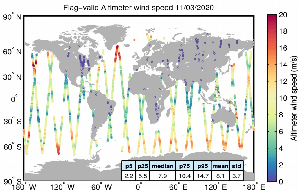
Figure 31. Geographical distribution of flag-valid wind data over oceans and lakes for 11/03/2020. The statistical values shown in the table refer to the wind in m/s and are calculated over all measurements shown in the figure.
