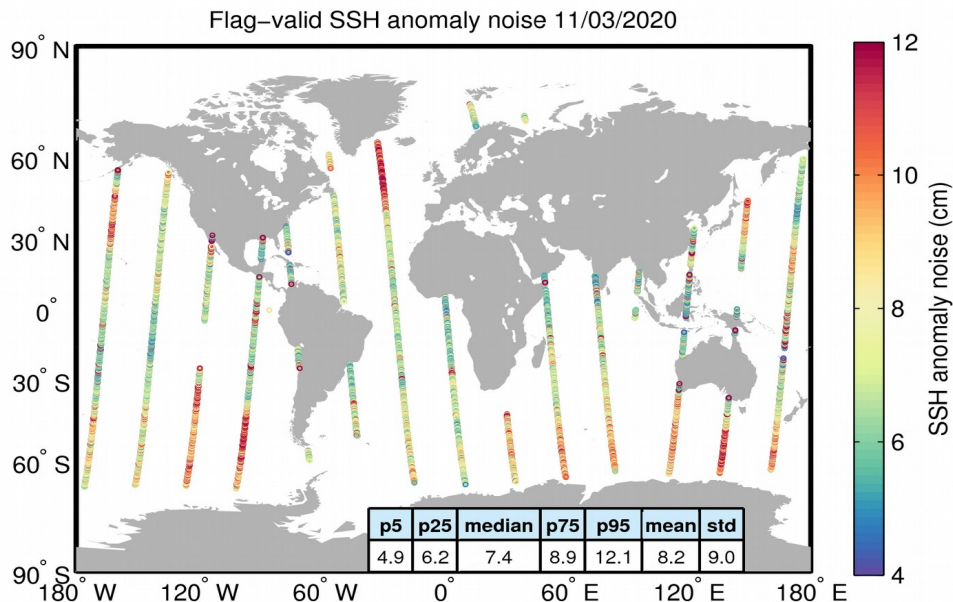
Figure 8. Geographical distribution of flag-valid 20-Hz SSH anomaly measurement noise over oceans and lakes for 11/03/2020. The statistical values shown in the table refer to the SSH anomaly noise and are calculated over all measurements shown in the figure.
