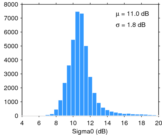
Figure 25. Histogram of flag-valid sigma0 over oceans and lakes for 11/03/2020. The mean ( \mu ) and standard deviation ( \sigma ) are also shown. Note that values outside [4 20] dB are excluded from the histogram for the sake of readability but not from the computation of \mu and \sigma .
