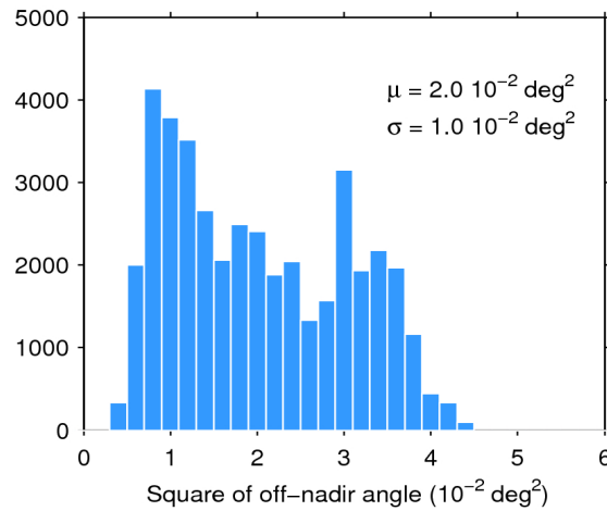
Figure 39. Histogram of flag-valid mispointing over oceans and lakes for 11/03/2020. The mean ( \mu ) and standard deviation ( \sigma ) are also shown. Note that values larger than 6 \cdot 10^{-2} \text{ deg}^2 are excluded from the histogram for the sake of readability but not from the computation of \mu and \sigma .
