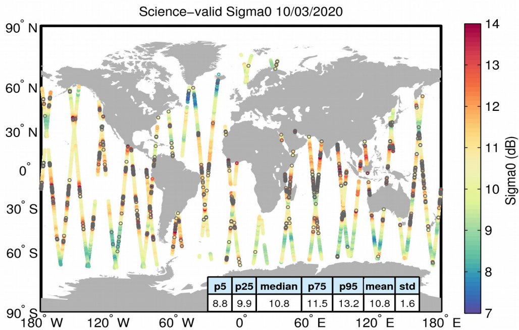
Figure 27. Geographical distribution of science-valid sigma0 data over oceans and lakes for 10/03/2020. The statistical values shown in the table refer to the sigma0 in dB and are calculated over all measurements shown in the figure. Gray circles denote records that have been rejected based on the editing criteria described in Table 4.
