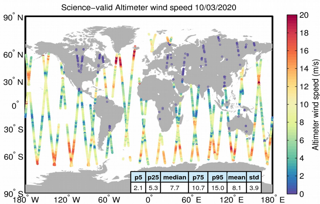
Figure 34. Geographical distribution of science-valid wind data over oceans and lakes for 10/03/2020. The statistical values shown in the table refer to the wind in m/s and are calculated over all measurements shown in the figure. Gray circles denote records that have been rejected based on the editing criteria described in Table 5.
