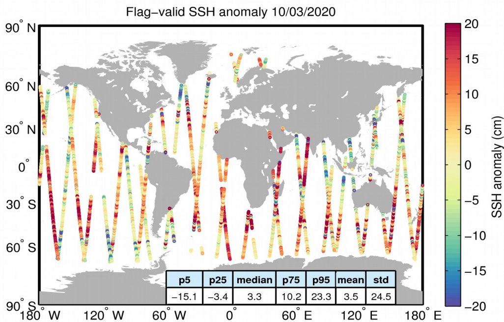
Figure 5. Geographical distribution of flag-valid 1-Hz SSH anomaly data over oceans and lakes for 10/03/2020. The statistical values shown in the table refer to the SSH anomaly in cm and are calculated over all measurements shown in the figure.
