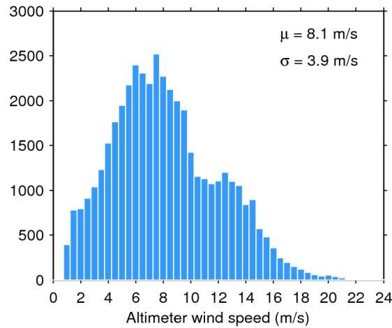
Figure 33. Histogram of flag-valid wind over oceans and lakes for 10/03/2020. The mean ( \mu ) and standard deviation ( \sigma ) are also shown. Note that values larger than 24 m/s are excluded from the histogram for the sake of readability but not from the computation of \mu and \sigma .
