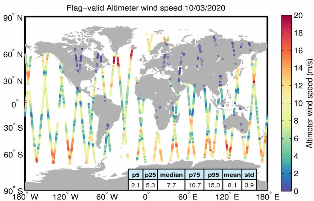
Figure 31. Geographical distribution of flag-valid wind data over oceans and lakes for 10/03/2020. The statistical values shown in the table refer to the wind in m/s and are calculated over all measurements shown in the figure.
