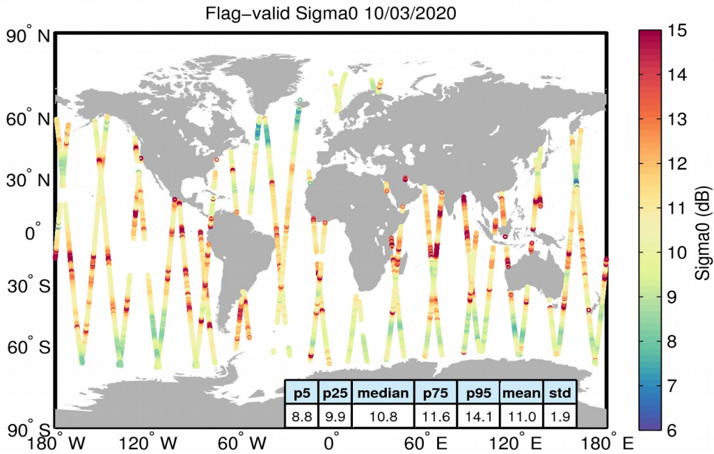
Figure 23. Geographical distribution of flag-valid sigma0 data over oceans and lakes for 10/03/2020. The statistical values shown in the table refer to the sigma0 in dB and are calculated over all measurements shown in the figure.
