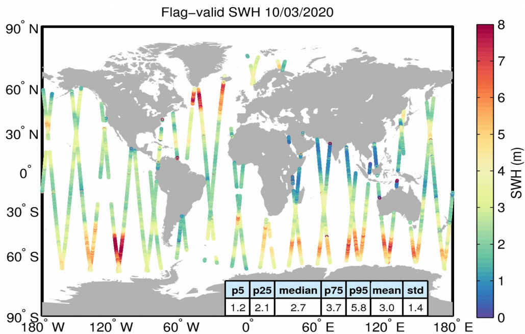
Figure 15. Geographical distribution of flag-valid SWH data over oceans and lakes for 10/03/2020. The statistical values shown in the table refer to the SWH in m and are calculated over all measurements shown in the figure.
