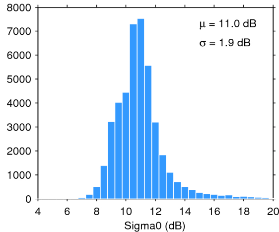
Figure 25. Histogram of flag-valid sigma0 over oceans and lakes for 10/03/2020. The mean ( \mu ) and standard deviation ( \sigma ) are also shown. Note that values outside [4 20] dB are excluded from the histogram for the sake of readability but not from the computation of \mu and \sigma .
