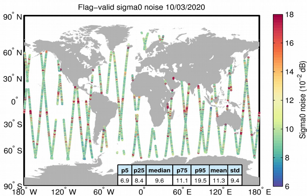
Figure 26. Geographical distribution of flag-valid 20-Hz sigma0 measurement noise over oceans and lakes for 10/03/2020. The statistical values shown in the figure refer to the sigma0 noise and are calculated over all measurements shown in the figure.
