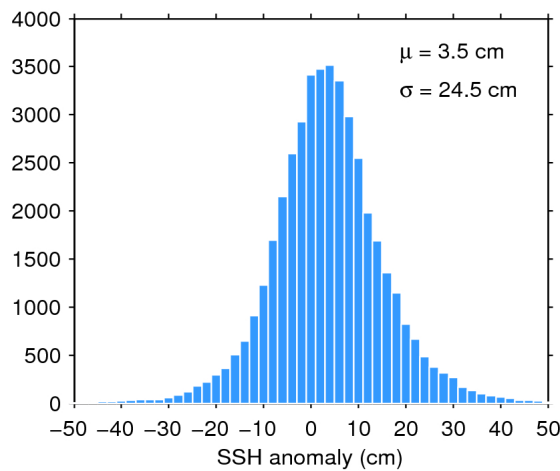
Figure 7. Histogram of flag-valid SSH anomaly over oceans and lakes for 10/03/2020. The mean ( \mu ) and standard deviation ( \sigma ) are also shown. Note that values outside [-50\ 50] cm are excluded from the histogram for the sake of readability but not from the computation of \mu and \sigma .
