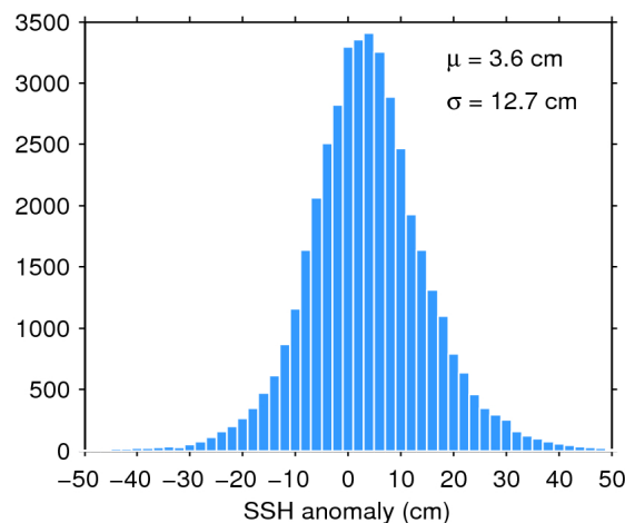
Figure 11. Histogram of science-valid SSH anomaly over oceans and lakes for 10/03/2020. The mean ( \mu ) and standard deviation ( \sigma ) are also shown. Note that values outside [-50 50] cm are excluded from the histogram for the sake of readability but not from the computation of \mu and \sigma .
