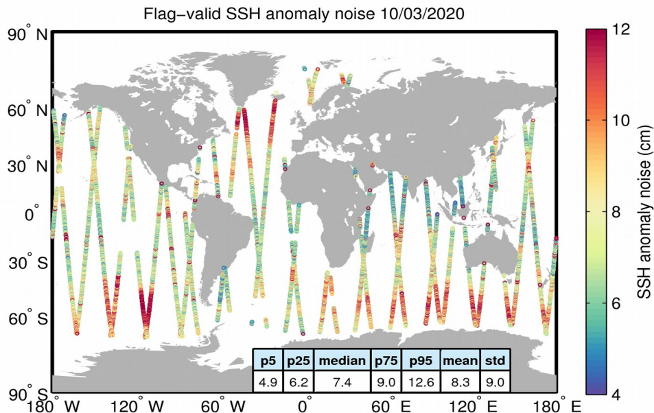
Figure 8. Geographical distribution of flag-valid 20-Hz SSH anomaly measurement noise over oceans and lakes for 10/03/2020. The statistical values shown in the table refer to the SSH anomaly noise and are calculated over all measurements shown in the figure.
