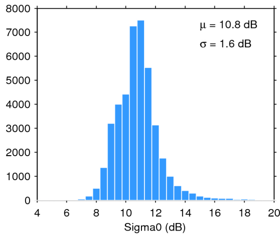
Figure 28. Histogram of science-valid sigma0 over oceans and lakes for 10/03/2020. The mean ( \mu ) and standard deviation ( \sigma ) are also shown. Note that values outside [4 20] dB are excluded from the histogram for the sake of readability but not from the computation of \mu and \sigma .
