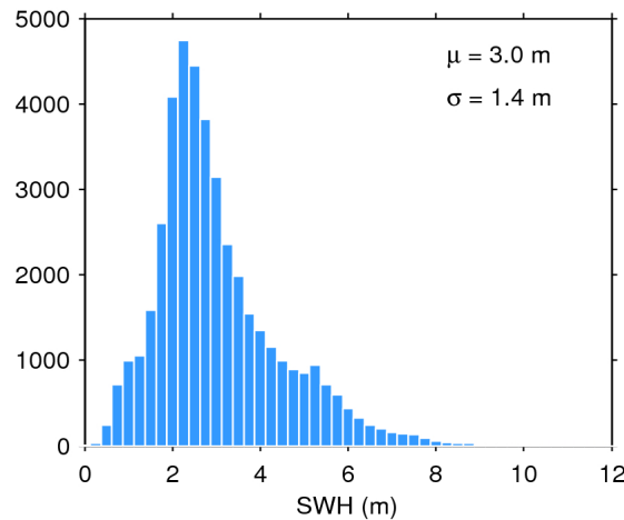
Figure 20. Histogram of science-valid SWH over oceans and lakes for 10/03/2020. The mean ( \mu ) and standard deviation ( \sigma ) are also shown. Note that values larger than 12 m are excluded from the histogram for the sake of readability but not from the computation of \mu and \sigma .
