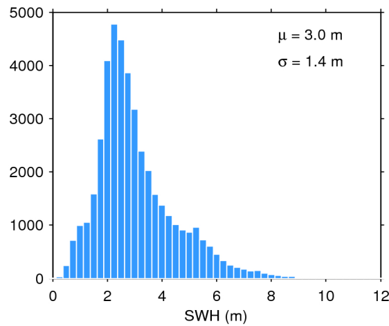
Figure 17. Histogram of flag-valid SWH over oceans and lakes for 10/03/2020. The mean ( \mu ) and standard deviation ( \sigma ) are also shown. Note that values larger than 12 m are excluded from the histogram for the sake of readability but not from the computation of \mu and \sigma .
