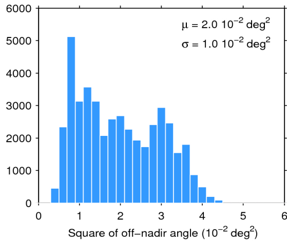
Figure 39. Histogram of flag-valid mispointing over oceans and lakes for 10/03/2020. The mean ( \mu ) and standard deviation ( \sigma ) are also shown. Note that values larger than 6 \cdot 10^{-2} \text{ deg}^2 are excluded from the histogram for the sake of readability but not from the computation of \mu and \sigma .
