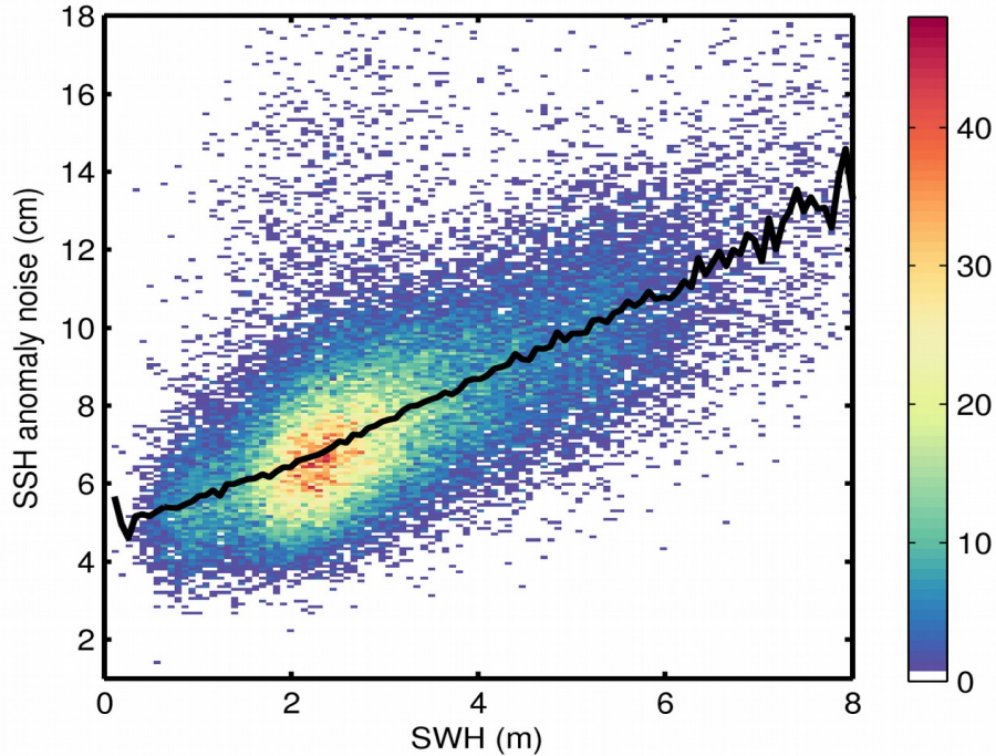
Figure 9. 2D histogram showing flag-valid SSH anomaly noise as a function of SWH for 10/03/2020. The black line denotes the median SSH anomaly noise as a function of SWH.
