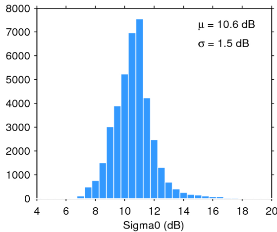
Figure 28. Histogram of science-valid sigma0 over oceans and lakes for 09/03/2020. The mean ( \mu ) and standard deviation ( \sigma ) are also shown. Note that values outside [4 20] dB are excluded from the histogram for the sake of readability but not from the computation of \mu and \sigma .
