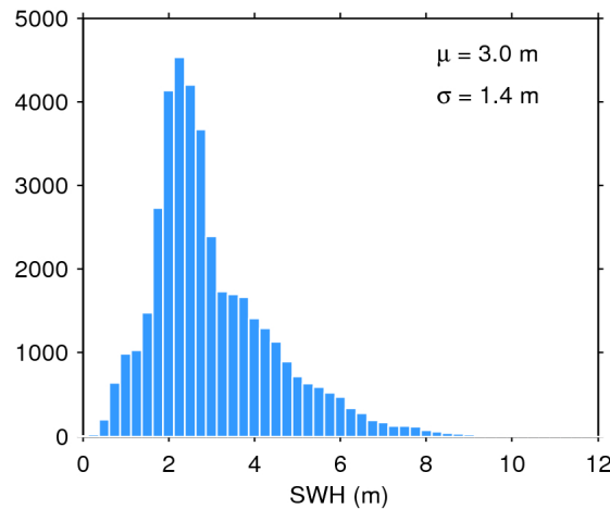
Figure 20. Histogram of science-valid SWH over oceans and lakes for 09/03/2020. The mean ( \mu ) and standard deviation ( \sigma ) are also shown. Note that values larger than 12 m are excluded from the histogram for the sake of readability but not from the computation of \mu and \sigma .
