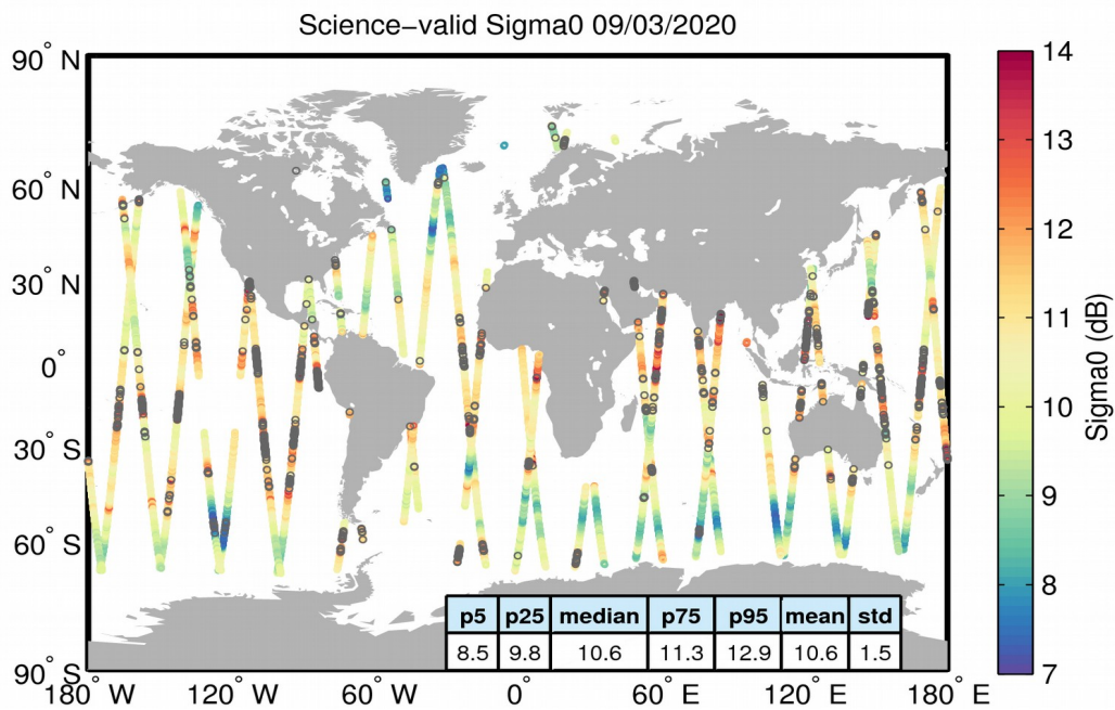
Figure 27. Geographical distribution of science-valid sigma0 data over oceans and lakes for 09/03/2020. The statistical values shown in the table refer to the sigma0 in dB and are calculated over all measurements shown in the figure. Gray circles denote records that have been rejected based on the editing criteria described in Table 4.
