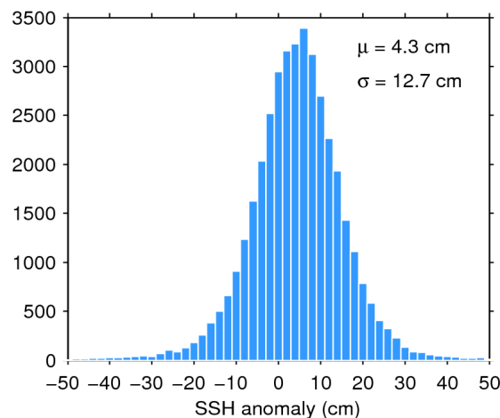
Figure 11. Histogram of science-valid SSH anomaly over oceans and lakes for 09/03/2020. The mean ( \mu ) and standard deviation ( \sigma ) are also shown. Note that values outside [-50 50] cm are excluded from the histogram for the sake of readability but not from the computation of \mu and \sigma .
