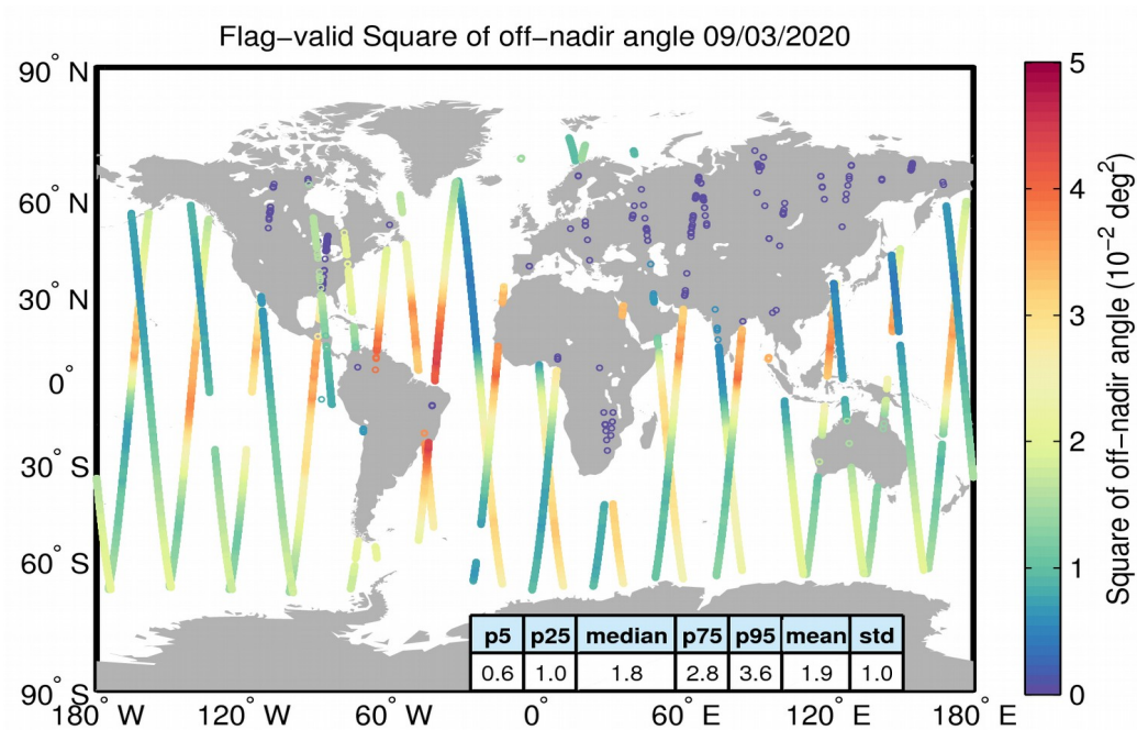
Figure 37. Geographical distribution of flag-valid mispointing data over oceans and lakes for 09/03/2020. The statistical values shown in the table refer to the mispointing in 10^{-2} \text{ deg}^2 and are calculated over all measurements shown in the figure.
