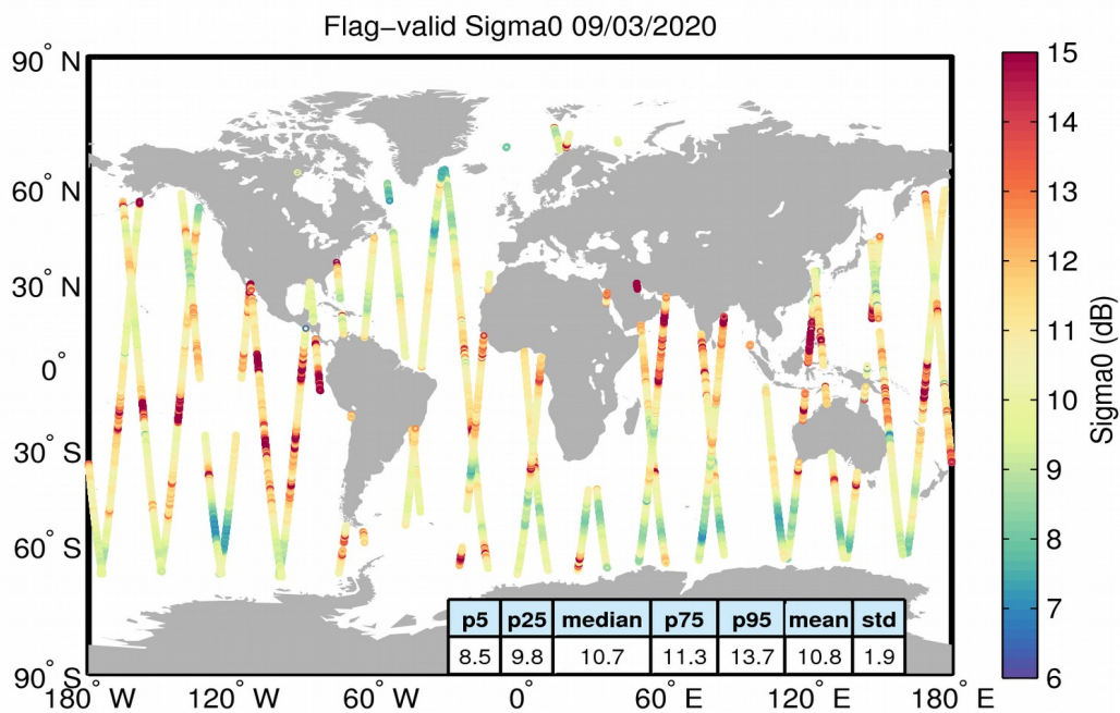
Figure 23. Geographical distribution of flag-valid sigma0 data over oceans and lakes for 09/03/2020. The statistical values shown in the table refer to the sigma0 in dB and are calculated over all measurements shown in the figure.
