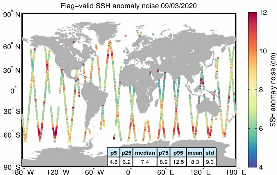
Figure 8. Geographical distribution of flag-valid 20-Hz SSH anomaly measurement noise over oceans and lakes for 09/03/2020. The statistical values shown in the table refer to the SSH anomaly noise and are calculated over all measurements shown in the figure.
