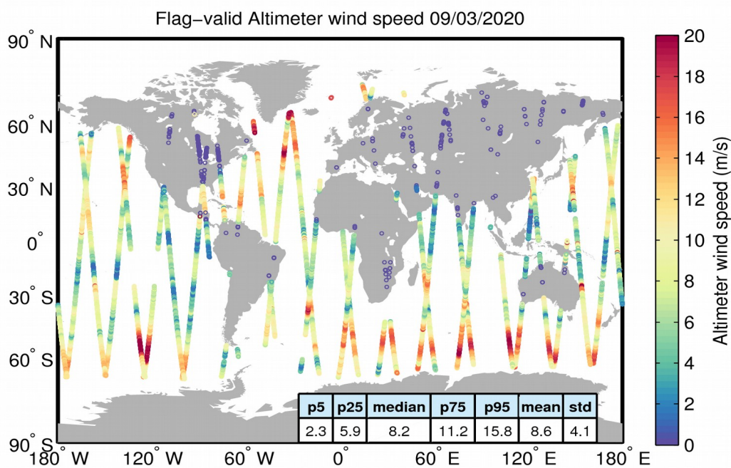
Figure 31. Geographical distribution of flag-valid wind data over oceans and lakes for 09/03/2020. The statistical values shown in the table refer to the wind in m/s and are calculated over all measurements shown in the figure.
