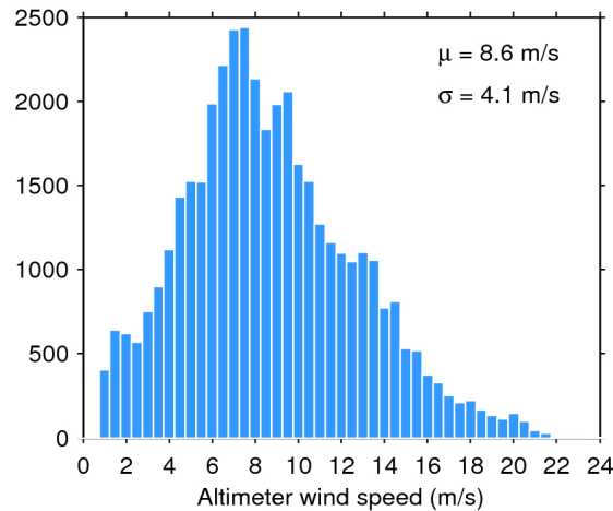
Figure 33. Histogram of flag-valid wind over oceans and lakes for 09/03/2020. The mean ( \mu ) and standard deviation ( \sigma ) are also shown. Note that values larger than 24 m/s are excluded from the histogram for the sake of readability but not from the computation of \mu and \sigma .
