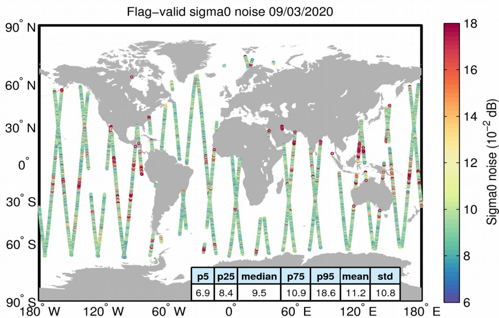
Figure 26. Geographical distribution of flag-valid 20-Hz sigma0 measurement noise over oceans and lakes for 09/03/2020. The statistical values shown in the table refer to the sigma0 noise and are calculated over all measurements shown in the figure.
