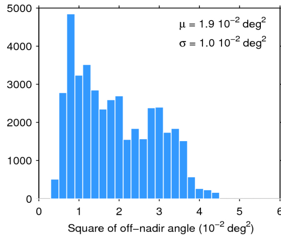
Figure 39. Histogram of flag-valid mispointing over oceans and lakes for 09/03/2020. The mean ( \mu ) and standard deviation ( \sigma ) are also shown. Note that values larger than 6 \cdot 10^{-2} \text{ deg}^2 are excluded from the histogram for the sake of readability but not from the computation of \mu and \sigma .
