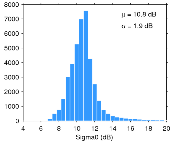
Figure 25. Histogram of flag-valid sigma0 over oceans and lakes for 09/03/2020. The mean ( \mu ) and standard deviation ( \sigma ) are also shown. Note that values outside [4 20] dB are excluded from the histogram for the sake of readability but not from the computation of \mu and \sigma .
