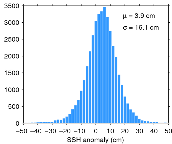
Figure 7. Histogram of flag-valid SSH anomaly over oceans and lakes for 09/03/2020. The mean ( \mu ) and standard deviation ( \sigma ) are also shown. Note that values outside [-50\ 50] cm are excluded from the histogram for the sake of readability but not from the computation of \mu and \sigma .
