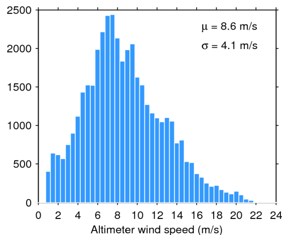
Figure 35. Histogram of science-valid wind over oceans and lakes for 09/03/2020. The mean ( \mu ) and standard deviation ( \sigma ) are also shown. Note that values larger than 24 m/s are excluded from the histogram for the sake of readability but not from the computation of \mu and \sigma .
