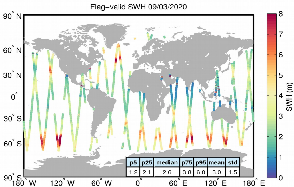
Figure 15. Geographical distribution of flag-valid SWH data over oceans and lakes for 09/03/2020. The statistical values shown in the table refer to the SWH in m and are calculated over all measurements shown in the figure.
