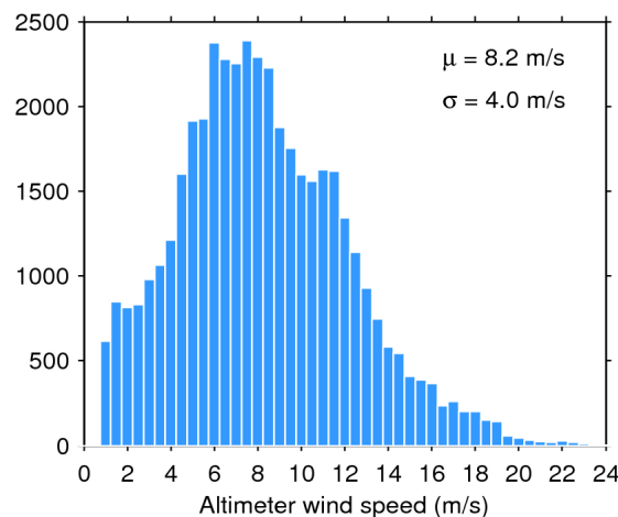
Figure 35. Histogram of science-valid wind over oceans and lakes for 08/03/2020. The mean ( \mu ) and standard deviation ( \sigma ) are also shown. Note that values larger than 24 m/s are excluded from the histogram for the sake of readability but not from the computation of \mu and \sigma .
