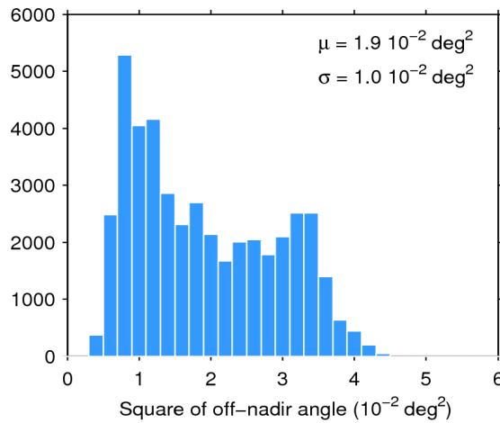
Figure 39. Histogram of flag-valid mispointing over oceans and lakes for 08/03/2020. The mean ( \mu ) and standard deviation ( \sigma ) are also shown. Note that values larger than 6 \cdot 10^{-2} \text{ deg}^2 are excluded from the histogram for the sake of readability but not from the computation of \mu and \sigma .
