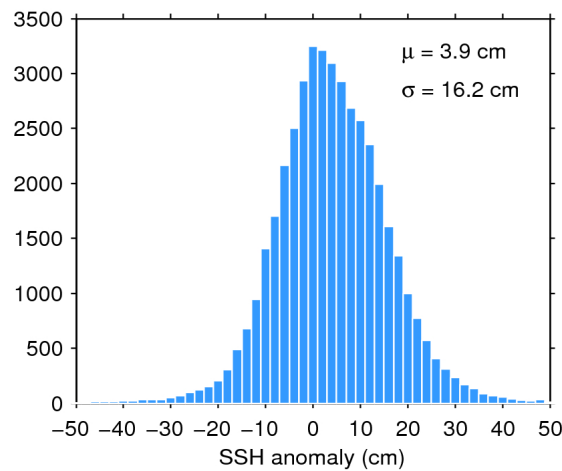
Figure 7. Histogram of flag-valid SSH anomaly over oceans and lakes for 08/03/2020. The mean ( \mu ) and standard deviation ( \sigma ) are also shown. Note that values outside [-50\ 50] cm are excluded from the histogram for the sake of readability but not from the computation of \mu and \sigma .
