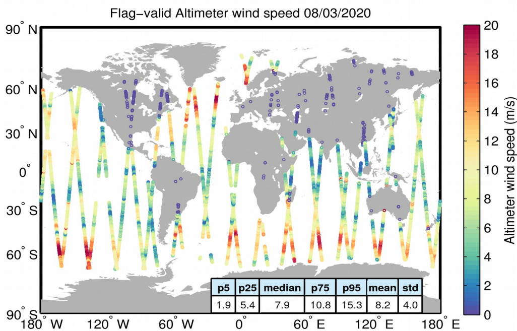
Figure 31. Geographical distribution of flag-valid wind data over oceans and lakes for 08/03/2020. The statistical values shown in the table refer to the wind in m/s and are calculated over all measurements shown in the figure.
