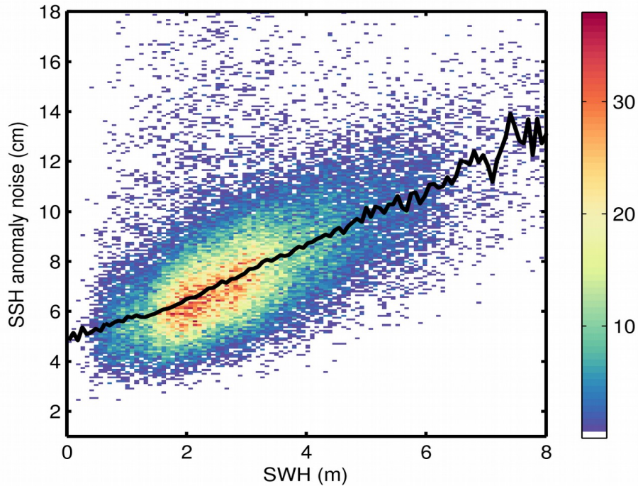
Figure 9. 2D histogram showing flag-valid SSH anomaly noise as a function of SWH for 08/03/2020. The black line denotes the median SSH anomaly noise as a function of SWH.
