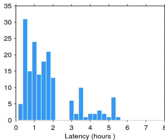
Figure 2. Histogram of the data latency for 08/03/2020. The y-axis denotes the number of files that are made available with a delay of x-hours with respect to the mean time of the records stored in the file.
