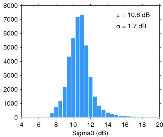
Figure 28. Histogram of science-valid sigma0 over oceans and lakes for 08/03/2020. The mean ( \mu ) and standard deviation ( \sigma ) are also shown. Note that values outside [4 20] dB are excluded from the histogram for the sake of readability but not from the computation of \mu and \sigma .
