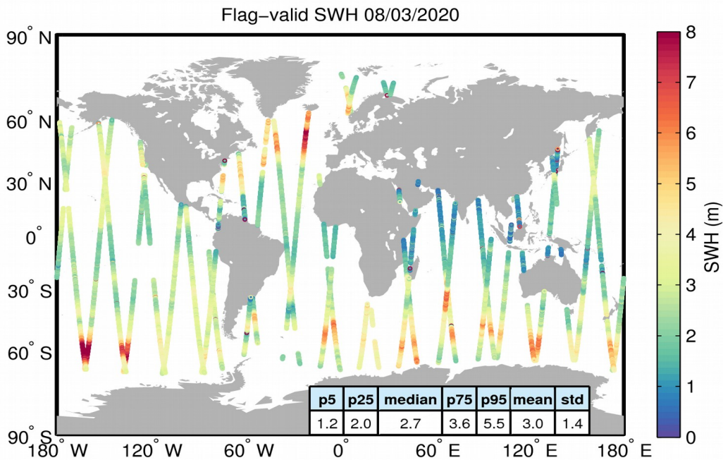
Figure 15. Geographical distribution of flag-valid SWH data over oceans and lakes for 08/03/2020. The statistical values shown in the table refer to the SWH in m and are calculated over all measurements shown in the figure.
