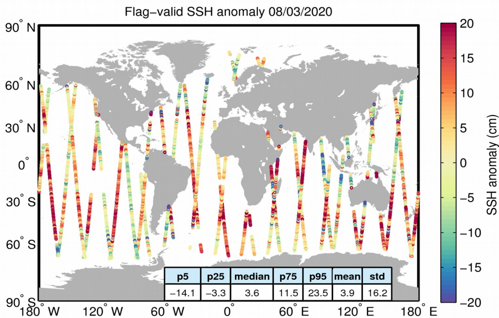
Figure 5. Geographical distribution of flag-valid 1-Hz SSH anomaly data over oceans and lakes for 08/03/2020. The statistical values shown in the table refer to the SSH anomaly in cm and are calculated over all measurements shown in the figure.
