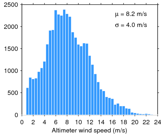
Figure 33. Histogram of flag-valid wind over oceans and lakes for 08/03/2020. The mean ( \mu ) and standard deviation ( \sigma ) are also shown. Note that values larger than 24 m/s are excluded from the histogram for the sake of readability but not from the computation of \mu and \sigma .
