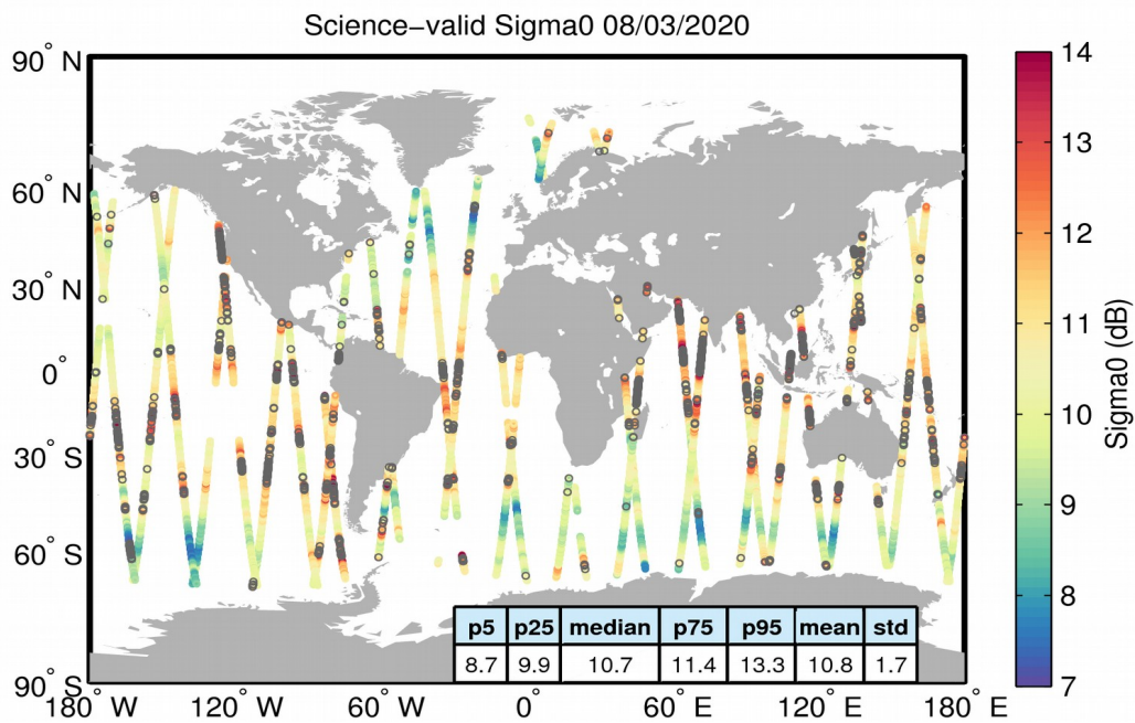
Figure 27. Geographical distribution of science-valid sigma0 data over oceans and lakes for 08/03/2020. The statistical values shown in the table refer to the sigma0 in dB and are calculated over all measurements shown in the figure. Gray circles denote records that have been rejected based on the editing criteria described in Table 4.
