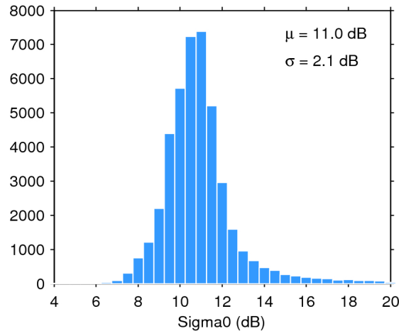
Figure 25. Histogram of flag-valid sigma0 over oceans and lakes for 08/03/2020. The mean ( \mu ) and standard deviation ( \sigma ) are also shown. Note that values outside [4 20] dB are excluded from the histogram for the sake of readability but not from the computation of \mu and \sigma .
