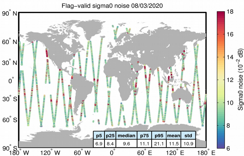
Figure 26. Geographical distribution of flag-valid 20-Hz sigma0 measurement noise over oceans and lakes for 08/03/2020. The statistical values shown in the table refer to the sigma0 noise and are calculated over all measurements shown in the figure.
