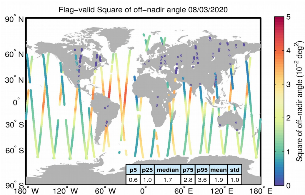
Figure 37. Geographical distribution of flag-valid mispointing data over oceans and lakes for 08/03/2020. The statistical values shown in the table refer to the mispointing in 10^{-2} \text{ deg}^2 and are calculated over all measurements shown in the figure.
