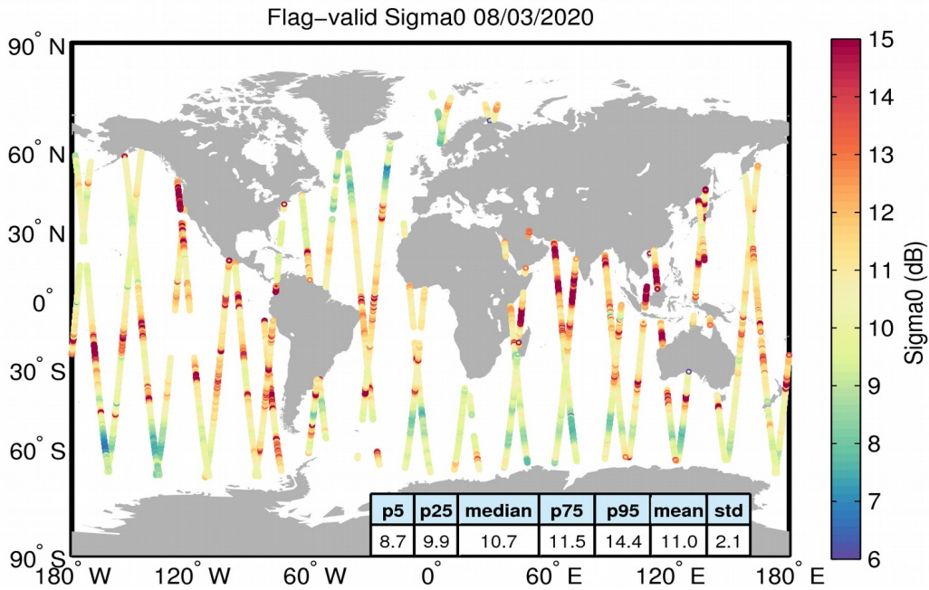
Figure 23. Geographical distribution of flag-valid sigma0 data over oceans and lakes for 08/03/2020. The statistical values shown in the table refer to the sigma0 in dB and are calculated over all measurements shown in the figure.
