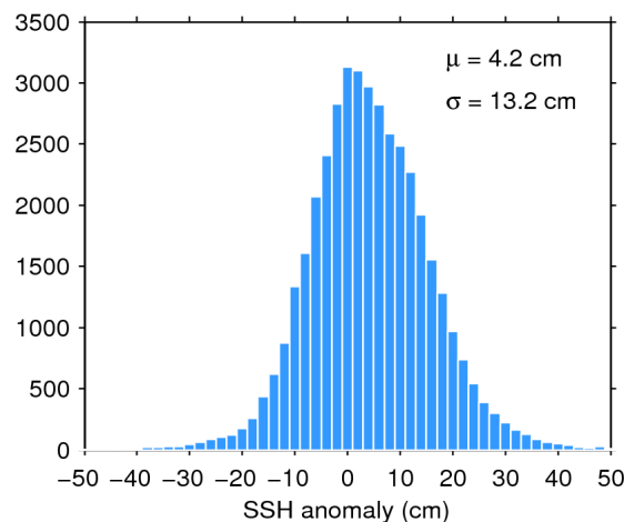
Figure 11. Histogram of science-valid SSH anomaly over oceans and lakes for 08/03/2020. The mean ( \mu ) and standard deviation ( \sigma ) are also shown. Note that values outside [-50 50] cm are excluded from the histogram for the sake of readability but not from the computation of \mu and \sigma .
