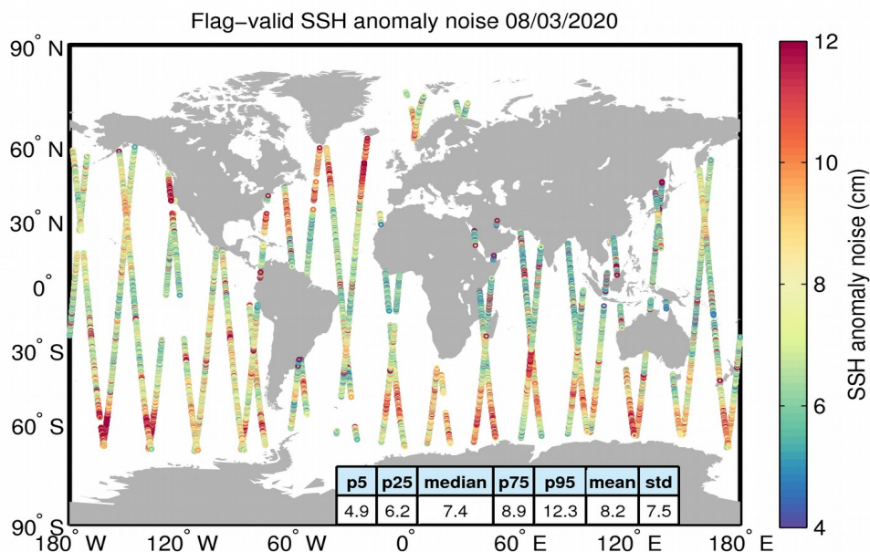
Figure 8. Geographical distribution of flag-valid 20-Hz SSH anomaly measurement noise over oceans and lakes for 08/03/2020. The statistical values shown in the table refer to the SSH anomaly noise and are calculated over all measurements shown in the figure.
