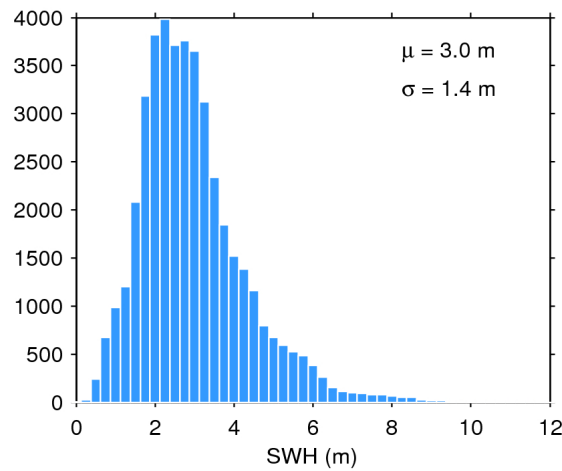
Figure 17. Histogram of flag-valid SWH over oceans and lakes for 08/03/2020. The mean ( \mu ) and standard deviation ( \sigma ) are also shown. Note that values larger than 12 m are excluded from the histogram for the sake of readability but not from the computation of \mu and \sigma .
