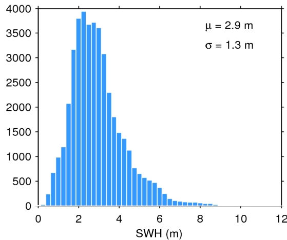
Figure 20. Histogram of science-valid SWH over oceans and lakes for 08/03/2020. The mean ( \mu ) and standard deviation ( \sigma ) are also shown. Note that values larger than 12 m are excluded from the histogram for the sake of readability but not from the computation of \mu and \sigma .
