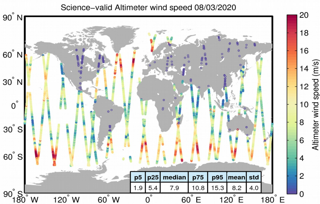
Figure 34. Geographical distribution of science-valid wind data over oceans and lakes for 08/03/2020. The statistical values shown in the table refer to the wind in m/s and are calculated over all measurements shown in the figure. Gray circles denote records that have been rejected based on the editing criteria described in Table 5.
