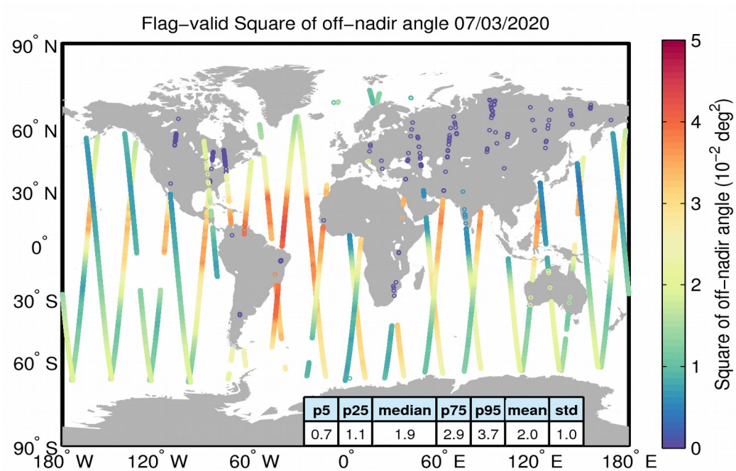
Figure 37. Geographical distribution of flag-valid mispointing data over oceans and lakes for 07/03/2020. The statistical values shown in the table refer to the mispointing in 10^{-2} deg 2 and are calculated over all measurements shown in the figure.
