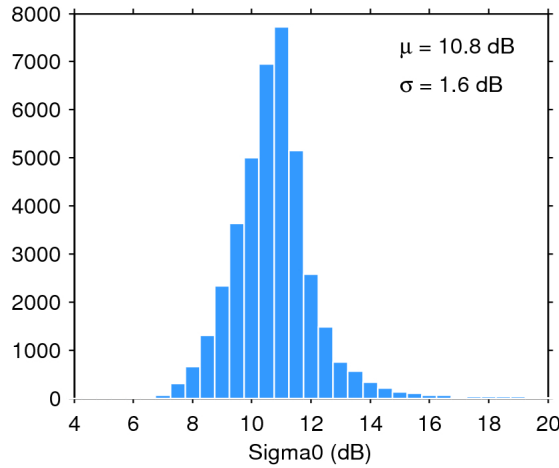
Figure 28. Histogram of science-valid sigma0 over oceans and lakes for 07/03/2020. The mean ( \mu ) and standard deviation ( \sigma ) are also shown. Note that values outside [4 20] dB are excluded from the histogram for the sake of readability but not from the computation of \mu and \sigma .
