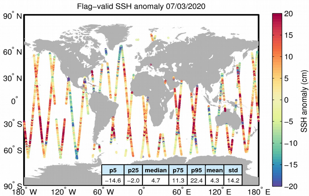
Figure 5. Geographical distribution of flag-valid 1-Hz SSH anomaly data over oceans and lakes for 07/03/2020. The statistical values shown in the table refer to the SSH anomaly in cm and are calculated over all measurements shown in the figure.
