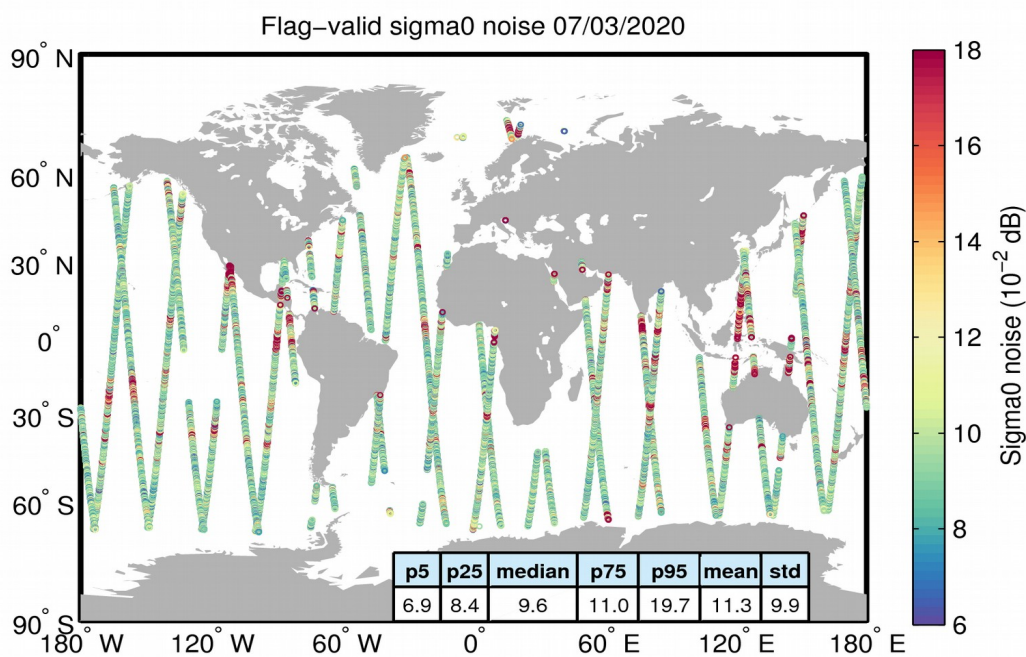
Figure 26. Geographical distribution of flag-valid 20-Hz sigma0 measurement noise over oceans and lakes for 07/03/2020. The statistical values shown in the figure refer to the sigma0 noise and are calculated over all measurements shown in the figure.
