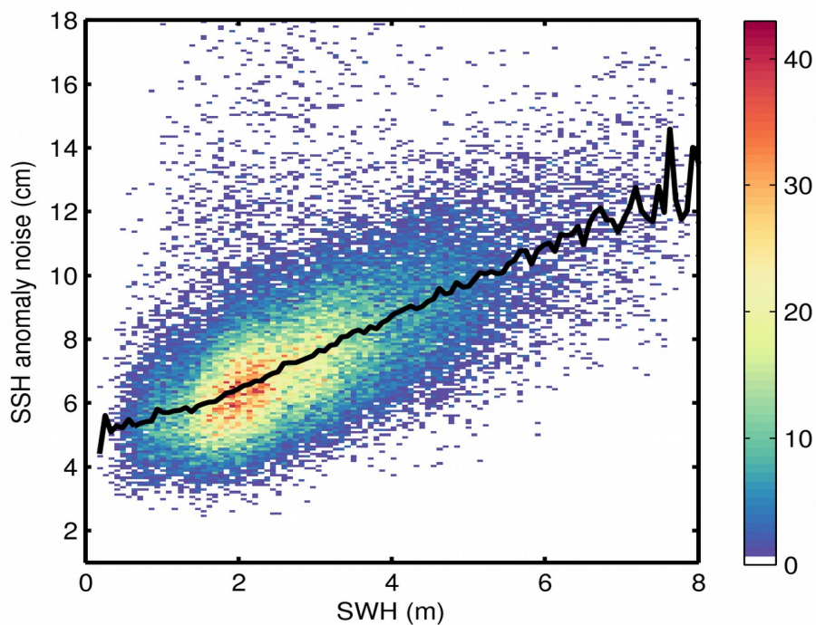
Figure 9. 2D histogram showing flag-valid SSH anomaly noise as a function of SWH for 07/03/2020. The black line denotes the median SSH anomaly noise as a function of SWH.
