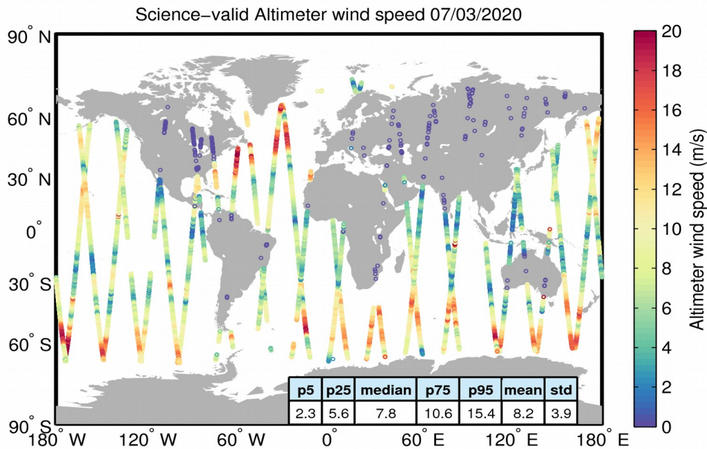
Figure 34. Geographical distribution of science-valid wind data over oceans and lakes for 07/03/2020. The statistical values shown in the table refer to the wind in m/s and are calculated over all measurements shown in the figure. Gray circles denote records that have been rejected based on the editing criteria described in Table 5.
