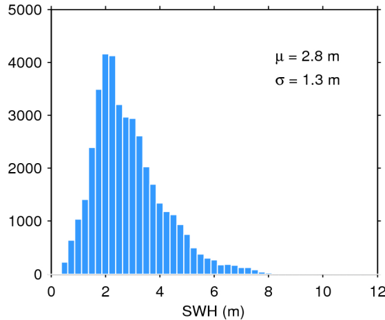
Figure 20. Histogram of science-valid SWH over oceans and lakes for 07/03/2020. The mean ( \mu ) and standard deviation ( \sigma ) are also shown. Note that values larger than 12 m are excluded from the histogram for the sake of readability but not from the computation of \mu and \sigma .
