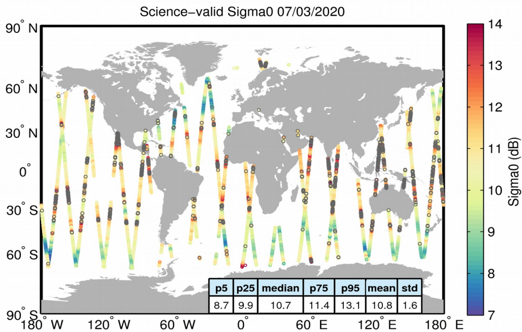
Figure 27. Geographical distribution of science-valid sigma0 data over oceans and lakes for 07/03/2020. The statistical values shown in the table refer to the sigma0 in dB and are calculated over all measurements shown in the figure. Gray circles denote records that have been rejected based on the editing criteria described in Table 4.
