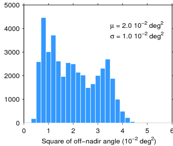
Figure 39. Histogram of flag-valid mispointing over oceans and lakes for 07/03/2020. The mean ( \mu ) and standard deviation ( \sigma ) are also shown. Note that values larger than 6 \cdot 10^{-2} \text{ deg}^2 are excluded from the histogram for the sake of readability but not from the computation of \mu and \sigma .
