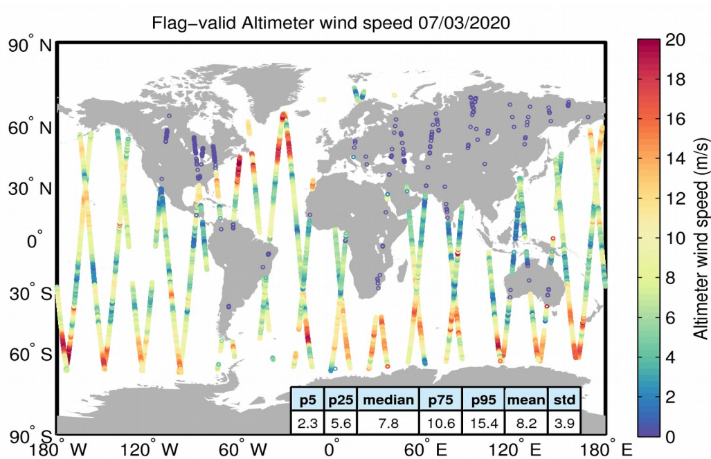
Figure 31. Geographical distribution of flag-valid wind data over oceans and lakes for 07/03/2020. The statistical values shown in the table refer to the wind in m/s and are calculated over all measurements shown in the figure.
