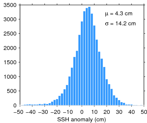
Figure 7. Histogram of flag-valid SSH anomaly over oceans and lakes for 07/03/2020. The mean ( \mu ) and standard deviation ( \sigma ) are also shown. Note that values outside [-50 50] cm are excluded from the histogram for the sake of readability but not from the computation of \mu and \sigma .
