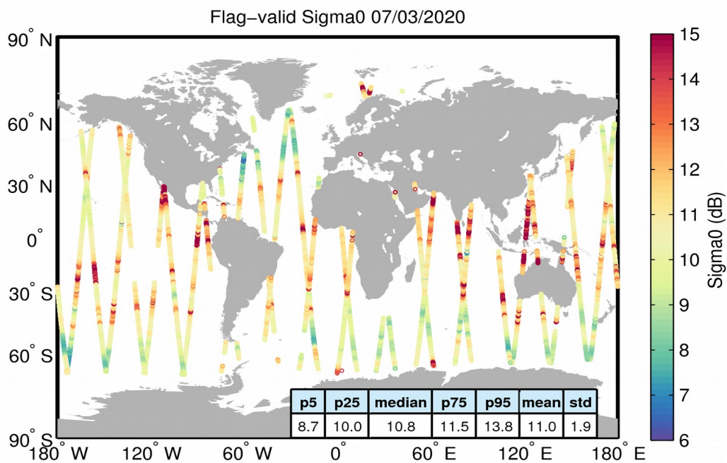
Figure 23. Geographical distribution of flag-valid sigma0 data over oceans and lakes for 07/03/2020. The statistical values shown in the table refer to the sigma0 in dB and are calculated over all measurements shown in the figure.
