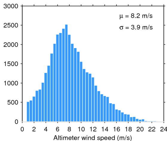
Figure 35. Histogram of science-valid wind over oceans and lakes for 07/03/2020. The mean ( \mu ) and standard deviation ( \sigma ) are also shown. Note that values larger than 24 m/s are excluded from the histogram for the sake of readability but not from the computation of \mu and \sigma .
