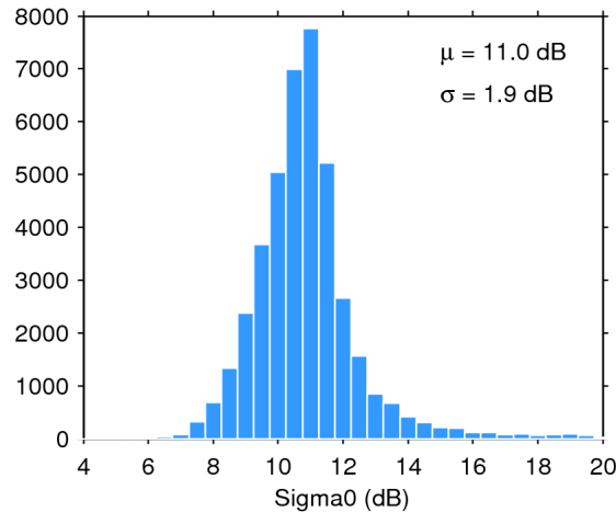
Figure 25. Histogram of flag-valid sigma0 over oceans and lakes for 07/03/2020. The mean ( \mu ) and standard deviation ( \sigma ) are also shown. Note that values outside [4 20] dB are excluded from the histogram for the sake of readability but not from the computation of \mu and \sigma .
