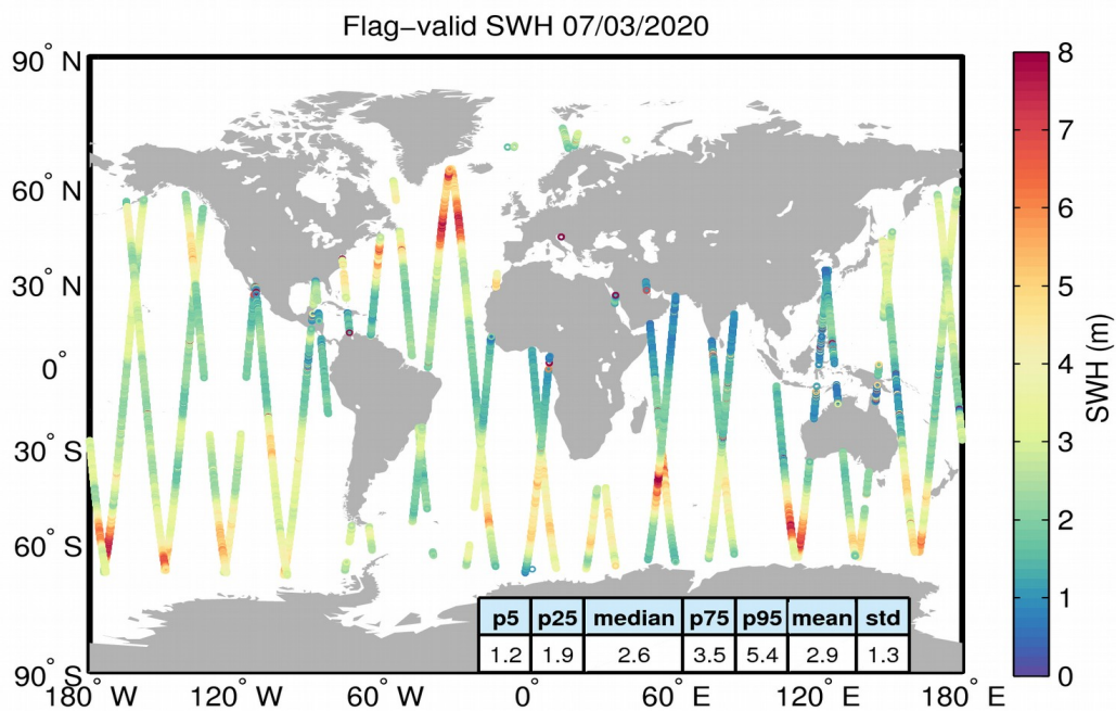
Figure 15. Geographical distribution of flag-valid SWH data over oceans and lakes for 07/03/2020. The statistical values shown in the table refer to the SWH in m and are calculated over all measurements shown in the figure.
