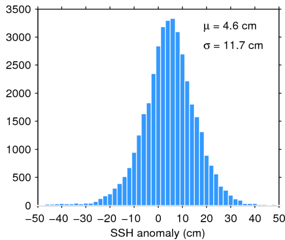
Figure 11. Histogram of science-valid SSH anomaly over oceans and lakes for 07/03/2020. The mean ( \mu ) and standard deviation ( \sigma ) are also shown. Note that values outside [-50 50] cm are excluded from the histogram for the sake of readability but not from the computation of \mu and \sigma .
