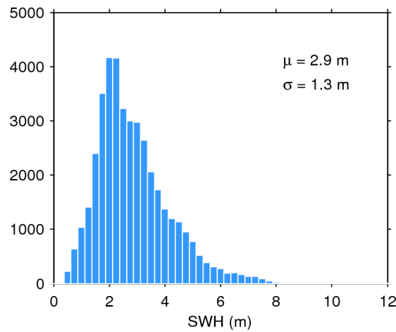
Figure 17. Histogram of flag-valid SWH over oceans and lakes for 07/03/2020. The mean ( \mu ) and standard deviation ( \sigma ) are also shown. Note that values larger than 12 m are excluded from the histogram for the sake of readability but not from the computation of \mu and \sigma .
