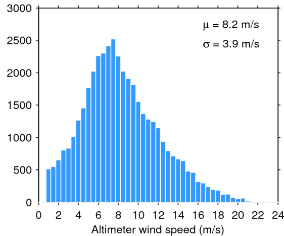
Figure 33. Histogram of flag-valid wind over oceans and lakes for 07/03/2020. The mean ( \mu ) and standard deviation ( \sigma ) are also shown. Note that values larger than 24 m/s are excluded from the histogram for the sake of readability but not from the computation of \mu and \sigma .
