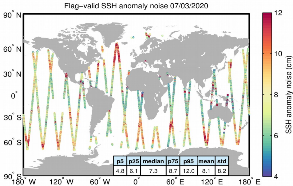
Figure 8. Geographical distribution of flag-valid 20-Hz SSH anomaly measurement noise over oceans and lakes for 07/03/2020. The statistical values shown in the table refer to the SSH anomaly noise and are calculated over all measurements shown in the figure.
