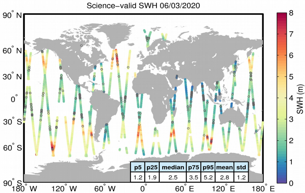
Figure 19. Geographical distribution of science-valid SWH data over oceans and lakes for 06/03/2020. The statistical values shown in the table refer to the SWH in m and are calculated over all measurements shown in the figure. Gray circles denote records that have been rejected based on the editing criteria described in Table 3.
