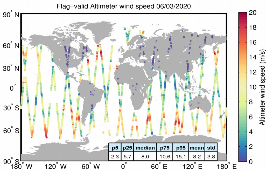
Figure 31. Geographical distribution of flag-valid wind data over oceans and lakes for 06/03/2020. The statistical values shown in the table refer to the wind in m/s and are calculated over all measurements shown in the figure.
