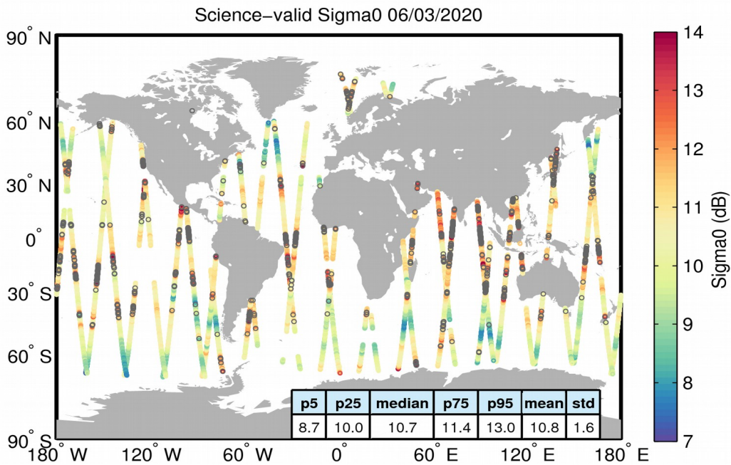
Figure 27. Geographical distribution of science-valid sigma0 data over oceans and lakes for 06/03/2020. The statistical values shown in the table refer to the sigma0 in dB and are calculated over all measurements shown in the figure. Gray circles denote records that have been rejected based on the editing criteria described in Table 4.
