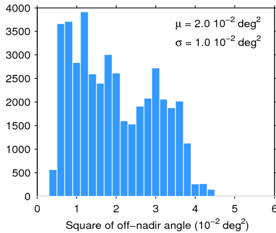
Figure 39. Histogram of flag-valid mispointing over oceans and lakes for 06/03/2020. The mean ( \mu ) and standard deviation ( \sigma ) are also shown. Note that values larger than 6 \cdot 10^{-2} \text{ deg}^2 are excluded from the histogram for the sake of readability but not from the computation of \mu and \sigma .
