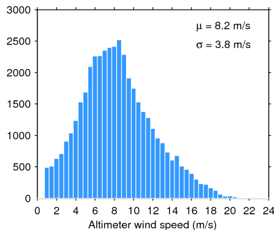
Figure 35. Histogram of science-valid wind over oceans and lakes for 06/03/2020. The mean ( \mu ) and standard deviation ( \sigma ) are also shown. Note that values larger than 24 m/s are excluded from the histogram for the sake of readability but not from the computation of \mu and \sigma .
