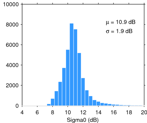
Figure 25. Histogram of flag-valid sigma0 over oceans and lakes for 06/03/2020. The mean ( \mu ) and standard deviation ( \sigma ) are also shown. Note that values outside [4 20] dB are excluded from the histogram for the sake of readability but not from the computation of \mu and \sigma .
