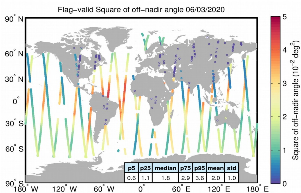
Figure 37. Geographical distribution of flag-valid mispointing data over oceans and lakes for 06/03/2020. The statistical values shown in the table refer to the mispointing in 10^{-2} \text{ deg}^2 and are calculated over all measurements shown in the figure.
