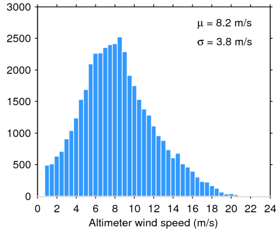
Figure 33. Histogram of flag-valid wind over oceans and lakes for 06/03/2020. The mean ( \mu ) and standard deviation ( \sigma ) are also shown. Note that values larger than 24 m/s are excluded from the histogram for the sake of readability but not from the computation of \mu and \sigma .
