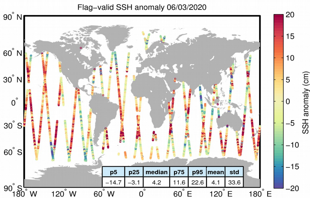
Figure 5. Geographical distribution of flag-valid 1-Hz SSH anomaly data over oceans and lakes for 06/03/2020. The statistical values shown in the table refer to the SSH anomaly in cm and are calculated over all measurements shown in the figure.
