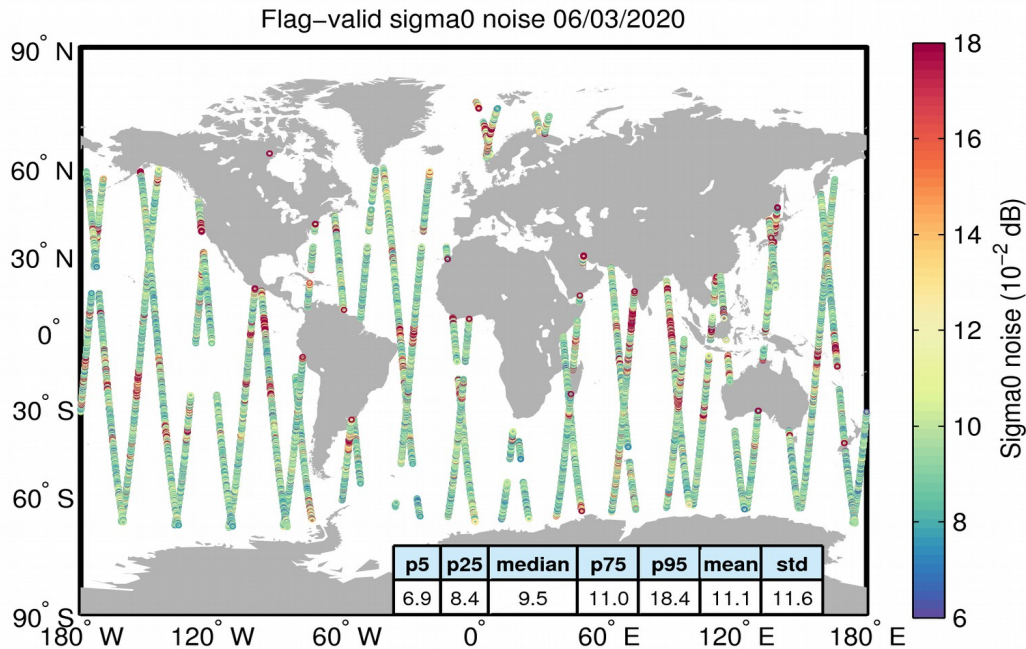
Figure 26. Geographical distribution of flag-valid 20-Hz sigma0 measurement noise over oceans and lakes for 06/03/2020. The statistical values shown in the table refer to the sigma0 noise and are calculated over all measurements shown in the figure.
