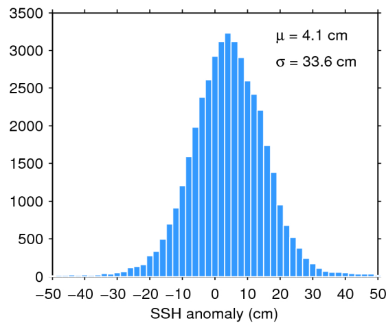
Figure 7. Histogram of flag-valid SSH anomaly over oceans and lakes for 06/03/2020. The mean ( \mu ) and standard deviation ( \sigma ) are also shown. Note that values outside [-50\ 50] cm are excluded from the histogram for the sake of readability but not from the computation of \mu and \sigma .
