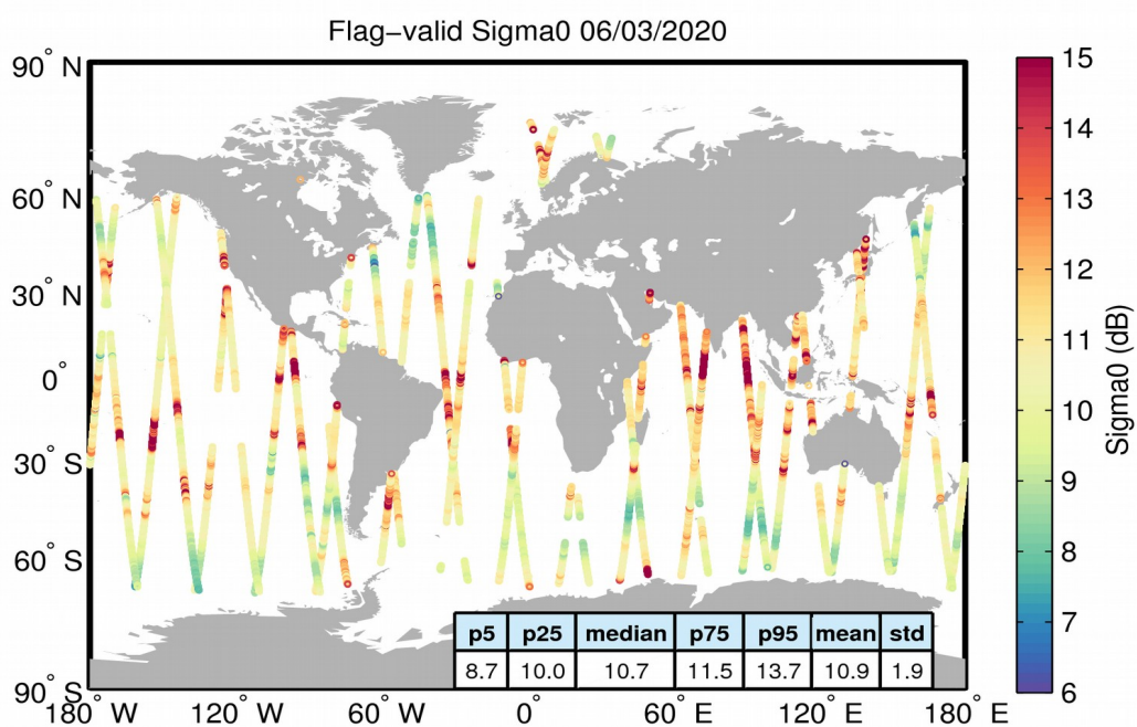
Figure 23. Geographical distribution of flag-valid sigma0 data over oceans and lakes for 06/03/2020. The statistical values shown in the table refer to the sigma0 in dB and are calculated over all measurements shown in the figure.
