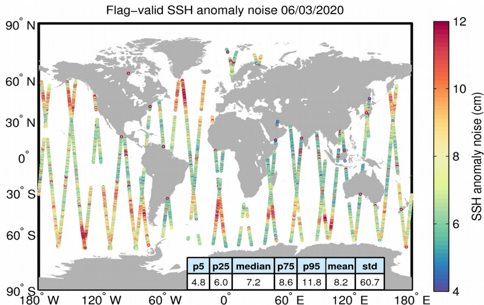
Figure 8. Geographical distribution of flag-valid 20-Hz SSH anomaly measurement noise over oceans and lakes for 06/03/2020. The statistical values shown in the table refer to the SSH anomaly noise and are calculated over all measurements shown in the figure.
