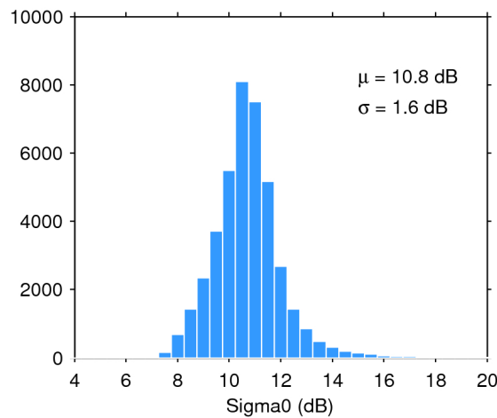
Figure 28. Histogram of science-valid sigma0 over oceans and lakes for 06/03/2020. The mean ( \mu ) and standard deviation ( \sigma ) are also shown. Note that values outside [4 20] dB are excluded from the histogram for the sake of readability but not from the computation of \mu and \sigma .
