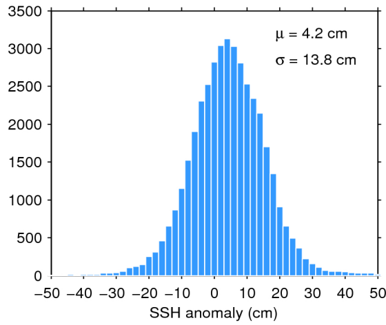
Figure 11. Histogram of science-valid SSH anomaly over oceans and lakes for 06/03/2020. The mean ( \mu ) and standard deviation ( \sigma ) are also shown. Note that values outside [-50 50] cm are excluded from the histogram for the sake of readability but not from the computation of \mu and \sigma .
