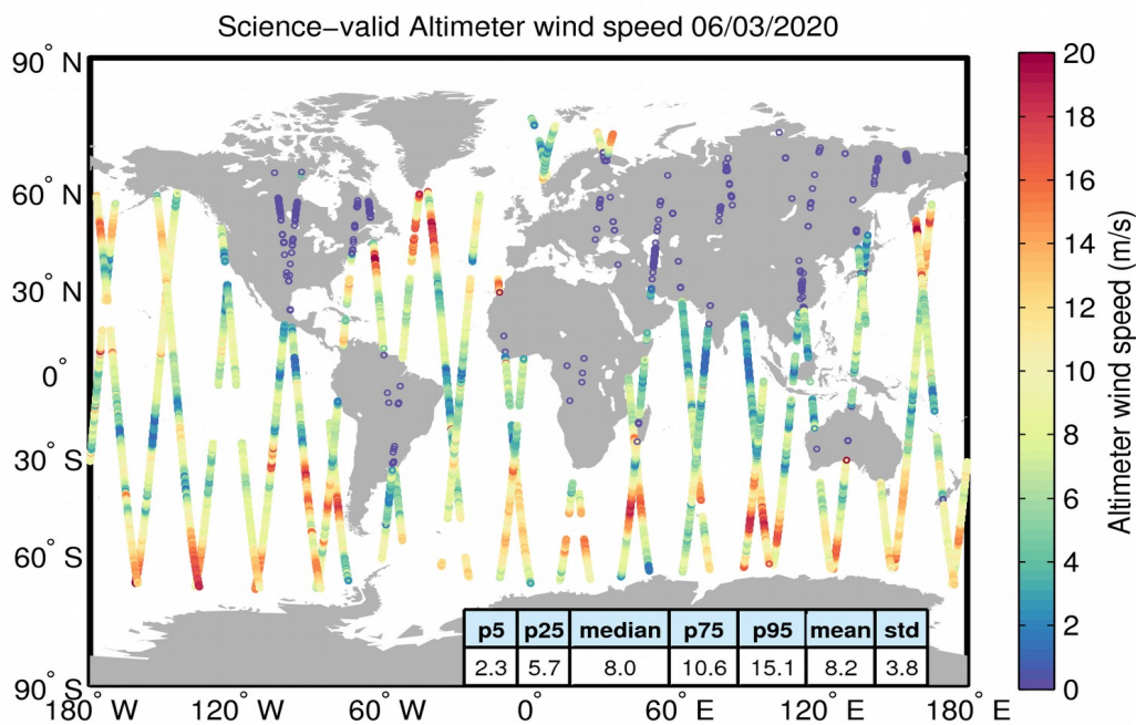
Figure 34. Geographical distribution of science-valid wind data over oceans and lakes for 06/03/2020. The statistical values shown in the table refer to the wind in m/s and are calculated over all measurements shown in the figure. Gray circles denote records that have been rejected based on the editing criteria described in Table 5.
