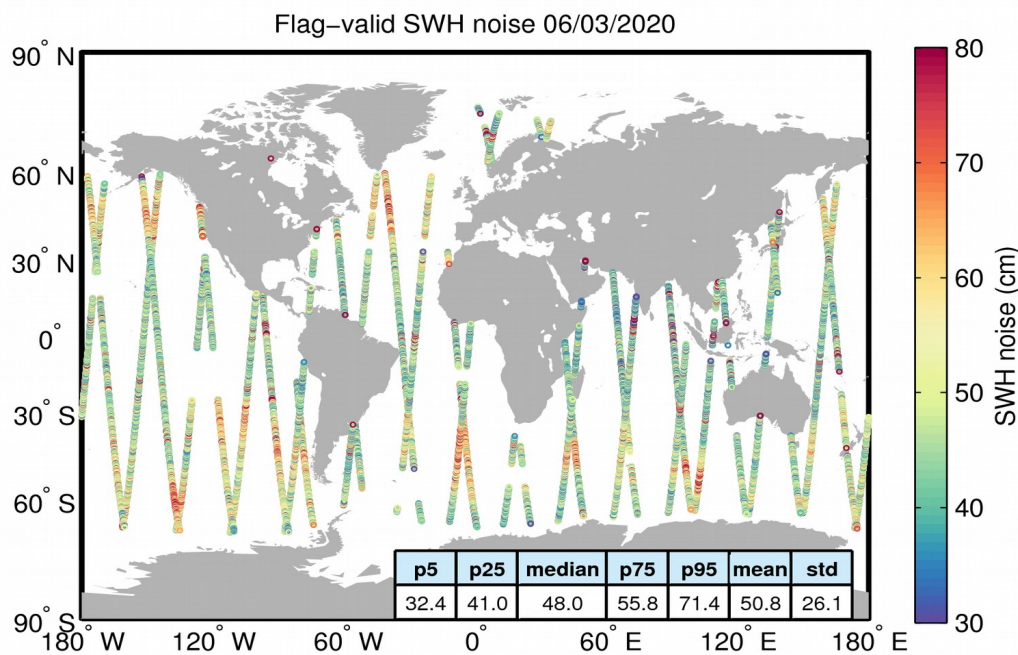
Figure 18. Geographical distribution of flag-valid 20-Hz SWH measurement noise over oceans and lakes for 06/03/2020. The statistical values shown in the figure refer to the SWH noise and are calculated over all measurements shown in the figure.
