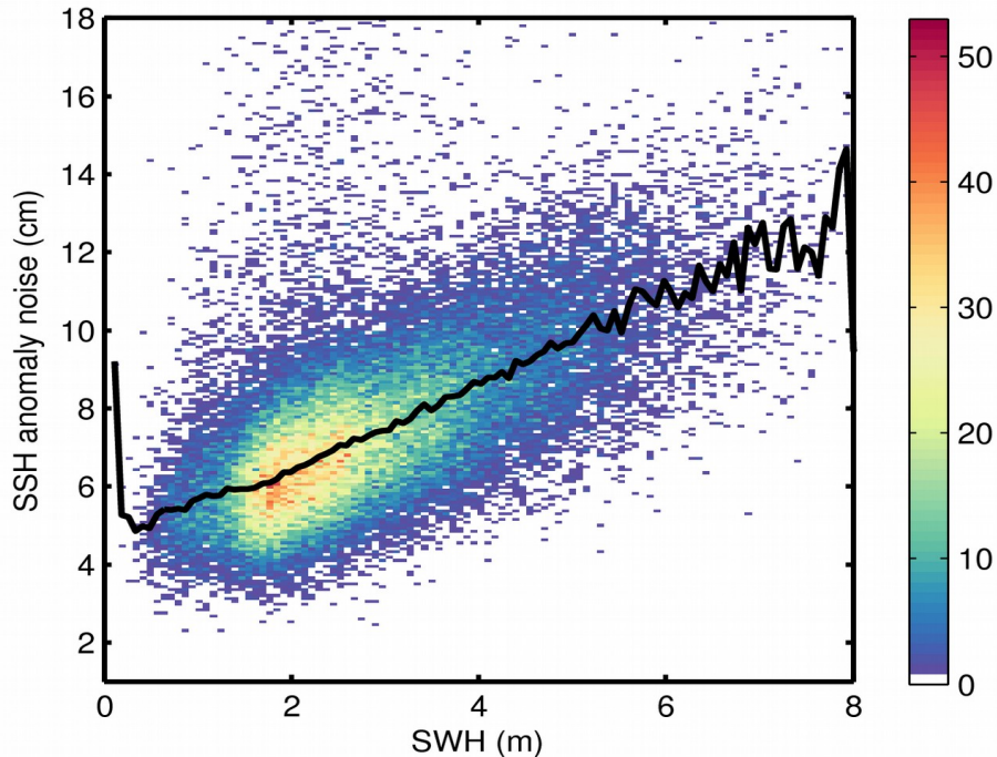
Figure 9. 2D histogram showing flag-valid SSH anomaly noise as a function of SWH for 06/03/2020. The black line denotes the median SSH anomaly noise as a function of SWH.
