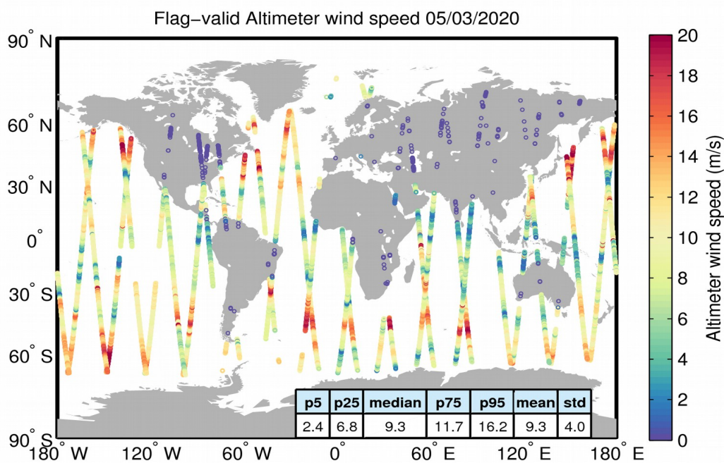
Figure 31. Geographical distribution of flag-valid wind data over oceans and lakes for 05/03/2020. The statistical values shown in the table refer to the wind in m/s and are calculated over all measurements shown in the figure.
