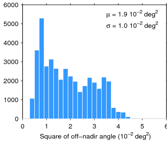
Figure 39. Histogram of flag-valid mispointing over oceans and lakes for 05/03/2020. The mean ( \mu ) and standard deviation ( \sigma ) are also shown. Note that values larger than 6 \cdot 10^{-2} \text{ deg}^2 are excluded from the histogram for the sake of readability but not from the computation of \mu and \sigma .
