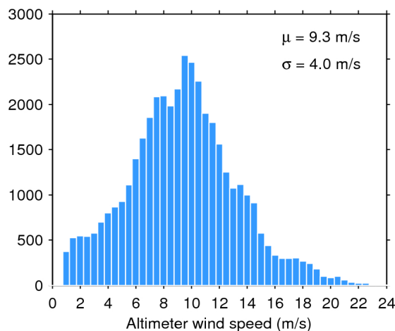
Figure 35. Histogram of science-valid wind over oceans and lakes for 05/03/2020. The mean ( \mu ) and standard deviation ( \sigma ) are also shown. Note that values larger than 24 m/s are excluded from the histogram for the sake of readability but not from the computation of \mu and \sigma .
