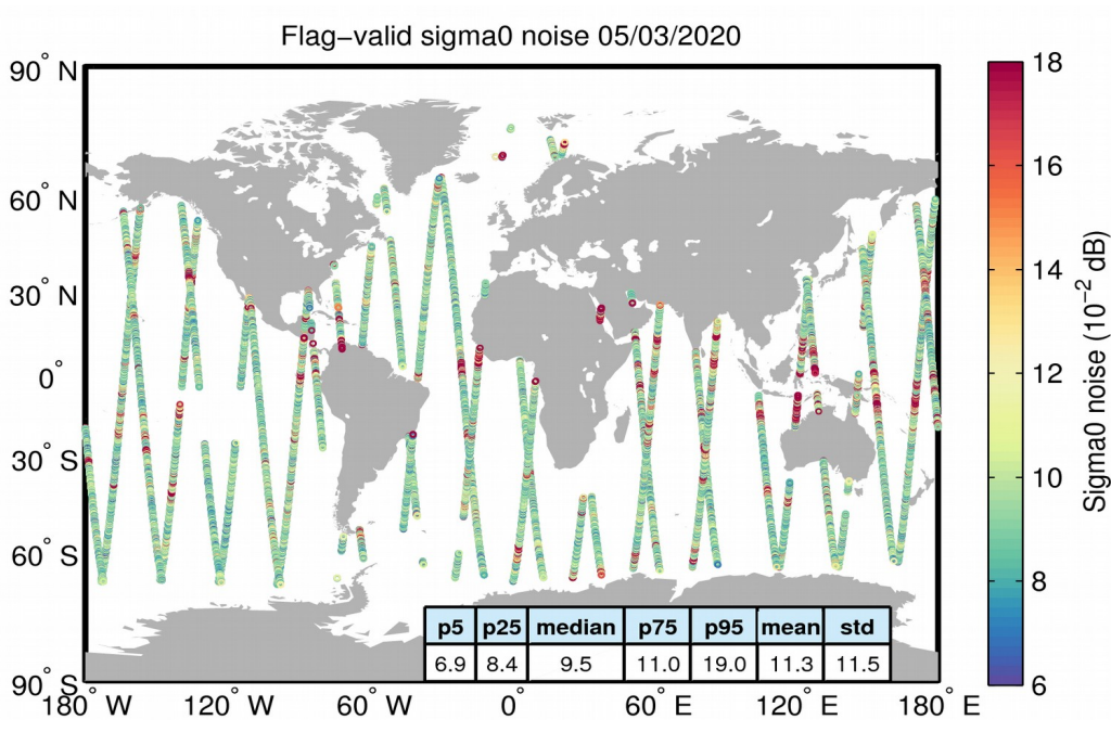
Figure 26. Geographical distribution of flag-valid 20-Hz sigma0 measurement noise over oceans and lakes for 05/03/2020. The statistical values shown in the table refer to the sigma0 noise and are calculated over all measurements shown in the figure.
