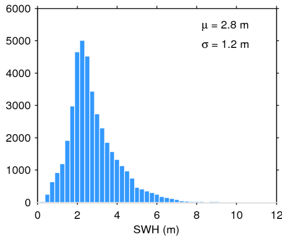
Figure 20. Histogram of science-valid SWH over oceans and lakes for 05/03/2020. The mean ( \mu ) and standard deviation ( \sigma ) are also shown. Note that values larger than 12 m are excluded from the histogram for the sake of readability but not from the computation of \mu and \sigma .
