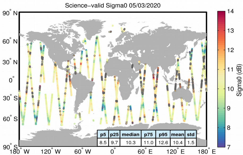
Figure 27. Geographical distribution of science-valid sigma0 data over oceans and lakes for 05/03/2020. The statistical values shown in the table refer to the sigma0 in dB and are calculated over all measurements shown in the figure. Gray circles denote records that have been rejected based on the editing criteria described in Table 4.
