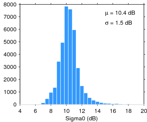
Figure 28. Histogram of science-valid sigma0 over oceans and lakes for 05/03/2020. The mean ( \mu ) and standard deviation ( \sigma ) are also shown. Note that values outside [4 20] dB are excluded from the histogram for the sake of readability but not from the computation of \mu and \sigma .
