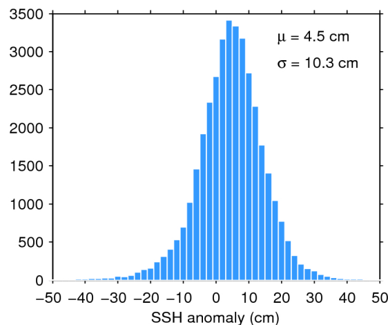
Figure 11. Histogram of science-valid SSH anomaly over oceans and lakes for 05/03/2020. The mean ( \mu ) and standard deviation ( \sigma ) are also shown. Note that values outside [-50 50] cm are excluded from the histogram for the sake of readability but not from the computation of \mu and \sigma .
