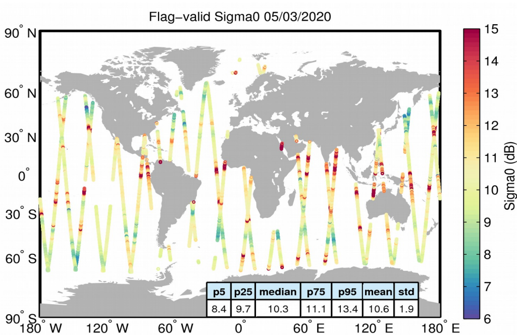
Figure 23. Geographical distribution of flag-valid sigma0 data over oceans and lakes for 05/03/2020. The statistical values shown in the table refer to the sigma0 in dB and are calculated over all measurements shown in the figure.
