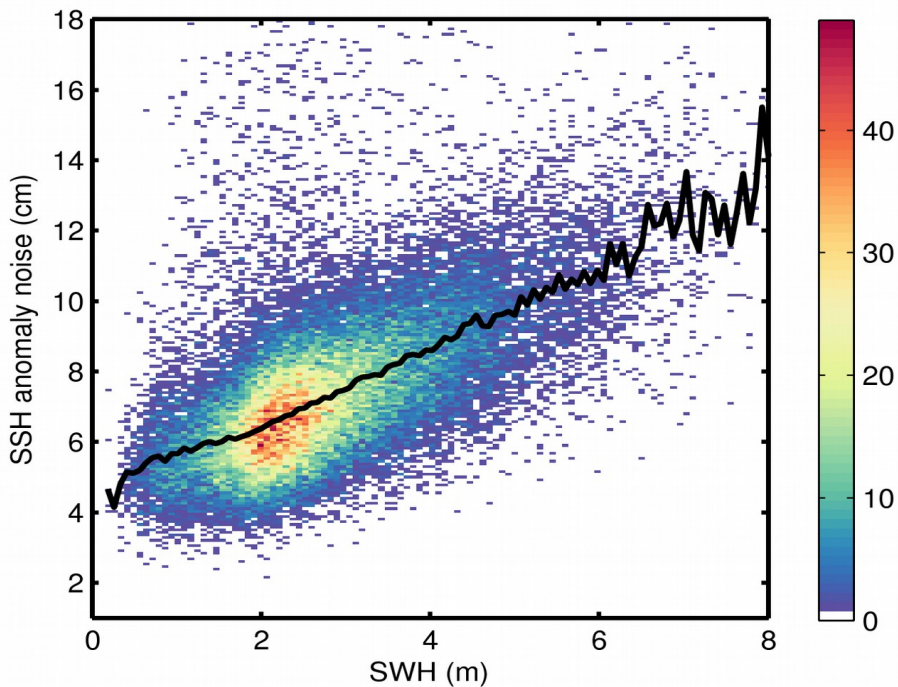
Figure 9. 2D histogram showing flag-valid SSH anomaly noise as a function of SWH for 05/03/2020. The black line denotes the median SSH anomaly noise as a function of SWH.
