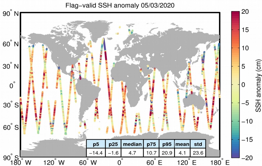
Figure 5. Geographical distribution of flag-valid 1-Hz SSH anomaly data over oceans and lakes for 05/03/2020. The statistical values shown in the table refer to the SSH anomaly in cm and are calculated over all measurements shown in the figure.
