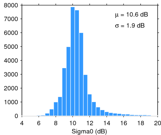
Figure 25. Histogram of flag-valid sigma0 over oceans and lakes for 05/03/2020. The mean ( \mu ) and standard deviation ( \sigma ) are also shown. Note that values outside [4 20] dB are excluded from the histogram for the sake of readability but not from the computation of \mu and \sigma .
