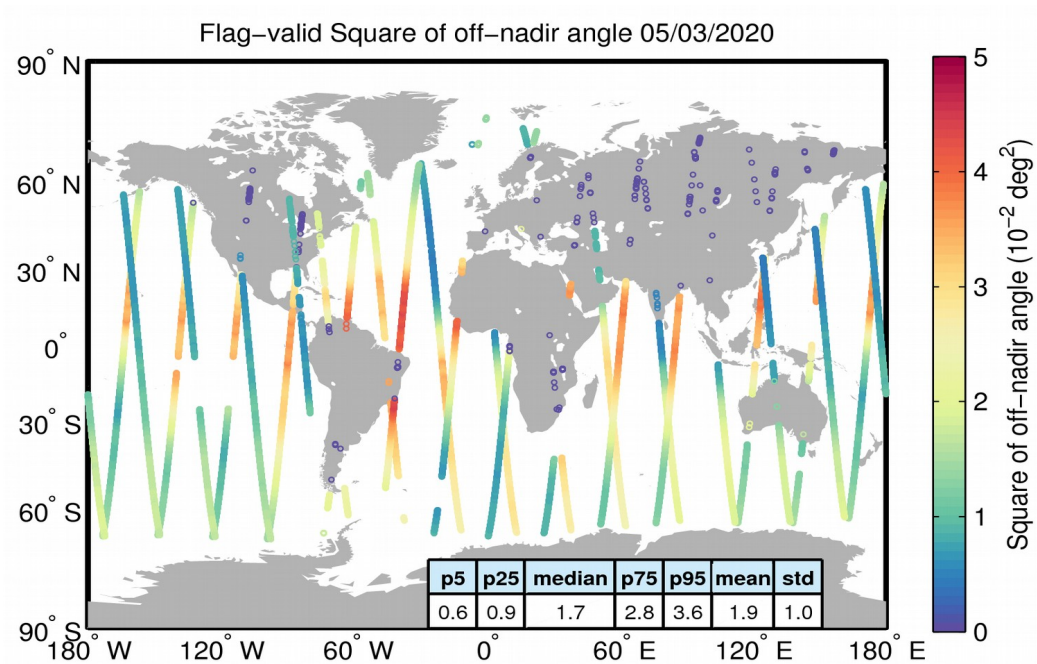
Figure 37. Geographical distribution of flag-valid mispointing data over oceans and lakes for 05/03/2020. The statistical values shown in the table refer to the mispointing in 10^{-2} \text{ deg}^2 and are calculated over all measurements shown in the figure.
