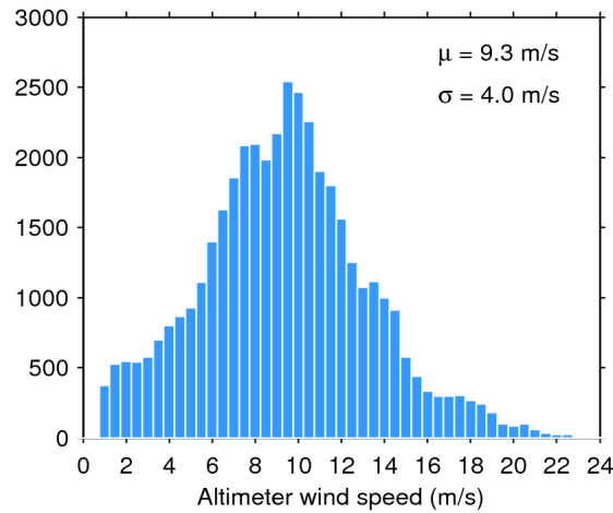
Figure 33. Histogram of flag-valid wind over oceans and lakes for 05/03/2020. The mean ( \mu ) and standard deviation ( \sigma ) are also shown. Note that values larger than 24 m/s are excluded from the histogram for the sake of readability but not from the computation of \mu and \sigma .
