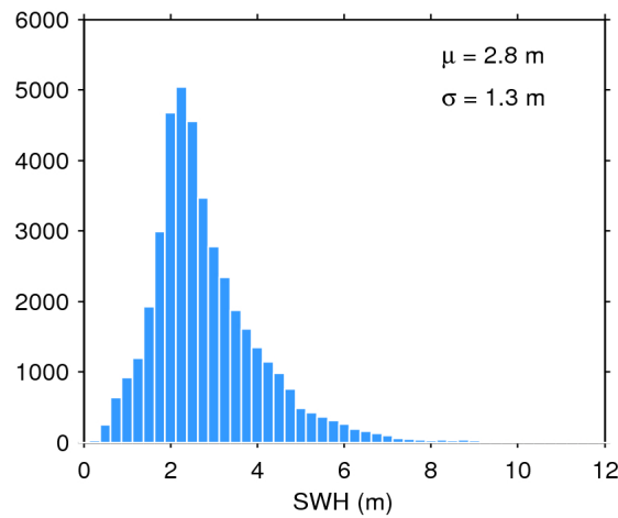
Figure 17. Histogram of flag-valid SWH over oceans and lakes for 05/03/2020. The mean ( \mu ) and standard deviation ( \sigma ) are also shown. Note that values larger than 12 m are excluded from the histogram for the sake of readability but not from the computation of \mu and \sigma .
