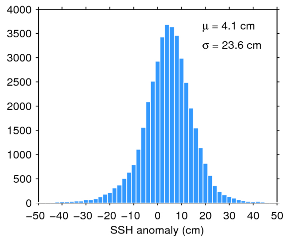
Figure 7. Histogram of flag-valid SSH anomaly over oceans and lakes for 05/03/2020. The mean ( \mu ) and standard deviation ( \sigma ) are also shown. Note that values outside [-50 50] cm are excluded from the histogram for the sake of readability but not from the computation of \mu and \sigma .
