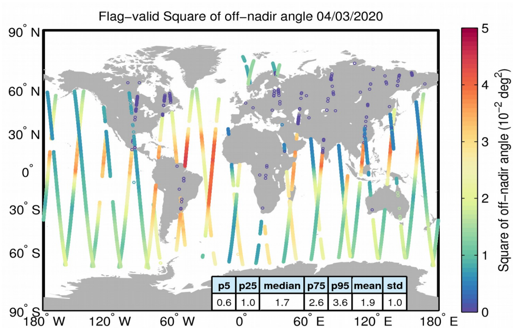
Figure 37. Geographical distribution of flag-valid mispointing data over oceans and lakes for 04/03/2020. The statistical values shown in the table refer to the mispointing in 10^{-2} \text{ deg}^2 and are calculated over all measurements shown in the figure.
