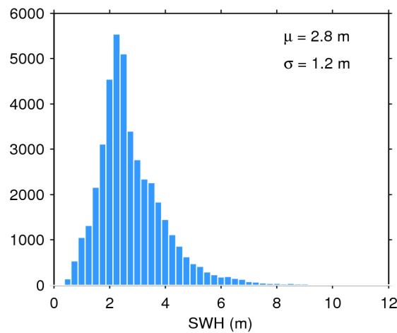
Figure 17. Histogram of flag-valid SWH over oceans and lakes for 04/03/2020. The mean ( \mu ) and standard deviation ( \sigma ) are also shown. Note that values larger than 12 m are excluded from the histogram for the sake of readability but not from the computation of \mu and \sigma .
