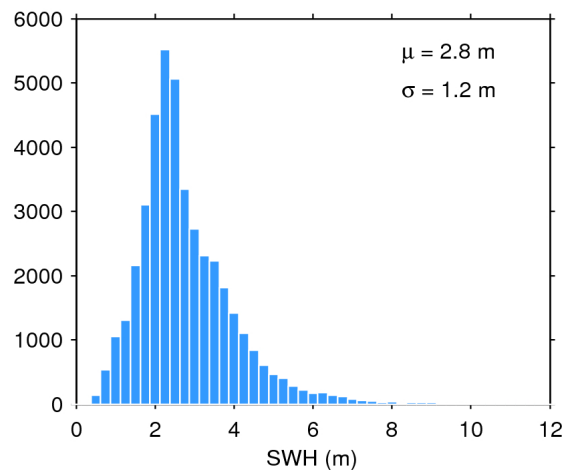
Figure 20. Histogram of science-valid SWH over oceans and lakes for 04/03/2020. The mean ( \mu ) and standard deviation ( \sigma ) are also shown. Note that values larger than 12 m are excluded from the histogram for the sake of readability but not from the computation of \mu and \sigma .
