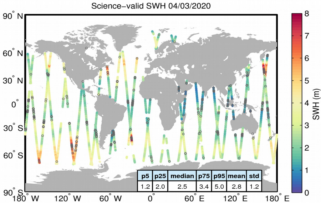
Figure 19. Geographical distribution of science-valid SWH data over oceans and lakes for 04/03/2020. The statistical values shown in the table refer to the SWH in m and are calculated over all measurements shown in the figure. Gray circles denote records that have been rejected based on the editing criteria described in Table 3.
