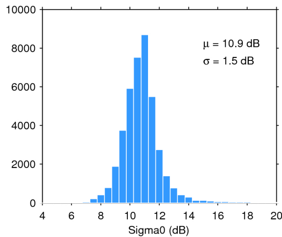
Figure 28. Histogram of science-valid sigma0 over oceans and lakes for 04/03/2020. The mean ( \mu ) and standard deviation ( \sigma ) are also shown. Note that values outside [4 20] dB are excluded from the histogram for the sake of readability but not from the computation of \mu and \sigma .
