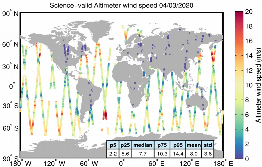
Figure 34. Geographical distribution of science-valid wind data over oceans and lakes for 04/03/2020. The statistical values shown in the table refer to the wind in m/s and are calculated over all measurements shown in the figure. Gray circles denote records that have been rejected based on the editing criteria described in Table 5.
