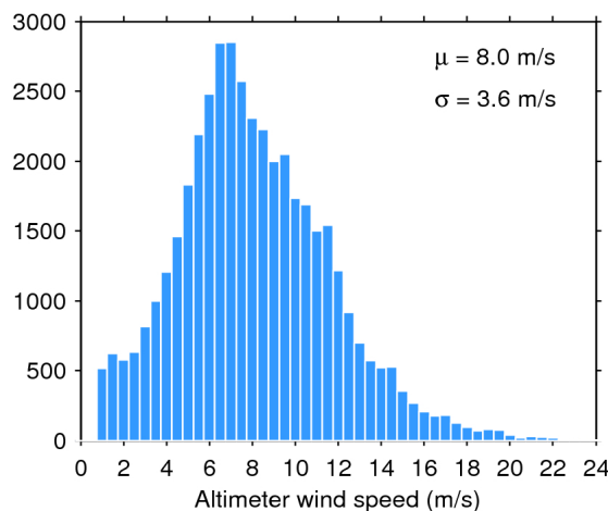
Figure 35. Histogram of science-valid wind over oceans and lakes for 04/03/2020. The mean ( \mu ) and standard deviation ( \sigma ) are also shown. Note that values larger than 24 m/s are excluded from the histogram for the sake of readability but not from the computation of \mu and \sigma .
