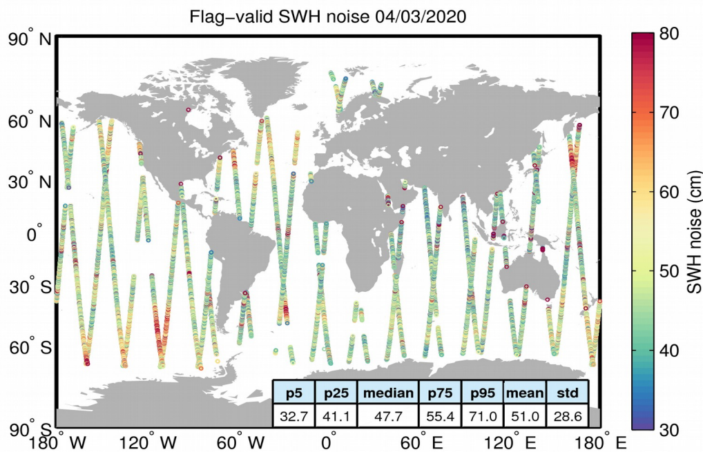
Figure 18. Geographical distribution of flag-valid 20-Hz SWH measurement noise over oceans and lakes for 04/03/2020. The statistical values shown in the figure refer to the SWH noise and are calculated over all measurements shown in the figure.
