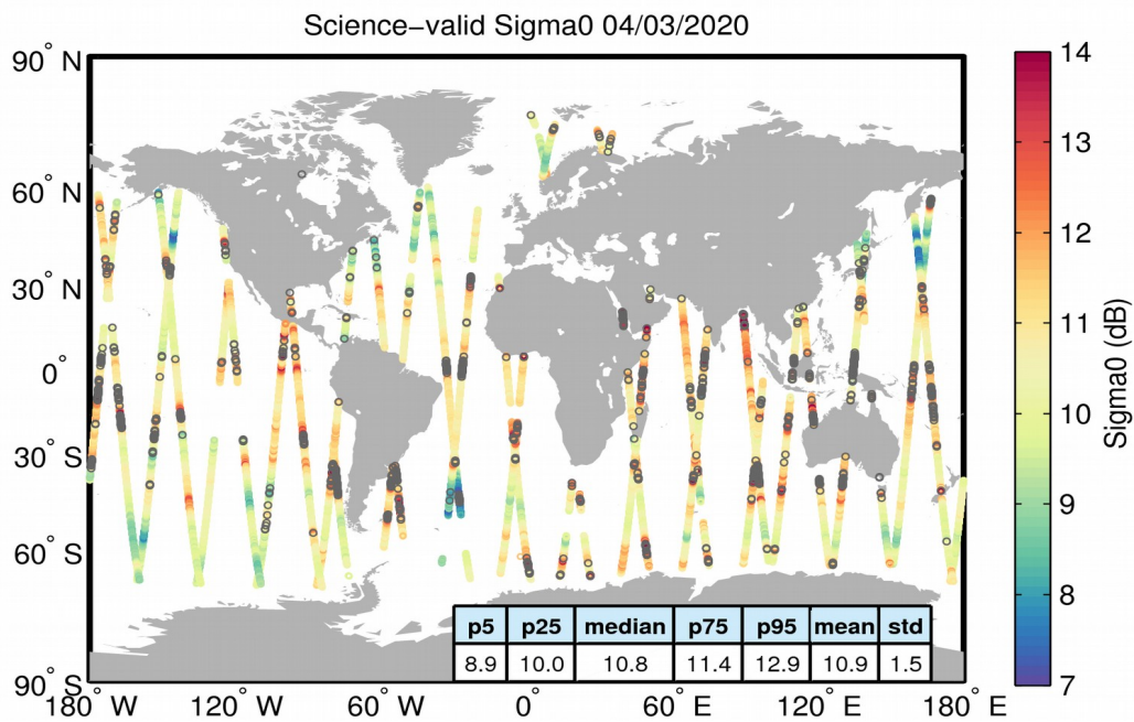
Figure 27. Geographical distribution of science-valid sigma0 data over oceans and lakes for 04/03/2020. The statistical values shown in the table refer to the sigma0 in dB and are calculated over all measurements shown in the figure. Gray circles denote records that have been rejected based on the editing criteria described in Table 4.
