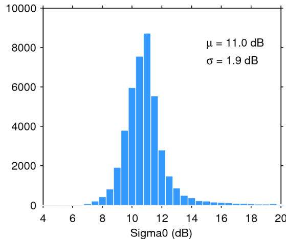
Figure 25. Histogram of flag-valid sigma0 over oceans and lakes for 04/03/2020. The mean ( \mu ) and standard deviation ( \sigma ) are also shown. Note that values outside [4 20] dB are excluded from the histogram for the sake of readability but not from the computation of \mu and \sigma .
