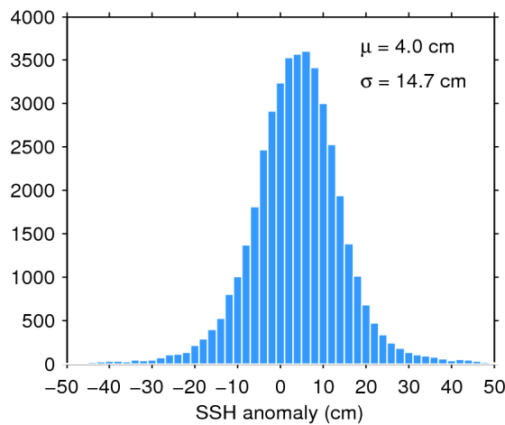
Figure 7. Histogram of flag-valid SSH anomaly over oceans and lakes for 04/03/2020. The mean ( \mu ) and standard deviation ( \sigma ) are also shown. Note that values outside [-50\ 50] cm are excluded from the histogram for the sake of readability but not from the computation of \mu and \sigma .
