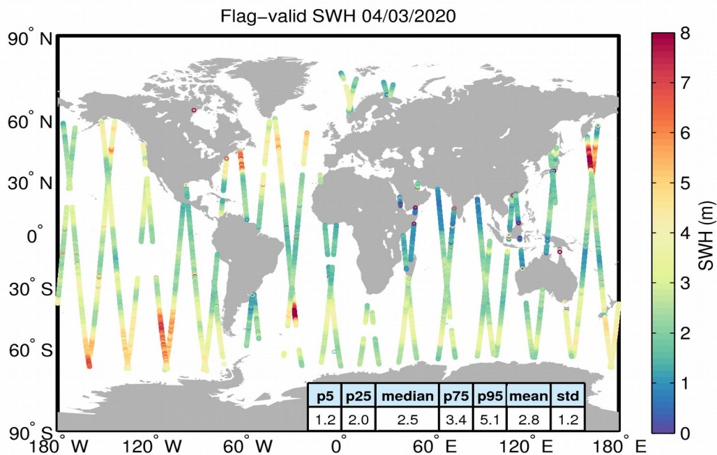
Figure 15. Geographical distribution of flag-valid SWH data over oceans and lakes for 04/03/2020. The statistical values shown in the table refer to the SWH in m and are calculated over all measurements shown in the figure.
