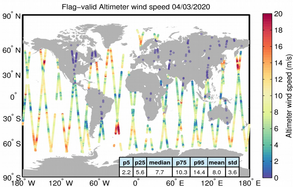
Figure 31. Geographical distribution of flag-valid wind data over oceans and lakes for 04/03/2020. The statistical values shown in the table refer to the wind in m/s and are calculated over all measurements shown in the figure.
