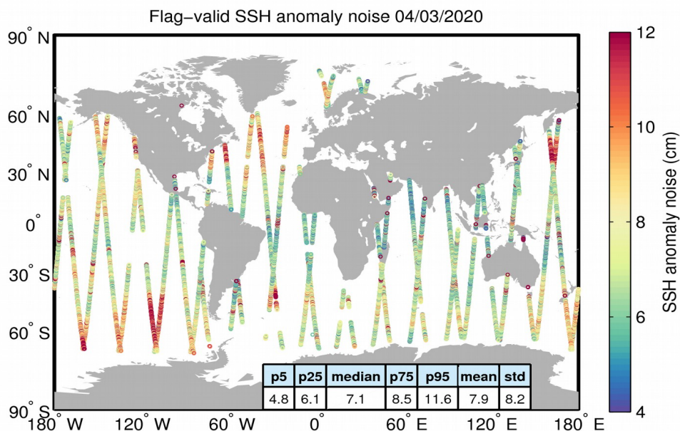
Figure 8. Geographical distribution of flag-valid 20-Hz SSH anomaly measurement noise over oceans and lakes for 04/03/2020. The statistical values shown in the table refer to the SSH anomaly noise and are calculated over all measurements shown in the figure.
