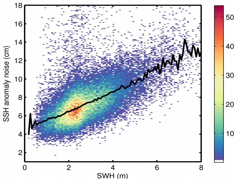
Figure 9. 2D histogram showing flag-valid SSH anomaly noise as a function of SWH for 04/03/2020. The black line denotes the median SSH anomaly noise as a function of SWH.
