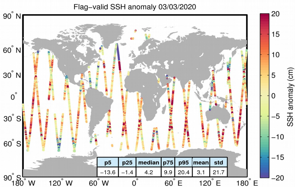
Figure 5. Geographical distribution of flag-valid 1-Hz SSH anomaly data over oceans and lakes for 03/03/2020. The statistical values shown in the table refer to the SSH anomaly in cm and are calculated over all measurements shown in the figure.
