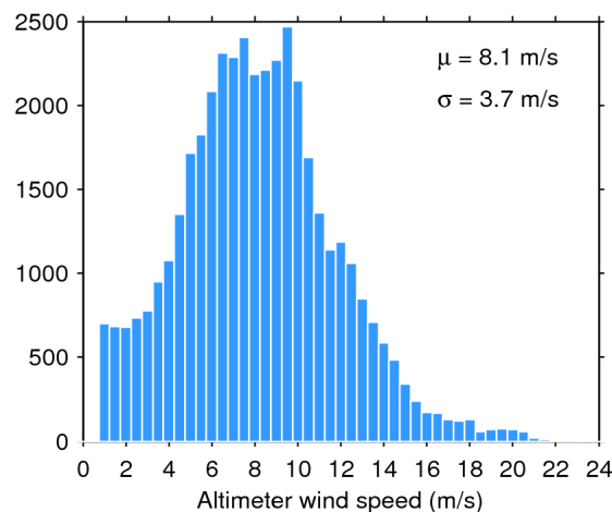
Figure 35. Histogram of science-valid wind over oceans and lakes for 03/03/2020. The mean ( \mu ) and standard deviation ( \sigma ) are also shown. Note that values larger than 24 m/s are excluded from the histogram for the sake of readability but not from the computation of \mu and \sigma .
