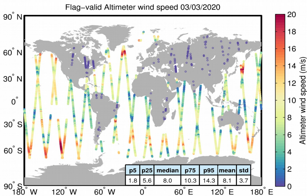
Figure 31. Geographical distribution of flag-valid wind data over oceans and lakes for 03/03/2020. The statistical values shown in the table refer to the wind in m/s and are calculated over all measurements shown in the figure.
