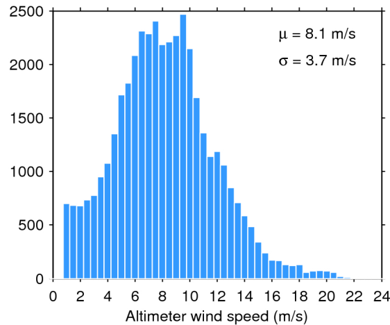
Figure 33. Histogram of flag-valid wind over oceans and lakes for 03/03/2020. The mean ( \mu ) and standard deviation ( \sigma ) are also shown. Note that values larger than 24 m/s are excluded from the histogram for the sake of readability but not from the computation of \mu and \sigma .
