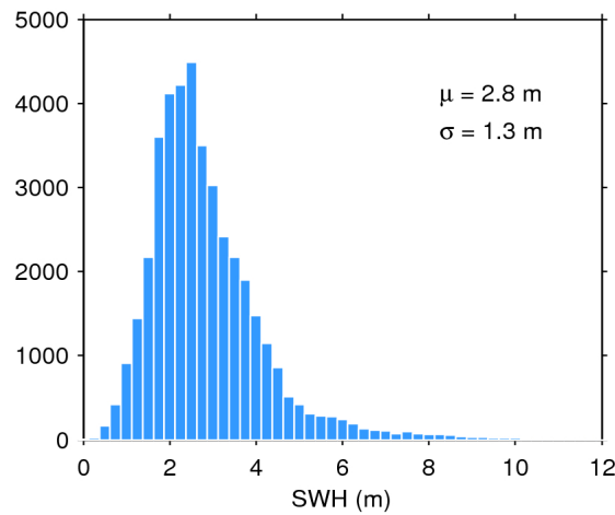
Figure 17. Histogram of flag-valid SWH over oceans and lakes for 03/03/2020. The mean ( \mu ) and standard deviation ( \sigma ) are also shown. Note that values larger than 12 m are excluded from the histogram for the sake of readability but not from the computation of \mu and \sigma .
