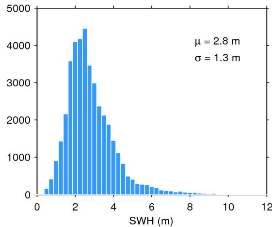
Figure 20. Histogram of science-valid SWH over oceans and lakes for 03/03/2020. The mean ( \mu ) and standard deviation ( \sigma ) are also shown. Note that values larger than 12 m are excluded from the histogram for the sake of readability but not from the computation of \mu and \sigma .
