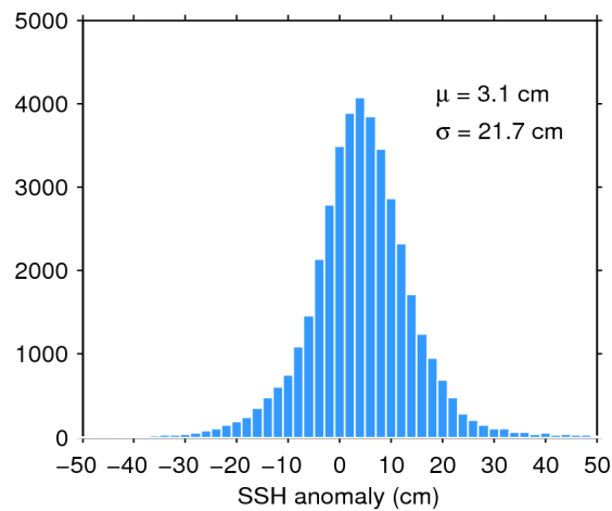
Figure 7. Histogram of flag-valid SSH anomaly over oceans and lakes for 03/03/2020. The mean ( \mu ) and standard deviation ( \sigma ) are also shown. Note that values outside [-50\ 50] cm are excluded from the histogram for the sake of readability but not from the computation of \mu and \sigma .
