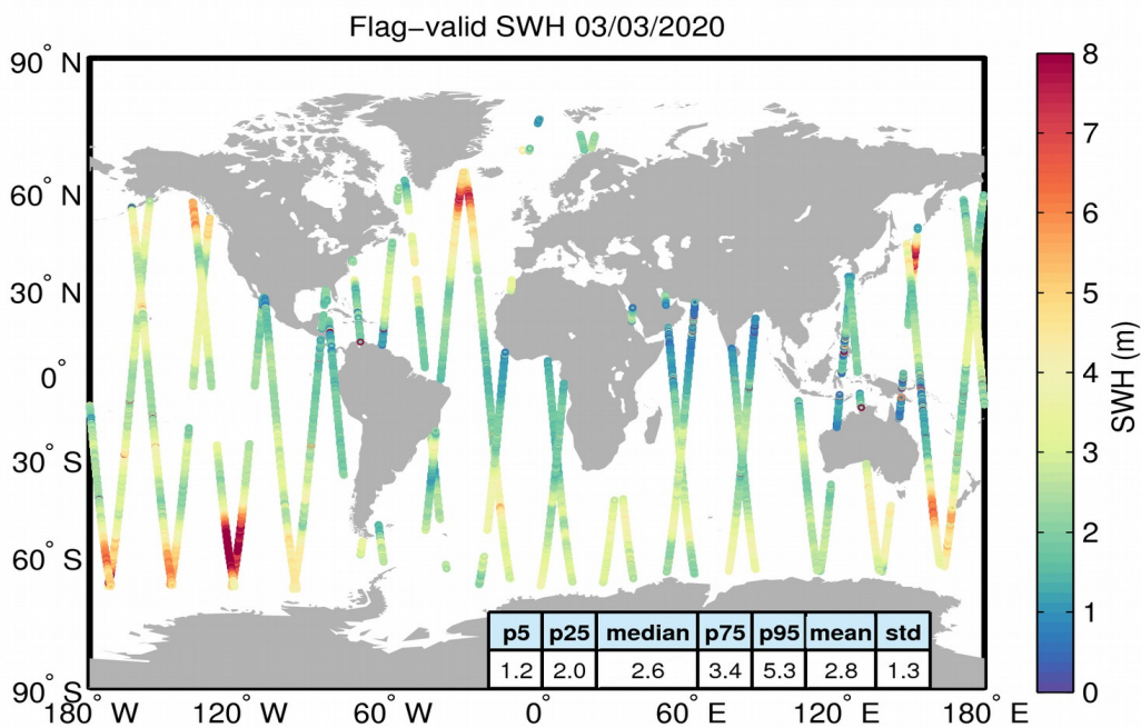
Figure 15. Geographical distribution of flag-valid SWH data over oceans and lakes for 03/03/2020. The statistical values shown in the table refer to the SWH in m and are calculated over all measurements shown in the figure.
