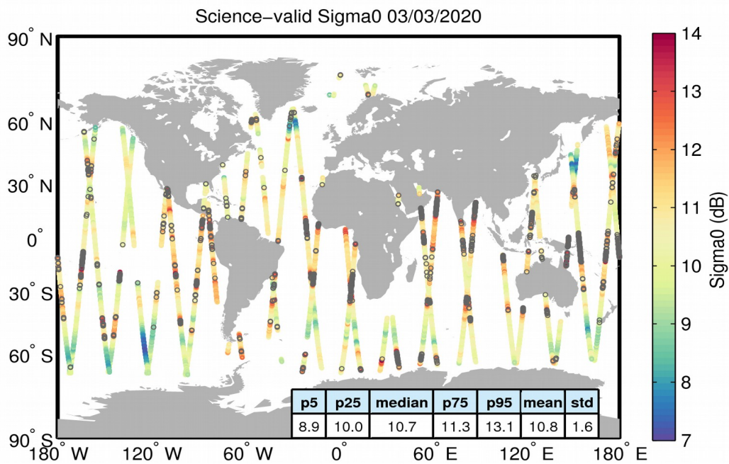
Figure 27. Geographical distribution of science-valid sigma0 data over oceans and lakes for 03/03/2020. The statistical values shown in the table refer to the sigma0 in dB and are calculated over all measurements shown in the figure. Gray circles denote records that have been rejected based on the editing criteria described in Table 4.
