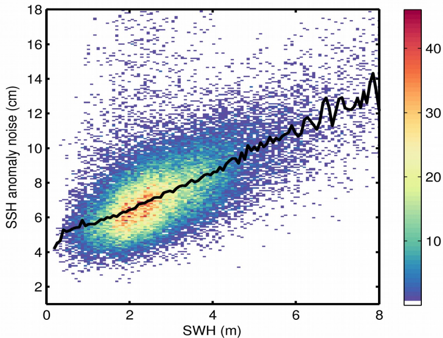
Figure 9. 2D histogram showing flag-valid SSH anomaly noise as a function of SWH for 03/03/2020. The black line denotes the median SSH anomaly noise as a function of SWH.
