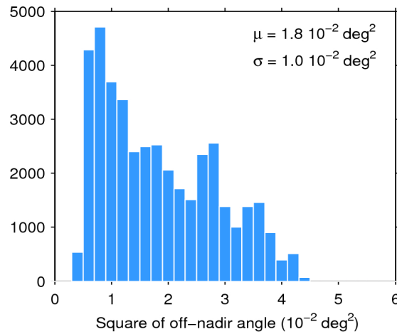
Figure 39. Histogram of flag-valid mispointing over oceans and lakes for 03/03/2020. The mean ( \mu ) and standard deviation ( \sigma ) are also shown. Note that values larger than 6 \cdot 10^{-2} \text{ deg}^2 are excluded from the histogram for the sake of readability but not from the computation of \mu and \sigma .
