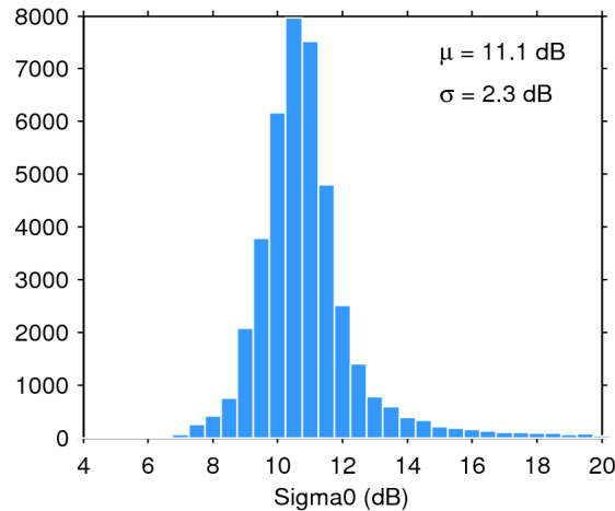
Figure 25. Histogram of flag-valid sigma0 over oceans and lakes for 03/03/2020. The mean ( \mu ) and standard deviation ( \sigma ) are also shown. Note that values outside [4 20] dB are excluded from the histogram for the sake of readability but not from the computation of \mu and \sigma .
