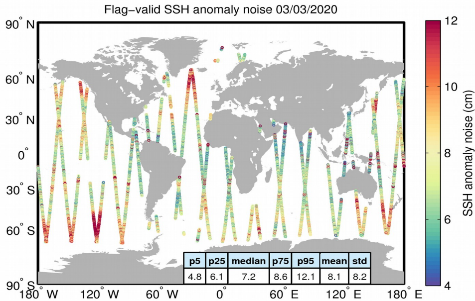
Figure 8. Geographical distribution of flag-valid 20-Hz SSH anomaly measurement noise over oceans and lakes for 03/03/2020. The statistical values shown in the table refer to the SSH anomaly noise and are calculated over all measurements shown in the figure.
