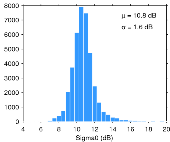
Figure 28. Histogram of science-valid sigma0 over oceans and lakes for 03/03/2020. The mean ( \mu ) and standard deviation ( \sigma ) are also shown. Note that values outside [4 20] dB are excluded from the histogram for the sake of readability but not from the computation of \mu and \sigma .
