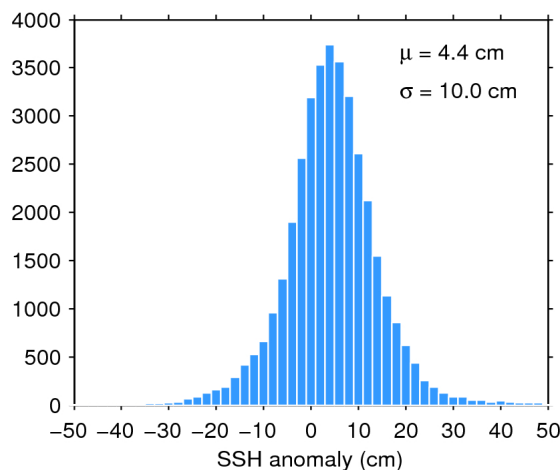
Figure 11. Histogram of science-valid SSH anomaly over oceans and lakes for 03/03/2020. The mean ( \mu ) and standard deviation ( \sigma ) are also shown. Note that values outside [-50 50] cm are excluded from the histogram for the sake of readability but not from the computation of \mu and \sigma .
