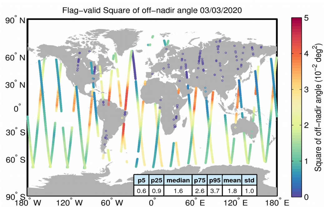
Figure 37. Geographical distribution of flag-valid mispointing data over oceans and lakes for 03/03/2020. The statistical values shown in the table refer to the mispointing in 10^{-2} \text{ deg}^2 and are calculated over all measurements shown in the figure.
