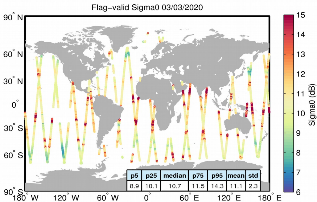
Figure 23. Geographical distribution of flag-valid sigma0 data over oceans and lakes for 03/03/2020. The statistical values shown in the table refer to the sigma0 in dB and are calculated over all measurements shown in the figure.
