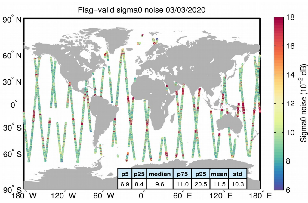
Figure 26. Geographical distribution of flag-valid 20-Hz sigma0 measurement noise over oceans and lakes for 03/03/2020. The statistical values shown in the table refer to the sigma0 noise and are calculated over all measurements shown in the figure.
