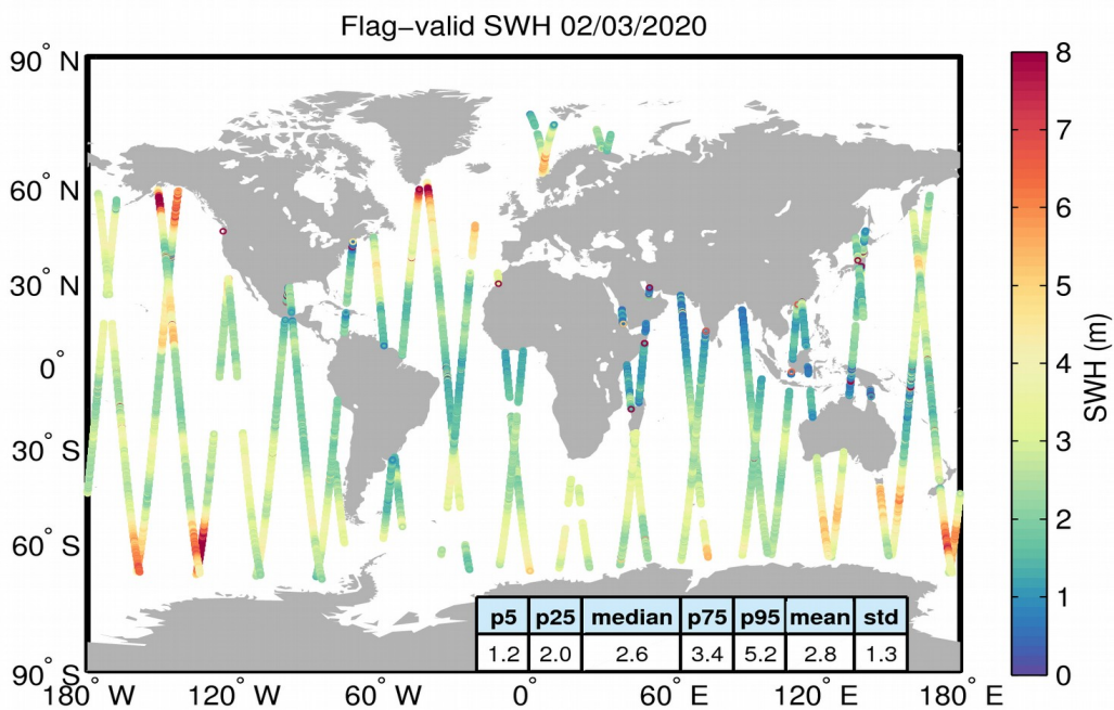
Figure 15. Geographical distribution of flag-valid SWH data over oceans and lakes for 02/03/2020. The statistical values shown in the table refer to the SWH in m and are calculated over all measurements shown in the figure.
