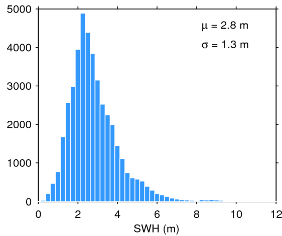
Figure 17. Histogram of flag-valid SWH over oceans and lakes for 02/03/2020. The mean ( \mu ) and standard deviation ( \sigma ) are also shown. Note that values larger than 12 m are excluded from the histogram for the sake of readability but not from the computation of \mu and \sigma .
