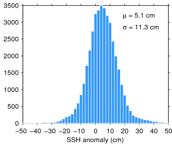
Figure 11. Histogram of science-valid SSH anomaly over oceans and lakes for 02/03/2020. The mean ( \mu ) and standard deviation ( \sigma ) are also shown. Note that values outside [-50 50] cm are excluded from the histogram for the sake of readability but not from the computation of \mu and \sigma .
