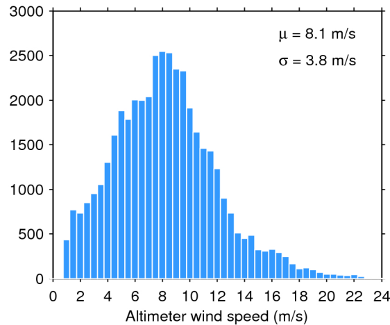
Figure 33. Histogram of flag-valid wind over oceans and lakes for 02/03/2020. The mean ( \mu ) and standard deviation ( \sigma ) are also shown. Note that values larger than 24 m/s are excluded from the histogram for the sake of readability but not from the computation of \mu and \sigma .
