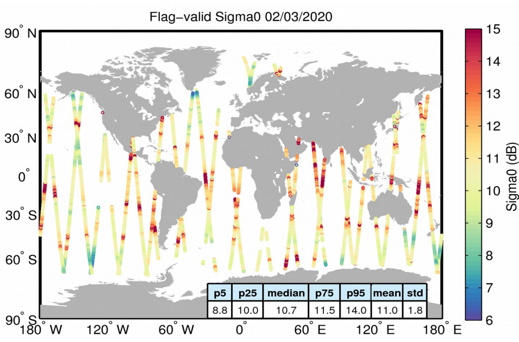
Figure 23. Geographical distribution of flag-valid sigma0 data over oceans and lakes for 02/03/2020. The statistical values shown in the table refer to the sigma0 in dB and are calculated over all measurements shown in the figure.
