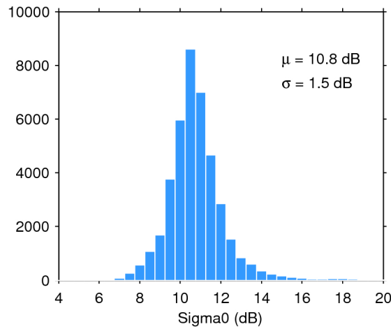
Figure 28. Histogram of science-valid sigma0 over oceans and lakes for 02/03/2020. The mean ( \mu ) and standard deviation ( \sigma ) are also shown. Note that values outside [4 20] dB are excluded from the histogram for the sake of readability but not from the computation of \mu and \sigma .
