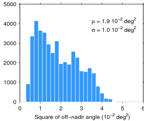
Figure 39. Histogram of flag-valid mispointing over oceans and lakes for 02/03/2020. The mean ( \mu ) and standard deviation ( \sigma ) are also shown. Note that values larger than 6 \cdot 10^{-2} \text{ deg}^2 are excluded from the histogram for the sake of readability but not from the computation of \mu and \sigma .
