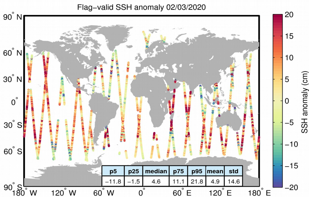
Figure 5. Geographical distribution of flag-valid 1-Hz SSH anomaly data over oceans and lakes for 02/03/2020. The statistical values shown in the table refer to the SSH anomaly in cm and are calculated over all measurements shown in the figure.
