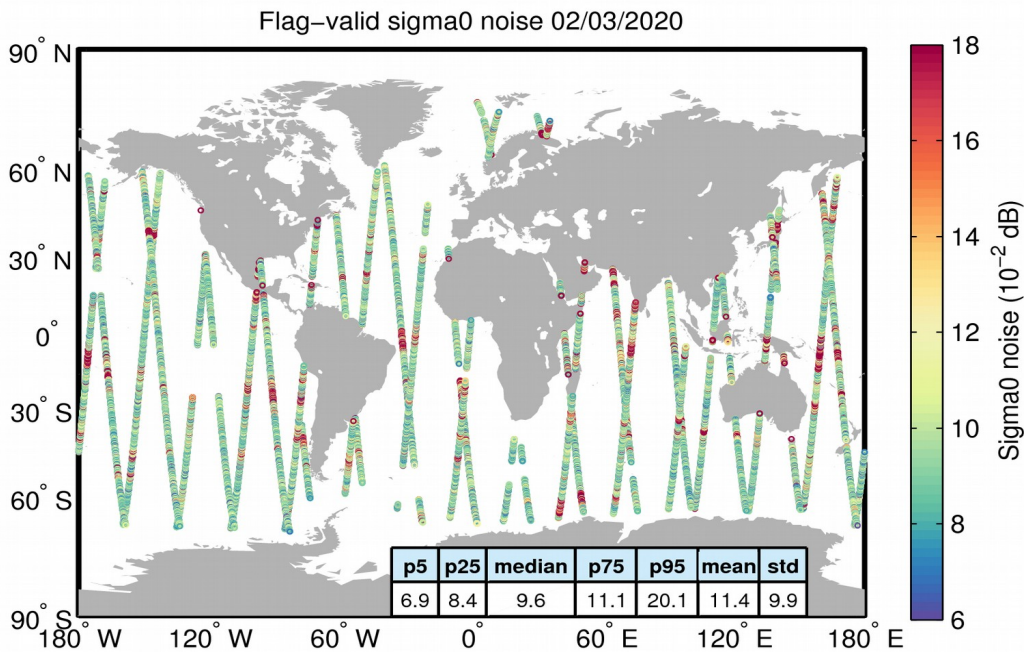
Figure 26. Geographical distribution of flag-valid 20-Hz sigma0 measurement noise over oceans and lakes for 02/03/2020. The statistical values shown in the table refer to the sigma0 noise and are calculated over all measurements shown in the figure.
