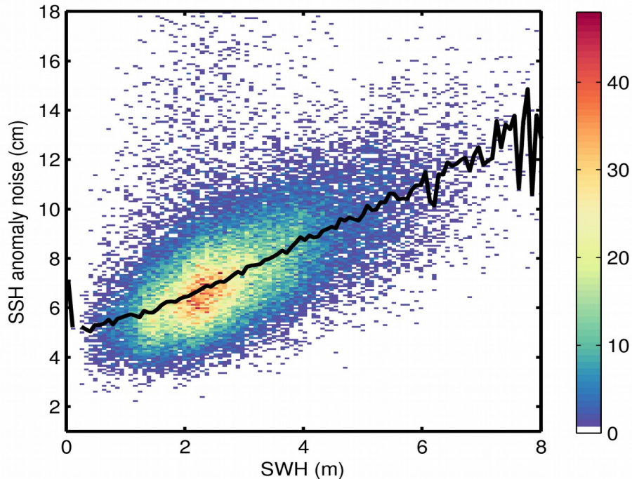
Figure 9. 2D histogram showing flag-valid SSH anomaly noise as a function of SWH for 02/03/2020. The black line denotes the median SSH anomaly noise as a function of SWH.
