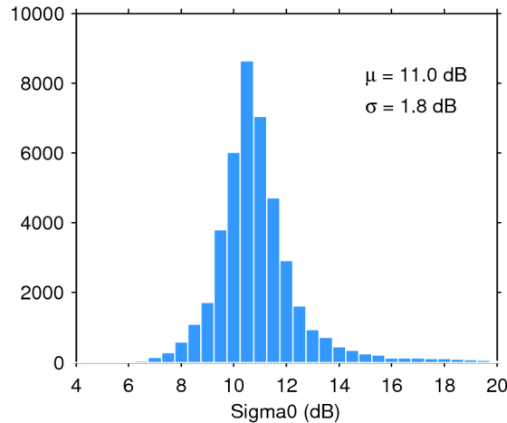
Figure 25. Histogram of flag-valid sigma0 over oceans and lakes for 02/03/2020. The mean ( \mu ) and standard deviation ( \sigma ) are also shown. Note that values outside [4 20] dB are excluded from the histogram for the sake of readability but not from the computation of \mu and \sigma .
