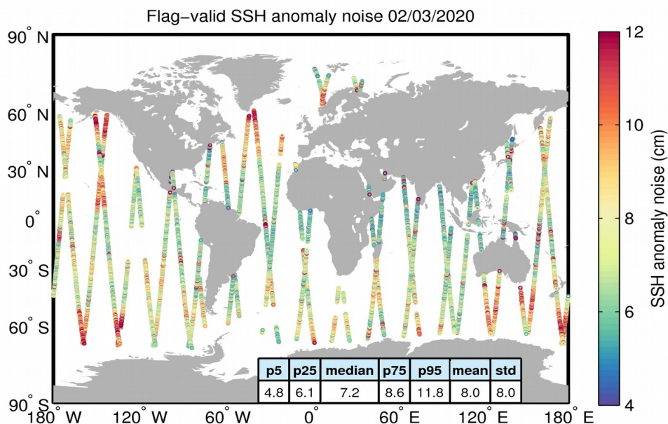
Figure 8. Geographical distribution of flag-valid 20-Hz SSH anomaly measurement noise over oceans and lakes for 02/03/2020. The statistical values shown in the table refer to the SSH anomaly noise and are calculated over all measurements shown in the figure.
