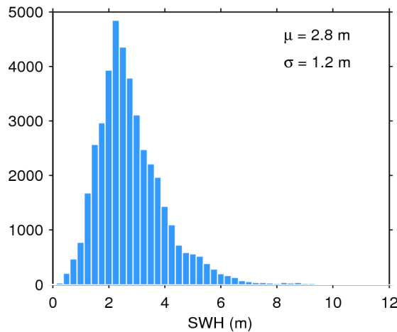
Figure 20. Histogram of science-valid SWH over oceans and lakes for 02/03/2020. The mean ( \mu ) and standard deviation ( \sigma ) are also shown. Note that values larger than 12 m are excluded from the histogram for the sake of readability but not from the computation of \mu and \sigma .
