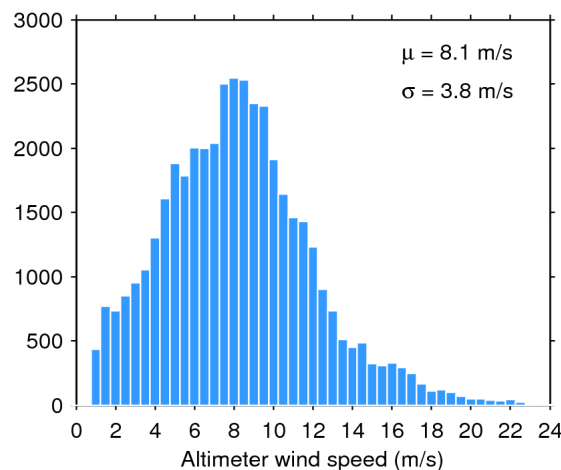
Figure 35. Histogram of science-valid wind over oceans and lakes for 02/03/2020. The mean ( \mu ) and standard deviation ( \sigma ) are also shown. Note that values larger than 24 m/s are excluded from the histogram for the sake of readability but not from the computation of \mu and \sigma .
