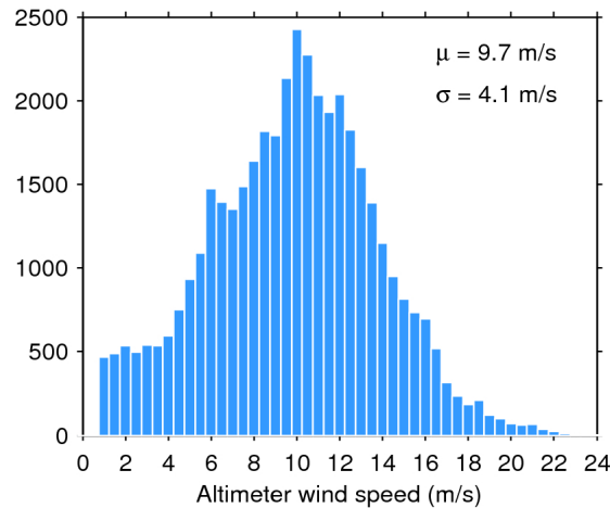
Figure 33. Histogram of flag-valid wind over oceans and lakes for 01/03/2020. The mean ( \mu ) and standard deviation ( \sigma ) are also shown. Note that values larger than 24 m/s are excluded from the histogram for the sake of readability but not from the computation of \mu and \sigma .
