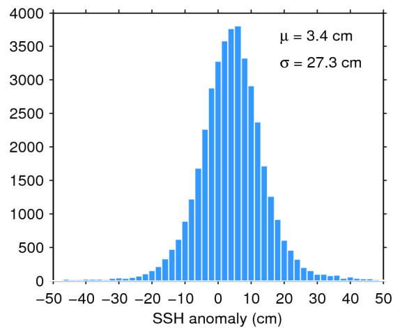
Figure 7. Histogram of flag-valid SSH anomaly over oceans and lakes for 01/03/2020. The mean ( \mu ) and standard deviation ( \sigma ) are also shown. Note that values outside [-50 \ 50] cm are excluded from the histogram for the sake of readability but not from the computation of \mu and \sigma .
