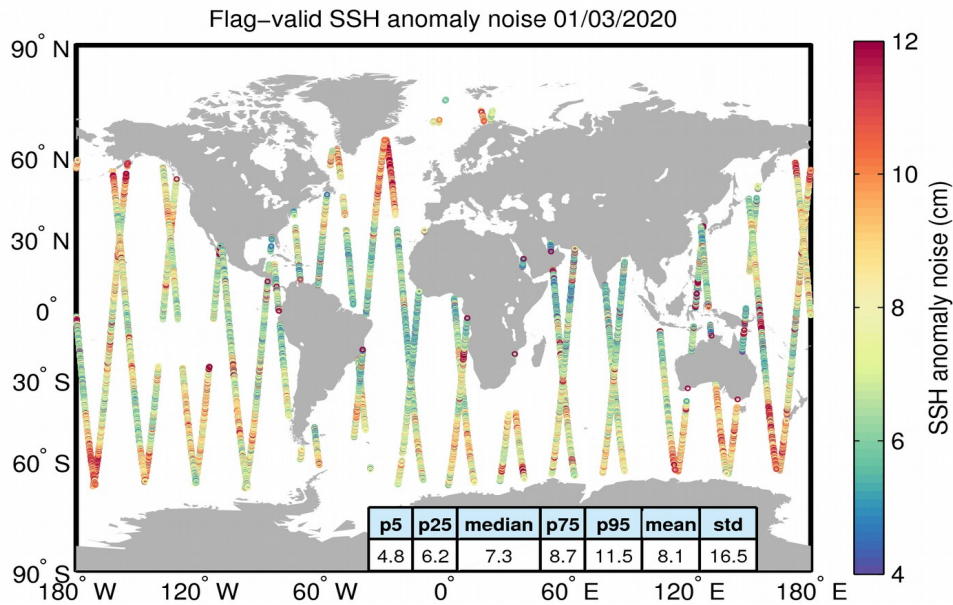
Figure 8. Geographical distribution of flag-valid 20-Hz SSH anomaly measurement noise over oceans and lakes for 01/03/2020. The statistical values shown in the table refer to the SSH anomaly noise and are calculated over all measurements shown in the figure.
