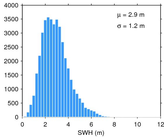
Figure 17. Histogram of flag-valid SWH over oceans and lakes for 01/03/2020. The mean ( \mu ) and standard deviation ( \sigma ) are also shown. Note that values larger than 12 m are excluded from the histogram for the sake of readability but not from the computation of \mu and \sigma .
