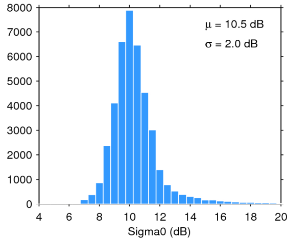
Figure 25. Histogram of flag-valid sigma0 over oceans and lakes for 01/03/2020. The mean ( \mu ) and standard deviation ( \sigma ) are also shown. Note that values outside [4 20] dB are excluded from the histogram for the sake of readability but not from the computation of \mu and \sigma .
