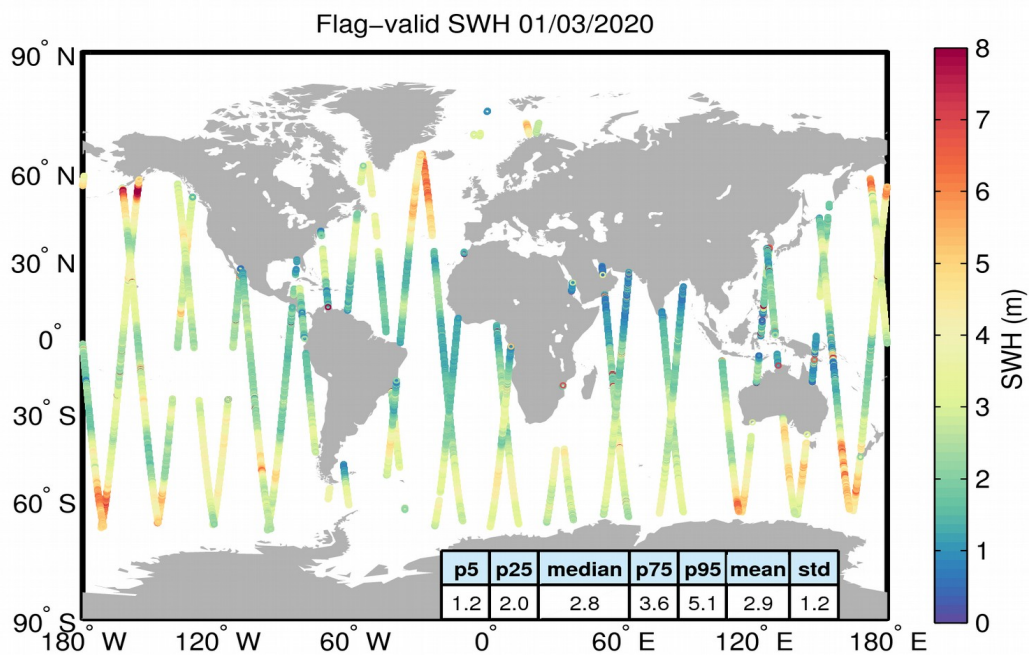
Figure 15. Geographical distribution of flag-valid SWH data over oceans and lakes for 01/03/2020. The statistical values shown in the table refer to the SWH in m and are calculated over all measurements shown in the figure.
