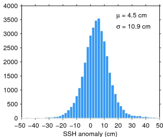
Figure 11. Histogram of science-valid SSH anomaly over oceans and lakes for 01/03/2020. The mean ( \mu ) and standard deviation ( \sigma ) are also shown. Note that values outside [-50 50] cm are excluded from the histogram for the sake of readability but not from the computation of \mu and \sigma .
