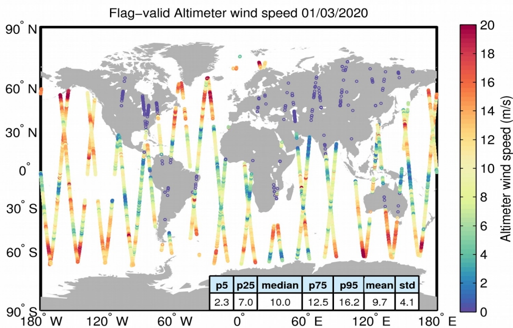
Figure 31. Geographical distribution of flag-valid wind data over oceans and lakes for 01/03/2020. The statistical values shown in the table refer to the wind in m/s and are calculated over all measurements shown in the figure.
