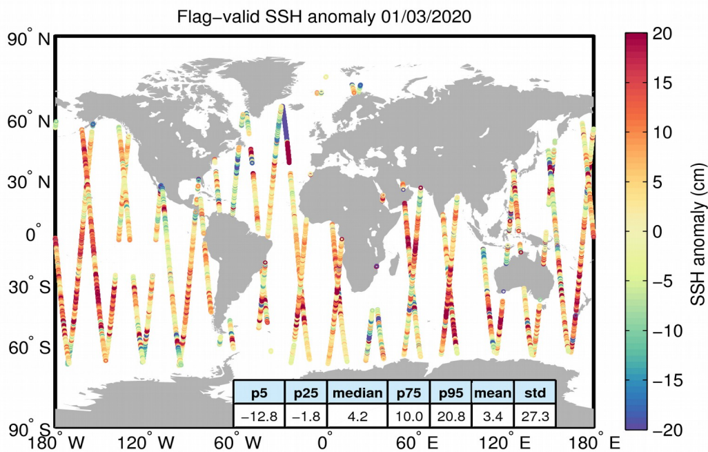
Figure 5. Geographical distribution of flag-valid 1-Hz SSH anomaly data over oceans and lakes for 01/03/2020. The statistical values shown in the table refer to the SSH anomaly in cm and are calculated over all measurements shown in the figure.
