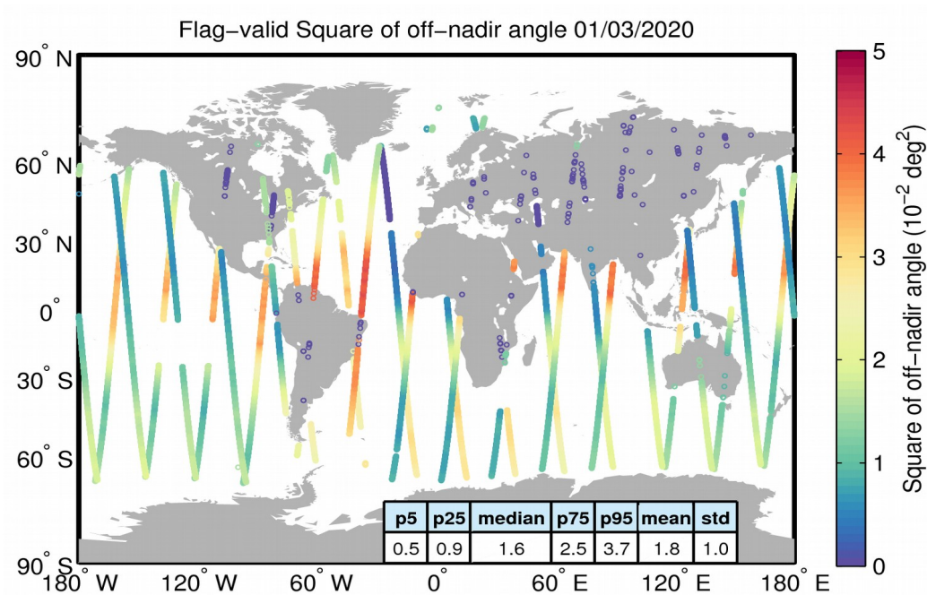
Figure 37. Geographical distribution of flag-valid mispointing data over oceans and lakes for 01/03/2020. The statistical values shown in the table refer to the mispointing in 10^{-2} \text{ deg}^2 and are calculated over all measurements shown in the figure.
