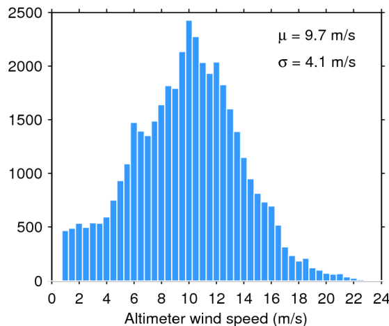
Figure 35. Histogram of science-valid wind over oceans and lakes for 01/03/2020. The mean ( \mu ) and standard deviation ( \sigma ) are also shown. Note that values larger than 24 m/s are excluded from the histogram for the sake of readability but not from the computation of \mu and \sigma .
