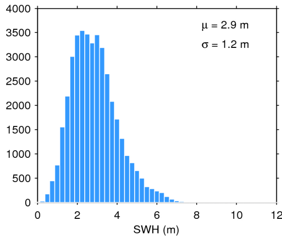
Figure 20. Histogram of science-valid SWH over oceans and lakes for 01/03/2020. The mean ( \mu ) and standard deviation ( \sigma ) are also shown. Note that values larger than 12 m are excluded from the histogram for the sake of readability but not from the computation of \mu and \sigma .
