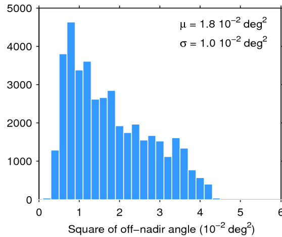
Figure 39. Histogram of flag-valid mispointing over oceans and lakes for 01/03/2020. The mean ( \mu ) and standard deviation ( \sigma ) are also shown. Note that values larger than 6 \cdot 10^{-2} \text{ deg}^2 are excluded from the histogram for the sake of readability but not from the computation of \mu and \sigma .
