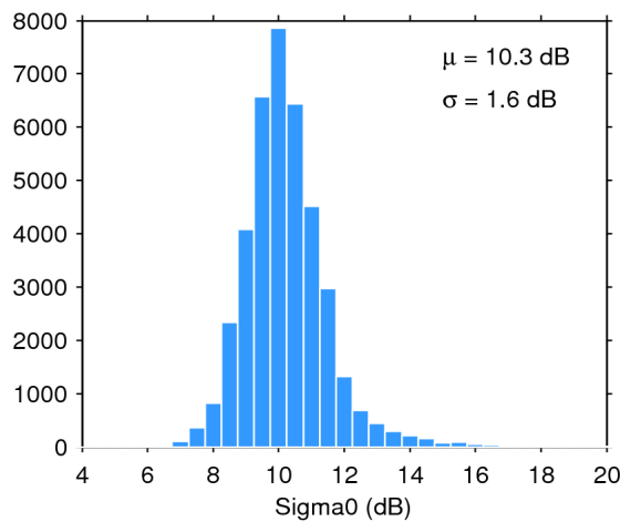
Figure 28. Histogram of science-valid sigma0 over oceans and lakes for 01/03/2020. The mean ( \mu ) and standard deviation ( \sigma ) are also shown. Note that values outside [4 20] dB are excluded from the histogram for the sake of readability but not from the computation of \mu and \sigma .
