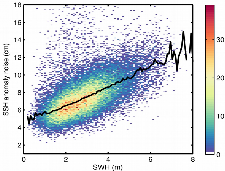
Figure 9. 2D histogram showing flag-valid SSH anomaly noise as a function of SWH for 01/03/2020. The black line denotes the median SSH anomaly noise as a function of SWH.
