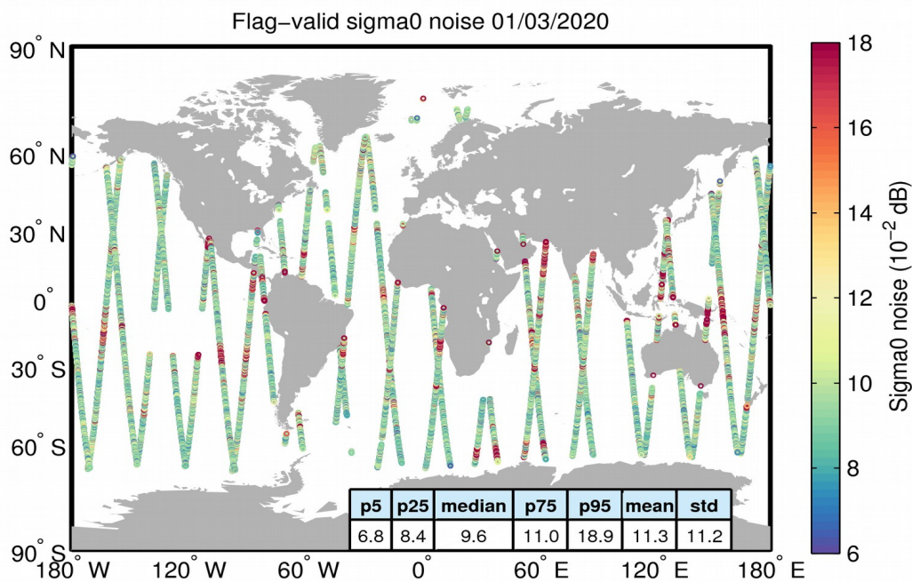
Figure 26. Geographical distribution of flag-valid 20-Hz sigma0 measurement noise over oceans and lakes for 01/03/2020. The statistical values shown in the table refer to the sigma0 noise and are calculated over all measurements shown in the figure.
