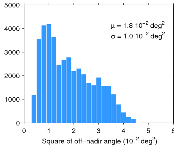
Figure 39. Histogram of flag-valid mispointing over oceans and lakes for 29/02/2020. The mean ( \mu ) and standard deviation ( \sigma ) are also shown. Note that values larger than 6 \cdot 10^{-2} \text{ deg}^2 are excluded from the histogram for the sake of readability but not from the computation of \mu and \sigma .
