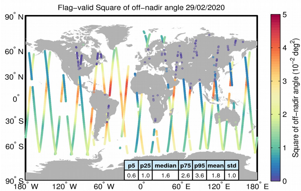
Figure 37. Geographical distribution of flag-valid mispointing data over oceans and lakes for 29/02/2020. The statistical values shown in the table refer to the mispointing in 10^{-2} \text{ deg}^2 and are calculated over all measurements shown in the figure.
