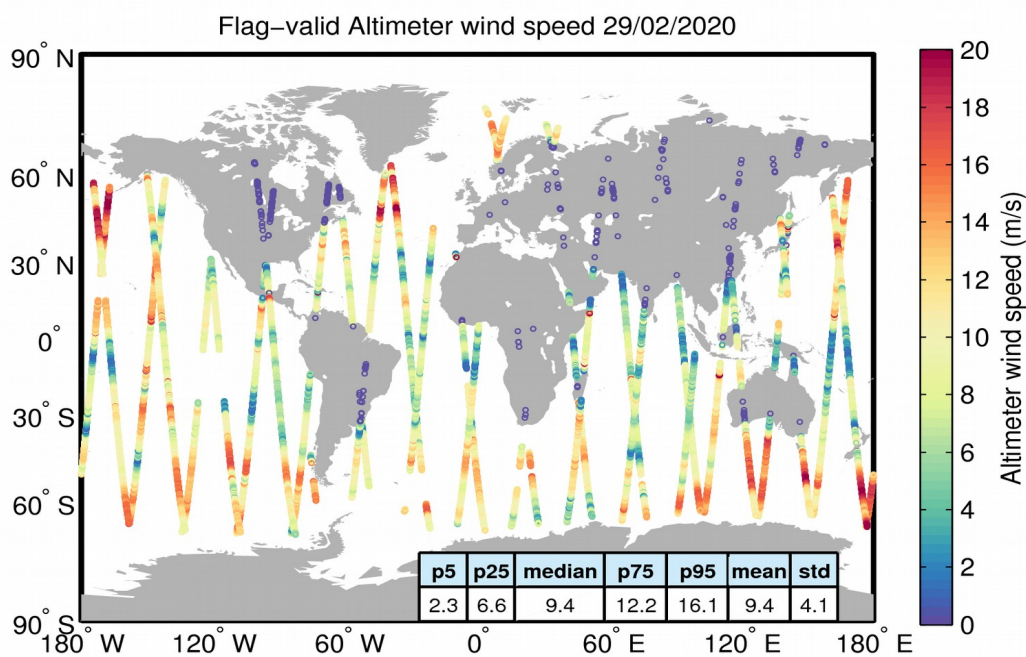
Figure 31. Geographical distribution of flag-valid wind data over oceans and lakes for 29/02/2020. The statistical values shown in the table refer to the wind in m/s and are calculated over all measurements shown in the figure.
