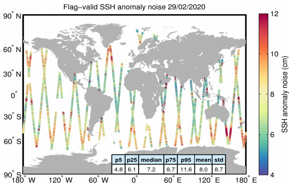
Figure 8. Geographical distribution of flag-valid 20-Hz SSH anomaly measurement noise over oceans and lakes for 29/02/2020. The statistical values shown in the table refer to the SSH anomaly noise and are calculated over all measurements shown in the figure.
