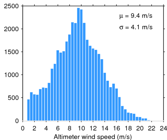
Figure 35. Histogram of science-valid wind over oceans and lakes for 29/02/2020. The mean ( \mu ) and standard deviation ( \sigma ) are also shown. Note that values larger than 24 m/s are excluded from the histogram for the sake of readability but not from the computation of \mu and \sigma .
