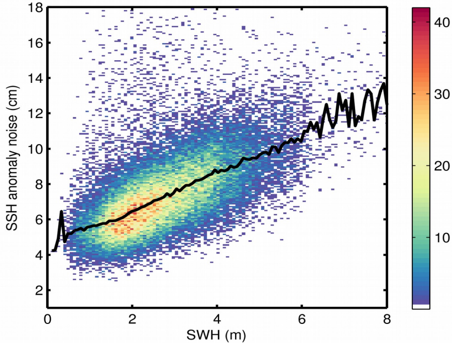
Figure 9. 2D histogram showing flag-valid SSH anomaly noise as a function of SWH for 29/02/2020. The black line denotes the median SSH anomaly noise as a function of SWH.
