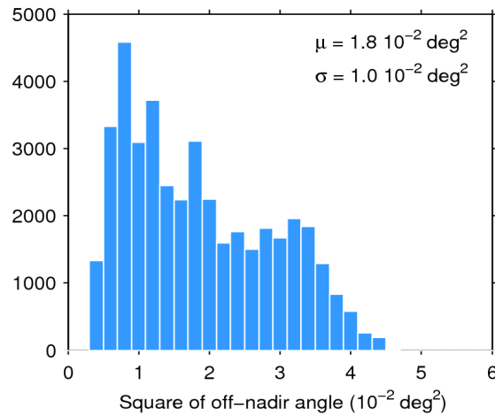
Figure 39. Histogram of flag-valid mispointing over oceans and lakes for 28/02/2020. The mean ( \mu ) and standard deviation ( \sigma ) are also shown. Note that values larger than 6 \cdot 10^{-2} \text{ deg}^2 are excluded from the histogram for the sake of readability but not from the computation of \mu and \sigma .
