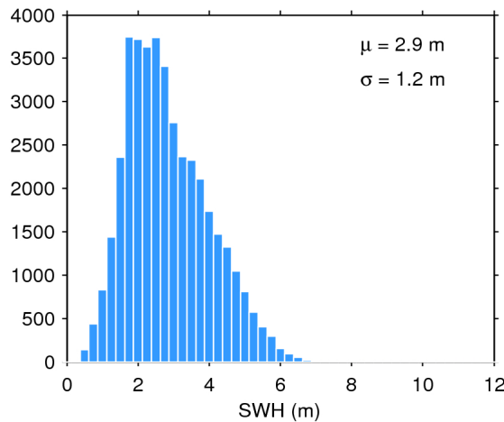
Figure 20. Histogram of science-valid SWH over oceans and lakes for 28/02/2020. The mean ( \mu ) and standard deviation ( \sigma ) are also shown. Note that values larger than 12 m are excluded from the histogram for the sake of readability but not from the computation of \mu and \sigma .
