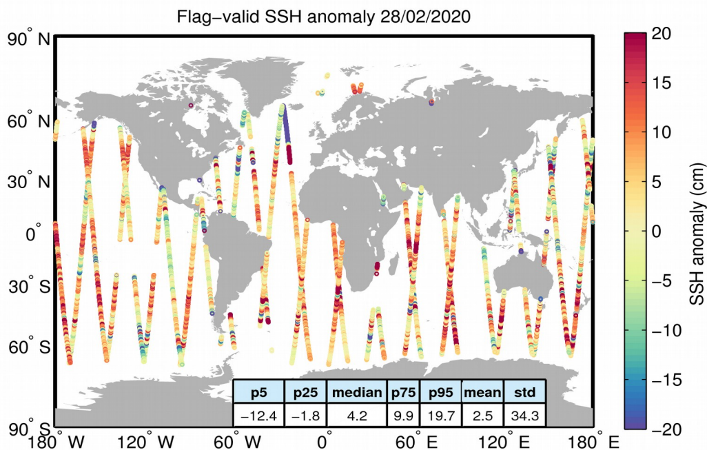
Figure 5. Geographical distribution of flag-valid 1-Hz SSH anomaly data over oceans and lakes for 28/02/2020. The statistical values shown in the table refer to the SSH anomaly in cm and are calculated over all measurements shown in the figure.
