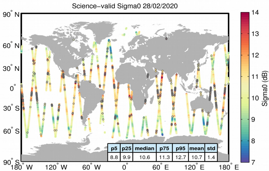
Figure 27. Geographical distribution of science-valid sigma0 data over oceans and lakes for 28/02/2020. The statistical values shown in the table refer to the sigma0 in dB and are calculated over all measurements shown in the figure. Gray circles denote records that have been rejected based on the editing criteria described in Table 4.
