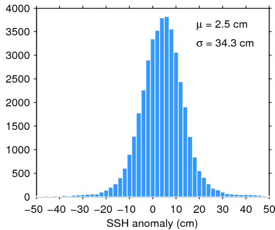
Figure 7. Histogram of flag-valid SSH anomaly over oceans and lakes for 28/02/2020. The mean ( \mu ) and standard deviation ( \sigma ) are also shown. Note that values outside [-50 50] cm are excluded from the histogram for the sake of readability but not from the computation of \mu and \sigma .
