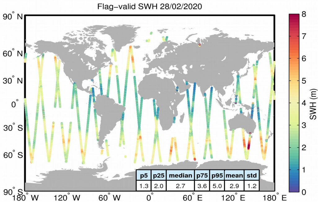
Figure 15. Geographical distribution of flag-valid SWH data over oceans and lakes for 28/02/2020. The statistical values shown in the table refer to the SWH in m and are calculated over all measurements shown in the figure.
