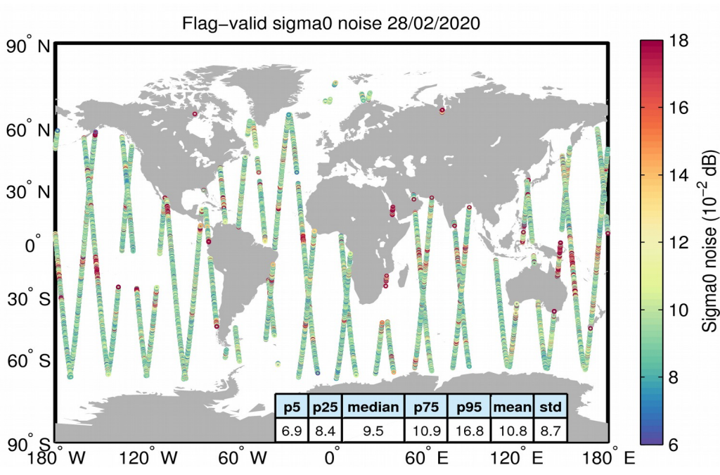
Figure 26. Geographical distribution of flag-valid 20-Hz sigma0 measurement noise over oceans and lakes for 28/02/2020. The statistical values shown in the table refer to the sigma0 noise and are calculated over all measurements shown in the figure.
