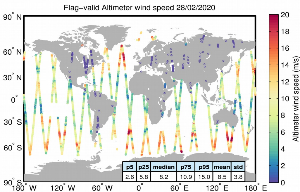
Figure 31. Geographical distribution of flag-valid wind data over oceans and lakes for 28/02/2020. The statistical values shown in the table refer to the wind in m/s and are calculated over all measurements shown in the figure.
