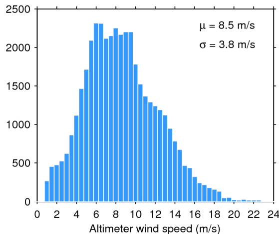
Figure 35. Histogram of science-valid wind over oceans and lakes for 28/02/2020. The mean ( \mu ) and standard deviation ( \sigma ) are also shown. Note that values larger than 24 m/s are excluded from the histogram for the sake of readability but not from the computation of \mu and \sigma .
