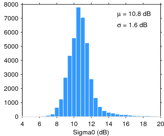
Figure 25. Histogram of flag-valid sigma0 over oceans and lakes for 28/02/2020. The mean ( \mu ) and standard deviation ( \sigma ) are also shown. Note that values outside [4 20] dB are excluded from the histogram for the sake of readability but not from the computation of \mu and \sigma .
