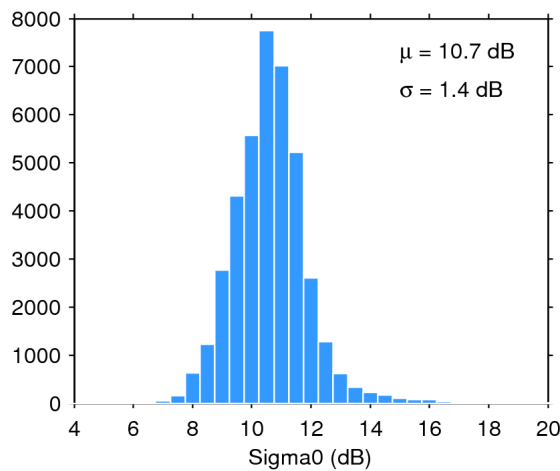
Figure 28. Histogram of science-valid sigma0 over oceans and lakes for 28/02/2020. The mean ( \mu ) and standard deviation ( \sigma ) are also shown. Note that values outside [4 20] dB are excluded from the histogram for the sake of readability but not from the computation of \mu and \sigma .
