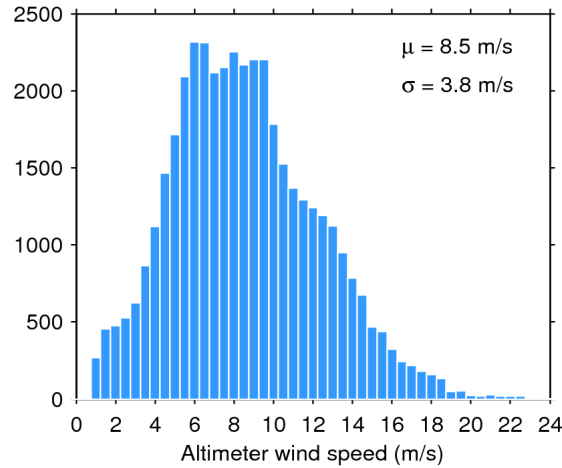
Figure 33. Histogram of flag-valid wind over oceans and lakes for 28/02/2020. The mean ( \mu ) and standard deviation ( \sigma ) are also shown. Note that values larger than 24 m/s are excluded from the histogram for the sake of readability but not from the computation of \mu and \sigma .
