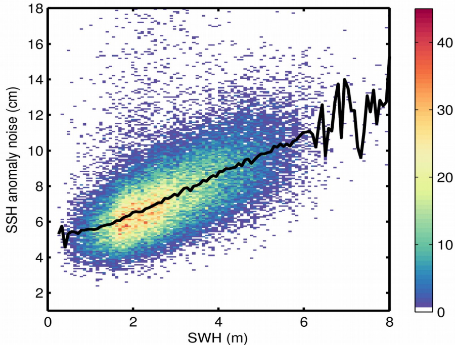
Figure 9. 2D histogram showing flag-valid SSH anomaly noise as a function of SWH for 28/02/2020. The black line denotes the median SSH anomaly noise as a function of SWH.
