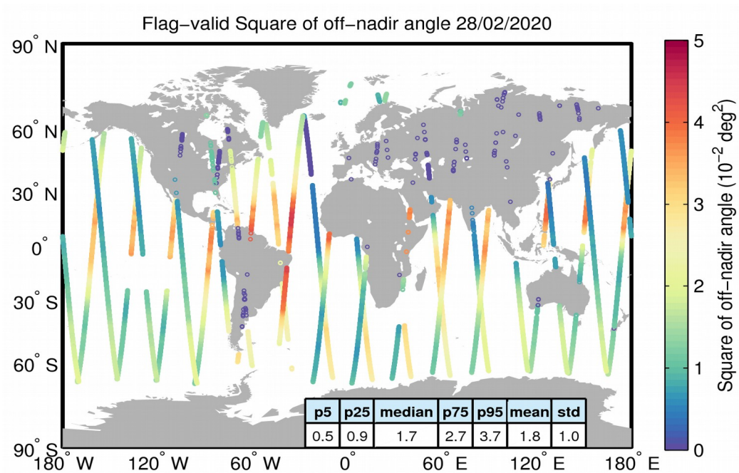
Figure 37. Geographical distribution of flag-valid mispointing data over oceans and lakes for 28/02/2020. The statistical values shown in the table refer to the mispointing in 10^{-2} \text{ deg}^2 and are calculated over all measurements shown in the figure.
