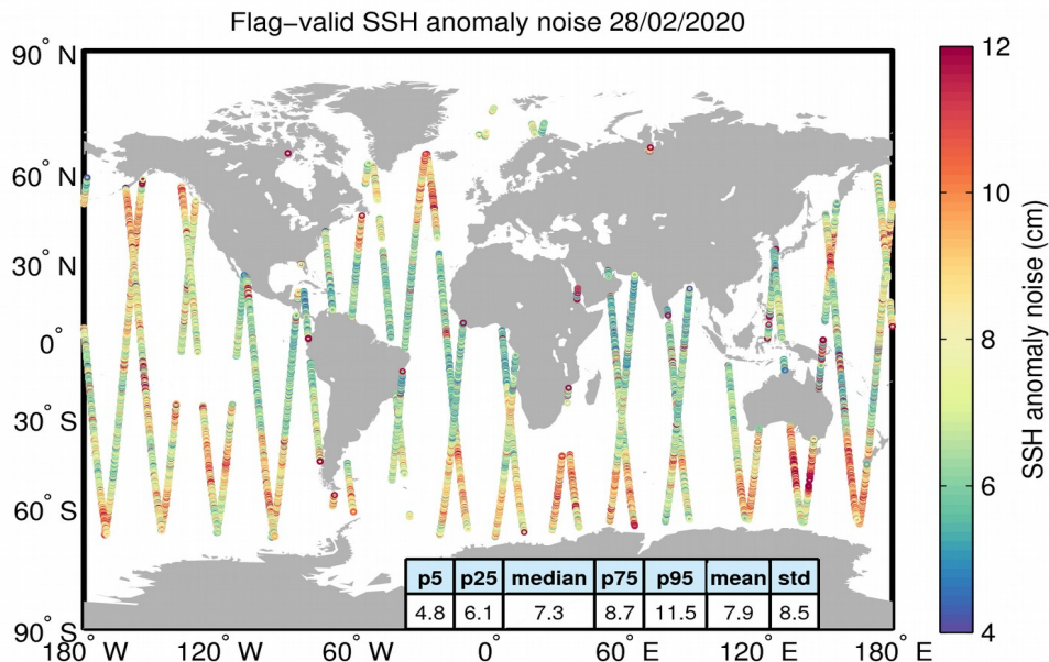
Figure 8. Geographical distribution of flag-valid 20-Hz SSH anomaly measurement noise over oceans and lakes for 28/02/2020. The statistical values shown in the table refer to the SSH anomaly noise and are calculated over all measurements shown in the figure.
