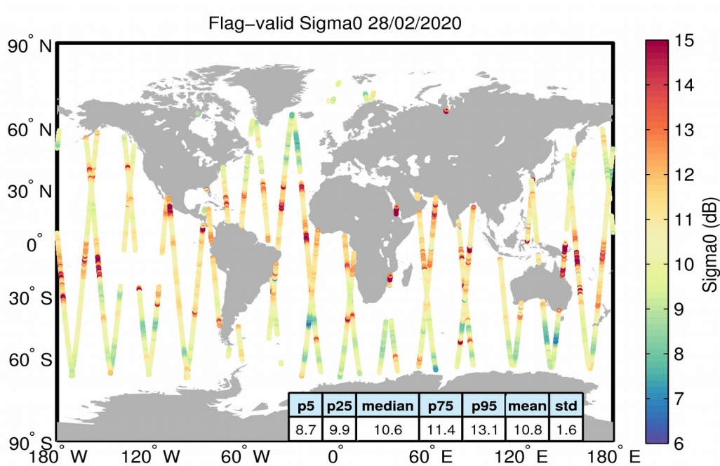
Figure 23. Geographical distribution of flag-valid sigma0 data over oceans and lakes for 28/02/2020. The statistical values shown in the table refer to the sigma0 in dB and are calculated over all measurements shown in the figure.
