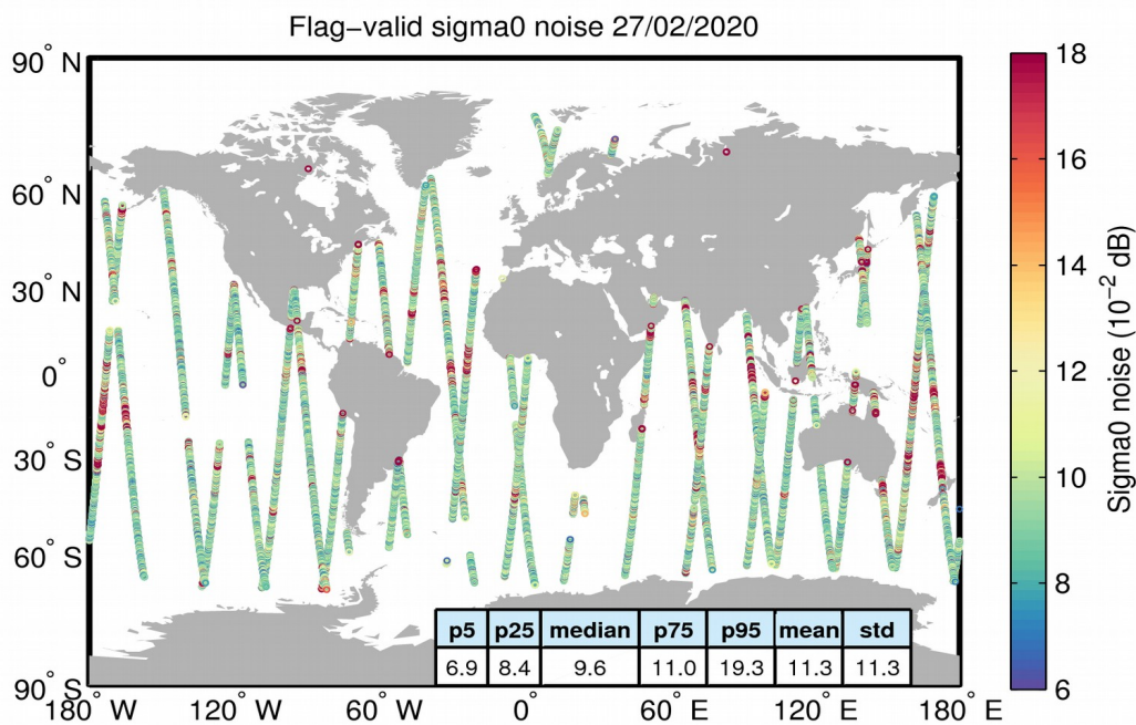
Figure 26. Geographical distribution of flag-valid 20-Hz sigma0 measurement noise over oceans and lakes for 27/02/2020. The statistical values shown in the table refer to the sigma0 noise and are calculated over all measurements shown in the figure.
