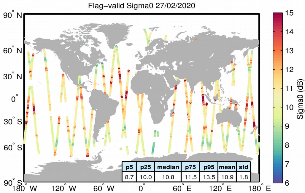
Figure 23. Geographical distribution of flag-valid sigma0 data over oceans and lakes for 27/02/2020. The statistical values shown in the table refer to the sigma0 in dB and are calculated over all measurements shown in the figure.
