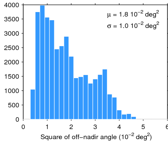
Figure 39. Histogram of flag-valid mispointing over oceans and lakes for 27/02/2020. The mean ( \mu ) and standard deviation ( \sigma ) are also shown. Note that values larger than 6 \cdot 10^{-2} \text{ deg}^2 are excluded from the histogram for the sake of readability but not from the computation of \mu and \sigma .
