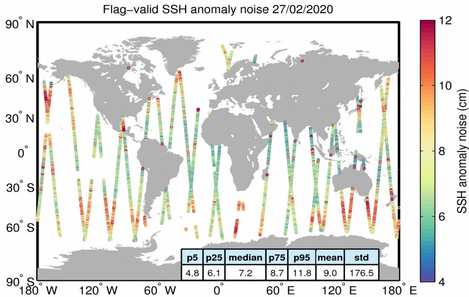
Figure 8. Geographical distribution of flag-valid 20-Hz SSH anomaly measurement noise over oceans and lakes for 27/02/2020. The statistical values shown in the table refer to the SSH anomaly noise and are calculated over all measurements shown in the figure.
