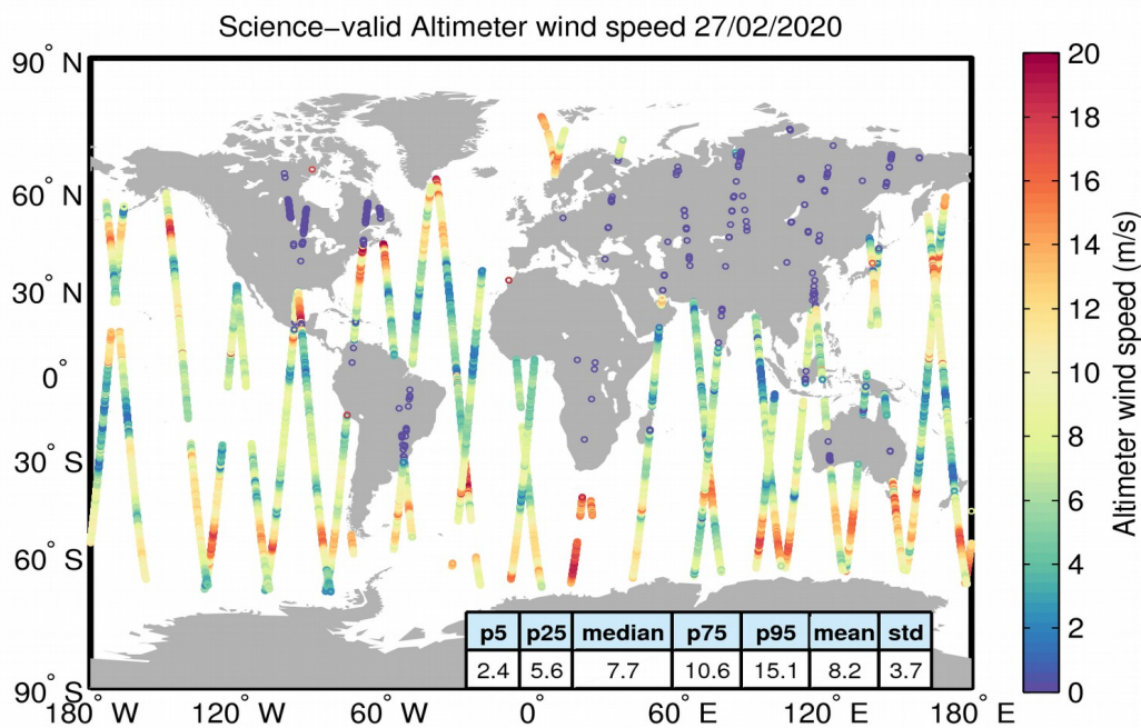
Figure 34. Geographical distribution of science-valid wind data over oceans and lakes for 27/02/2020. The statistical values shown in the table refer to the wind in m/s and are calculated over all measurements shown in the figure. Gray circles denote records that have been rejected based on the editing criteria described in Table 5.
