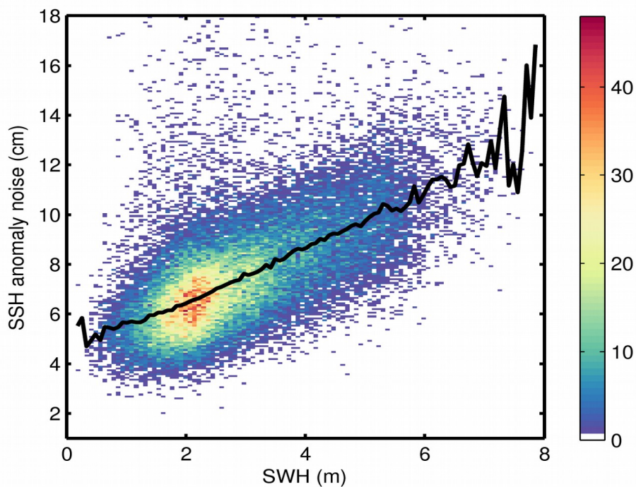
Figure 9. 2D histogram showing flag-valid SSH anomaly noise as a function of SWH for 27/02/2020. The black line denotes the median SSH anomaly noise as a function of SWH.
