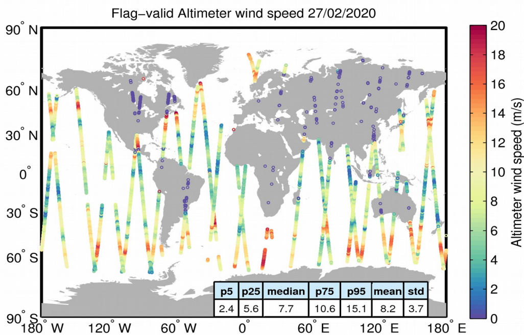
Figure 31. Geographical distribution of flag-valid wind data over oceans and lakes for 27/02/2020. The statistical values shown in the table refer to the wind in m/s and are calculated over all measurements shown in the figure.
