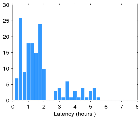
Figure 2. Histogram of the data latency for 27/02/2020. The y-axis denotes the number of files that are made available with a delay of x-hours with respect to the mean time of the records stored in the file.
