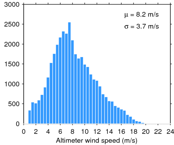
Figure 33. Histogram of flag-valid wind over oceans and lakes for 27/02/2020. The mean ( \mu ) and standard deviation ( \sigma ) are also shown. Note that values larger than 24 m/s are excluded from the histogram for the sake of readability but not from the computation of \mu and \sigma .
