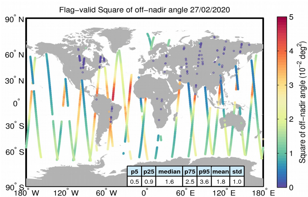
Figure 37. Geographical distribution of flag-valid mispointing data over oceans and lakes for 27/02/2020. The statistical values shown in the table refer to the mispointing in 10^{-2} \text{ deg}^2 and are calculated over all measurements shown in the figure.
