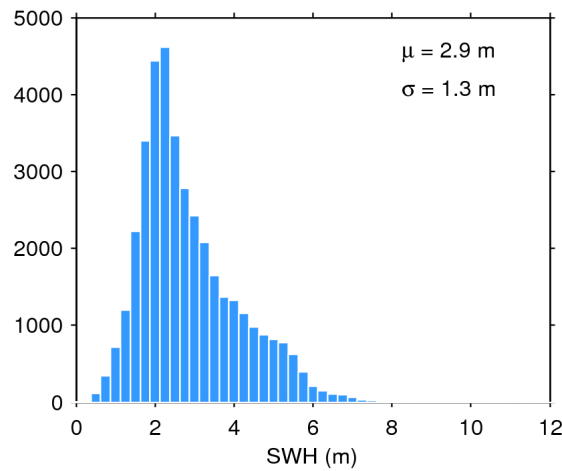
Figure 17. Histogram of flag-valid SWH over oceans and lakes for 27/02/2020. The mean ( \mu ) and standard deviation ( \sigma ) are also shown. Note that values larger than 12 m are excluded from the histogram for the sake of readability but not from the computation of \mu and \sigma .
