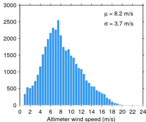
Figure 35. Histogram of science-valid wind over oceans and lakes for 27/02/2020. The mean ( \mu ) and standard deviation ( \sigma ) are also shown. Note that values larger than 24 m/s are excluded from the histogram for the sake of readability but not from the computation of \mu and \sigma .
