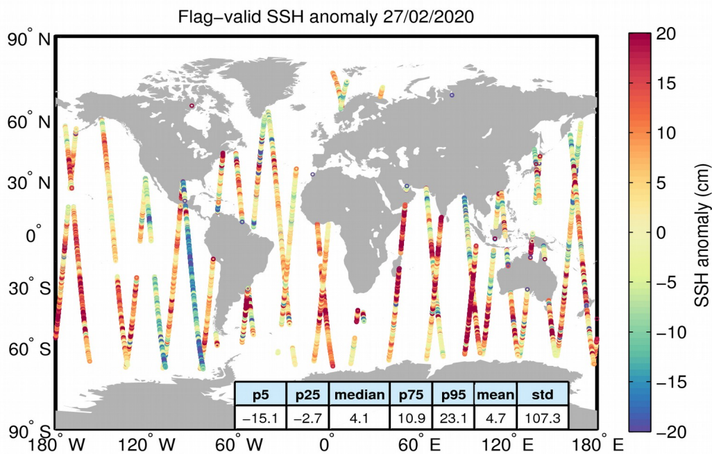
Figure 5. Geographical distribution of flag-valid 1-Hz SSH anomaly data over oceans and lakes for 27/02/2020. The statistical values shown in the table refer to the SSH anomaly in cm and are calculated over all measurements shown in the figure.
