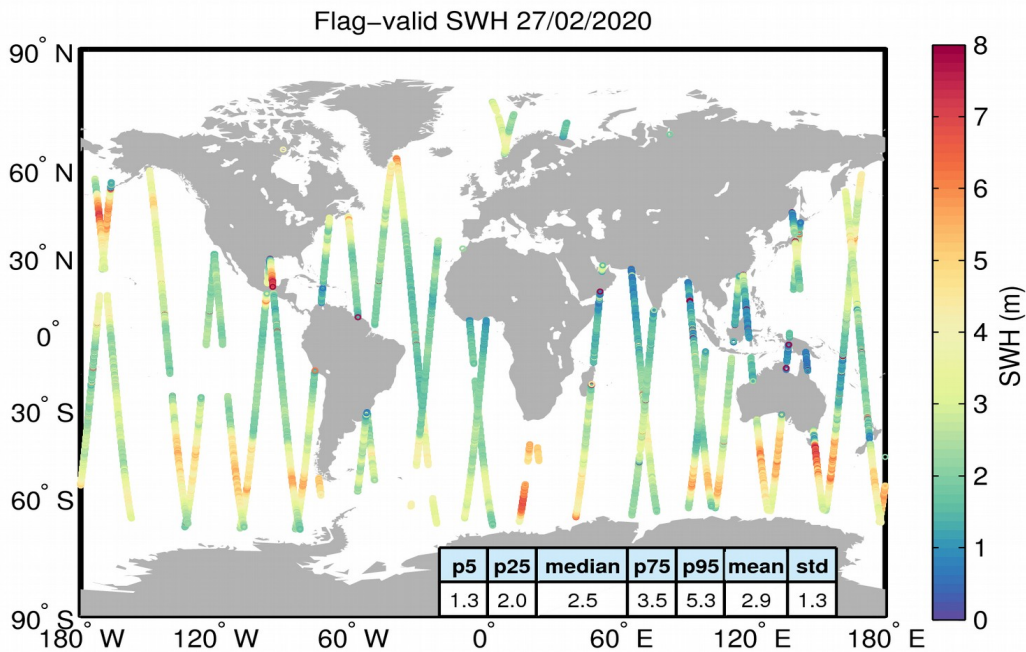
Figure 15. Geographical distribution of flag-valid SWH data over oceans and lakes for 27/02/2020. The statistical values shown in the table refer to the SWH in m and are calculated over all measurements shown in the figure.
