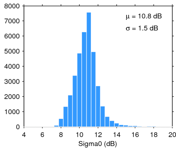
Figure 28. Histogram of science-valid sigma0 over oceans and lakes for 27/02/2020. The mean ( \mu ) and standard deviation ( \sigma ) are also shown. Note that values outside [4 20] dB are excluded from the histogram for the sake of readability but not from the computation of \mu and \sigma .
