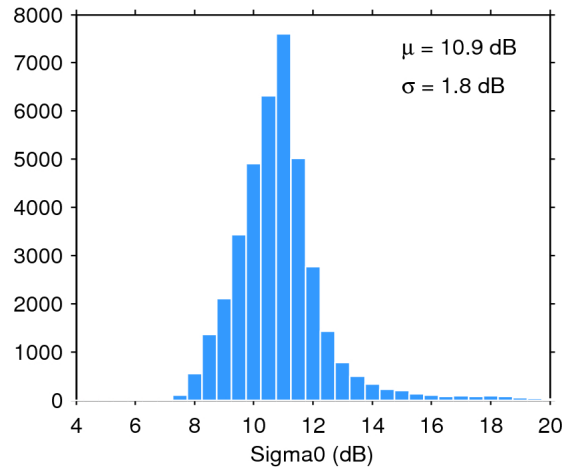
Figure 25. Histogram of flag-valid sigma0 over oceans and lakes for 27/02/2020. The mean ( \mu ) and standard deviation ( \sigma ) are also shown. Note that values outside [4 20] dB are excluded from the histogram for the sake of readability but not from the computation of \mu and \sigma .
