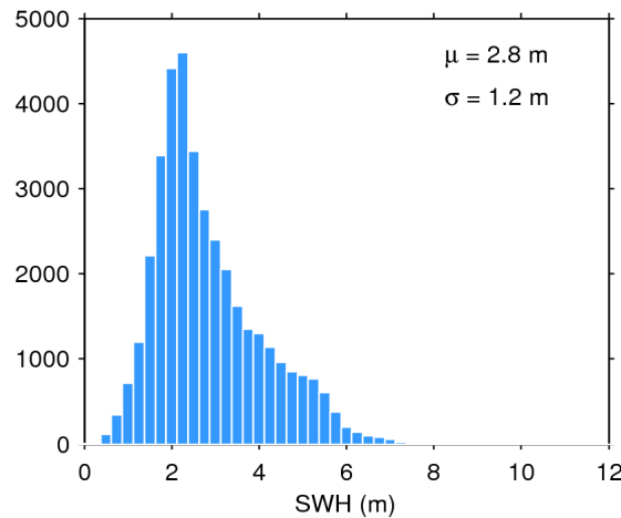
Figure 20. Histogram of science-valid SWH over oceans and lakes for 27/02/2020. The mean ( \mu ) and standard deviation ( \sigma ) are also shown. Note that values larger than 12 m are excluded from the histogram for the sake of readability but not from the computation of \mu and \sigma .
