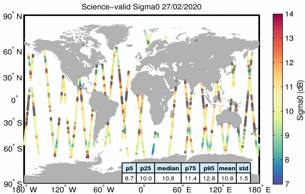
Figure 27. Geographical distribution of science-valid sigma0 data over oceans and lakes for 27/02/2020. The statistical values shown in the table refer to the sigma0 in dB and are calculated over all measurements shown in the figure. Gray circles denote records that have been rejected based on the editing criteria described in Table 4.
