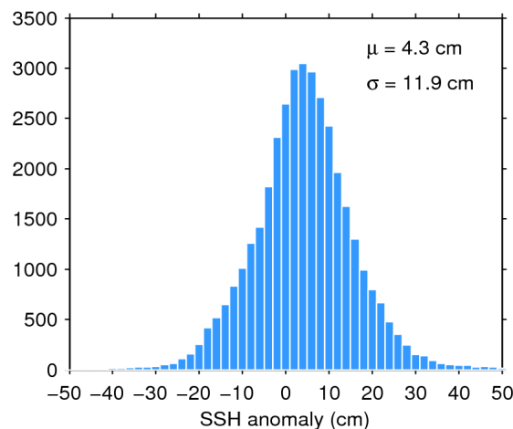
Figure 11. Histogram of science-valid SSH anomaly over oceans and lakes for 27/02/2020. The mean ( \mu ) and standard deviation ( \sigma ) are also shown. Note that values outside [-50 50] cm are excluded from the histogram for the sake of readability but not from the computation of \mu and \sigma .
