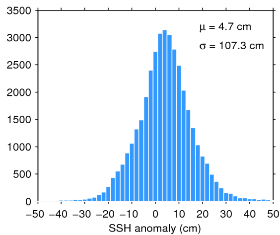
Figure 7. Histogram of flag-valid SSH anomaly over oceans and lakes for 27/02/2020. The mean ( \mu ) and standard deviation ( \sigma ) are also shown. Note that values outside [-50 50] cm are excluded from the histogram for the sake of readability but not from the computation of \mu and \sigma .
