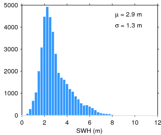
Figure 17. Histogram of flag-valid SWH over oceans and lakes for 26/02/2020. The mean ( \mu ) and standard deviation ( \sigma ) are also shown. Note that values larger than 12 m are excluded from the histogram for the sake of readability but not from the computation of \mu and \sigma .
