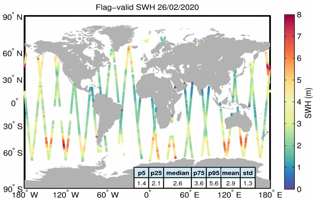
Figure 15. Geographical distribution of flag-valid SWH data over oceans and lakes for 26/02/2020. The statistical values shown in the table refer to the SWH in m and are calculated over all measurements shown in the figure.
