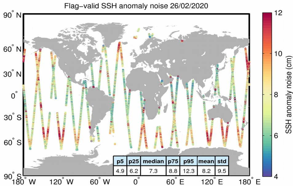
Figure 8. Geographical distribution of flag-valid 20-Hz SSH anomaly measurement noise over oceans and lakes for 26/02/2020. The statistical values shown in the table refer to the SSH anomaly noise and are calculated over all measurements shown in the figure.
