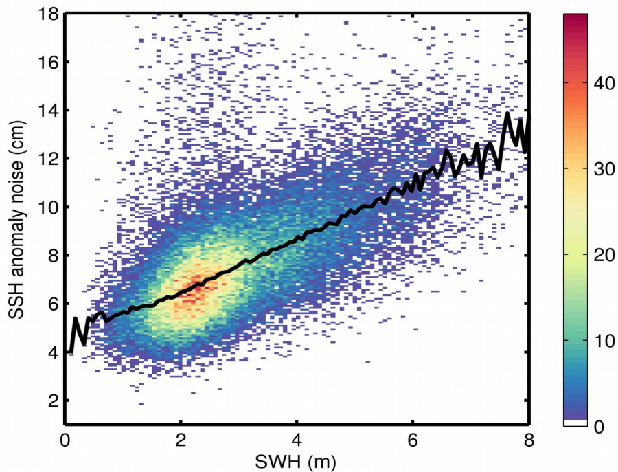
Figure 9. 2D histogram showing flag-valid SSH anomaly noise as a function of SWH for 26/02/2020. The black line denotes the median SSH anomaly noise as a function of SWH.
