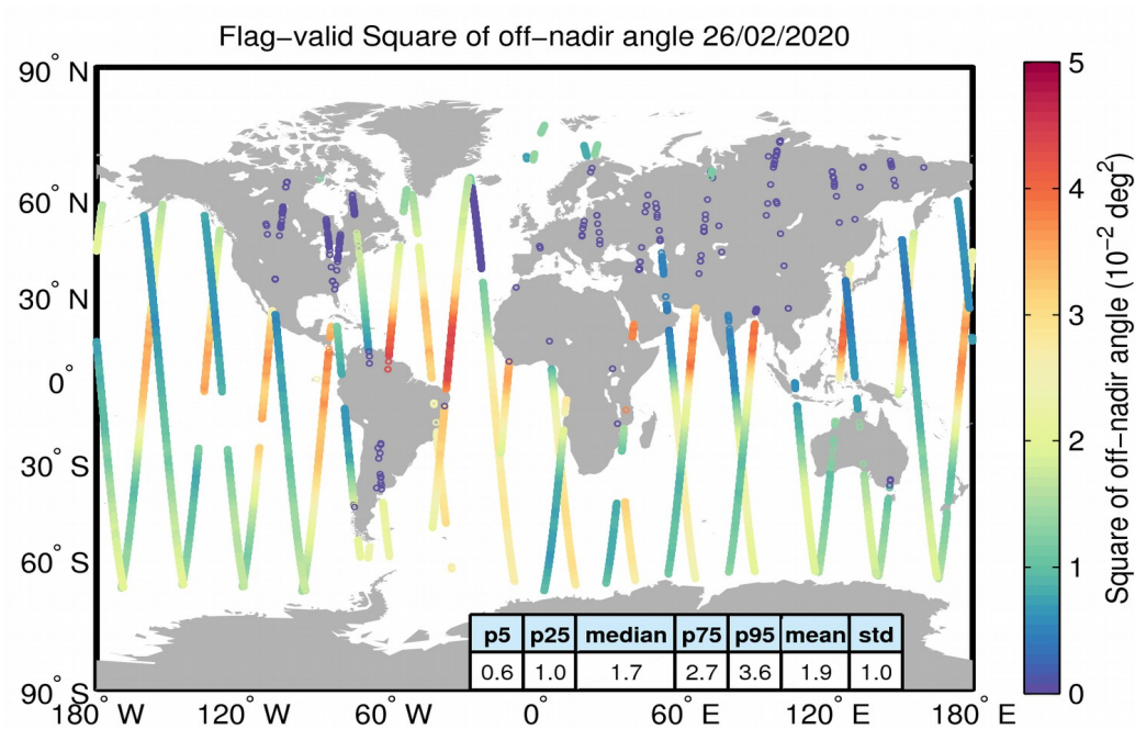
Figure 37. Geographical distribution of flag-valid mispointing data over oceans and lakes for 26/02/2020. The statistical values shown in the table refer to the mispointing in 10^{-2} \text{ deg}^2 and are calculated over all measurements shown in the figure.
