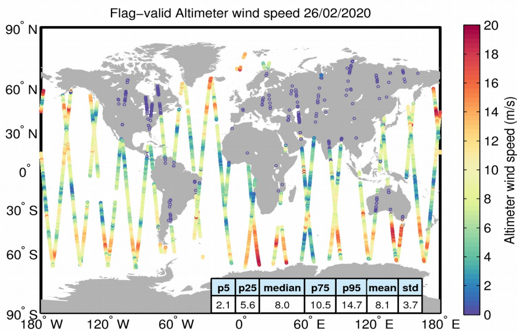
Figure 31. Geographical distribution of flag-valid wind data over oceans and lakes for 26/02/2020. The statistical values shown in the table refer to the wind in m/s and are calculated over all measurements shown in the figure.
