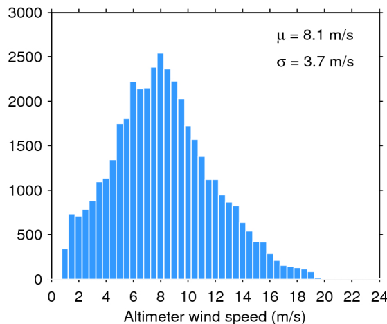
Figure 35. Histogram of science-valid wind over oceans and lakes for 26/02/2020. The mean ( \mu ) and standard deviation ( \sigma ) are also shown. Note that values larger than 24 m/s are excluded from the histogram for the sake of readability but not from the computation of \mu and \sigma .
