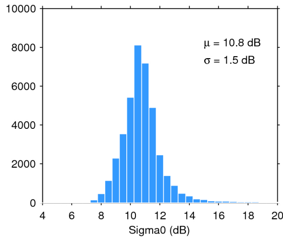
Figure 28. Histogram of science-valid sigma0 over oceans and lakes for 26/02/2020. The mean ( \mu ) and standard deviation ( \sigma ) are also shown. Note that values outside [4 20] dB are excluded from the histogram for the sake of readability but not from the computation of \mu and \sigma .
