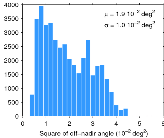
Figure 39. Histogram of flag-valid mispointing over oceans and lakes for 26/02/2020. The mean ( \mu ) and standard deviation ( \sigma ) are also shown. Note that values larger than 6 \cdot 10^{-2} \text{ deg}^2 are excluded from the histogram for the sake of readability but not from the computation of \mu and \sigma .
