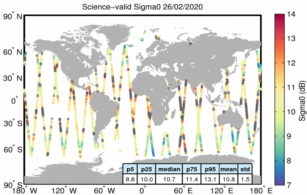
Figure 27. Geographical distribution of science-valid sigma0 data over oceans and lakes for 26/02/2020. The statistical values shown in the table refer to the sigma0 in dB and are calculated over all measurements shown in the figure. Gray circles denote records that have been rejected based on the editing criteria described in Table 4.
