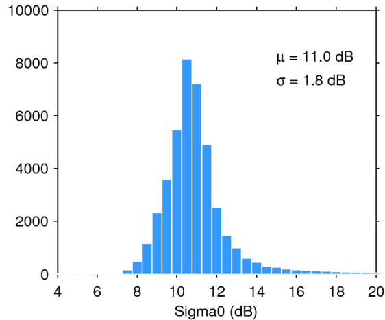
Figure 25. Histogram of flag-valid sigma0 over oceans and lakes for 26/02/2020. The mean ( \mu ) and standard deviation ( \sigma ) are also shown. Note that values outside [4 20] dB are excluded from the histogram for the sake of readability but not from the computation of \mu and \sigma .
