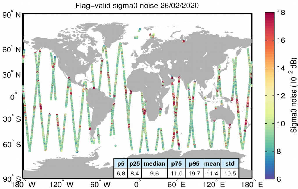
Figure 26. Geographical distribution of flag-valid 20-Hz sigma0 measurement noise over oceans and lakes for 26/02/2020. The statistical values shown in the table refer to the sigma0 noise and are calculated over all measurements shown in the figure.
