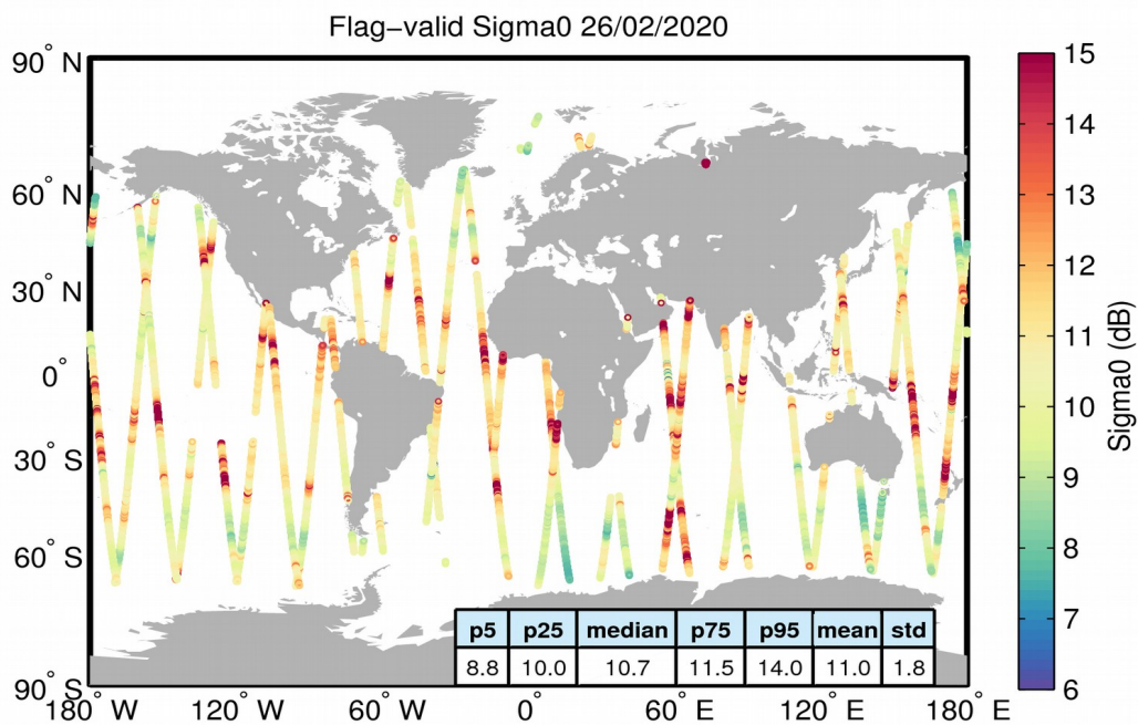
Figure 23. Geographical distribution of flag-valid sigma0 data over oceans and lakes for 26/02/2020. The statistical values shown in the table refer to the sigma0 in dB and are calculated over all measurements shown in the figure.
