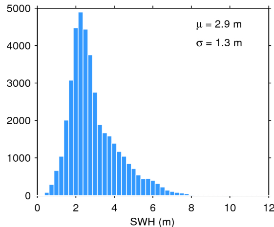
Figure 20. Histogram of science-valid SWH over oceans and lakes for 26/02/2020. The mean ( \mu ) and standard deviation ( \sigma ) are also shown. Note that values larger than 12 m are excluded from the histogram for the sake of readability but not from the computation of \mu and \sigma .
