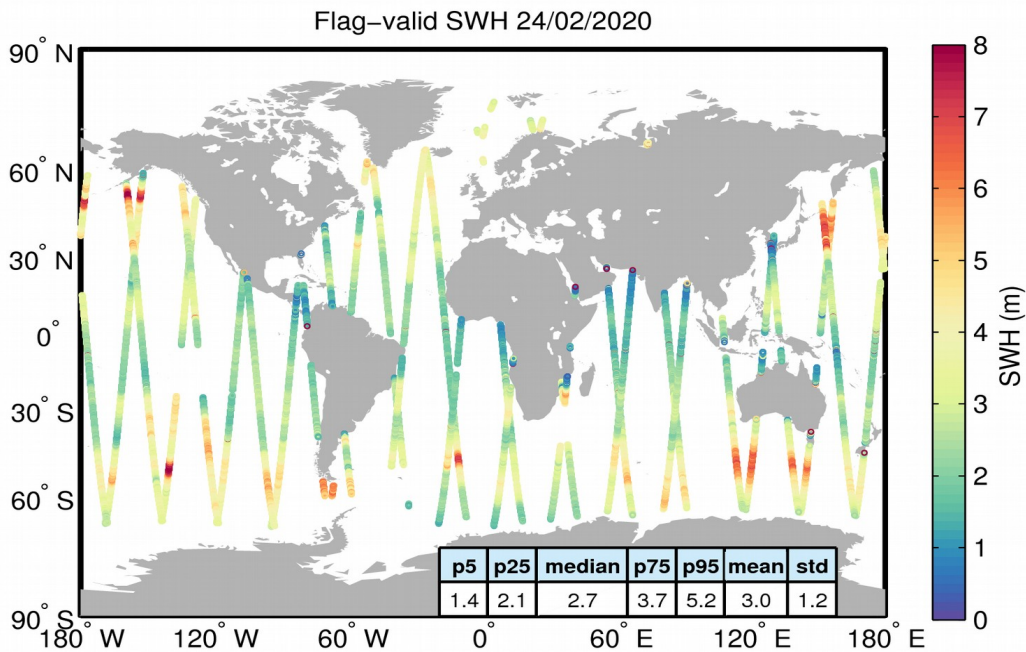
Figure 15. Geographical distribution of flag-valid SWH data over oceans and lakes for 24/02/2020. The statistical values shown in the table refer to the SWH in m and are calculated over all measurements shown in the figure.
