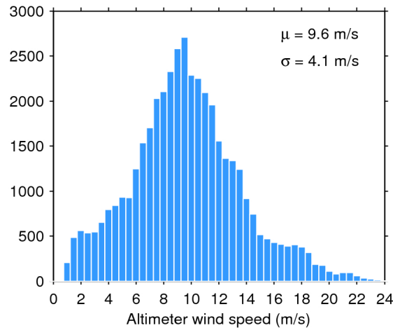
Figure 33. Histogram of flag-valid wind over oceans and lakes for 24/02/2020. The mean ( \mu ) and standard deviation ( \sigma ) are also shown. Note that values larger than 24 m/s are excluded from the histogram for the sake of readability but not from the computation of \mu and \sigma .
