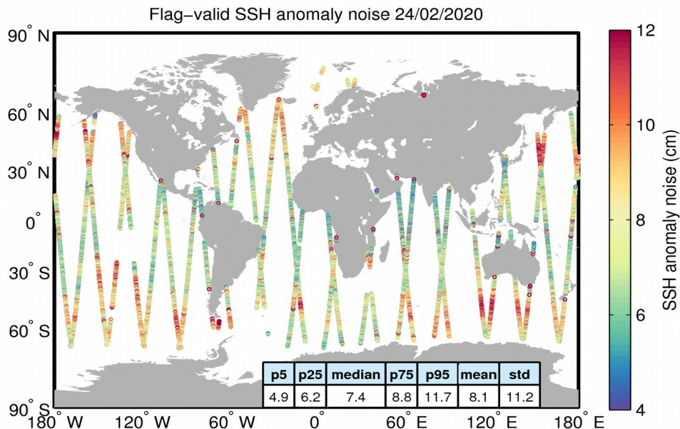
Figure 8. Geographical distribution of flag-valid 20-Hz SSH anomaly measurement noise over oceans and lakes for 24/02/2020. The statistical values shown in the table refer to the SSH anomaly noise and are calculated over all measurements shown in the figure.
