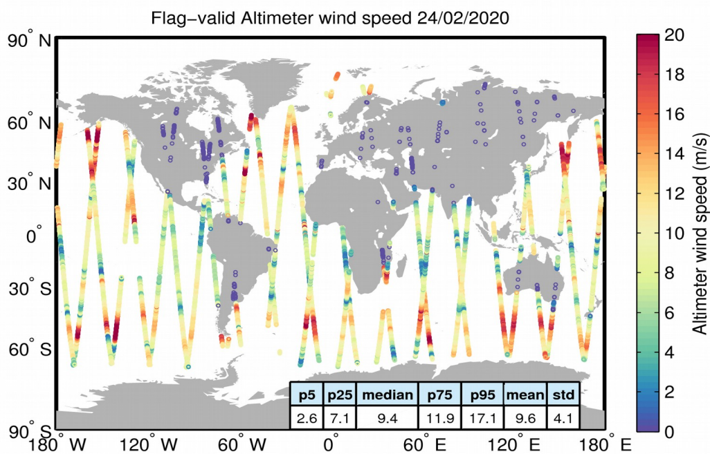
Figure 31. Geographical distribution of flag-valid wind data over oceans and lakes for 24/02/2020. The statistical values shown in the table refer to the wind in m/s and are calculated over all measurements shown in the figure.
