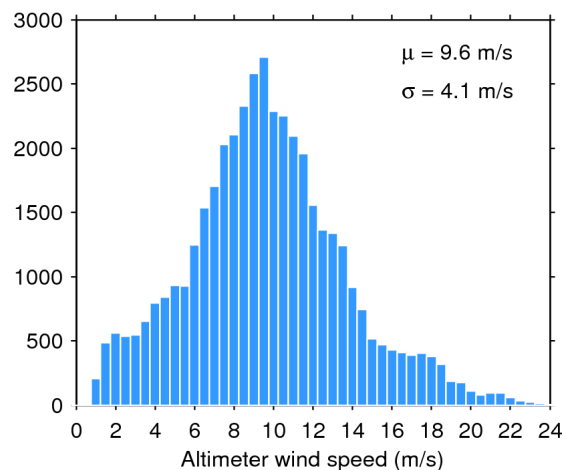
Figure 35. Histogram of science-valid wind over oceans and lakes for 24/02/2020. The mean ( \mu ) and standard deviation ( \sigma ) are also shown. Note that values larger than 24 m/s are excluded from the histogram for the sake of readability but not from the computation of \mu and \sigma .
