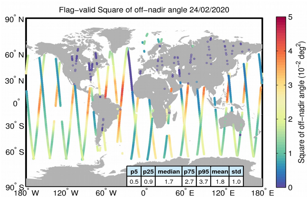
Figure 37. Geographical distribution of flag-valid mispointing data over oceans and lakes for 24/02/2020. The statistical values shown in the table refer to the mispointing in 10^{-2} \text{ deg}^2 and are calculated over all measurements shown in the figure.
