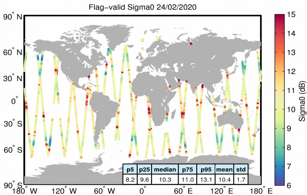
Figure 23. Geographical distribution of flag-valid sigma0 data over oceans and lakes for 24/02/2020. The statistical values shown in the table refer to the sigma0 in dB and are calculated over all measurements shown in the figure.
