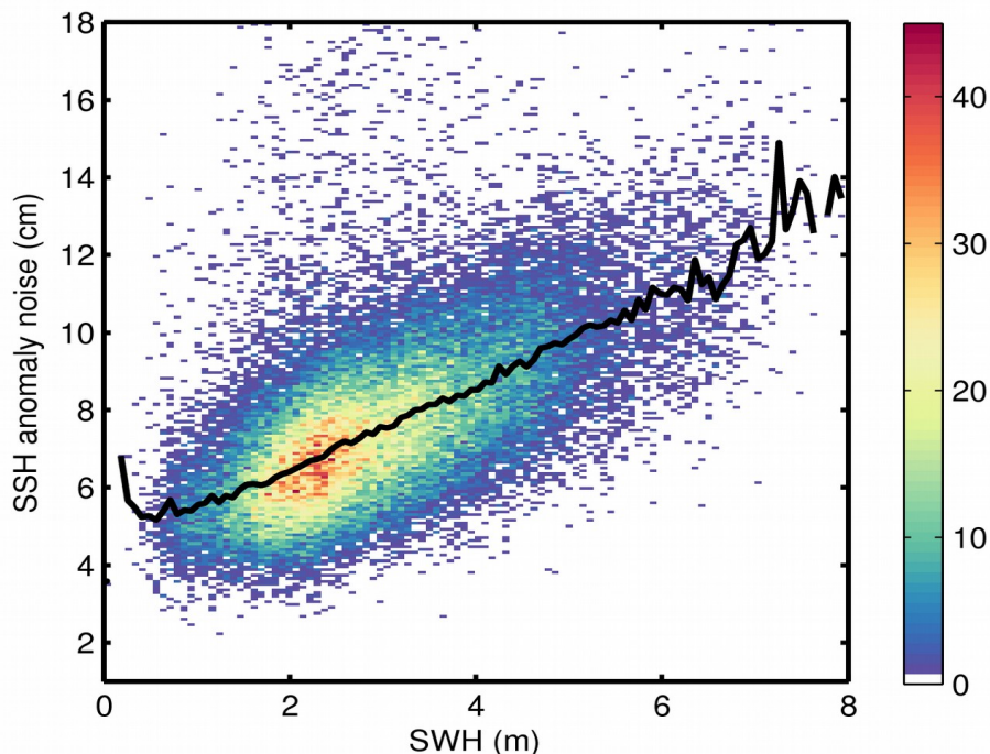
Figure 9. 2D histogram showing flag-valid SSH anomaly noise as a function of SWH for 24/02/2020. The black line denotes the median SSH anomaly noise as a function of SWH.
