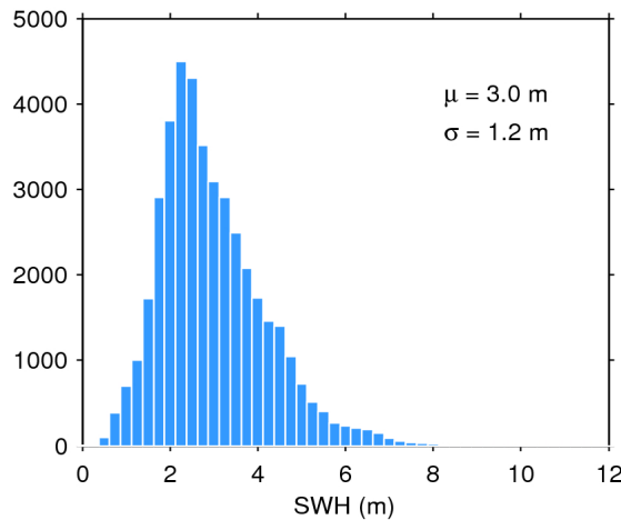
Figure 20. Histogram of science-valid SWH over oceans and lakes for 24/02/2020. The mean ( \mu ) and standard deviation ( \sigma ) are also shown. Note that values larger than 12 m are excluded from the histogram for the sake of readability but not from the computation of \mu and \sigma .
