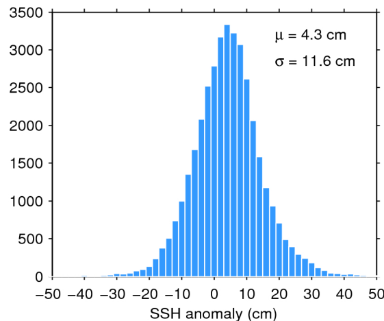
Figure 11. Histogram of science-valid SSH anomaly over oceans and lakes for 24/02/2020. The mean ( \mu ) and standard deviation ( \sigma ) are also shown. Note that values outside [-50 50] cm are excluded from the histogram for the sake of readability but not from the computation of \mu and \sigma .
