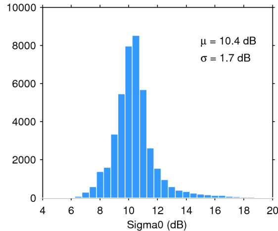
Figure 25. Histogram of flag-valid sigma0 over oceans and lakes for 24/02/2020. The mean ( \mu ) and standard deviation ( \sigma ) are also shown. Note that values outside [4 20] dB are excluded from the histogram for the sake of readability but not from the computation of \mu and \sigma .
