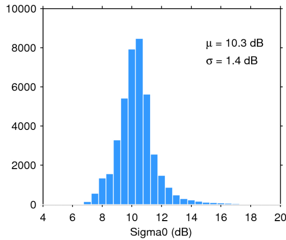
Figure 28. Histogram of science-valid sigma0 over oceans and lakes for 24/02/2020. The mean ( \mu ) and standard deviation ( \sigma ) are also shown. Note that values outside [4 20] dB are excluded from the histogram for the sake of readability but not from the computation of \mu and \sigma .
