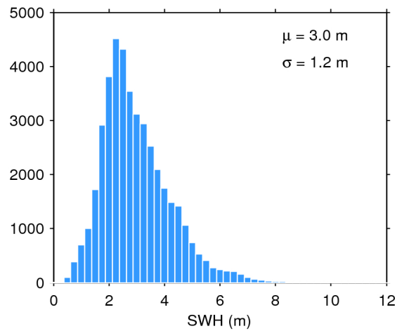
Figure 17. Histogram of flag-valid SWH over oceans and lakes for 24/02/2020. The mean ( \mu ) and standard deviation ( \sigma ) are also shown. Note that values larger than 12 m are excluded from the histogram for the sake of readability but not from the computation of \mu and \sigma .
