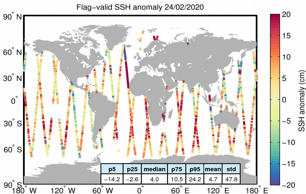
Figure 5. Geographical distribution of flag-valid 1-Hz SSH anomaly data over oceans and lakes for 24/02/2020. The statistical values shown in the table refer to the SSH anomaly in cm and are calculated over all measurements shown in the figure.
