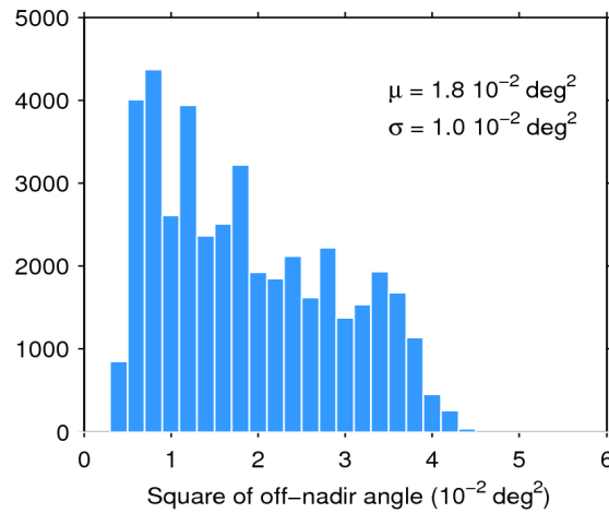
Figure 39. Histogram of flag-valid mispointing over oceans and lakes for 24/02/2020. The mean ( \mu ) and standard deviation ( \sigma ) are also shown. Note that values larger than 6 \cdot 10^{-2} \text{ deg}^2 are excluded from the histogram for the sake of readability but not from the computation of \mu and \sigma .
