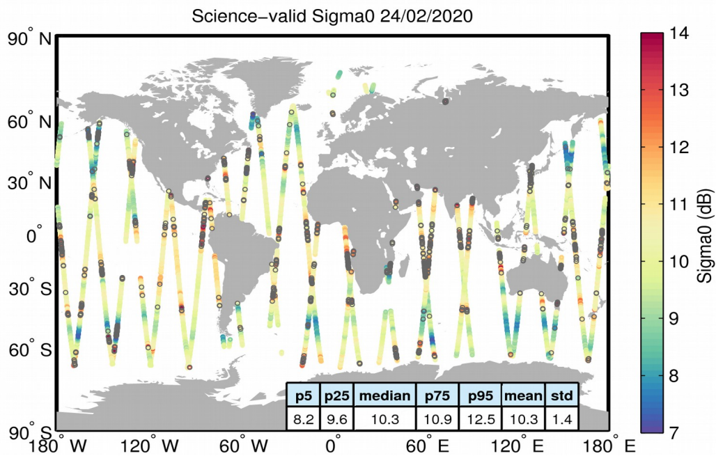
Figure 27. Geographical distribution of science-valid sigma0 data over oceans and lakes for 24/02/2020. The statistical values shown in the table refer to the sigma0 in dB and are calculated over all measurements shown in the figure. Gray circles denote records that have been rejected based on the editing criteria described in Table 4.
