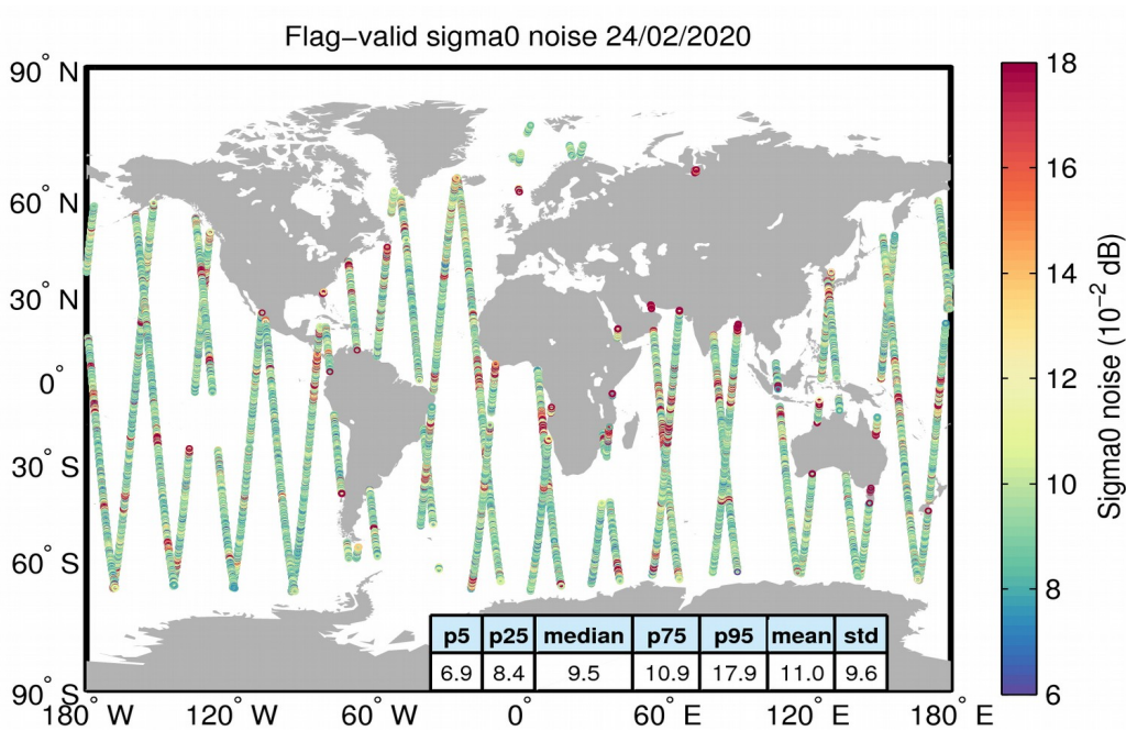
Figure 26. Geographical distribution of flag-valid 20-Hz sigma0 measurement noise over oceans and lakes for 24/02/2020. The statistical values shown in the table refer to the sigma0 noise and are calculated over all measurements shown in the figure.
