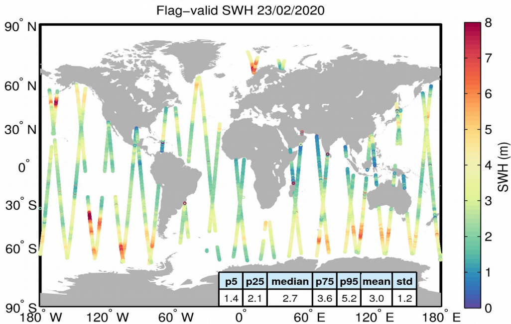
Figure 15. Geographical distribution of flag-valid SWH data over oceans and lakes for 23/02/2020. The statistical values shown in the table refer to the SWH in m and are calculated over all measurements shown in the figure.
