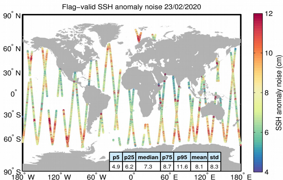
Figure 8. Geographical distribution of flag-valid 20-Hz SSH anomaly measurement noise over oceans and lakes for 23/02/2020. The statistical values shown in the table refer to the SSH anomaly noise and are calculated over all measurements shown in the figure.
