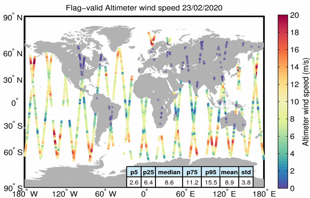
Figure 31. Geographical distribution of flag-valid wind data over oceans and lakes for 23/02/2020. The statistical values shown in the table refer to the wind in m/s and are calculated over all measurements shown in the figure.
