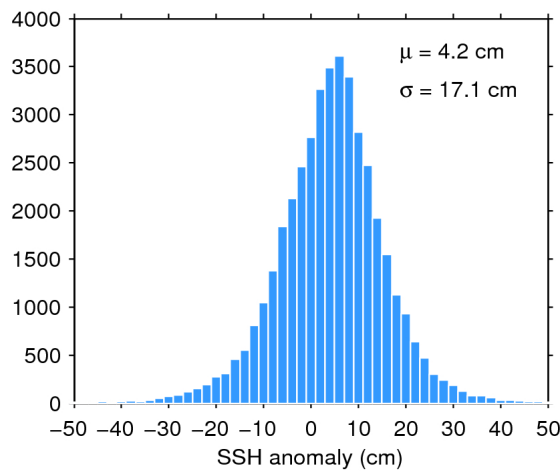
Figure 7. Histogram of flag-valid SSH anomaly over oceans and lakes for 23/02/2020. The mean ( \mu ) and standard deviation ( \sigma ) are also shown. Note that values outside [-50 50] cm are excluded from the histogram for the sake of readability but not from the computation of \mu and \sigma .
