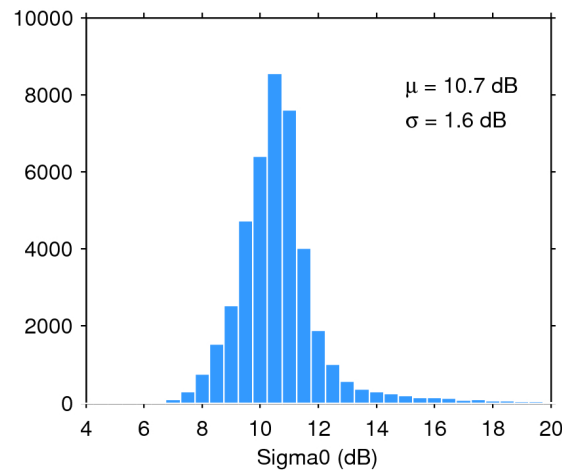
Figure 25. Histogram of flag-valid sigma0 over oceans and lakes for 23/02/2020. The mean ( \mu ) and standard deviation ( \sigma ) are also shown. Note that values outside [4 20] dB are excluded from the histogram for the sake of readability but not from the computation of \mu and \sigma .
