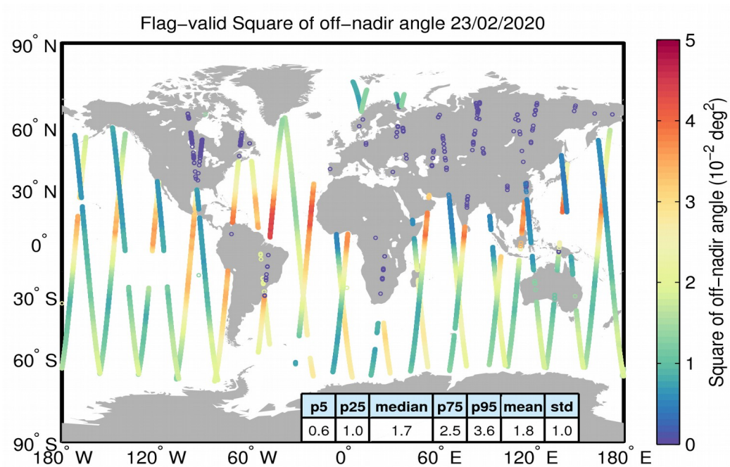
Figure 37. Geographical distribution of flag-valid mispointing data over oceans and lakes for 23/02/2020. The statistical values shown in the table refer to the mispointing in 10^{-2} \text{ deg}^2 and are calculated over all measurements shown in the figure.
