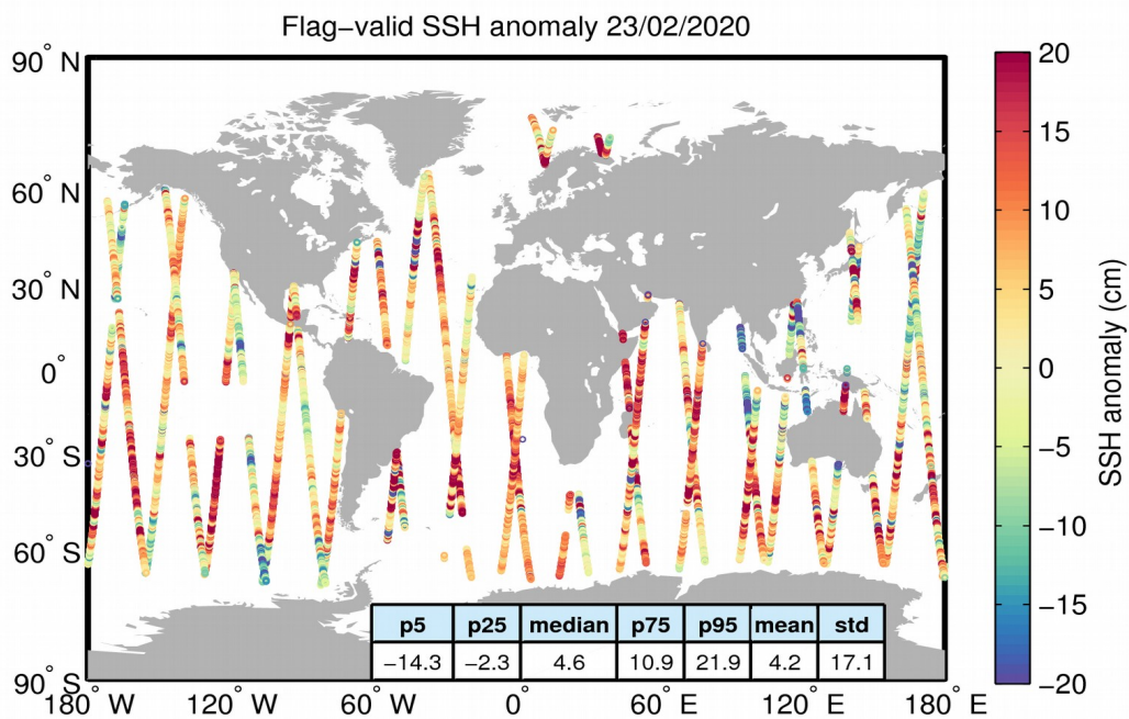
Figure 5. Geographical distribution of flag-valid 1-Hz SSH anomaly data over oceans and lakes for 23/02/2020. The statistical values shown in the table refer to the SSH anomaly in cm and are calculated over all measurements shown in the figure.
