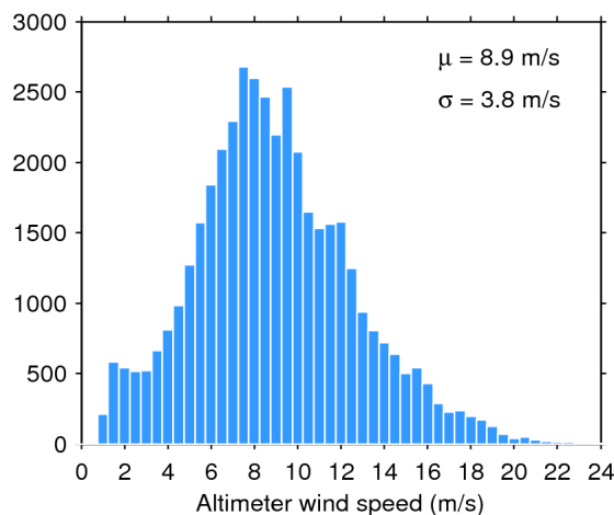
Figure 35. Histogram of science-valid wind over oceans and lakes for 23/02/2020. The mean ( \mu ) and standard deviation ( \sigma ) are also shown. Note that values larger than 24 m/s are excluded from the histogram for the sake of readability but not from the computation of \mu and \sigma .
