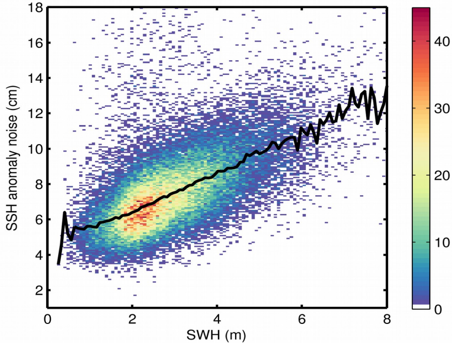
Figure 9. 2D histogram showing flag-valid SSH anomaly noise as a function of SWH for 23/02/2020. The black line denotes the median SSH anomaly noise as a function of SWH.
