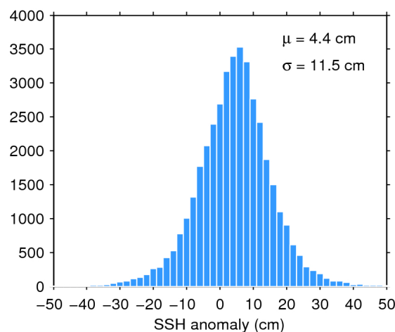
Figure 11. Histogram of science-valid SSH anomaly over oceans and lakes for 23/02/2020. The mean ( \mu ) and standard deviation ( \sigma ) are also shown. Note that values outside [-50 50] cm are excluded from the histogram for the sake of readability but not from the computation of \mu and \sigma .
