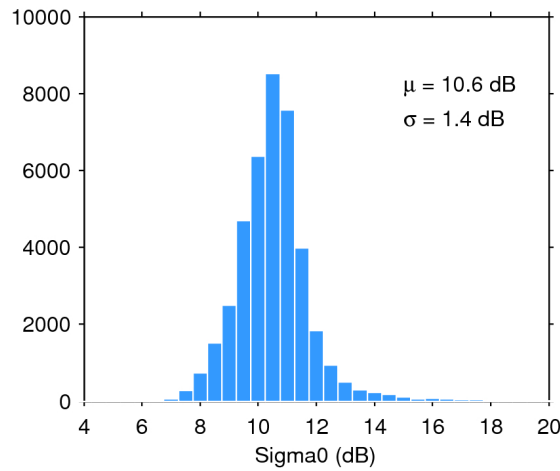
Figure 28. Histogram of science-valid sigma0 over oceans and lakes for 23/02/2020. The mean ( \mu ) and standard deviation ( \sigma ) are also shown. Note that values outside [4 20] dB are excluded from the histogram for the sake of readability but not from the computation of \mu and \sigma .
