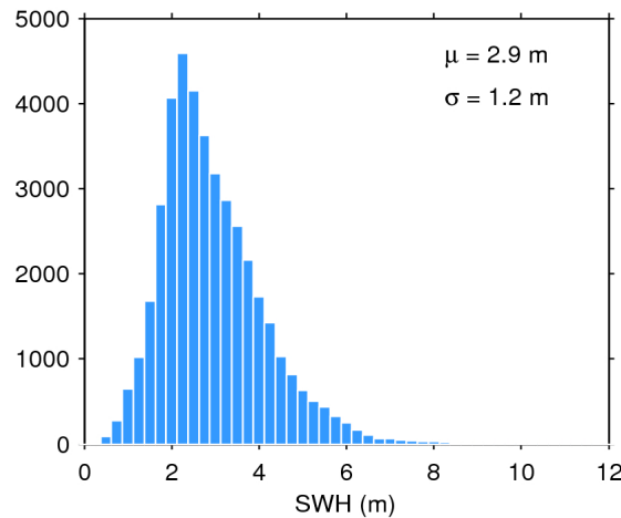
Figure 20. Histogram of science-valid SWH over oceans and lakes for 23/02/2020. The mean ( \mu ) and standard deviation ( \sigma ) are also shown. Note that values larger than 12 m are excluded from the histogram for the sake of readability but not from the computation of \mu and \sigma .
