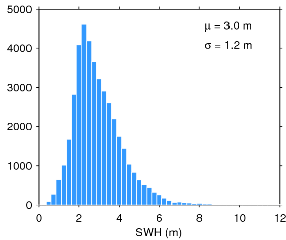
Figure 17. Histogram of flag-valid SWH over oceans and lakes for 23/02/2020. The mean ( \mu ) and standard deviation ( \sigma ) are also shown. Note that values larger than 12 m are excluded from the histogram for the sake of readability but not from the computation of \mu and \sigma .
