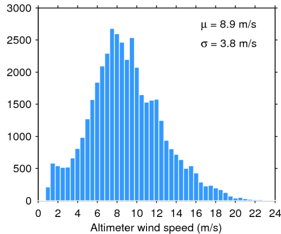
Figure 33. Histogram of flag-valid wind over oceans and lakes for 23/02/2020. The mean ( \mu ) and standard deviation ( \sigma ) are also shown. Note that values larger than 24 m/s are excluded from the histogram for the sake of readability but not from the computation of \mu and \sigma .
