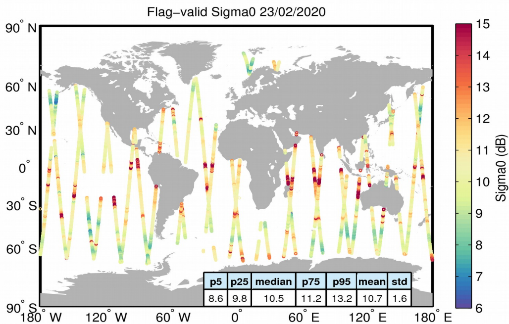
Figure 23. Geographical distribution of flag-valid sigma0 data over oceans and lakes for 23/02/2020. The statistical values shown in the table refer to the sigma0 in dB and are calculated over all measurements shown in the figure.
