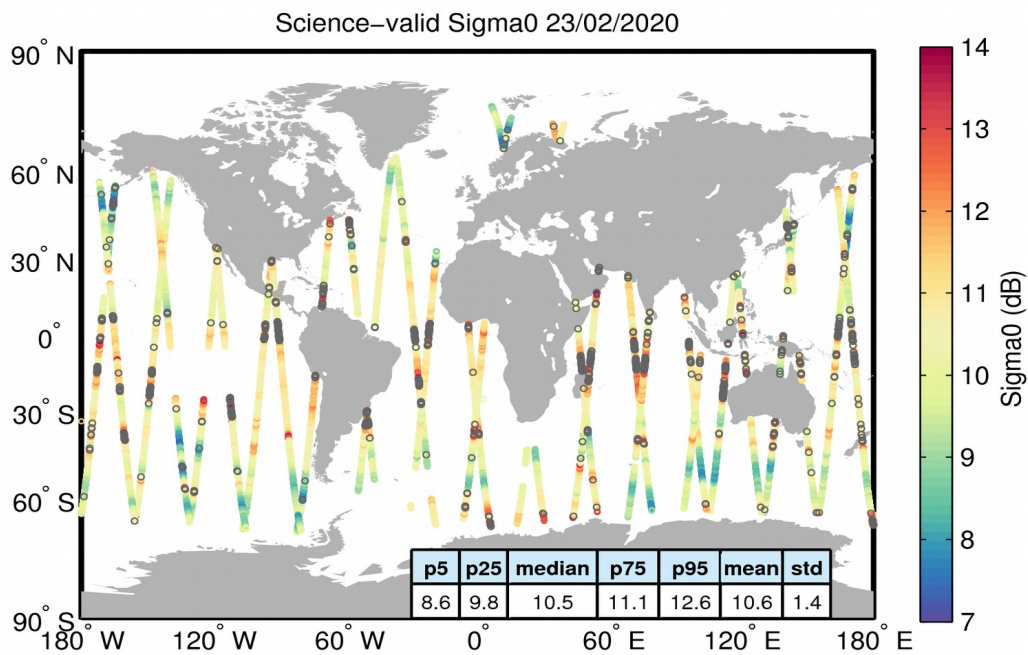
Figure 27. Geographical distribution of science-valid sigma0 data over oceans and lakes for 23/02/2020. The statistical values shown in the table refer to the sigma0 in dB and are calculated over all measurements shown in the figure. Gray circles denote records that have been rejected based on the editing criteria described in Table 4.
