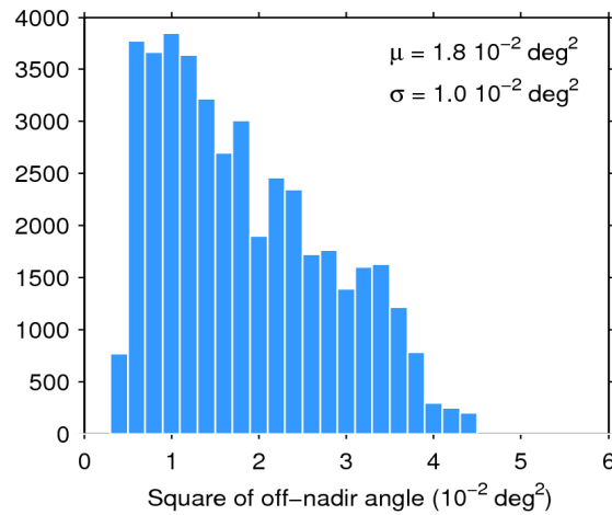
Figure 39. Histogram of flag-valid mispointing over oceans and lakes for 23/02/2020. The mean ( \mu ) and standard deviation ( \sigma ) are also shown. Note that values larger than 6 \cdot 10^{-2} \text{ deg}^2 are excluded from the histogram for the sake of readability but not from the computation of \mu and \sigma .
