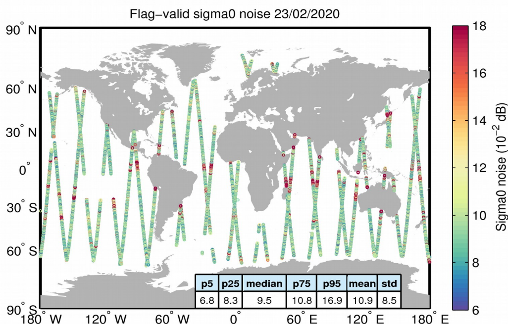
Figure 26. Geographical distribution of flag-valid 20-Hz sigma0 measurement noise over oceans and lakes for 23/02/2020. The statistical values shown in the table refer to the sigma0 noise and are calculated over all measurements shown in the figure.
