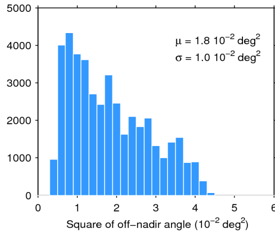
Figure 39. Histogram of flag-valid mispointing over oceans and lakes for 22/02/2020. The mean ( \mu ) and standard deviation ( \sigma ) are also shown. Note that values larger than 6 \cdot 10^{-2} \text{ deg}^2 are excluded from the histogram for the sake of readability but not from the computation of \mu and \sigma .
