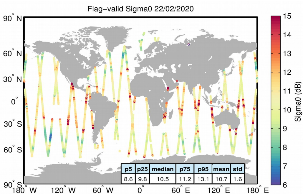
Figure 23. Geographical distribution of flag-valid sigma0 data over oceans and lakes for 22/02/2020. The statistical values shown in the table refer to the sigma0 in dB and are calculated over all measurements shown in the figure.
