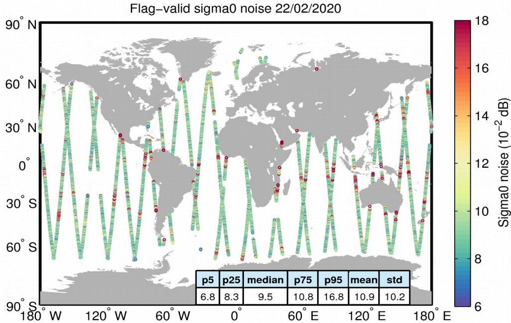
Figure 26. Geographical distribution of flag-valid 20-Hz sigma0 measurement noise over oceans and lakes for 22/02/2020. The statistical values shown in the table refer to the sigma0 noise and are calculated over all measurements shown in the figure.
