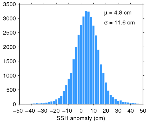
Figure 11. Histogram of science-valid SSH anomaly over oceans and lakes for 22/02/2020. The mean ( \mu ) and standard deviation ( \sigma ) are also shown. Note that values outside [-50 50] cm are excluded from the histogram for the sake of readability but not from the computation of \mu and \sigma .
