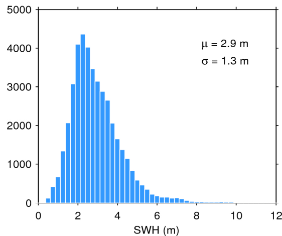
Figure 20. Histogram of science-valid SWH over oceans and lakes for 22/02/2020. The mean ( \mu ) and standard deviation ( \sigma ) are also shown. Note that values larger than 12 m are excluded from the histogram for the sake of readability but not from the computation of \mu and \sigma .
