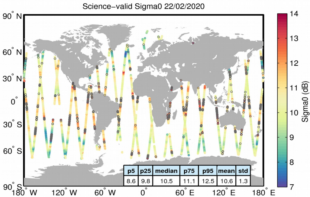
Figure 27. Geographical distribution of science-valid sigma0 data over oceans and lakes for 22/02/2020. The statistical values shown in the table refer to the sigma0 in dB and are calculated over all measurements shown in the figure. Gray circles denote records that have been rejected based on the editing criteria described in Table 4.
