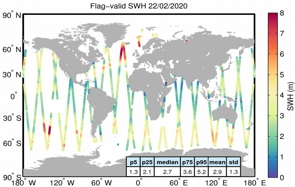
Figure 15. Geographical distribution of flag-valid SWH data over oceans and lakes for 22/02/2020. The statistical values shown in the table refer to the SWH in m and are calculated over all measurements shown in the figure.
