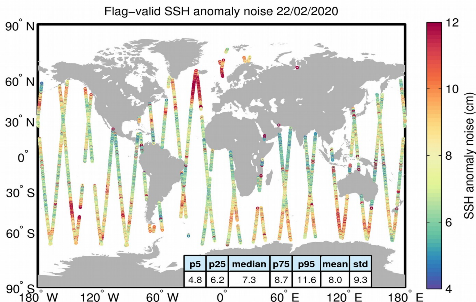
Figure 8. Geographical distribution of flag-valid 20-Hz SSH anomaly measurement noise over oceans and lakes for 22/02/2020. The statistical values shown in the table refer to the SSH anomaly noise and are calculated over all measurements shown in the figure.
