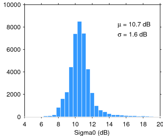
Figure 25. Histogram of flag-valid sigma0 over oceans and lakes for 22/02/2020. The mean ( \mu ) and standard deviation ( \sigma ) are also shown. Note that values outside [4 20] dB are excluded from the histogram for the sake of readability but not from the computation of \mu and \sigma .
