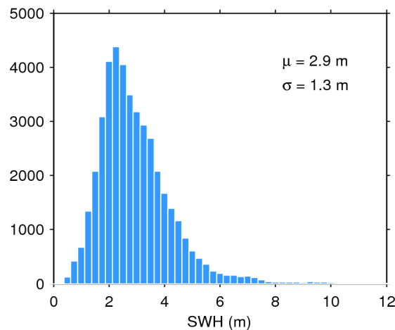
Figure 17. Histogram of flag-valid SWH over oceans and lakes for 22/02/2020. The mean ( \mu ) and standard deviation ( \sigma ) are also shown. Note that values larger than 12 m are excluded from the histogram for the sake of readability but not from the computation of \mu and \sigma .
