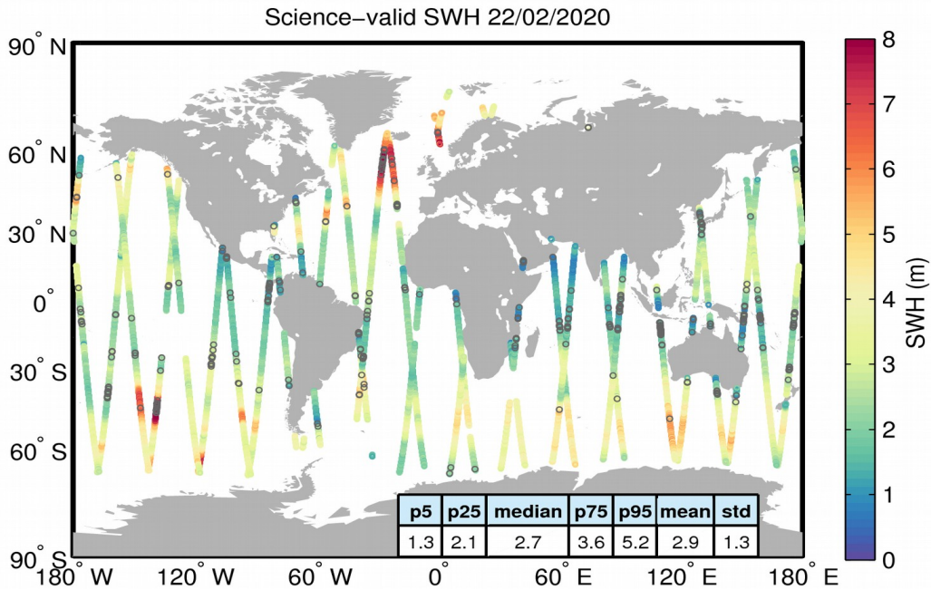
Figure 19. Geographical distribution of science-valid SWH data over oceans and lakes for 22/02/2020. The statistical values shown in the table refer to the SWH in m and are calculated over all measurements shown in the figure. Gray circles denote records that have been rejected based on the editing criteria described in Table 3.
