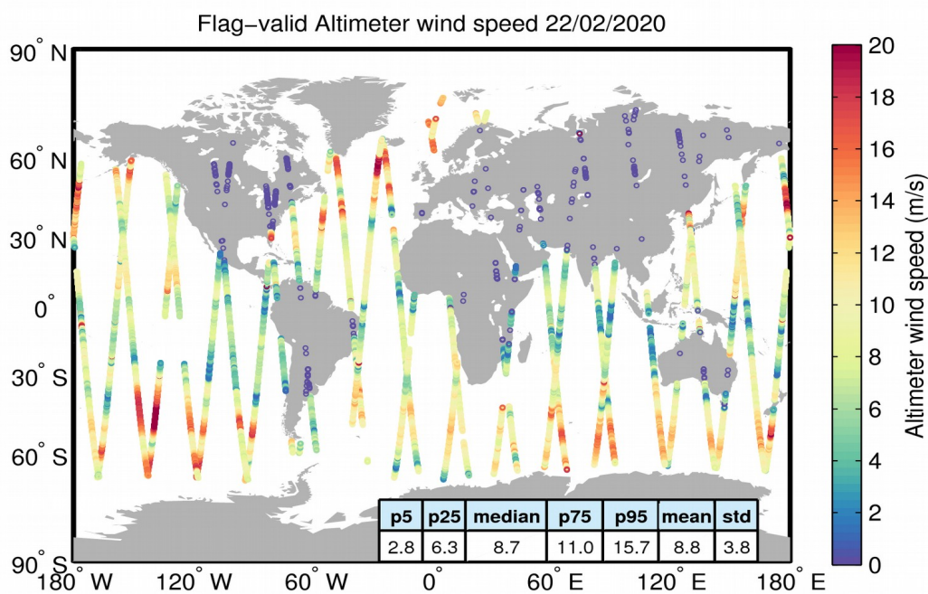
Figure 31. Geographical distribution of flag-valid wind data over oceans and lakes for 22/02/2020. The statistical values shown in the table refer to the wind in m/s and are calculated over all measurements shown in the figure.
