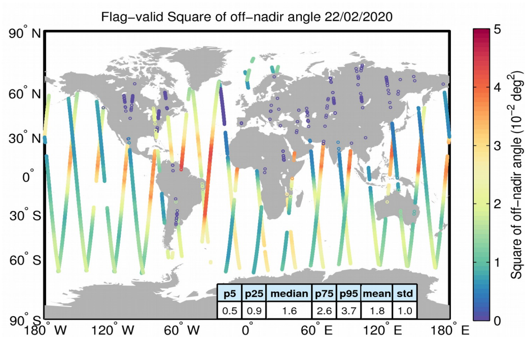
Figure 37. Geographical distribution of flag-valid mispointing data over oceans and lakes for 22/02/2020. The statistical values shown in the table refer to the mispointing in 10^{-2} deg 2 and are calculated over all measurements shown in the figure.
