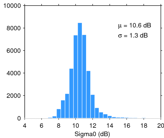
Figure 28. Histogram of science-valid sigma0 over oceans and lakes for 22/02/2020. The mean ( \mu ) and standard deviation ( \sigma ) are also shown. Note that values outside [4 20] dB are excluded from the histogram for the sake of readability but not from the computation of \mu and \sigma .
