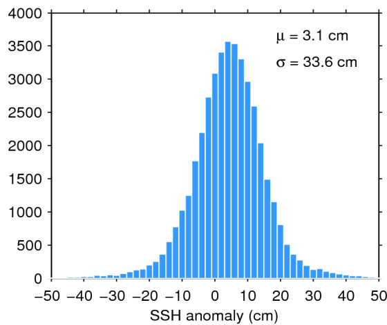
Figure 7. Histogram of flag-valid SSH anomaly over oceans and lakes for 22/02/2020. The mean ( \mu ) and standard deviation ( \sigma ) are also shown. Note that values outside [-50 50] cm are excluded from the histogram for the sake of readability but not from the computation of \mu and \sigma .
