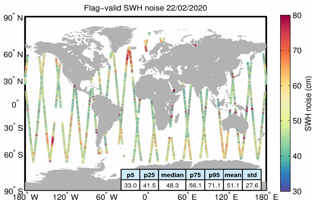
Figure 18. Geographical distribution of flag-valid 20-Hz SWH measurement noise over oceans and lakes for 22/02/2020. The statistical values shown in the figure refer to the SWH noise and are calculated over all measurements shown in the figure.
