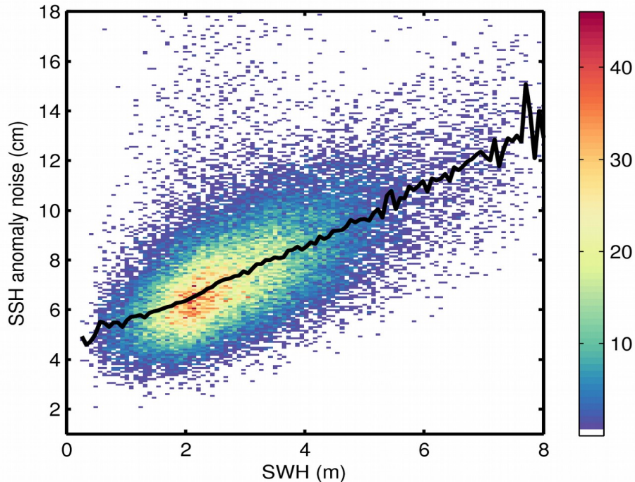
Figure 9. 2D histogram showing flag-valid SSH anomaly noise as a function of SWH for 22/02/2020. The black line denotes the median SSH anomaly noise as a function of SWH.
