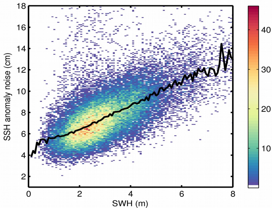
Figure 9. 2D histogram showing flag-valid SSH anomaly noise as a function of SWH for 21/02/2020. The black line denotes the median SSH anomaly noise as a function of SWH.
