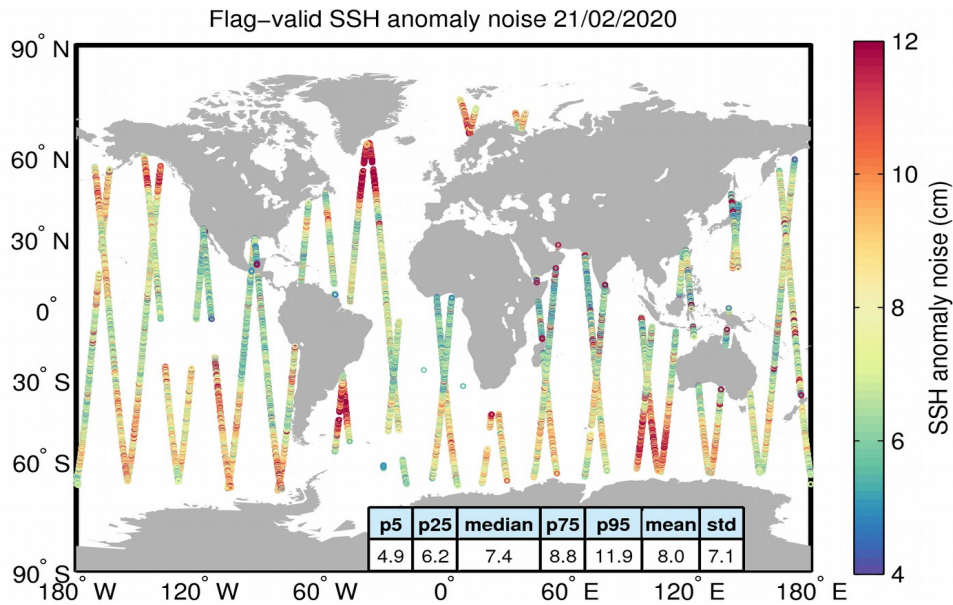
Figure 8. Geographical distribution of flag-valid 20-Hz SSH anomaly measurement noise over oceans and lakes for 21/02/2020. The statistical values shown in the table refer to the SSH anomaly noise and are calculated over all measurements shown in the figure.
