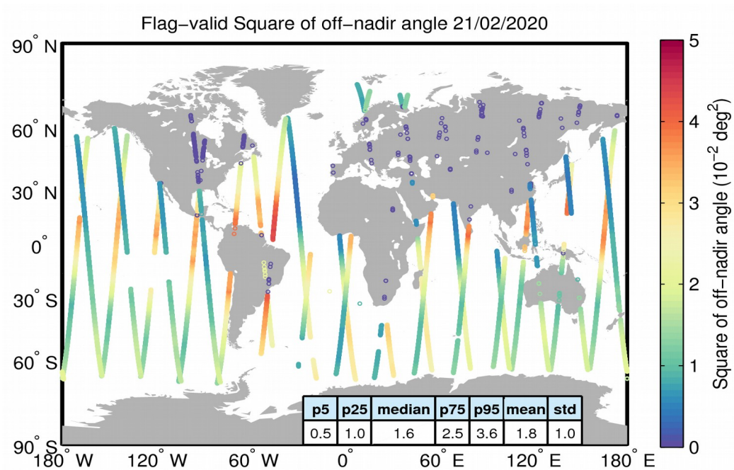
Figure 37. Geographical distribution of flag-valid mispointing data over oceans and lakes for 21/02/2020. The statistical values shown in the table refer to the mispointing in 10^{-2} \text{ deg}^2 and are calculated over all measurements shown in the figure.
