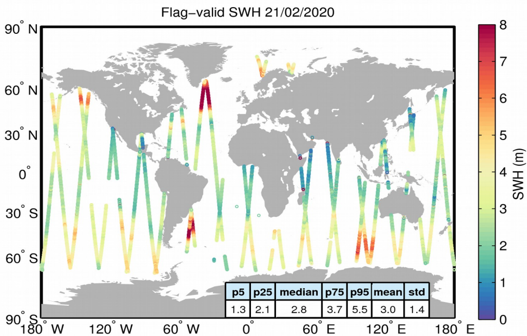
Figure 15. Geographical distribution of flag-valid SWH data over oceans and lakes for 21/02/2020. The statistical values shown in the table refer to the SWH in m and are calculated over all measurements shown in the figure.
