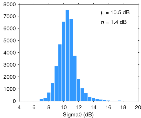
Figure 28. Histogram of science-valid sigma0 over oceans and lakes for 21/02/2020. The mean ( \mu ) and standard deviation ( \sigma ) are also shown. Note that values outside [4 20] dB are excluded from the histogram for the sake of readability but not from the computation of \mu and \sigma .
