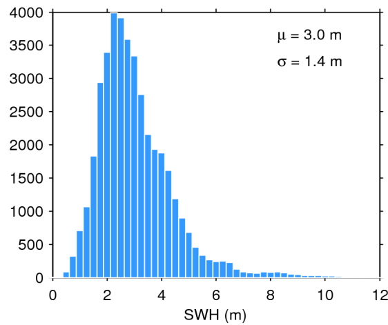
Figure 17. Histogram of flag-valid SWH over oceans and lakes for 21/02/2020. The mean ( \mu ) and standard deviation ( \sigma ) are also shown. Note that values larger than 12 m are excluded from the histogram for the sake of readability but not from the computation of \mu and \sigma .
