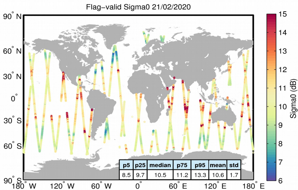
Figure 23. Geographical distribution of flag-valid sigma0 data over oceans and lakes for 21/02/2020. The statistical values shown in the table refer to the sigma0 in dB and are calculated over all measurements shown in the figure.
