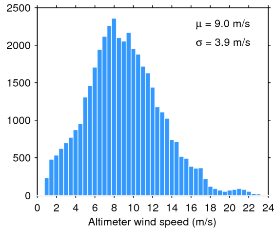
Figure 33. Histogram of flag-valid wind over oceans and lakes for 21/02/2020. The mean ( \mu ) and standard deviation ( \sigma ) are also shown. Note that values larger than 24 m/s are excluded from the histogram for the sake of readability but not from the computation of \mu and \sigma .
