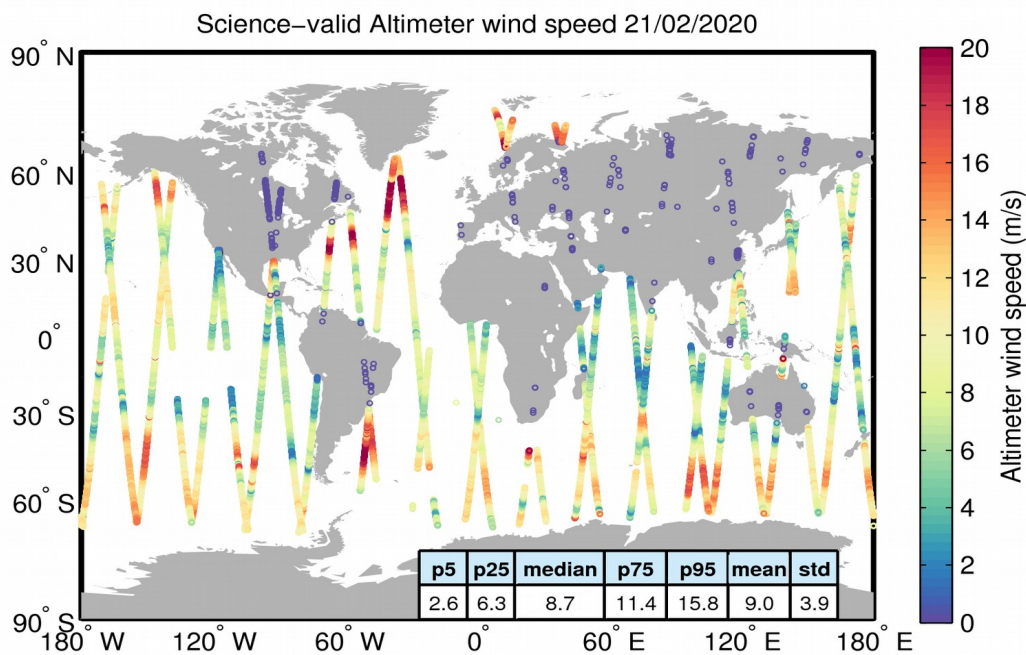
Figure 34. Geographical distribution of science-valid wind data over oceans and lakes for 21/02/2020. The statistical values shown in the table refer to the wind in m/s and are calculated over all measurements shown in the figure. Gray circles denote records that have been rejected based on the editing criteria described in Table 5.
