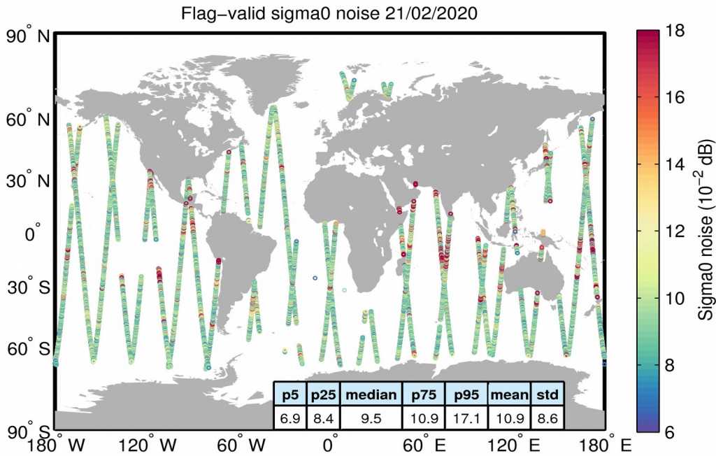
Figure 26. Geographical distribution of flag-valid 20-Hz sigma0 measurement noise over oceans and lakes for 21/02/2020. The statistical values shown in the table refer to the sigma0 noise and are calculated over all measurements shown in the figure.
