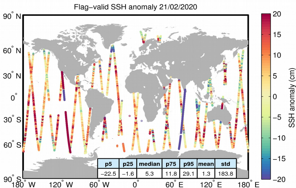
Figure 5. Geographical distribution of flag-valid 1-Hz SSH anomaly data over oceans and lakes for 21/02/2020. The statistical values shown in the table refer to the SSH anomaly in cm and are calculated over all measurements shown in the figure.
