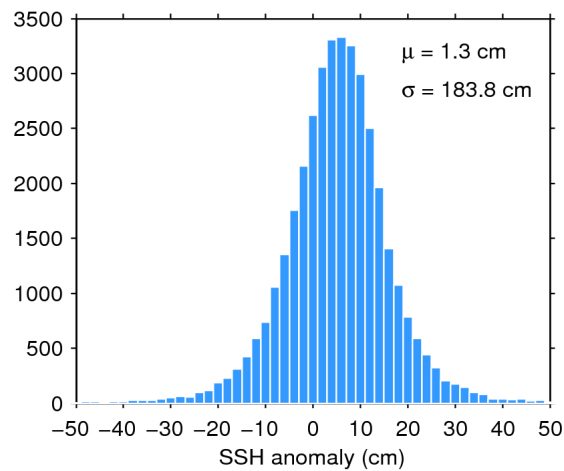
Figure 7. Histogram of flag-valid SSH anomaly over oceans and lakes for 21/02/2020. The mean ( \mu ) and standard deviation ( \sigma ) are also shown. Note that values outside [-50 50] cm are excluded from the histogram for the sake of readability but not from the computation of \mu and \sigma .
