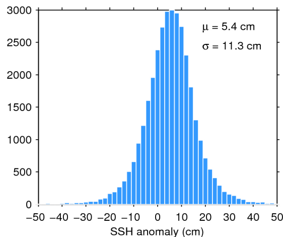
Figure 11. Histogram of science-valid SSH anomaly over oceans and lakes for 21/02/2020. The mean ( \mu ) and standard deviation ( \sigma ) are also shown. Note that values outside [-50 50] cm are excluded from the histogram for the sake of readability but not from the computation of \mu and \sigma .
