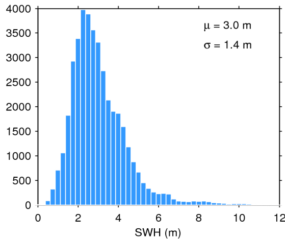
Figure 20. Histogram of science-valid SWH over oceans and lakes for 21/02/2020. The mean ( \mu ) and standard deviation ( \sigma ) are also shown. Note that values larger than 12 m are excluded from the histogram for the sake of readability but not from the computation of \mu and \sigma .
