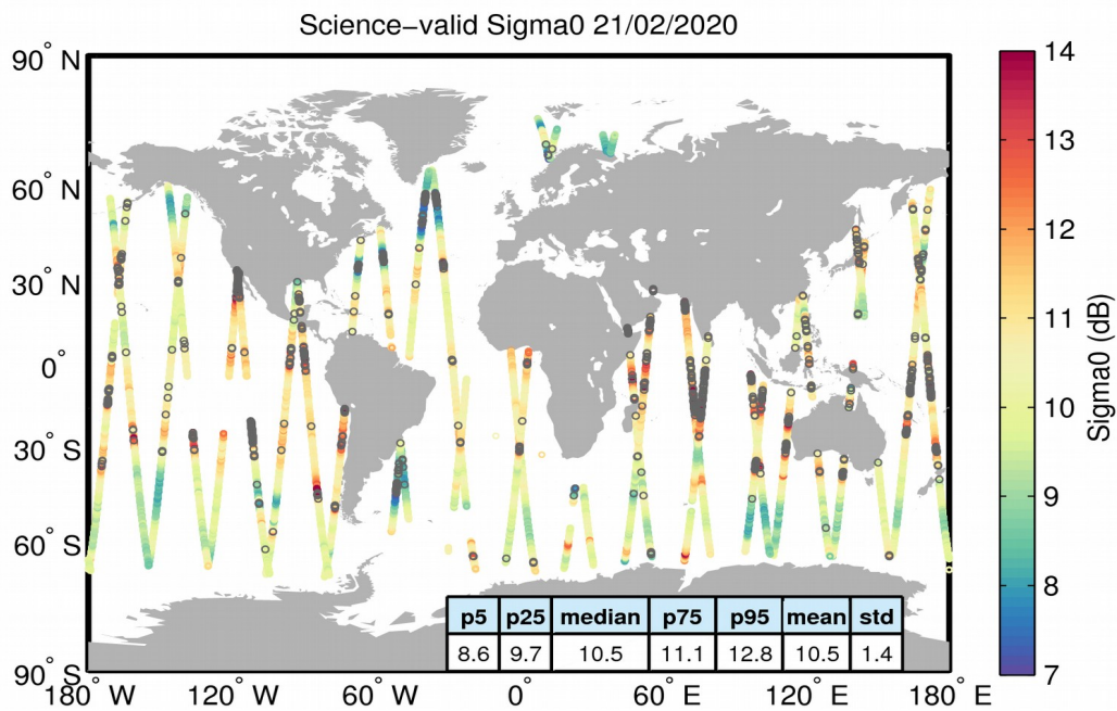
Figure 27. Geographical distribution of science-valid sigma0 data over oceans and lakes for 21/02/2020. The statistical values shown in the table refer to the sigma0 in dB and are calculated over all measurements shown in the figure. Gray circles denote records that have been rejected based on the editing criteria described in Table 4.
