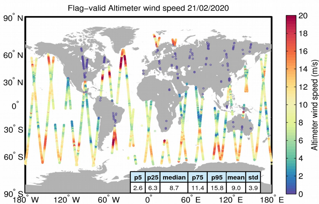
Figure 31. Geographical distribution of flag-valid wind data over oceans and lakes for 21/02/2020. The statistical values shown in the table refer to the wind in m/s and are calculated over all measurements shown in the figure.
