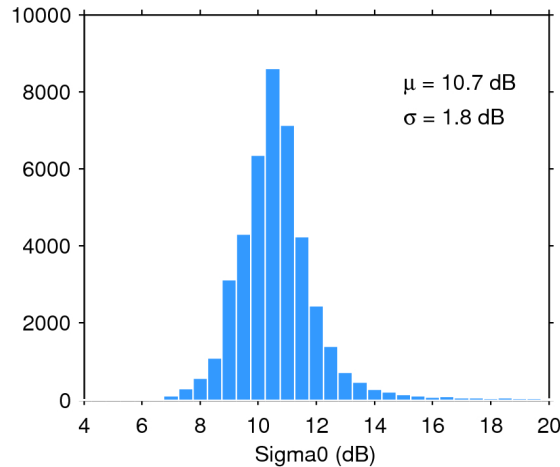
Figure 25. Histogram of flag-valid sigma0 over oceans and lakes for 20/02/2020. The mean ( \mu ) and standard deviation ( \sigma ) are also shown. Note that values outside [4 20] dB are excluded from the histogram for the sake of readability but not from the computation of \mu and \sigma .
