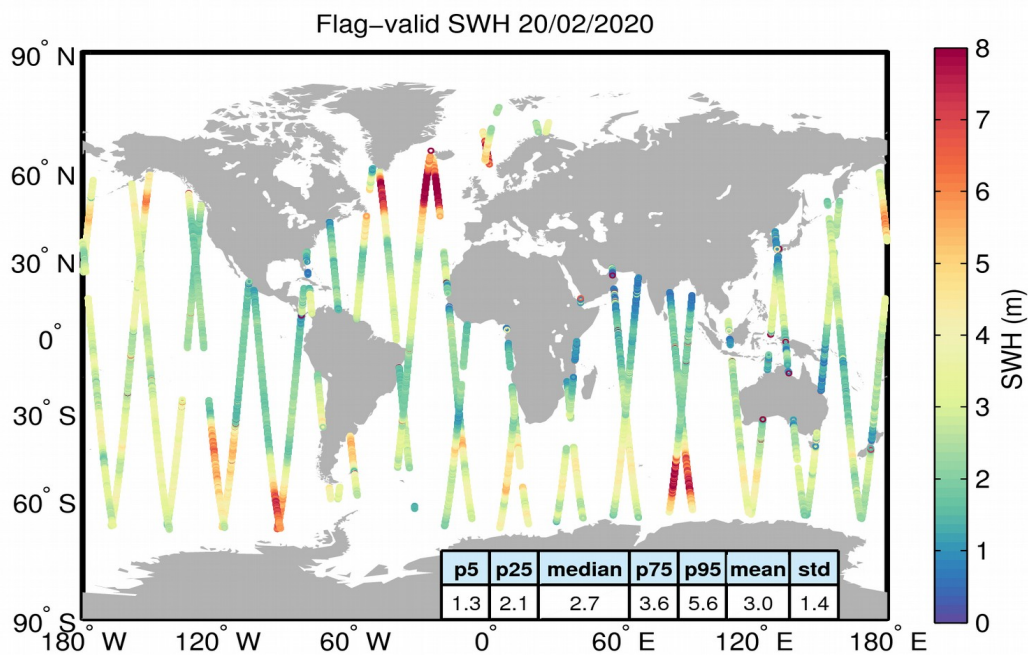
Figure 15. Geographical distribution of flag-valid SWH data over oceans and lakes for 20/02/2020. The statistical values shown in the table refer to the SWH in m and are calculated over all measurements shown in the figure.
