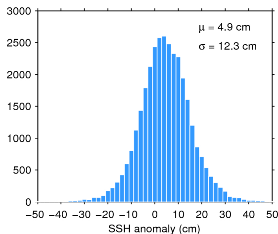
Figure 11. Histogram of science-valid SSH anomaly over oceans and lakes for 20/02/2020. The mean ( \mu ) and standard deviation ( \sigma ) are also shown. Note that values outside [-50 50] cm are excluded from the histogram for the sake of readability but not from the computation of \mu and \sigma .
