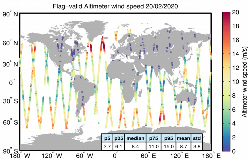
Figure 31. Geographical distribution of flag-valid wind data over oceans and lakes for 20/02/2020. The statistical values shown in the table refer to the wind in m/s and are calculated over all measurements shown in the figure.
