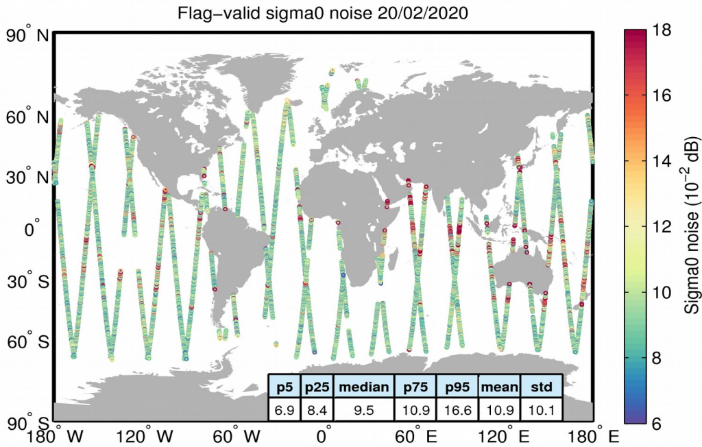
Figure 26. Geographical distribution of flag-valid 20-Hz sigma0 measurement noise over oceans and lakes for 20/02/2020. The statistical values shown in the table refer to the sigma0 noise and are calculated over all measurements shown in the figure.
