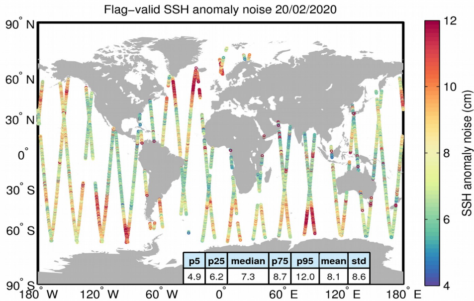
Figure 8. Geographical distribution of flag-valid 20-Hz SSH anomaly measurement noise over oceans and lakes for 20/02/2020. The statistical values shown in the table refer to the SSH anomaly noise and are calculated over all measurements shown in the figure.
