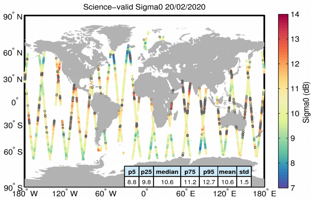
Figure 27. Geographical distribution of science-valid sigma0 data over oceans and lakes for 20/02/2020. The statistical values shown in the table refer to the sigma0 in dB and are calculated over all measurements shown in the figure. Gray circles denote records that have been rejected based on the editing criteria described in Table 4.
