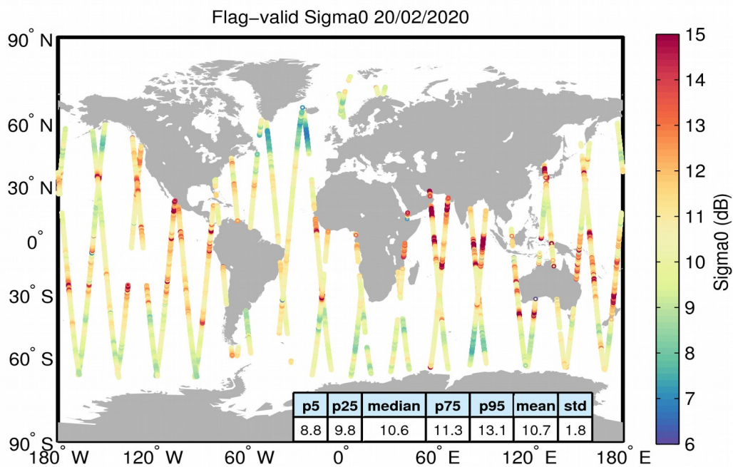
Figure 23. Geographical distribution of flag-valid sigma0 data over oceans and lakes for 20/02/2020. The statistical values shown in the table refer to the sigma0 in dB and are calculated over all measurements shown in the figure.
