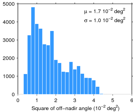
Figure 39. Histogram of flag-valid mispointing over oceans and lakes for 20/02/2020. The mean ( \mu ) and standard deviation ( \sigma ) are also shown. Note that values larger than 6 \cdot 10^{-2} \text{ deg}^2 are excluded from the histogram for the sake of readability but not from the computation of \mu and \sigma .
