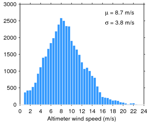
Figure 33. Histogram of flag-valid wind over oceans and lakes for 20/02/2020. The mean ( \mu ) and standard deviation ( \sigma ) are also shown. Note that values larger than 24 m/s are excluded from the histogram for the sake of readability but not from the computation of \mu and \sigma .
