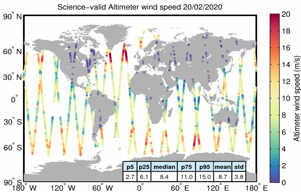
Figure 34. Geographical distribution of science-valid wind data over oceans and lakes for 20/02/2020. The statistical values shown in the table refer to the wind in m/s and are calculated over all measurements shown in the figure. Gray circles denote records that have been rejected based on the editing criteria described in Table 5.
