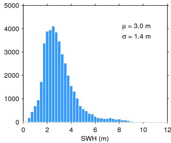
Figure 17. Histogram of flag-valid SWH over oceans and lakes for 20/02/2020. The mean ( \mu ) and standard deviation ( \sigma ) are also shown. Note that values larger than 12 m are excluded from the histogram for the sake of readability but not from the computation of \mu and \sigma .
