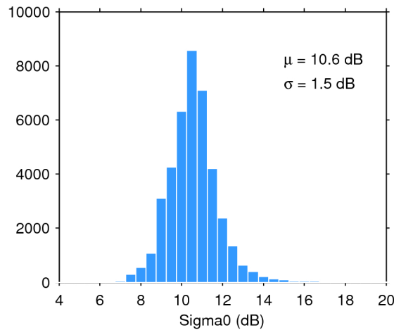
Figure 28. Histogram of science-valid sigma0 over oceans and lakes for 20/02/2020. The mean ( \mu ) and standard deviation ( \sigma ) are also shown. Note that values outside [4 20] dB are excluded from the histogram for the sake of readability but not from the computation of \mu and \sigma .
