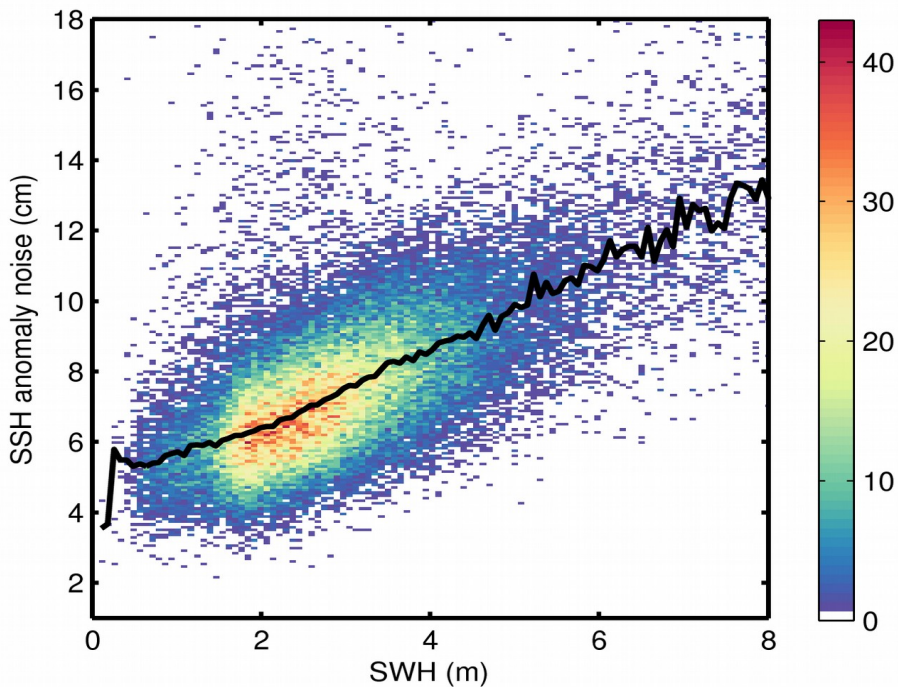
Figure 9. 2D histogram showing flag-valid SSH anomaly noise as a function of SWH for 20/02/2020. The black line denotes the median SSH anomaly noise as a function of SWH.
