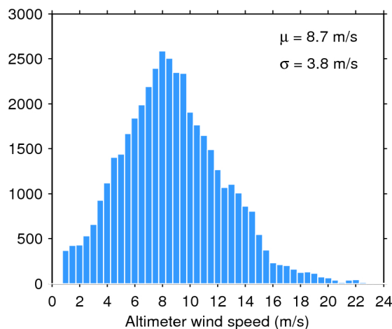
Figure 35. Histogram of science-valid wind over oceans and lakes for 20/02/2020. The mean ( \mu ) and standard deviation ( \sigma ) are also shown. Note that values larger than 24 m/s are excluded from the histogram for the sake of readability but not from the computation of \mu and \sigma .
