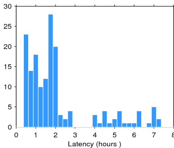
Figure 2. Histogram of the data latency for 20/02/2020. The y-axis denotes the number of files that are made available with a delay of x-hours with respect to the mean time of the records stored in the file.
