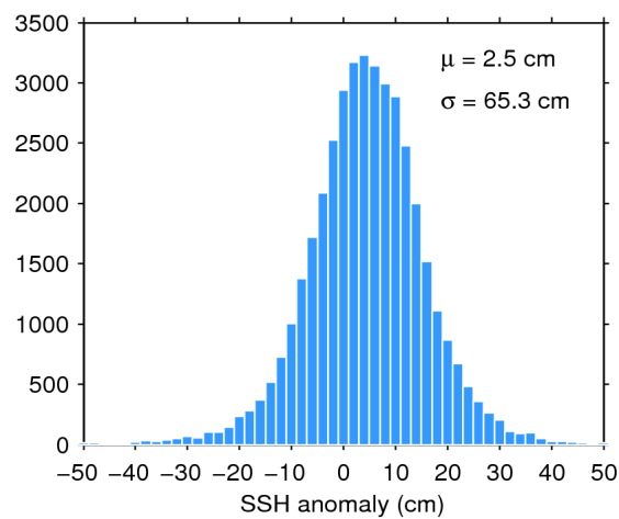
Figure 7. Histogram of flag-valid SSH anomaly over oceans and lakes for 20/02/2020. The mean ( \mu ) and standard deviation ( \sigma ) are also shown. Note that values outside [-50 50] cm are excluded from the histogram for the sake of readability but not from the computation of \mu and \sigma .
