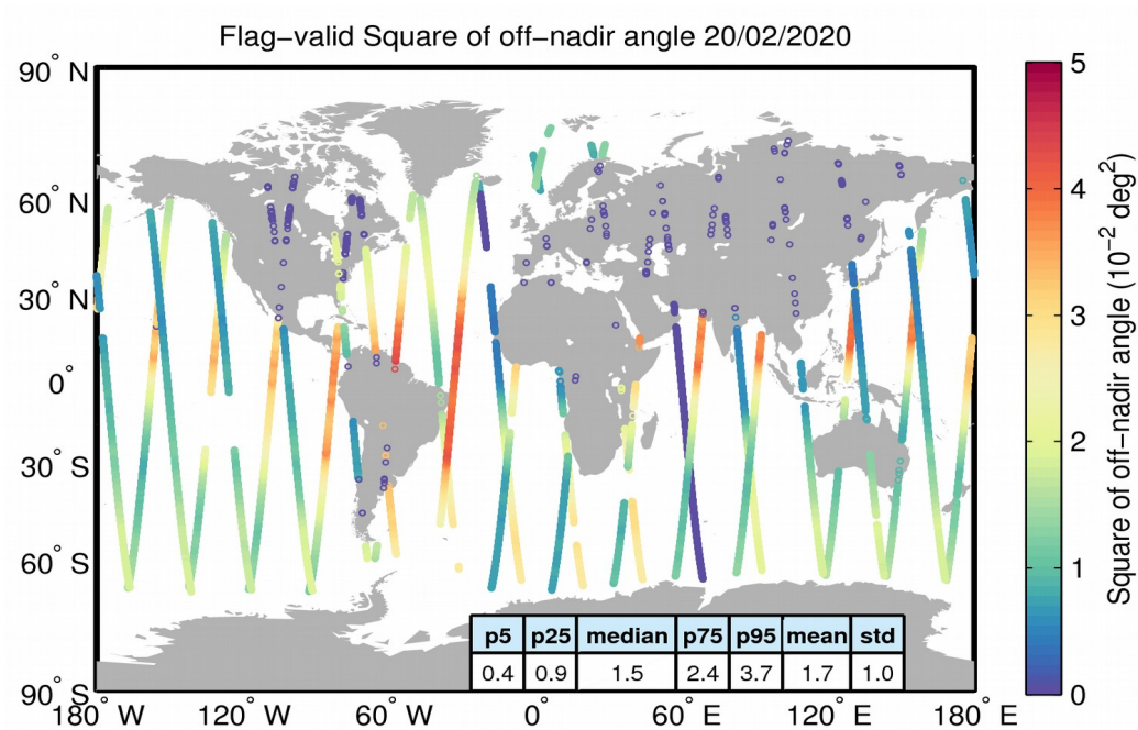
Figure 37. Geographical distribution of flag-valid mispointing data over oceans and lakes for 20/02/2020. The statistical values shown in the table refer to the mispointing in 10^{-2} deg 2 and are calculated over all measurements shown in the figure.
