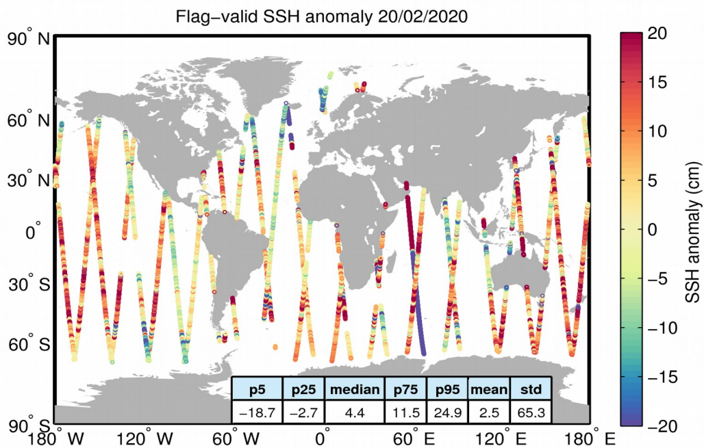
Figure 5. Geographical distribution of flag-valid 1-Hz SSH anomaly data over oceans and lakes for 20/02/2020. The statistical values shown in the table refer to the SSH anomaly in cm and are calculated over all measurements shown in the figure.
