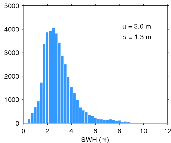
Figure 20. Histogram of science-valid SWH over oceans and lakes for 20/02/2020. The mean ( \mu ) and standard deviation ( \sigma ) are also shown. Note that values larger than 12 m are excluded from the histogram for the sake of readability but not from the computation of \mu and \sigma .
