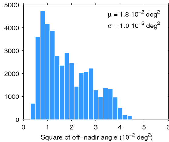
Figure 39. Histogram of flag-valid mispointing over oceans and lakes for 19/02/2020. The mean ( \mu ) and standard deviation ( \sigma ) are also shown. Note that values larger than 6 \cdot 10^{-2} \text{ deg}^2 are excluded from the histogram for the sake of readability but not from the computation of \mu and \sigma .
