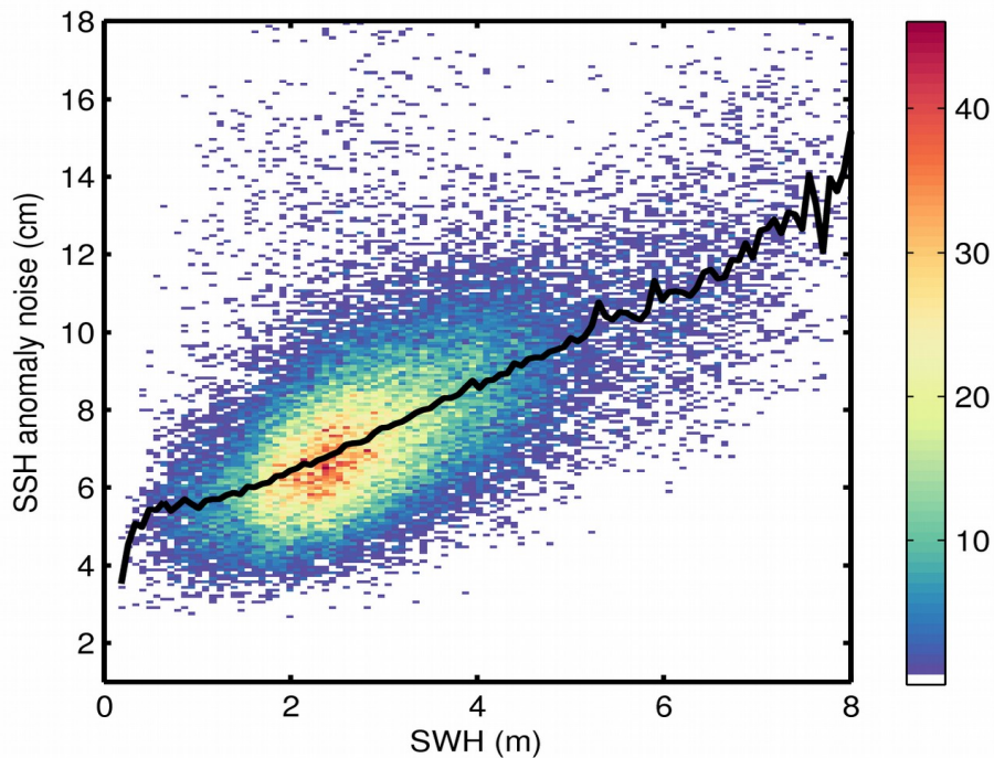
Figure 9. 2D histogram showing flag-valid SSH anomaly noise as a function of SWH for 19/02/2020. The black line denotes the median SSH anomaly noise as a function of SWH.
