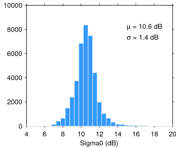
Figure 28. Histogram of science-valid sigma0 over oceans and lakes for 19/02/2020. The mean ( \mu ) and standard deviation ( \sigma ) are also shown. Note that values outside [4 20] dB are excluded from the histogram for the sake of readability but not from the computation of \mu and \sigma .
