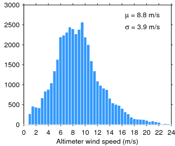
Figure 33. Histogram of flag-valid wind over oceans and lakes for 19/02/2020. The mean ( \mu ) and standard deviation ( \sigma ) are also shown. Note that values larger than 24 m/s are excluded from the histogram for the sake of readability but not from the computation of \mu and \sigma .
