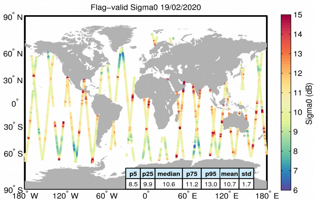
Figure 23. Geographical distribution of flag-valid sigma0 data over oceans and lakes for 19/02/2020. The statistical values shown in the table refer to the sigma0 in dB and are calculated over all measurements shown in the figure.
