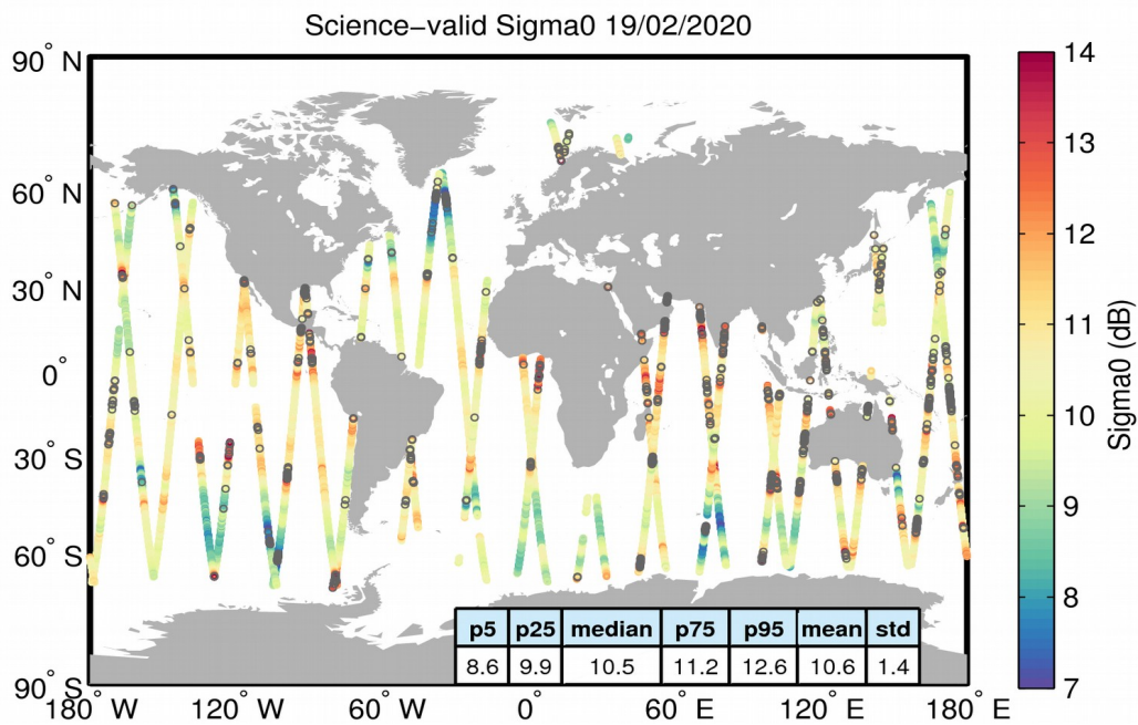
Figure 27. Geographical distribution of science-valid sigma0 data over oceans and lakes for 19/02/2020. The statistical values shown in the table refer to the sigma0 in dB and are calculated over all measurements shown in the figure. Gray circles denote records that have been rejected based on the editing criteria described in Table 4.
