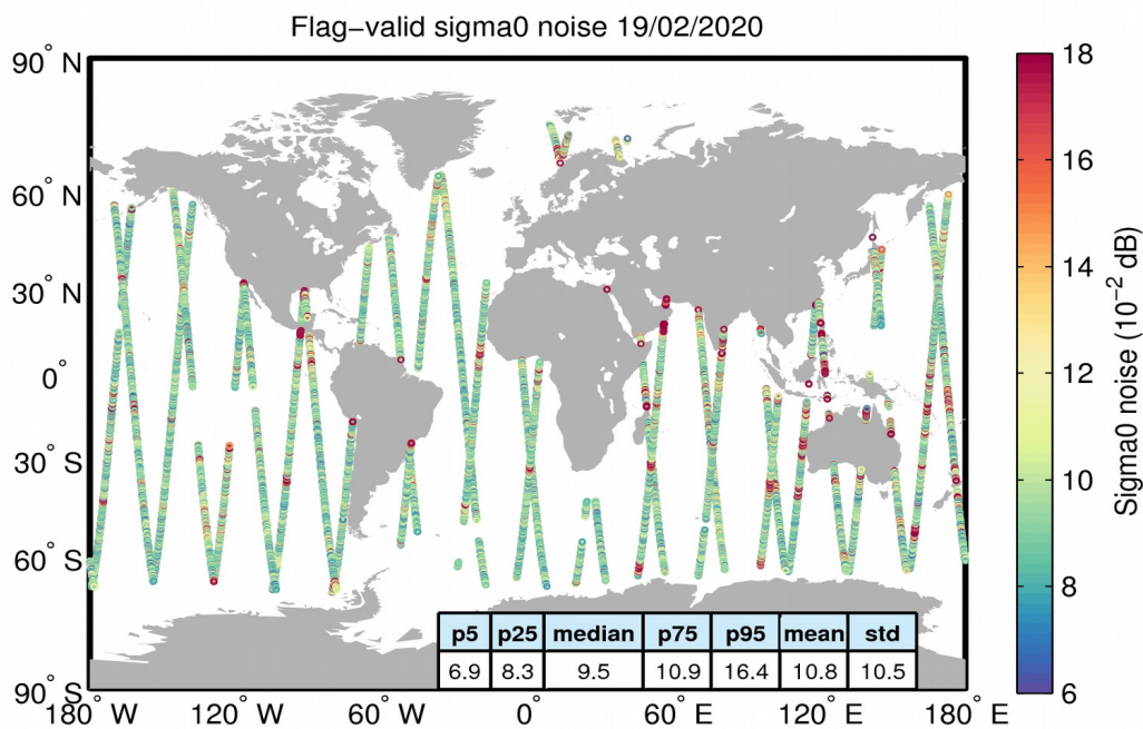
Figure 26. Geographical distribution of flag-valid 20-Hz sigma0 measurement noise over oceans and lakes for 19/02/2020. The statistical values shown in the table refer to the sigma0 noise and are calculated over all measurements shown in the figure.
