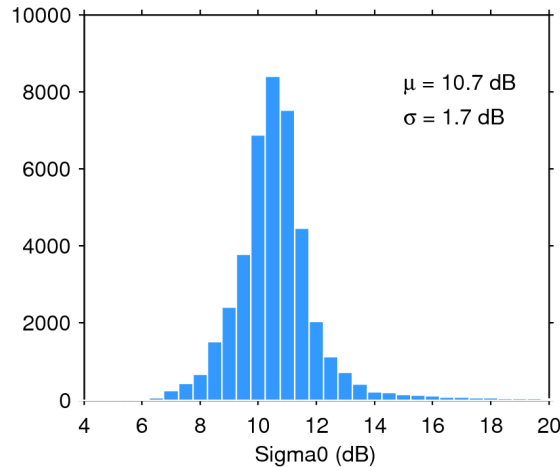
Figure 25. Histogram of flag-valid sigma0 over oceans and lakes for 19/02/2020. The mean ( \mu ) and standard deviation ( \sigma ) are also shown. Note that values outside [4 20] dB are excluded from the histogram for the sake of readability but not from the computation of \mu and \sigma .
