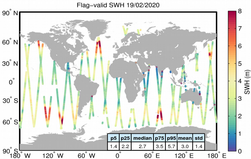
Figure 15. Geographical distribution of flag-valid SWH data over oceans and lakes for 19/02/2020. The statistical values shown in the table refer to the SWH in m and are calculated over all measurements shown in the figure.
