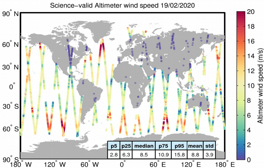
Figure 34. Geographical distribution of science-valid wind data over oceans and lakes for 19/02/2020. The statistical values shown in the table refer to the wind in m/s and are calculated over all measurements shown in the figure. Gray circles denote records that have been rejected based on the editing criteria described in Table 5.
