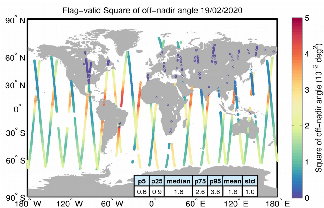
Figure 37. Geographical distribution of flag-valid mispointing data over oceans and lakes for 19/02/2020. The statistical values shown in the table refer to the mispointing in 10^{-2} deg 2 and are calculated over all measurements shown in the figure.
