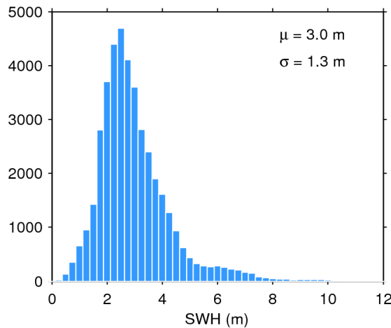
Figure 20. Histogram of science-valid SWH over oceans and lakes for 19/02/2020. The mean ( \mu ) and standard deviation ( \sigma ) are also shown. Note that values larger than 12 m are excluded from the histogram for the sake of readability but not from the computation of \mu and \sigma .
