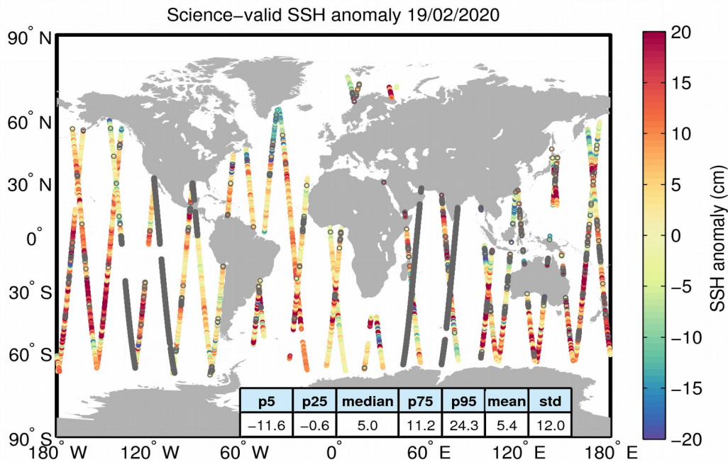
Figure 10. Geographical distribution of science-valid SSH anomaly data over oceans and lakes for 19/02/2020. The statistical values shown in the table refer to the SSH anomaly in cm and are calculated over all measurements shown in the figure. Gray circles denote records that have been rejected based on the editing criteria described in Table 2.
