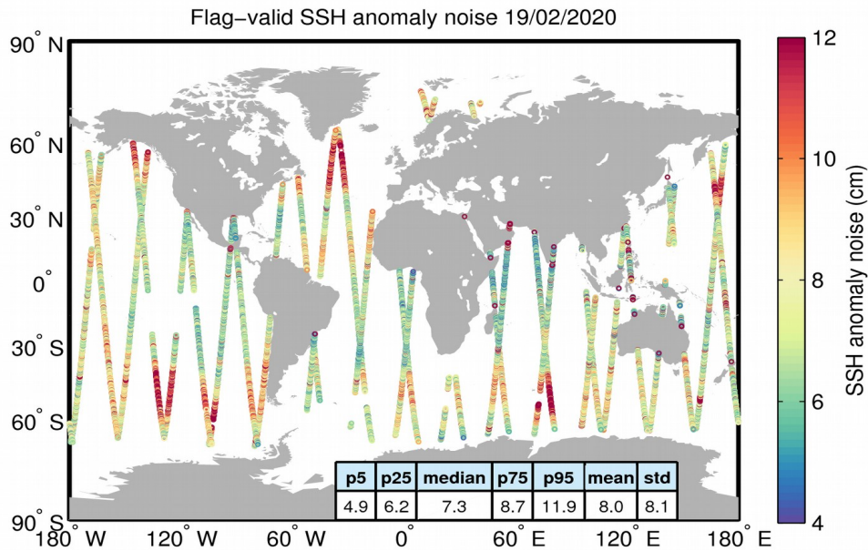
Figure 8. Geographical distribution of flag-valid 20-Hz SSH anomaly measurement noise over oceans and lakes for 19/02/2020. The statistical values shown in the table refer to the SSH anomaly noise and are calculated over all measurements shown in the figure.
