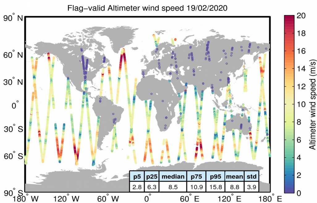
Figure 31. Geographical distribution of flag-valid wind data over oceans and lakes for 19/02/2020. The statistical values shown in the table refer to the wind in m/s and are calculated over all measurements shown in the figure.
