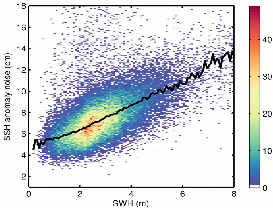
Figure 9. 2D histogram showing flag-valid SSH anomaly noise as a function of SWH for 18/02/2020. The black line denotes the median SSH anomaly noise as a function of SWH.
