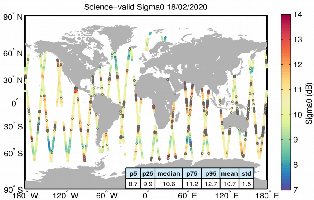
Figure 27. Geographical distribution of science-valid sigma0 data over oceans and lakes for 18/02/2020. The statistical values shown in the table refer to the sigma0 in dB and are calculated over all measurements shown in the figure. Gray circles denote records that have been rejected based on the editing criteria described in Table 4.
