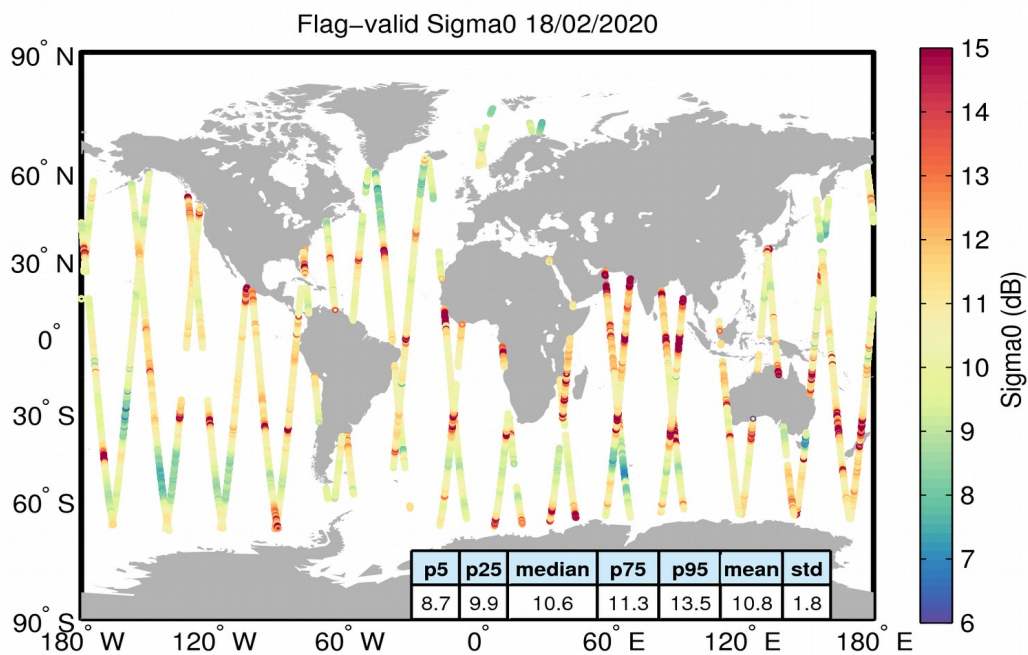
Figure 23. Geographical distribution of flag-valid sigma0 data over oceans and lakes for 18/02/2020. The statistical values shown in the table refer to the sigma0 in dB and are calculated over all measurements shown in the figure.
