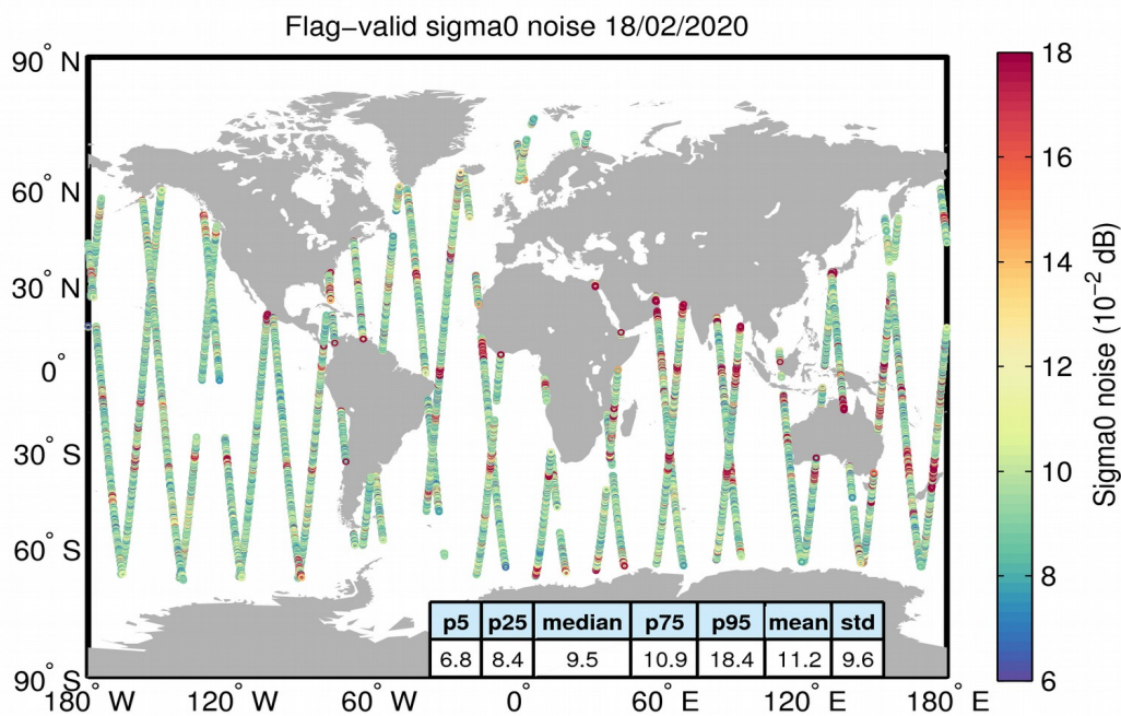
Figure 26. Geographical distribution of flag-valid 20-Hz sigma0 measurement noise over oceans and lakes for 18/02/2020. The statistical values shown in the table refer to the sigma0 noise and are calculated over all measurements shown in the figure.
