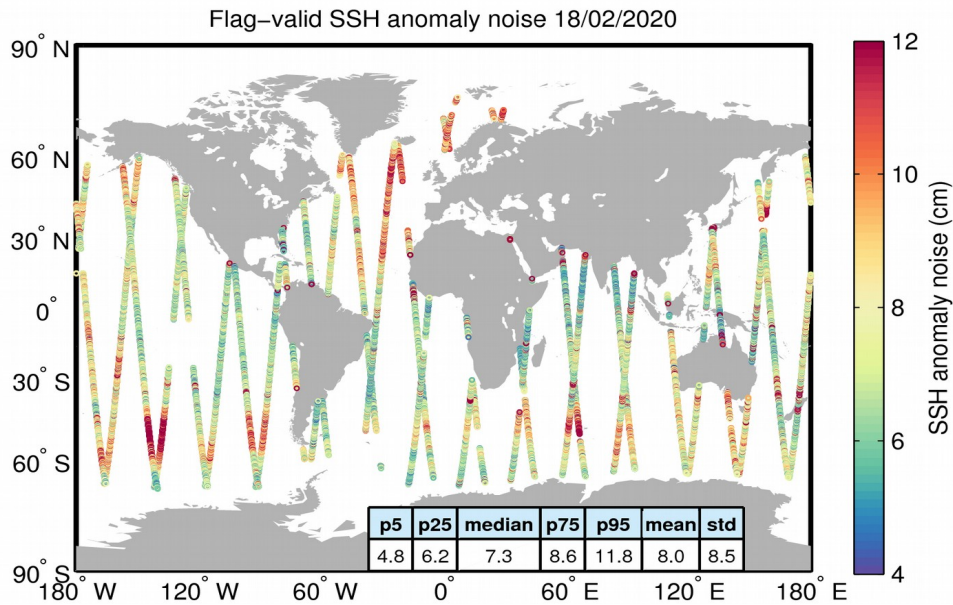
Figure 8. Geographical distribution of flag-valid 20-Hz SSH anomaly measurement noise over oceans and lakes for 18/02/2020. The statistical values shown in the table refer to the SSH anomaly noise and are calculated over all measurements shown in the figure.
