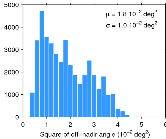
Figure 39. Histogram of flag-valid mispointing over oceans and lakes for 18/02/2020. The mean ( \mu ) and standard deviation ( \sigma ) are also shown. Note that values larger than 6 \cdot 10^{-2} \text{ deg}^2 are excluded from the histogram for the sake of readability but not from the computation of \mu and \sigma .
