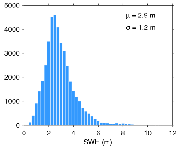
Figure 20. Histogram of science-valid SWH over oceans and lakes for 18/02/2020. The mean ( \mu ) and standard deviation ( \sigma ) are also shown. Note that values larger than 12 m are excluded from the histogram for the sake of readability but not from the computation of \mu and \sigma .
