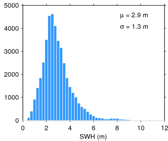
Figure 17. Histogram of flag-valid SWH over oceans and lakes for 18/02/2020. The mean ( \mu ) and standard deviation ( \sigma ) are also shown. Note that values larger than 12 m are excluded from the histogram for the sake of readability but not from the computation of \mu and \sigma .
