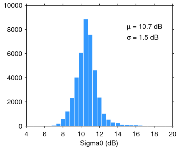
Figure 28. Histogram of science-valid sigma0 over oceans and lakes for 18/02/2020. The mean ( \mu ) and standard deviation ( \sigma ) are also shown. Note that values outside [4 20] dB are excluded from the histogram for the sake of readability but not from the computation of \mu and \sigma .
