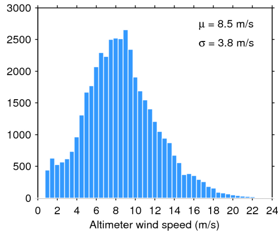
Figure 33. Histogram of flag-valid wind over oceans and lakes for 18/02/2020. The mean ( \mu ) and standard deviation ( \sigma ) are also shown. Note that values larger than 24 m/s are excluded from the histogram for the sake of readability but not from the computation of \mu and \sigma .
