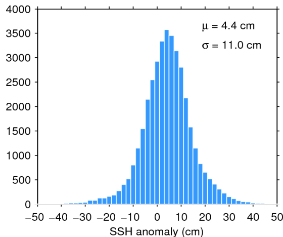
Figure 11. Histogram of science-valid SSH anomaly over oceans and lakes for 18/02/2020. The mean ( \mu ) and standard deviation ( \sigma ) are also shown. Note that values outside [-50 50] cm are excluded from the histogram for the sake of readability but not from the computation of \mu and \sigma .
