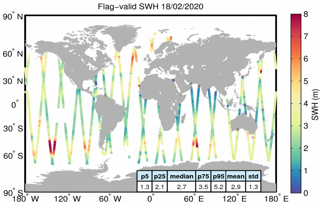
Figure 15. Geographical distribution of flag-valid SWH data over oceans and lakes for 18/02/2020. The statistical values shown in the table refer to the SWH in m and are calculated over all measurements shown in the figure.
