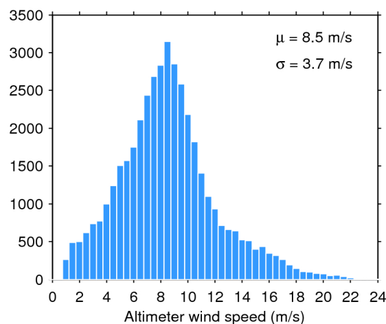
Figure 35. Histogram of science-valid wind over oceans and lakes for 17/02/2020. The mean ( \mu ) and standard deviation ( \sigma ) are also shown. Note that values larger than 24 m/s are excluded from the histogram for the sake of readability but not from the computation of \mu and \sigma .
