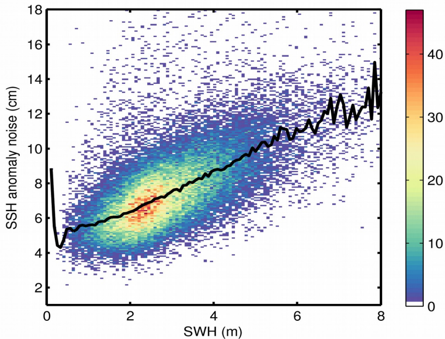
Figure 9. 2D histogram showing flag-valid SSH anomaly noise as a function of SWH for 17/02/2020. The black line denotes the median SSH anomaly noise as a function of SWH.
