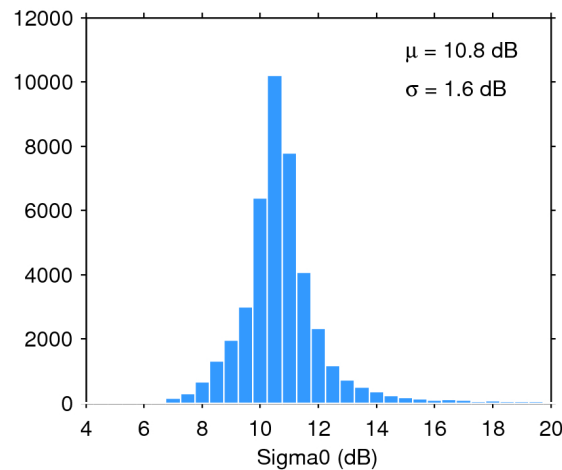
Figure 25. Histogram of flag-valid sigma0 over oceans and lakes for 17/02/2020. The mean ( \mu ) and standard deviation ( \sigma ) are also shown. Note that values outside [4 20] dB are excluded from the histogram for the sake of readability but not from the computation of \mu and \sigma .
