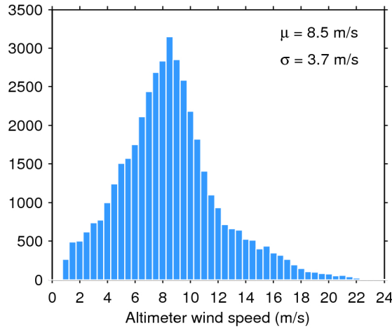
Figure 33. Histogram of flag-valid wind over oceans and lakes for 17/02/2020. The mean ( \mu ) and standard deviation ( \sigma ) are also shown. Note that values larger than 24 m/s are excluded from the histogram for the sake of readability but not from the computation of \mu and \sigma .
