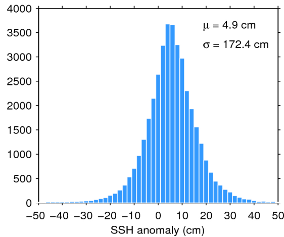
Figure 7. Histogram of flag-valid SSH anomaly over oceans and lakes for 17/02/2020. The mean ( \mu ) and standard deviation ( \sigma ) are also shown. Note that values outside [-50 50] cm are excluded from the histogram for the sake of readability but not from the computation of \mu and \sigma .
