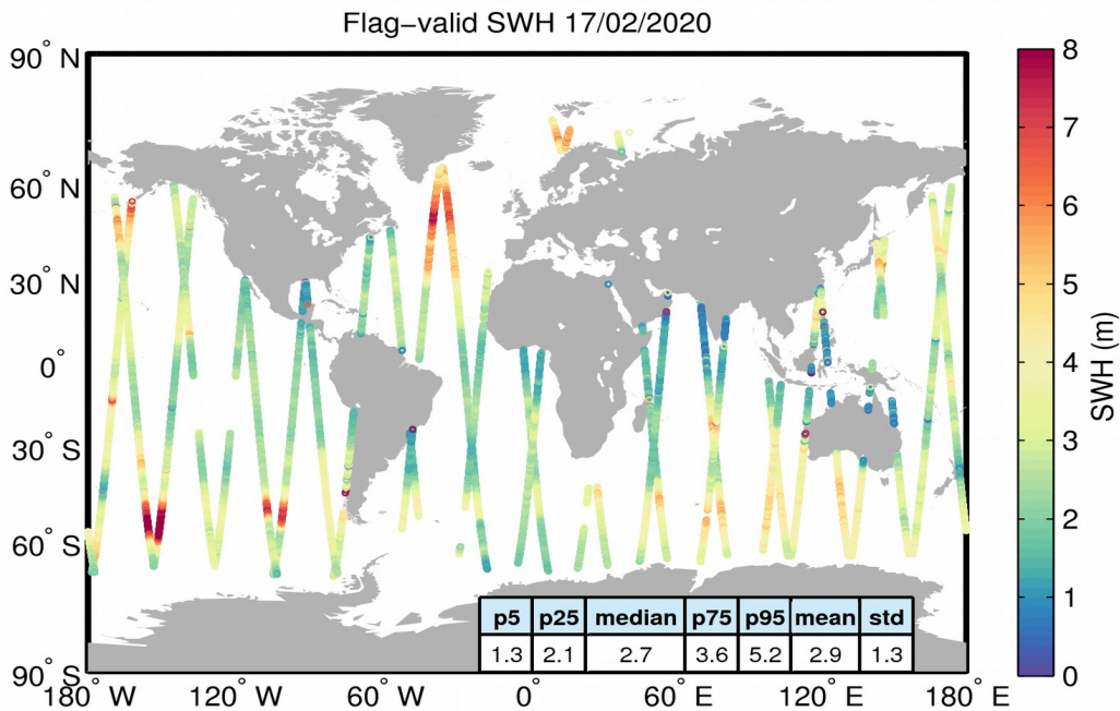
Figure 15. Geographical distribution of flag-valid SWH data over oceans and lakes for 17/02/2020. The statistical values shown in the table refer to the SWH in m and are calculated over all measurements shown in the figure.
