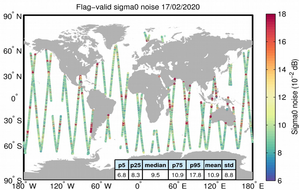
Figure 26. Geographical distribution of flag-valid 20-Hz sigma0 measurement noise over oceans and lakes for 17/02/2020. The statistical values shown in the table refer to the sigma0 noise and are calculated over all measurements shown in the figure.
