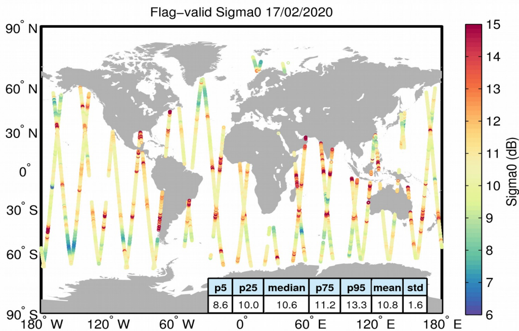
Figure 23. Geographical distribution of flag-valid sigma0 data over oceans and lakes for 17/02/2020. The statistical values shown in the table refer to the sigma0 in dB and are calculated over all measurements shown in the figure.
