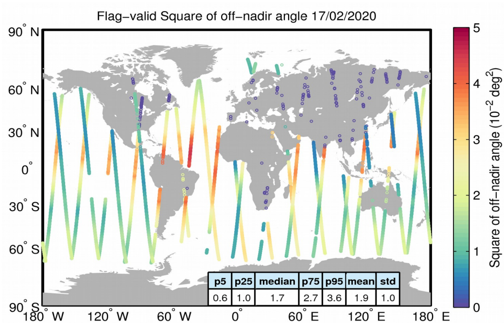
Figure 37. Geographical distribution of flag-valid mispointing data over oceans and lakes for 17/02/2020. The statistical values shown in the table refer to the mispointing in 10^{-2} \text{ deg}^2 and are calculated over all measurements shown in the figure.
