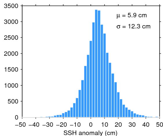
Figure 11. Histogram of science-valid SSH anomaly over oceans and lakes for 17/02/2020. The mean ( \mu ) and standard deviation ( \sigma ) are also shown. Note that values outside [-50 50] cm are excluded from the histogram for the sake of readability but not from the computation of \mu and \sigma .
