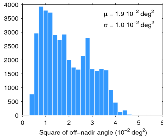
Figure 39. Histogram of flag-valid mispointing over oceans and lakes for 17/02/2020. The mean ( \mu ) and standard deviation ( \sigma ) are also shown. Note that values larger than 6 \cdot 10^{-2} \text{ deg}^2 are excluded from the histogram for the sake of readability but not from the computation of \mu and \sigma .
