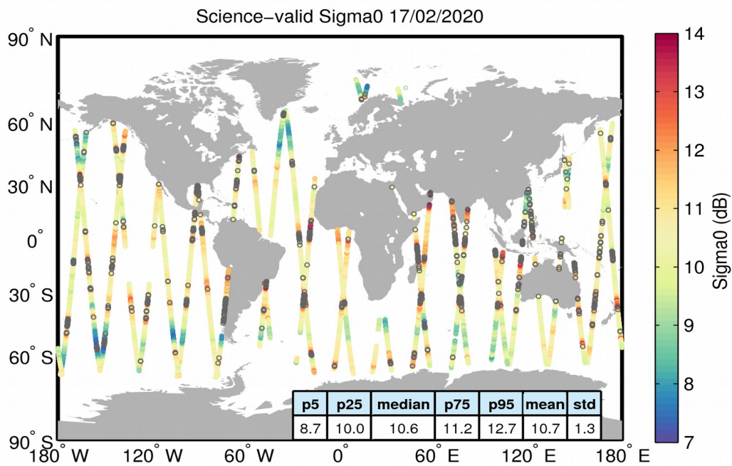
Figure 27. Geographical distribution of science-valid sigma0 data over oceans and lakes for 17/02/2020. The statistical values shown in the table refer to the sigma0 in dB and are calculated over all measurements shown in the figure. Gray circles denote records that have been rejected based on the editing criteria described in Table 4.
