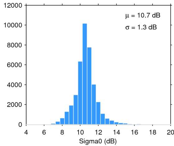
Figure 28. Histogram of science-valid sigma0 over oceans and lakes for 17/02/2020. The mean ( \mu ) and standard deviation ( \sigma ) are also shown. Note that values outside [4 20] dB are excluded from the histogram for the sake of readability but not from the computation of \mu and \sigma .
