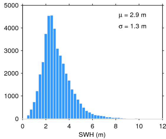
Figure 17. Histogram of flag-valid SWH over oceans and lakes for 17/02/2020. The mean ( \mu ) and standard deviation ( \sigma ) are also shown. Note that values larger than 12 m are excluded from the histogram for the sake of readability but not from the computation of \mu and \sigma .
