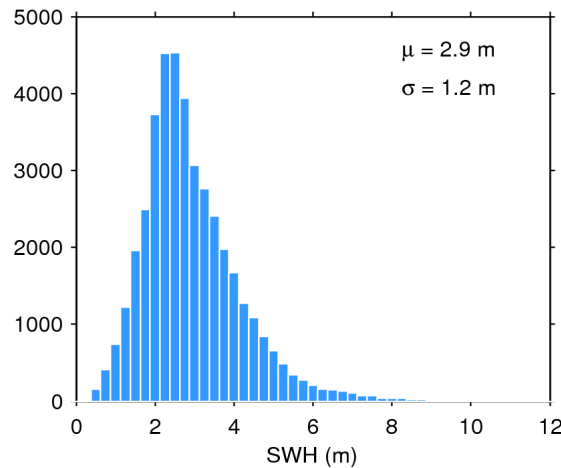
Figure 20. Histogram of science-valid SWH over oceans and lakes for 17/02/2020. The mean ( \mu ) and standard deviation ( \sigma ) are also shown. Note that values larger than 12 m are excluded from the histogram for the sake of readability but not from the computation of \mu and \sigma .
