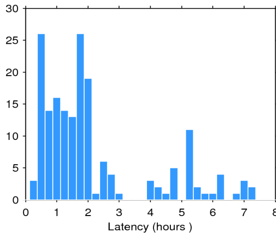
Figure 2. Histogram of the data latency for 16/02/2020. The y-axis denotes the number of files that are made available with a delay of x-hours with respect to the mean time of the records stored in the file.
