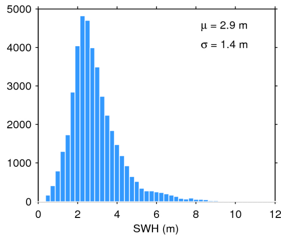
Figure 17. Histogram of flag-valid SWH over oceans and lakes for 16/02/2020. The mean ( \mu ) and standard deviation ( \sigma ) are also shown. Note that values larger than 12 m are excluded from the histogram for the sake of readability but not from the computation of \mu and \sigma .
