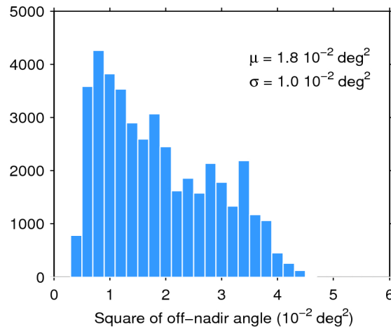
Figure 39. Histogram of flag-valid mispointing over oceans and lakes for 16/02/2020. The mean ( \mu ) and standard deviation ( \sigma ) are also shown. Note that values larger than 6 \cdot 10^{-2} \text{ deg}^2 are excluded from the histogram for the sake of readability but not from the computation of \mu and \sigma .
