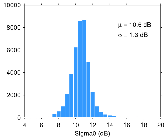
Figure 28. Histogram of science-valid sigma0 over oceans and lakes for 16/02/2020. The mean ( \mu ) and standard deviation ( \sigma ) are also shown. Note that values outside [4 20] dB are excluded from the histogram for the sake of readability but not from the computation of \mu and \sigma .
