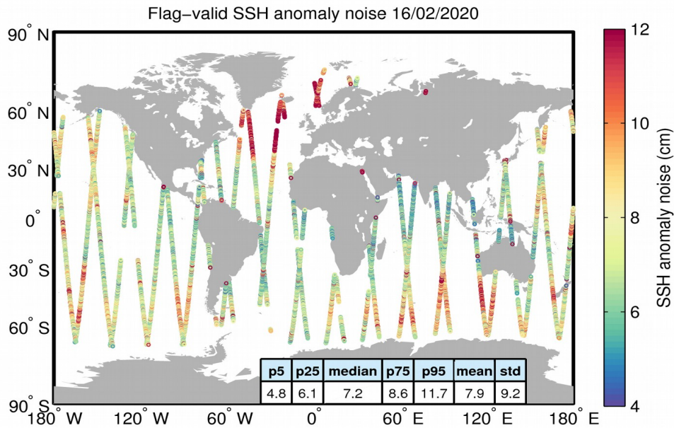
Figure 8. Geographical distribution of flag-valid 20-Hz SSH anomaly measurement noise over oceans and lakes for 16/02/2020. The statistical values shown in the table refer to the SSH anomaly noise and are calculated over all measurements shown in the figure.
