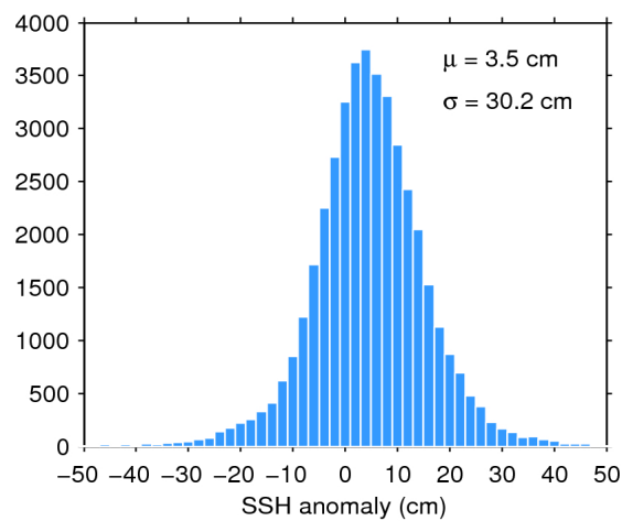
Figure 7. Histogram of flag-valid SSH anomaly over oceans and lakes for 16/02/2020. The mean ( \mu ) and standard deviation ( \sigma ) are also shown. Note that values outside [-50 50] cm are excluded from the histogram for the sake of readability but not from the computation of \mu and \sigma .
