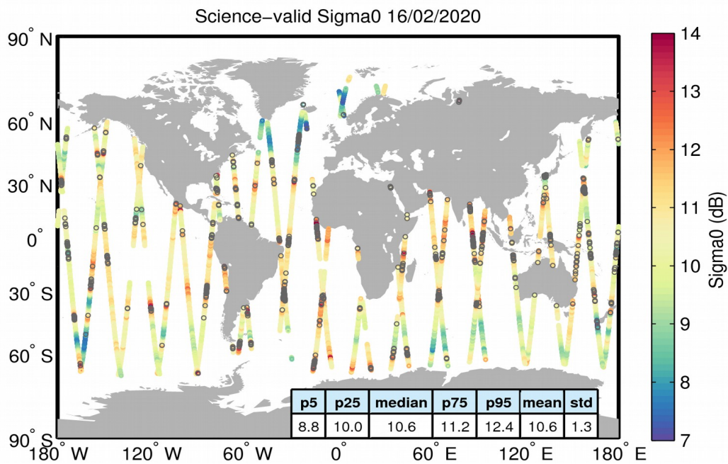
Figure 27. Geographical distribution of science-valid sigma0 data over oceans and lakes for 16/02/2020. The statistical values shown in the table refer to the sigma0 in dB and are calculated over all measurements shown in the figure. Gray circles denote records that have been rejected based on the editing criteria described in Table 4.
