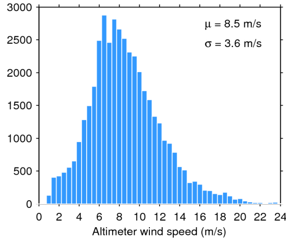
Figure 33. Histogram of flag-valid wind over oceans and lakes for 16/02/2020. The mean ( \mu ) and standard deviation ( \sigma ) are also shown. Note that values larger than 24 m/s are excluded from the histogram for the sake of readability but not from the computation of \mu and \sigma .
