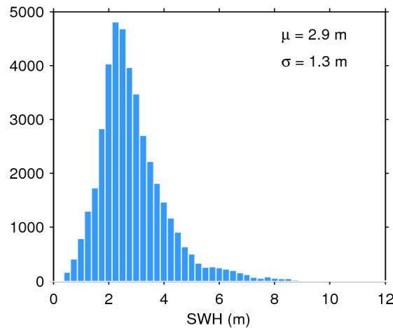
Figure 20. Histogram of science-valid SWH over oceans and lakes for 16/02/2020. The mean ( \mu ) and standard deviation ( \sigma ) are also shown. Note that values larger than 12 m are excluded from the histogram for the sake of readability but not from the computation of \mu and \sigma .
