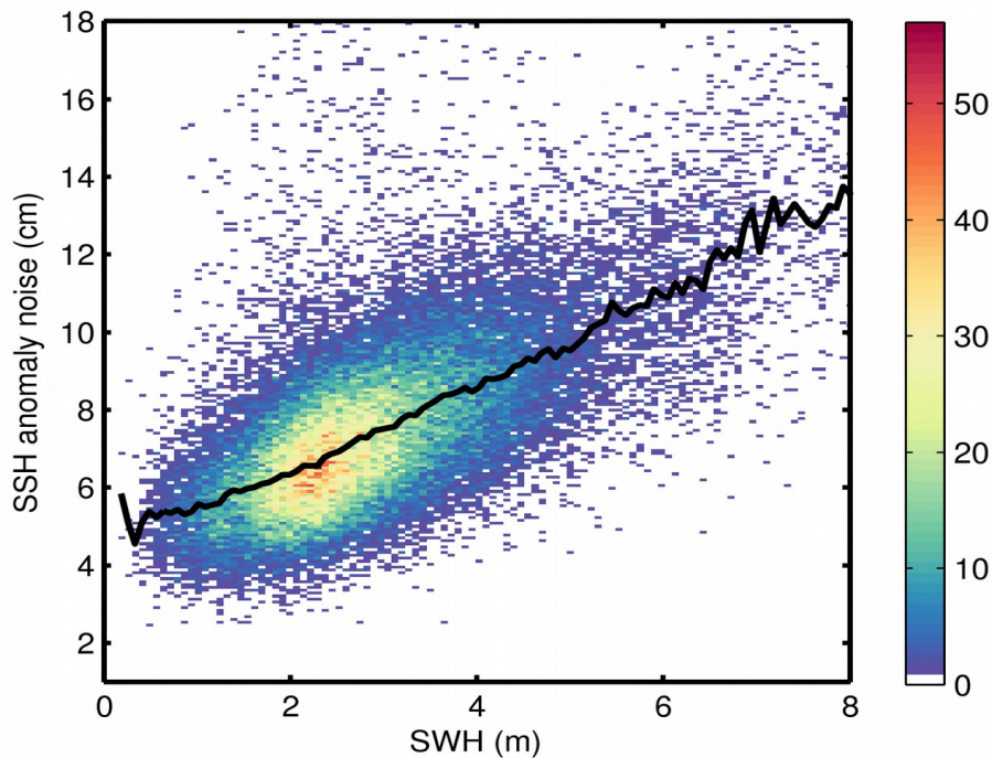
Figure 9. 2D histogram showing flag-valid SSH anomaly noise as a function of SWH for 16/02/2020. The black line denotes the median SSH anomaly noise as a function of SWH.
