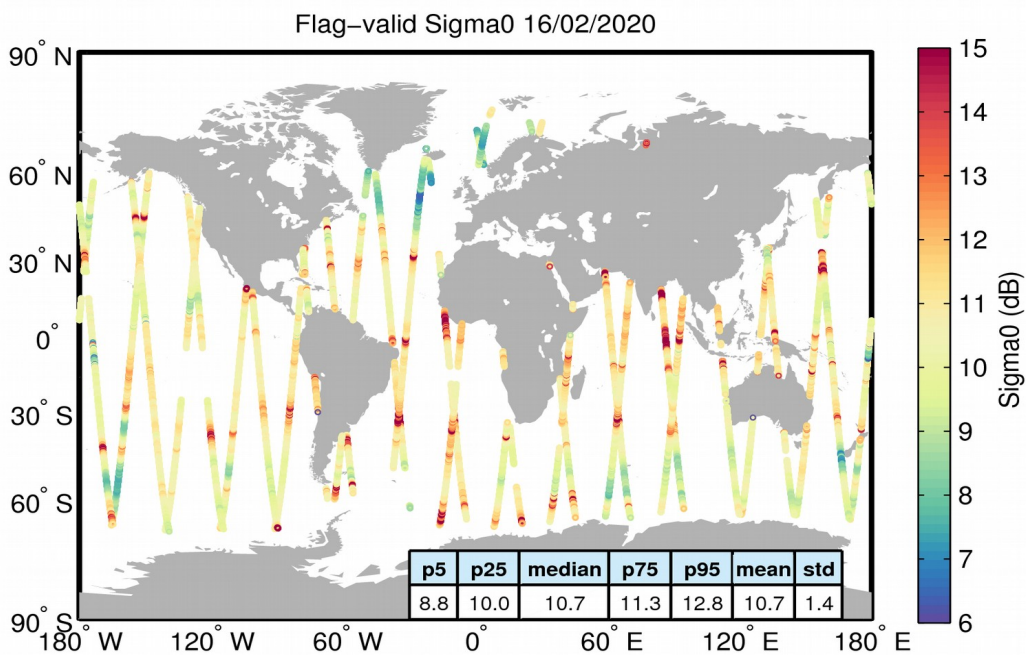
Figure 23. Geographical distribution of flag-valid sigma0 data over oceans and lakes for 16/02/2020. The statistical values shown in the table refer to the sigma0 in dB and are calculated over all measurements shown in the figure.
