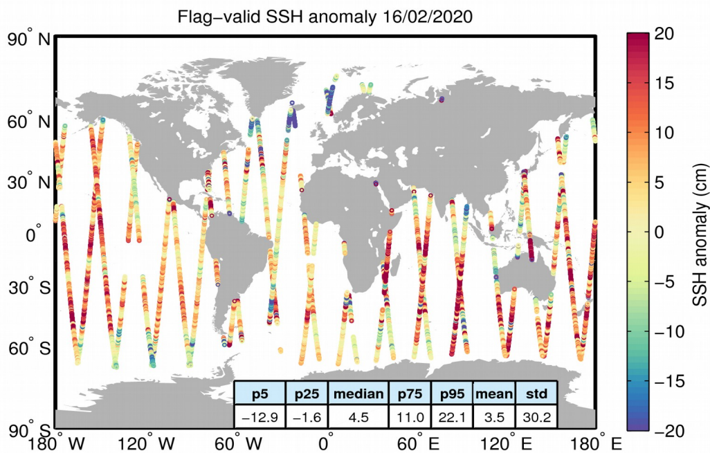
Figure 5. Geographical distribution of flag-valid 1-Hz SSH anomaly data over oceans and lakes for 16/02/2020. The statistical values shown in the table refer to the SSH anomaly in cm and are calculated over all measurements shown in the figure.
