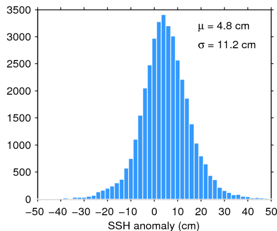
Figure 11. Histogram of science-valid SSH anomaly over oceans and lakes for 16/02/2020. The mean ( \mu ) and standard deviation ( \sigma ) are also shown. Note that values outside [-50 50] cm are excluded from the histogram for the sake of readability but not from the computation of \mu and \sigma .
