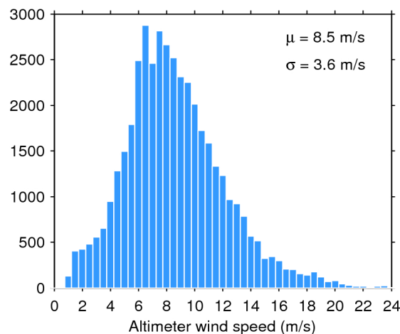
Figure 35. Histogram of science-valid wind over oceans and lakes for 16/02/2020. The mean ( \mu ) and standard deviation ( \sigma ) are also shown. Note that values larger than 24 m/s are excluded from the histogram for the sake of readability but not from the computation of \mu and \sigma .
