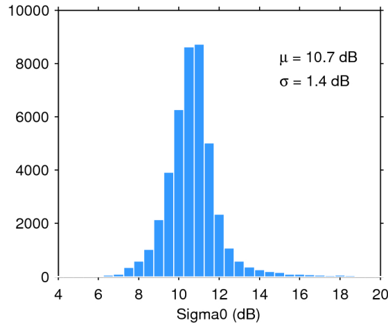
Figure 25. Histogram of flag-valid sigma0 over oceans and lakes for 16/02/2020. The mean ( \mu ) and standard deviation ( \sigma ) are also shown. Note that values outside [4 20] dB are excluded from the histogram for the sake of readability but not from the computation of \mu and \sigma .
