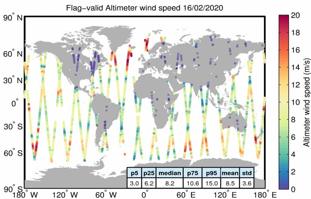
Figure 31. Geographical distribution of flag-valid wind data over oceans and lakes for 16/02/2020. The statistical values shown in the table refer to the wind in m/s and are calculated over all measurements shown in the figure.
