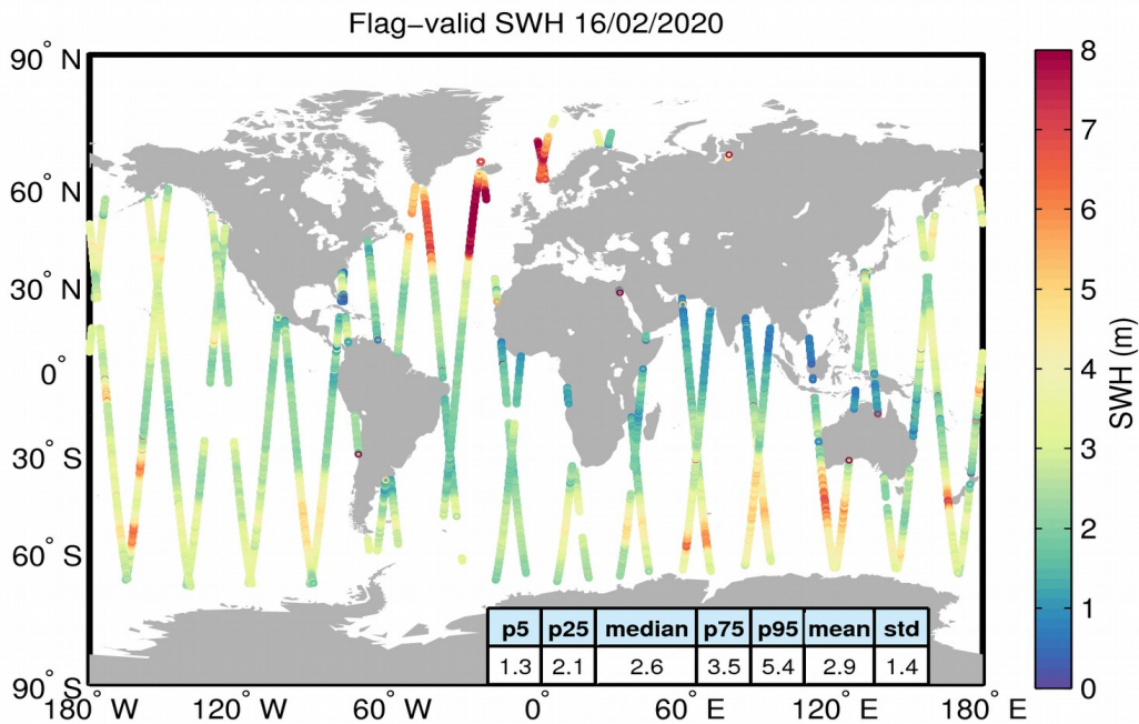
Figure 15. Geographical distribution of flag-valid SWH data over oceans and lakes for 16/02/2020. The statistical values shown in the table refer to the SWH in m and are calculated over all measurements shown in the figure.
