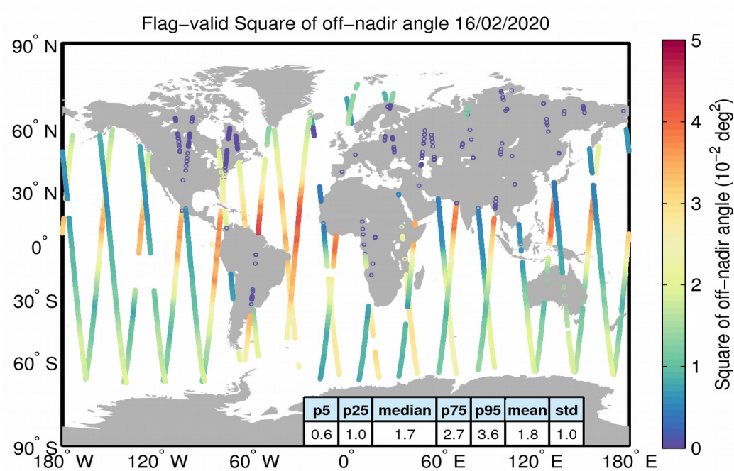
Figure 37. Geographical distribution of flag-valid mispointing data over oceans and lakes for 16/02/2020. The statistical values shown in the table refer to the mispointing in 10^{-2} deg 2 and are calculated over all measurements shown in the figure.
