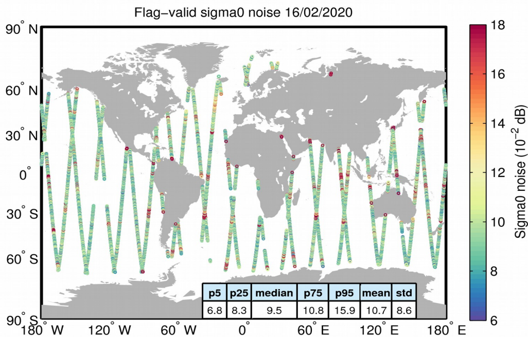
Figure 26. Geographical distribution of flag-valid 20-Hz sigma0 measurement noise over oceans and lakes for 16/02/2020. The statistical values shown in the table refer to the sigma0 noise and are calculated over all measurements shown in the figure.
