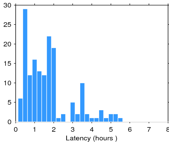
Figure 2. Histogram of the data latency for 15/02/2020. The y-axis denotes the number of files that are made available with a delay of x-hours with respect to the mean time of the records stored in the file.
