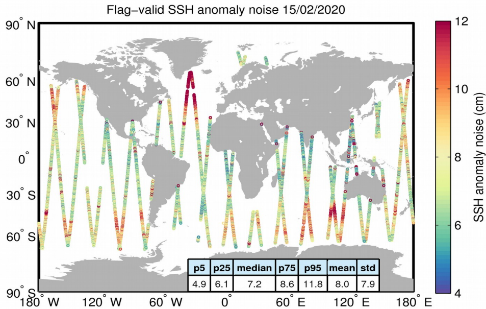
Figure 8. Geographical distribution of flag-valid 20-Hz SSH anomaly measurement noise over oceans and lakes for 15/02/2020. The statistical values shown in the table refer to the SSH anomaly noise and are calculated over all measurements shown in the figure.
