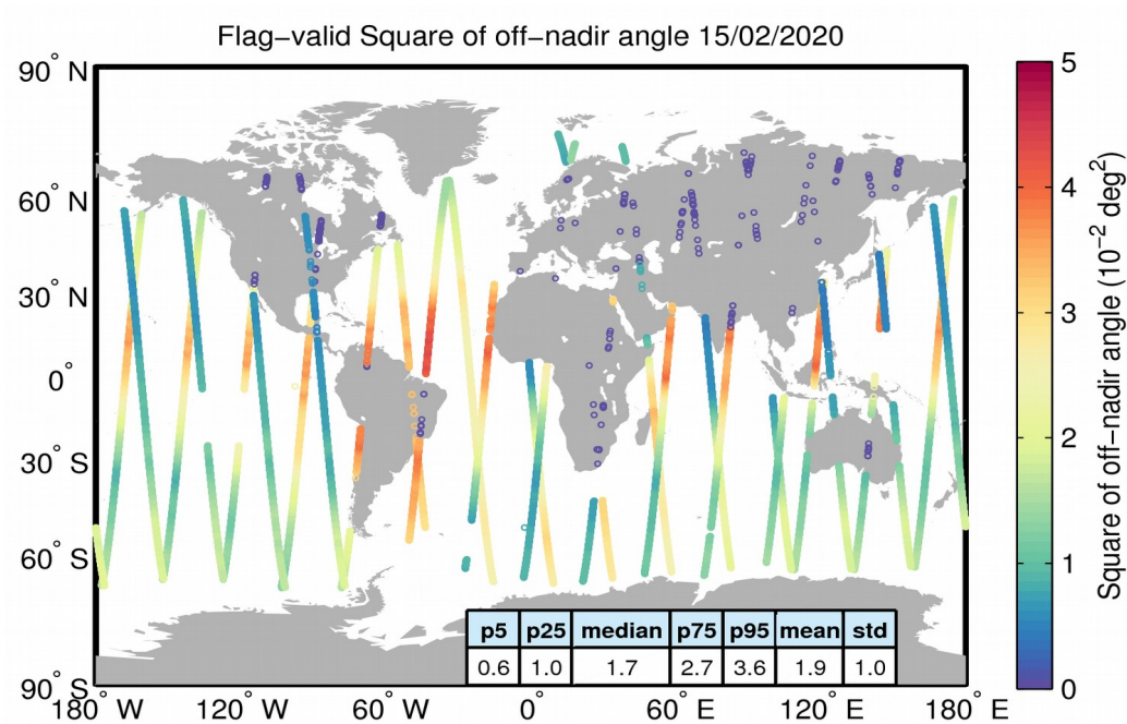
Figure 37. Geographical distribution of flag-valid mispointing data over oceans and lakes for 15/02/2020. The statistical values shown in the table refer to the mispointing in 10^{-2} \text{ deg}^2 and are calculated over all measurements shown in the figure.
