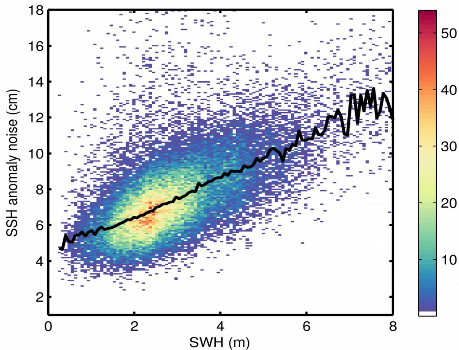
Figure 9. 2D histogram showing flag-valid SSH anomaly noise as a function of SWH for 15/02/2020. The black line denotes the median SSH anomaly noise as a function of SWH.
