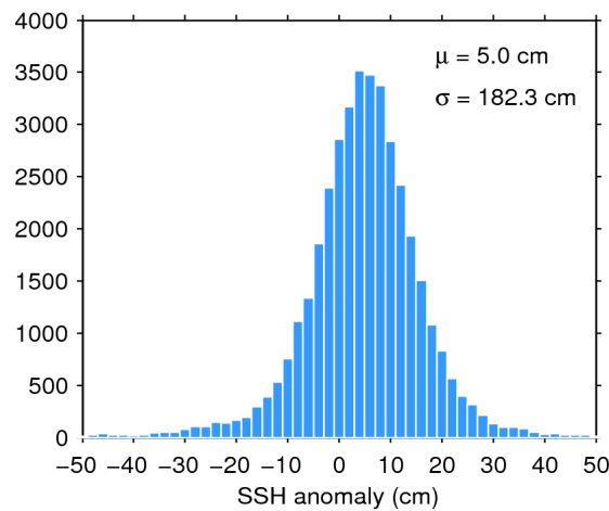
Figure 7. Histogram of flag-valid SSH anomaly over oceans and lakes for 15/02/2020. The mean ( \mu ) and standard deviation ( \sigma ) are also shown. Note that values outside [-50 50] cm are excluded from the histogram for the sake of readability but not from the computation of \mu and \sigma .
