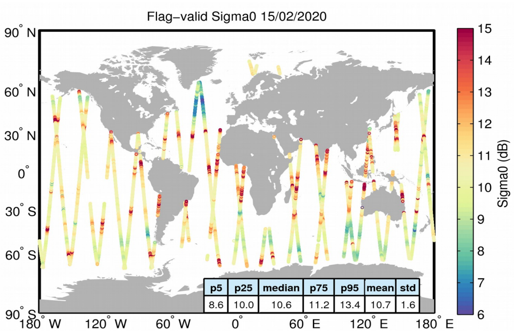
Figure 23. Geographical distribution of flag-valid sigma0 data over oceans and lakes for 15/02/2020. The statistical values shown in the table refer to the sigma0 in dB and are calculated over all measurements shown in the figure.
