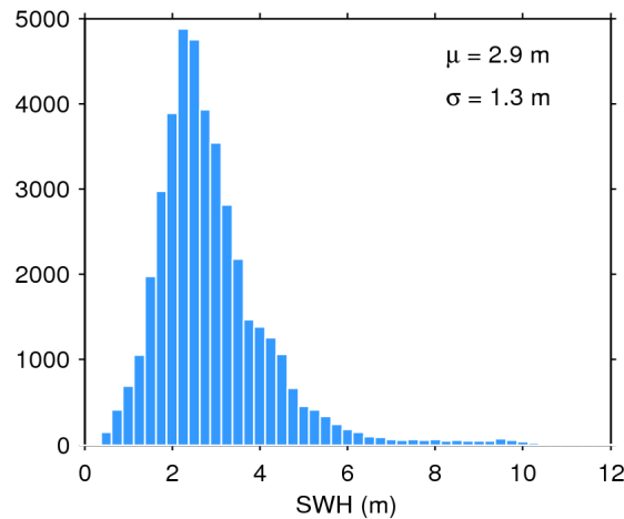
Figure 20. Histogram of science-valid SWH over oceans and lakes for 15/02/2020. The mean ( \mu ) and standard deviation ( \sigma ) are also shown. Note that values larger than 12 m are excluded from the histogram for the sake of readability but not from the computation of \mu and \sigma .
