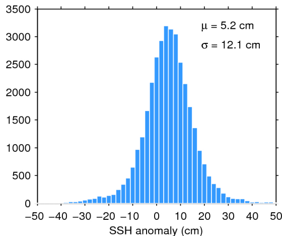
Figure 11. Histogram of science-valid SSH anomaly over oceans and lakes for 15/02/2020. The mean ( \mu ) and standard deviation ( \sigma ) are also shown. Note that values outside [-50 50] cm are excluded from the histogram for the sake of readability but not from the computation of \mu and \sigma .
