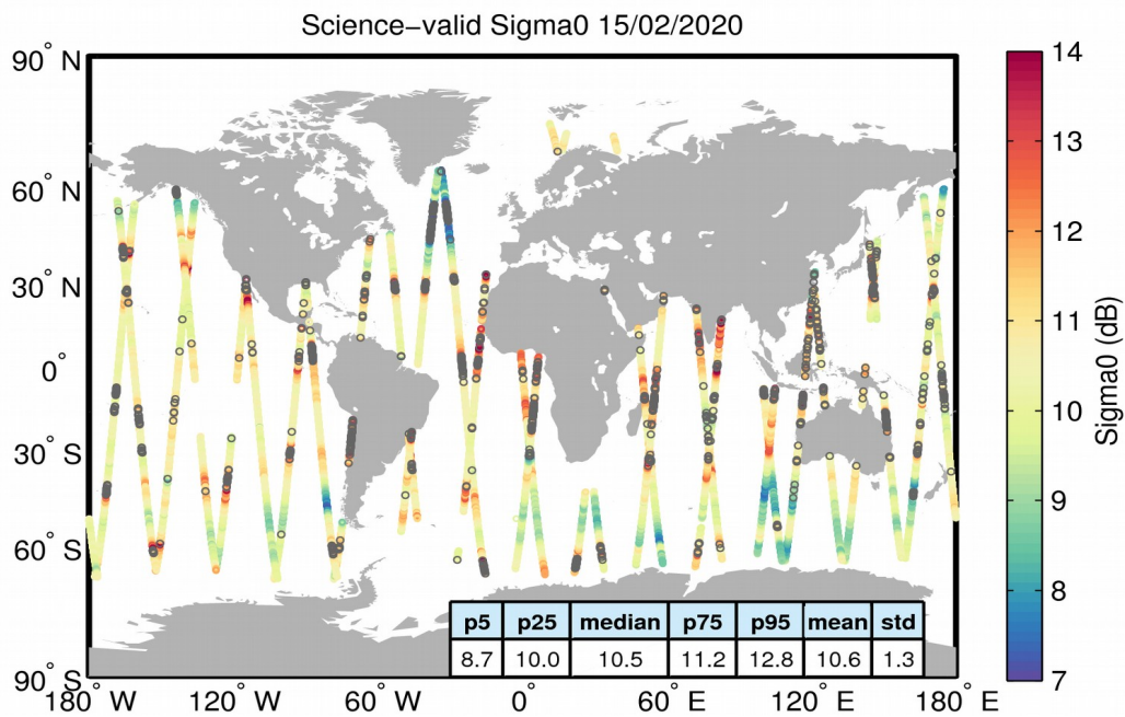
Figure 27. Geographical distribution of science-valid sigma0 data over oceans and lakes for 15/02/2020. The statistical values shown in the table refer to the sigma0 in dB and are calculated over all measurements shown in the figure. Gray circles denote records that have been rejected based on the editing criteria described in Table 4.
