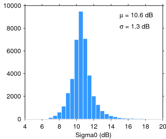
Figure 28. Histogram of science-valid sigma0 over oceans and lakes for 15/02/2020. The mean ( \mu ) and standard deviation ( \sigma ) are also shown. Note that values outside [4 20] dB are excluded from the histogram for the sake of readability but not from the computation of \mu and \sigma .
