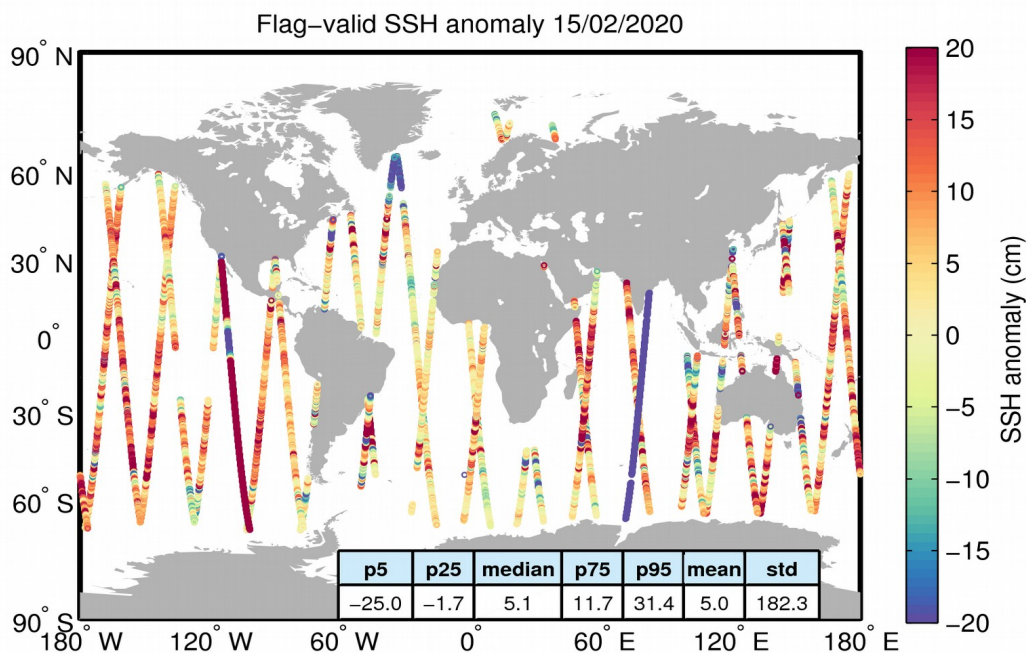
Figure 5. Geographical distribution of flag-valid 1-Hz SSH anomaly data over oceans and lakes for 15/02/2020. The statistical values shown in the table refer to the SSH anomaly in cm and are calculated over all measurements shown in the figure.
