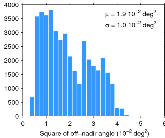
Figure 39. Histogram of flag-valid mispointing over oceans and lakes for 15/02/2020. The mean ( \mu ) and standard deviation ( \sigma ) are also shown. Note that values larger than 6 \cdot 10^{-2} \text{ deg}^2 are excluded from the histogram for the sake of readability but not from the computation of \mu and \sigma .
