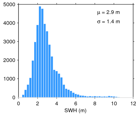
Figure 17. Histogram of flag-valid SWH over oceans and lakes for 15/02/2020. The mean ( \mu ) and standard deviation ( \sigma ) are also shown. Note that values larger than 12 m are excluded from the histogram for the sake of readability but not from the computation of \mu and \sigma .
