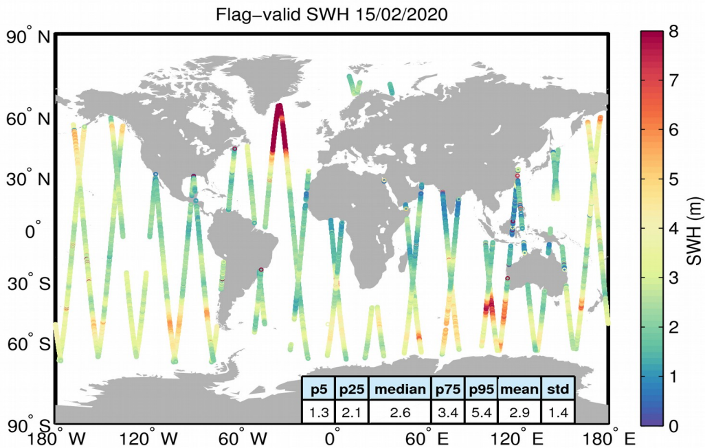
Figure 15. Geographical distribution of flag-valid SWH data over oceans and lakes for 15/02/2020. The statistical values shown in the table refer to the SWH in m and are calculated over all measurements shown in the figure.
