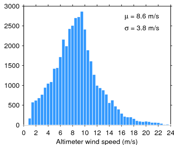
Figure 35. Histogram of science-valid wind over oceans and lakes for 15/02/2020. The mean ( \mu ) and standard deviation ( \sigma ) are also shown. Note that values larger than 24 m/s are excluded from the histogram for the sake of readability but not from the computation of \mu and \sigma .
