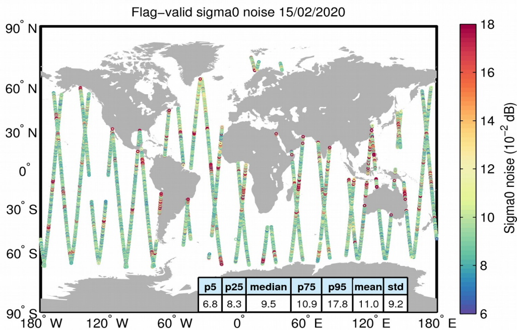
Figure 26. Geographical distribution of flag-valid 20-Hz sigma0 measurement noise over oceans and lakes for 15/02/2020. The statistical values shown in the figure refer to the sigma0 noise and are calculated over all measurements shown in the figure.
