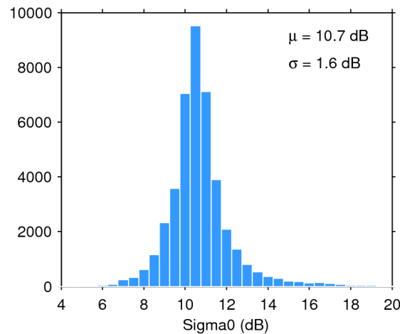
Figure 25. Histogram of flag-valid sigma0 over oceans and lakes for 15/02/2020. The mean ( \mu ) and standard deviation ( \sigma ) are also shown. Note that values outside [4 20] dB are excluded from the histogram for the sake of readability but not from the computation of \mu and \sigma .
