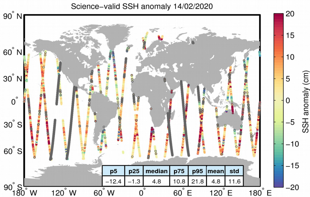
Figure 10. Geographical distribution of science-valid SSH anomaly data over oceans and lakes for 14/02/2020. The statistical values shown in the table refer to the SSH anomaly in cm and are calculated over all measurements shown in the figure. Gray circles denote records that have been rejected based on the editing criteria described in Table 2.
