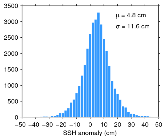
Figure 11. Histogram of science-valid SSH anomaly over oceans and lakes for 14/02/2020. The mean ( \mu ) and standard deviation ( \sigma ) are also shown. Note that values outside [-50 50] cm are excluded from the histogram for the sake of readability but not from the computation of \mu and \sigma .
