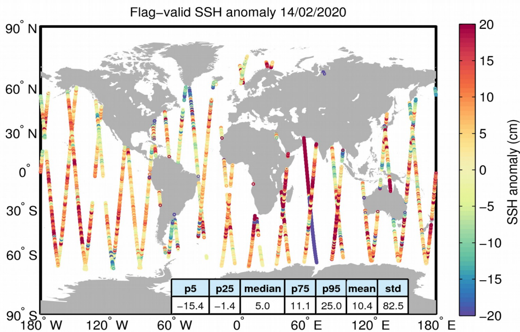
Figure 5. Geographical distribution of flag-valid 1-Hz SSH anomaly data over oceans and lakes for 14/02/2020. The statistical values shown in the table refer to the SSH anomaly in cm and are calculated over all measurements shown in the figure.
