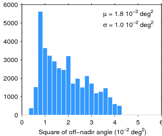
Figure 39. Histogram of flag-valid mispointing over oceans and lakes for 14/02/2020. The mean ( \mu ) and standard deviation ( \sigma ) are also shown. Note that values larger than 6 \cdot 10^{-2} \text{ deg}^2 are excluded from the histogram for the sake of readability but not from the computation of \mu and \sigma .
