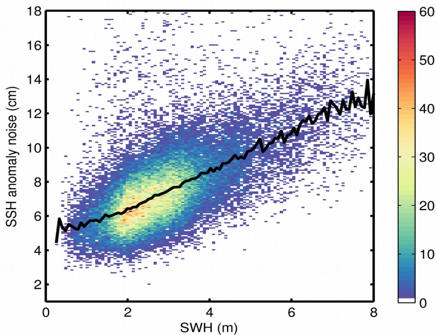
Figure 9. 2D histogram showing flag-valid SSH anomaly noise as a function of SWH for 14/02/2020. The black line denotes the median SSH anomaly noise as a function of SWH.
