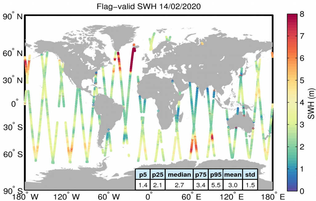
Figure 15. Geographical distribution of flag-valid SWH data over oceans and lakes for 14/02/2020. The statistical values shown in the table refer to the SWH in m and are calculated over all measurements shown in the figure.
