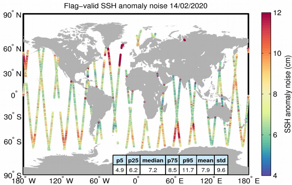
Figure 8. Geographical distribution of flag-valid 20-Hz SSH anomaly measurement noise over oceans and lakes for 14/02/2020. The statistical values shown in the table refer to the SSH anomaly noise and are calculated over all measurements shown in the figure.
