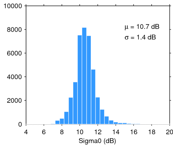
Figure 28. Histogram of science-valid sigma0 over oceans and lakes for 14/02/2020. The mean ( \mu ) and standard deviation ( \sigma ) are also shown. Note that values outside [4 20] dB are excluded from the histogram for the sake of readability but not from the computation of \mu and \sigma .
