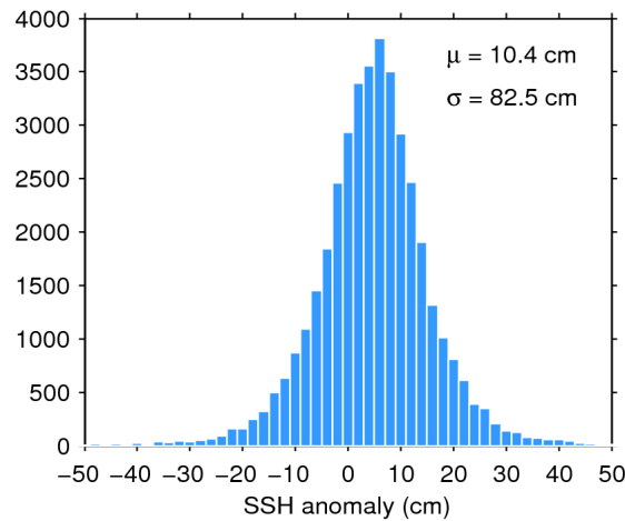
Figure 7. Histogram of flag-valid SSH anomaly over oceans and lakes for 14/02/2020. The mean ( \mu ) and standard deviation ( \sigma ) are also shown. Note that values outside [-50 50] cm are excluded from the histogram for the sake of readability but not from the computation of \mu and \sigma .
