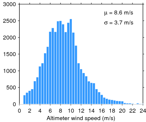
Figure 33. Histogram of flag-valid wind over oceans and lakes for 14/02/2020. The mean ( \mu ) and standard deviation ( \sigma ) are also shown. Note that values larger than 24 m/s are excluded from the histogram for the sake of readability but not from the computation of \mu and \sigma .
