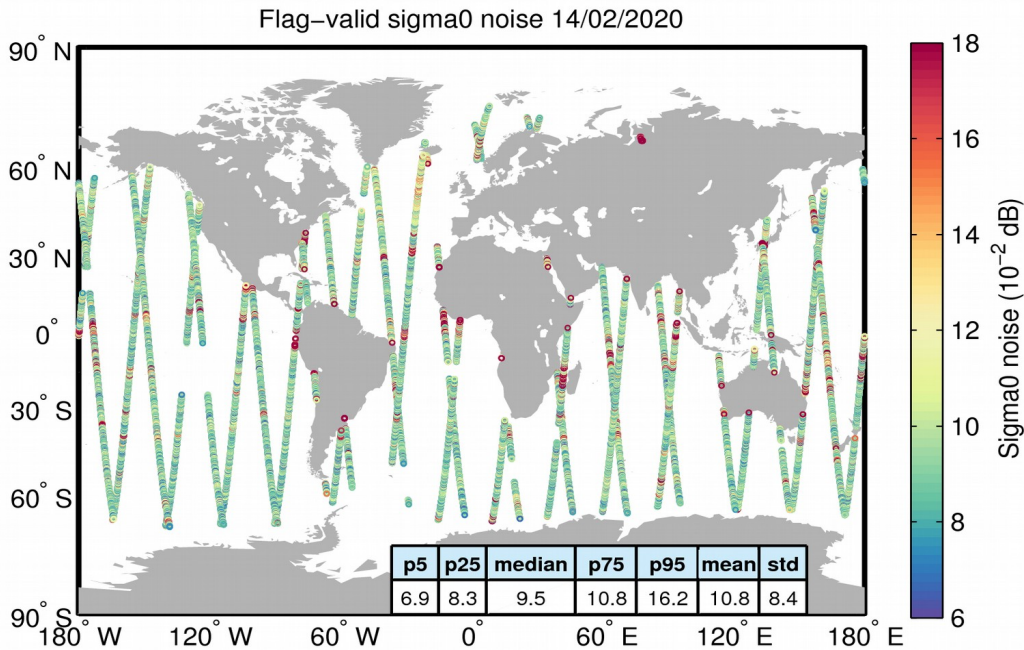
Figure 26. Geographical distribution of flag-valid 20-Hz sigma0 measurement noise over oceans and lakes for 14/02/2020. The statistical values shown in the table refer to the sigma0 noise and are calculated over all measurements shown in the figure.
