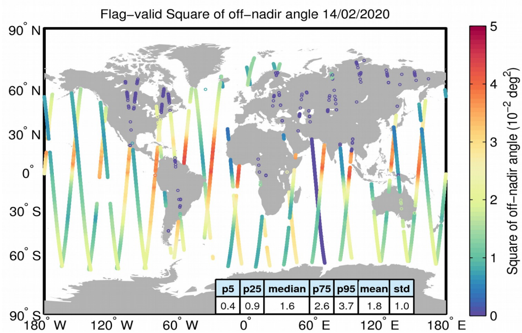
Figure 37. Geographical distribution of flag-valid mispointing data over oceans and lakes for 14/02/2020. The statistical values shown in the table refer to the mispointing in 10^{-2} \text{ deg}^2 and are calculated over all measurements shown in the figure.
