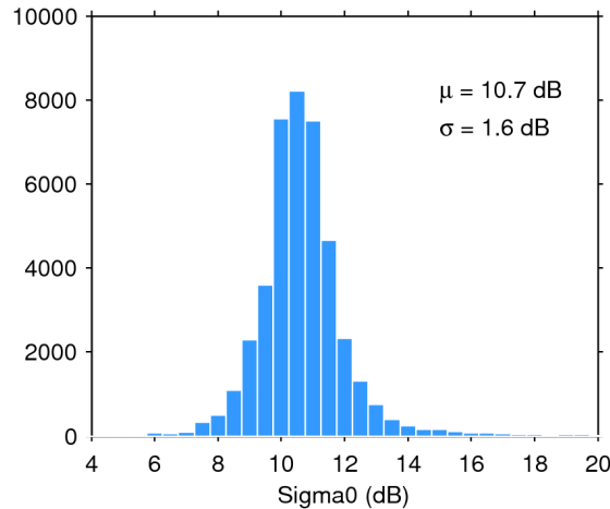
Figure 25. Histogram of flag-valid sigma0 over oceans and lakes for 14/02/2020. The mean ( \mu ) and standard deviation ( \sigma ) are also shown. Note that values outside [4 20] dB are excluded from the histogram for the sake of readability but not from the computation of \mu and \sigma .
