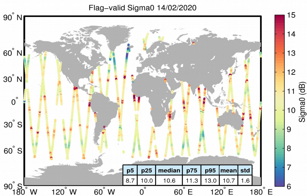
Figure 23. Geographical distribution of flag-valid sigma0 data over oceans and lakes for 14/02/2020. The statistical values shown in the table refer to the sigma0 in dB and are calculated over all measurements shown in the figure.
